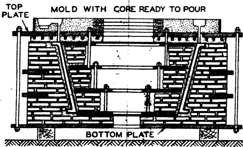
FIG. 33.—CONSTRUCTION OF LOAM MOLD
