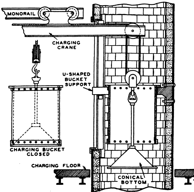
FIG. 67.—CHARGING BUCKET (WHITING DESIGN)
