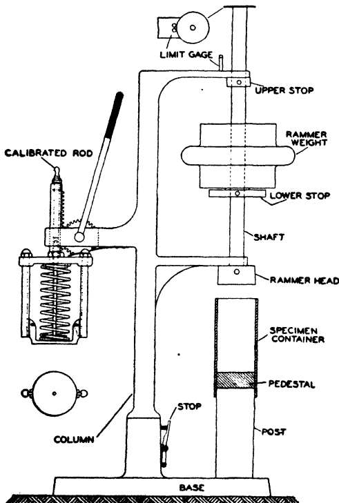
FIG. 170.—SAND RAMMER AND COMPRESSIVE-STRENGTH TESTER
