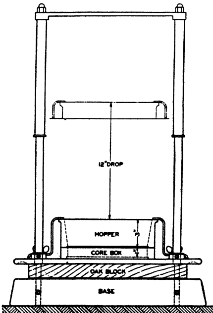
FIG. 172.—CORE-MAKING APPARATUS
