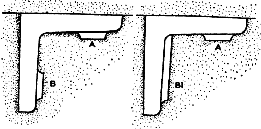
FIG. 153.—BOSSSES ON CASTING
