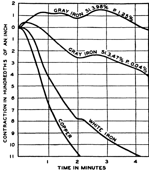
FIG. 146.—CONTRACTION CURVES
