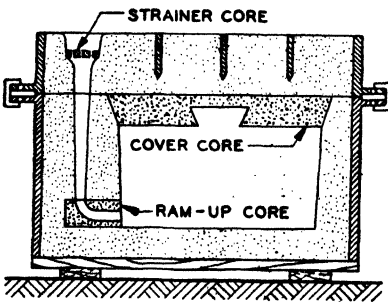
FIG. 53.—CORES IN MOLD
