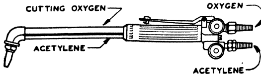
FIG. 83.—CUTTING TORCH
