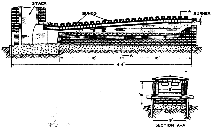
FIG. 73.—CROSS SECTION OF AIR FURNACE
