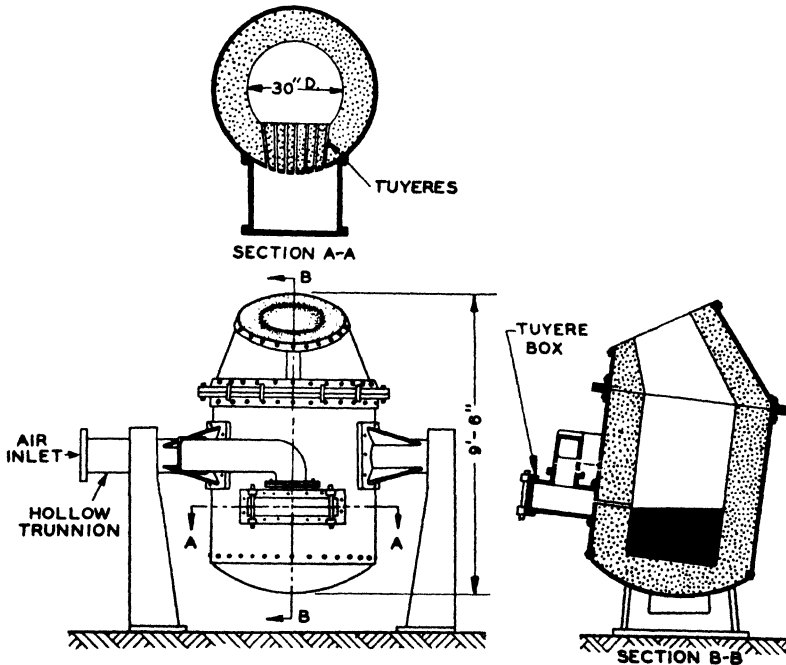
FIG. 120.—SIDE-BLOWN CONVERTER
