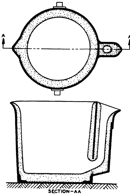
FIG. 123.—TEAPOT-SPOUT LADLE
