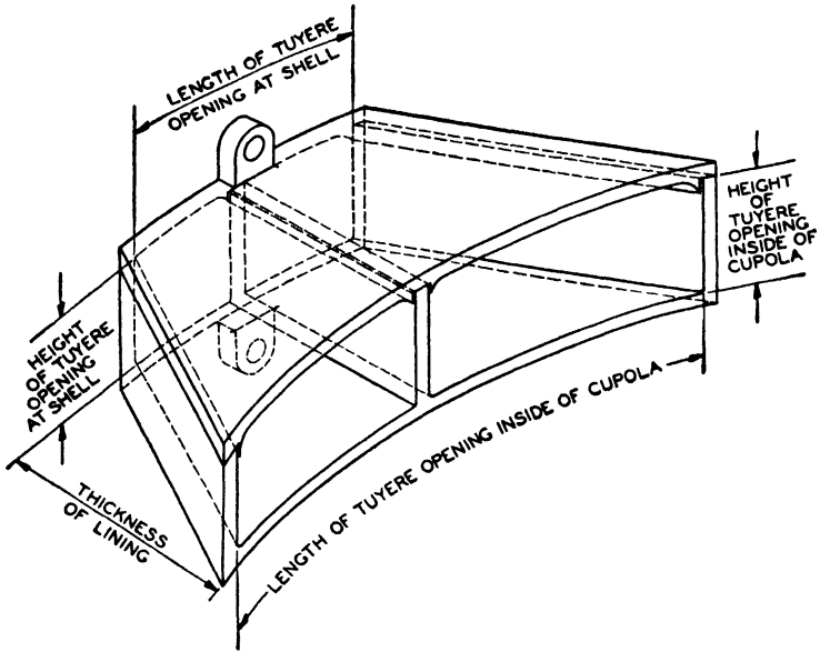
FIG. 161.—CUPOLA TUYERES
