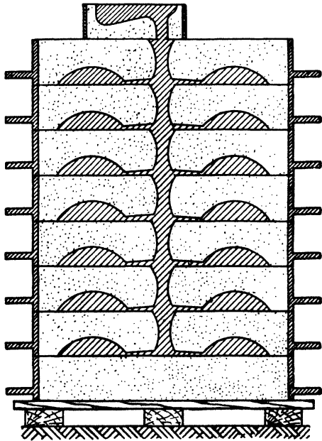
FIG. 41.—STACKED MOLD
