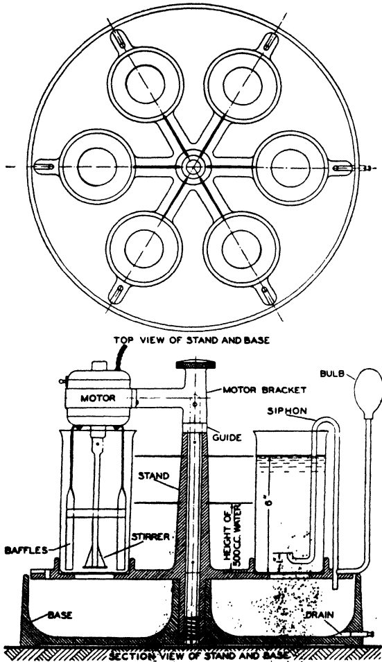
FIG. 169.—SAND-WASHING APPARATUS
