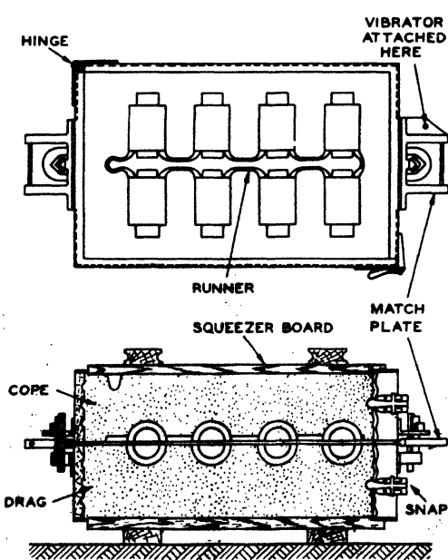
FIG. 27.—SNAP FLASK AND MATCH PLATE
