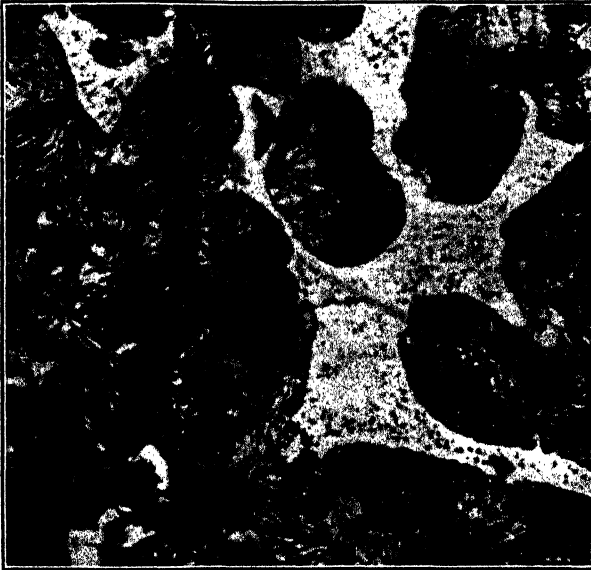
FIG. 95.—GRAY CAST IRON, ETCHED WITH 3 PER CENT NITAL, \times 1000 Dark areas are pearlite. Light spotted areas are steadite.
