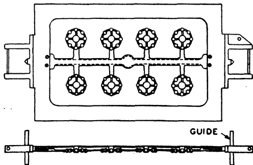
FIG. 26.—PATTERNS ON VIBRATOR FRAME
