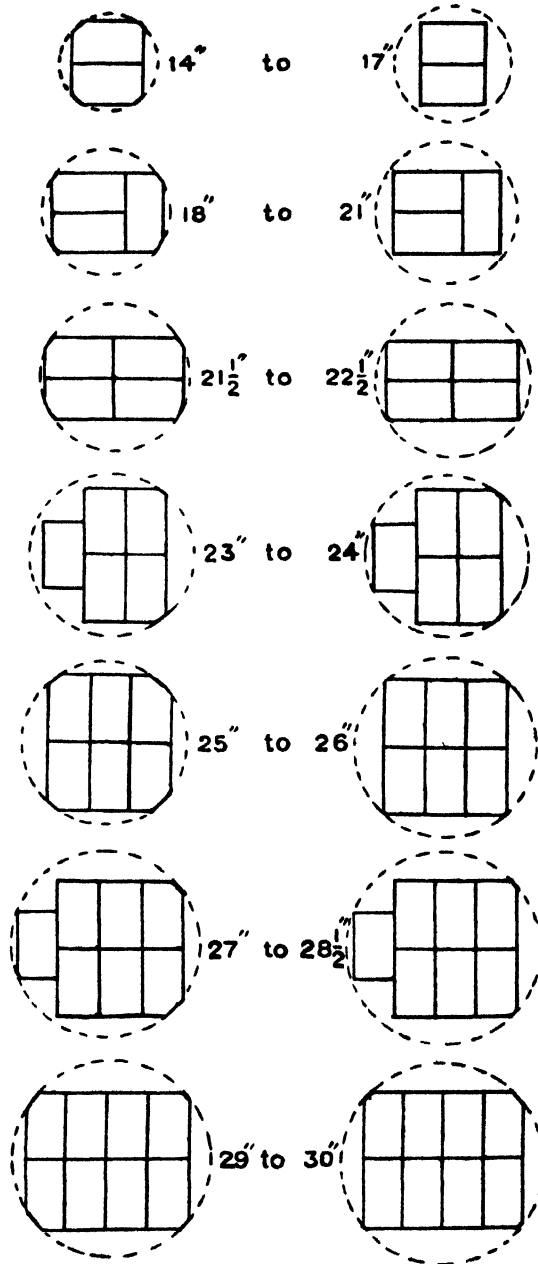
DIAGRAM 4. The method of cutting B. G. sleepers
