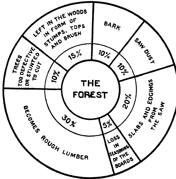
DIAGRAM 5. Wastage in conversion
