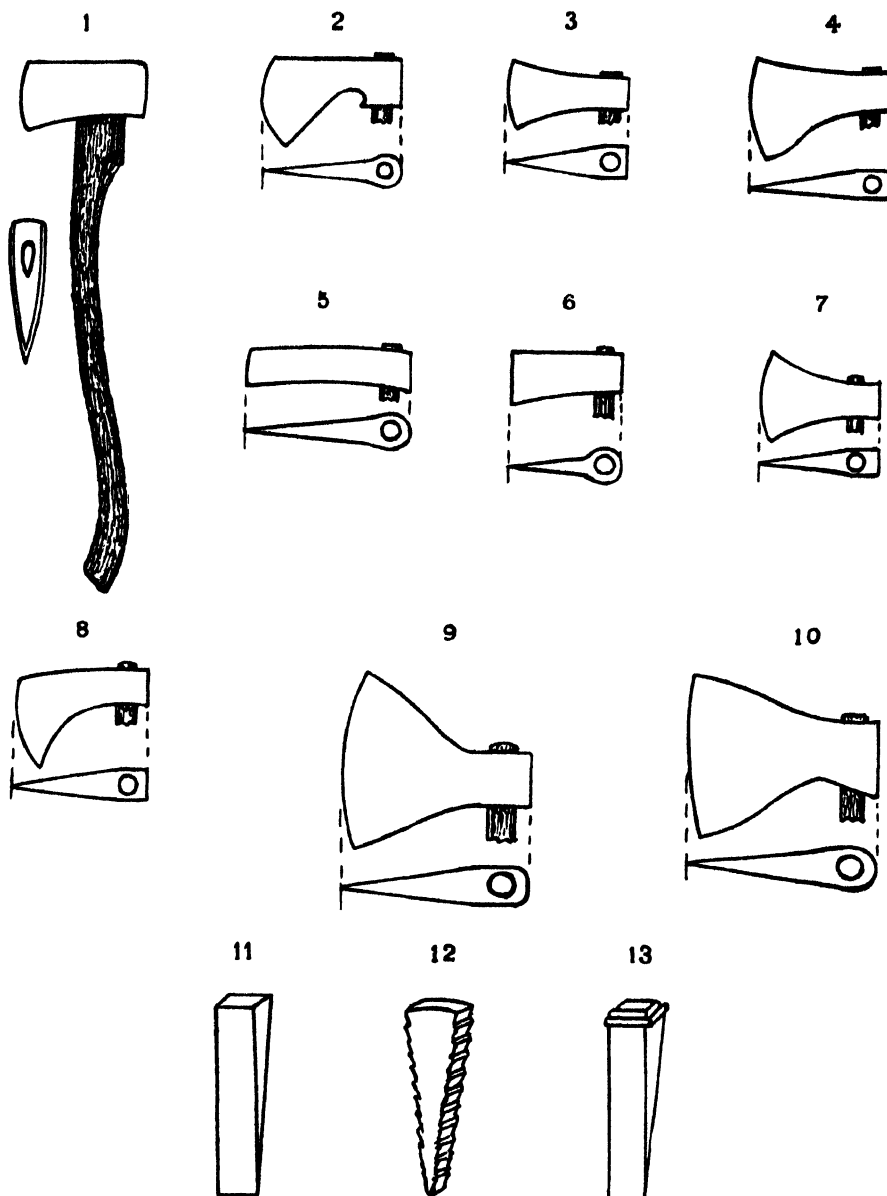
DIAGRAM 2. Implements used for felling, one-tenth natural size
