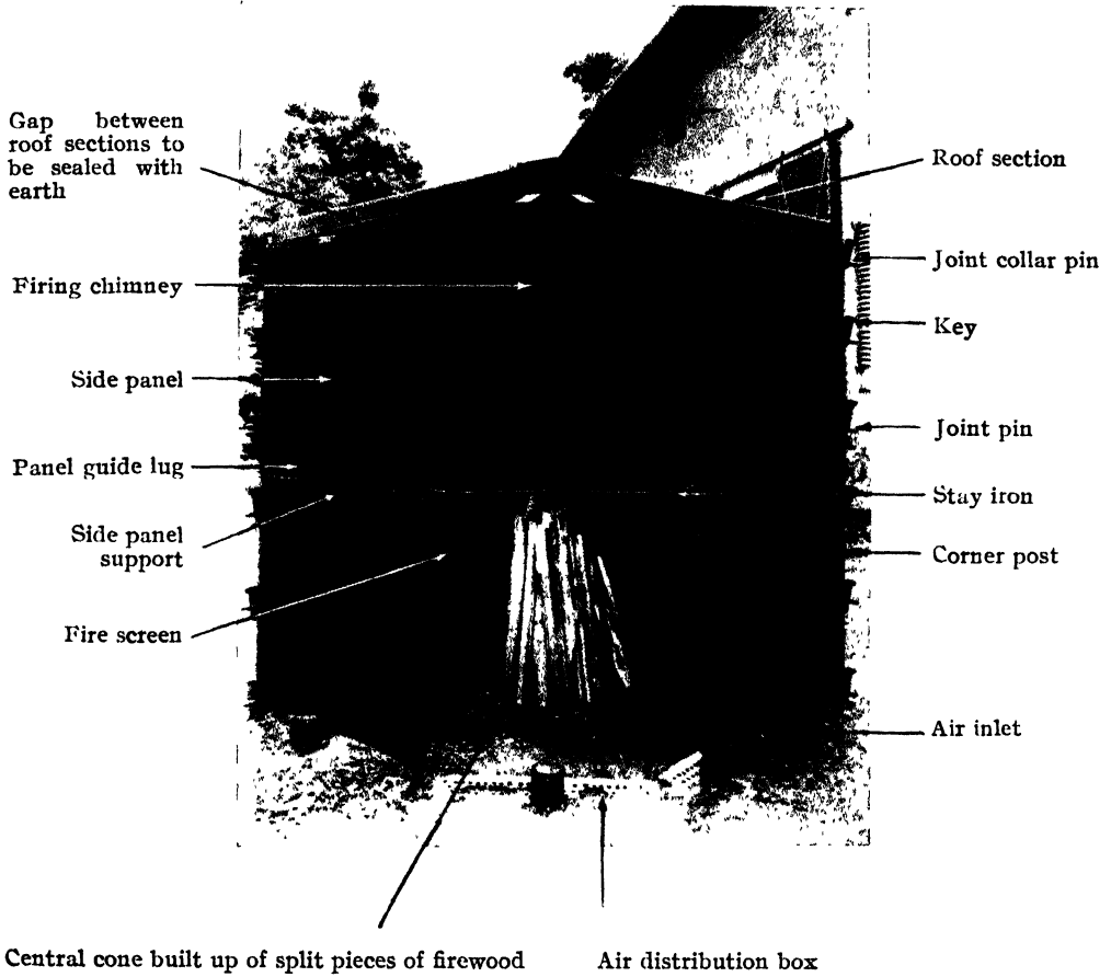
PLATE XVIII. Portable charcoal kiln
