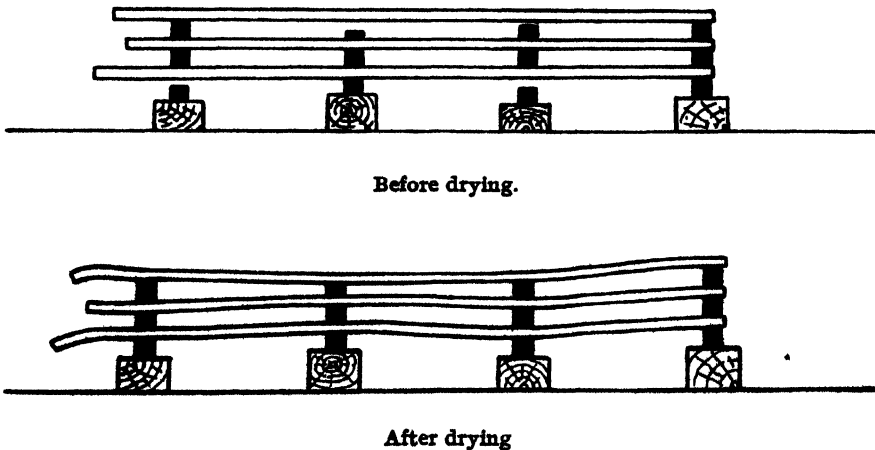
DIAGRAM 6. The effect of uneven foundations on timber piles. Even if the crossers are of uniform thickness, the whole stack of timber will be spoiled if the foundations are not level
