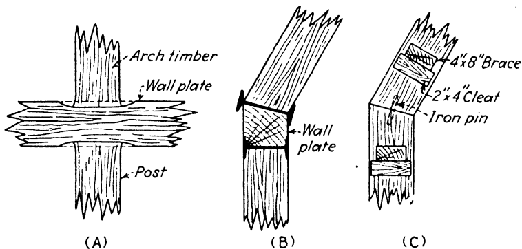
FIG. 312.—Typical joints between posts and arch timbers. A, post and rib in direct bearing on side grain of wall plate, wall plate subject to crushing. B, armored wall plate, posts and ribs bear against webs of steel beams. C, wall plate eliminated, posts and ribs in direct bearing; dowel pin keeps them from slipping; braces between sets are required to provide longitudinal stability otherwise given by wall plate.
