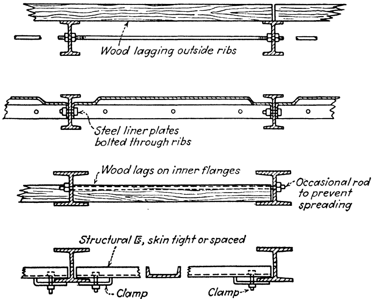
FIG. 325.—Various methods of lagging steel ribs.
