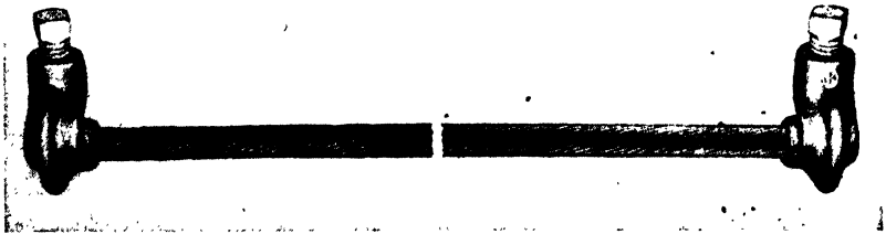
FIG. 100.—Copper rail bond, attached to base of rail by setscrews to improve conductivity of ground return past rail joints. (Courtesy of Ohio Brass Co.)
