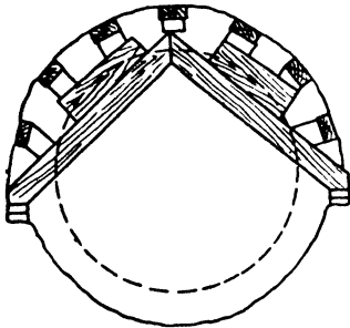
FIG. 188.—Horse-cup method of timbering.
