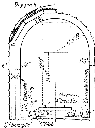
FIG. 17.—Typical single-track railroad tunnel. Note ballast walls to keep drainage ditches clear.
