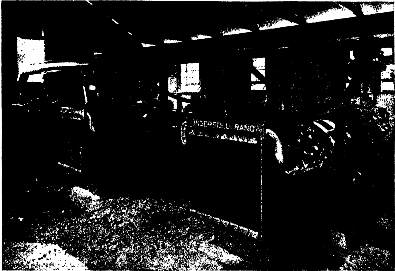
FIG. 166.—Radiator-cooled electric-drive compressors, Bates & Rogers Construction Corp., Pennsylvania Turnpike tunnels. Compressors are double compound units, driven by a single motor. (Courtesy of Ingersoll-Rand Co.)
