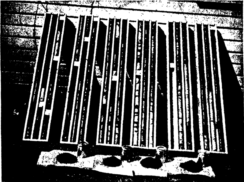
FIG. 14.—Core samples carefully boxed for inspection and preservation. The fines are kept in the sealed cans. (Courtesy Sullivan Machinery Co.)
