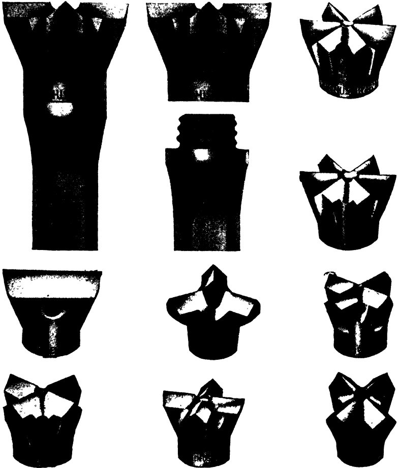
FIG. 288.—Various types of detachable bits for regular and special services. This make of bit has an upset shoulder which bears against a shoulder on the steel shank. (Courtesy of Timken Roller Bearing Co.)
