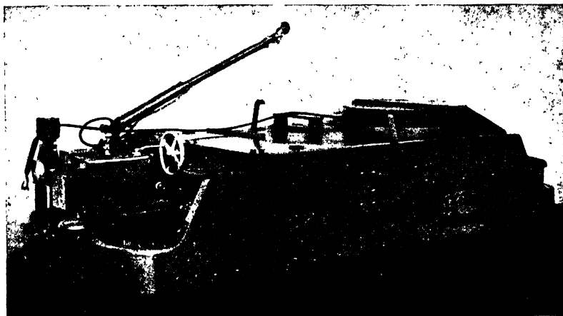
FIG. 123.—Jeffrey 8-ton trolley locomotive, 36-in. gage, equipped with two 40-hp. motors. Note the cable reel with automatic rewinder which permits the locomotive to work beyond the end of the trolley wire.
