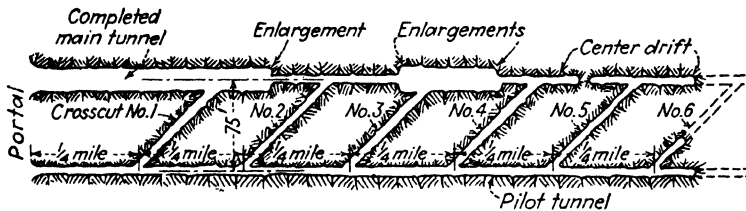
FIG. 278.—Pilot tunnel method of driving.
