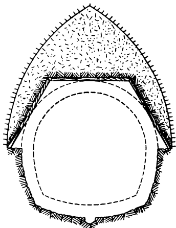
FIG. 311.—Natural arch in sandstone.
