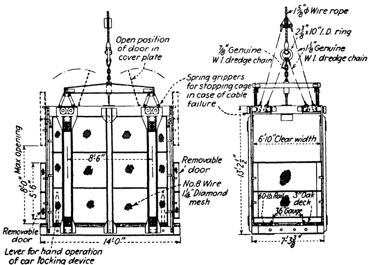
FIG. 133.—General design of muck skip (top) and cage, Shaft 19, Delaware Aqueduct. The skip and cage are in balance (Courtesy of Union Iron Works and Associated Contractors, Inc.)
