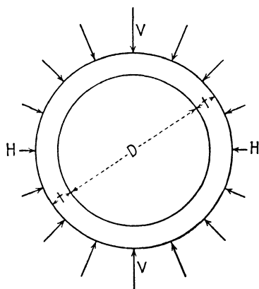
Fig. 23.—Unequal pressures on lining of soft-ground tunnel.
