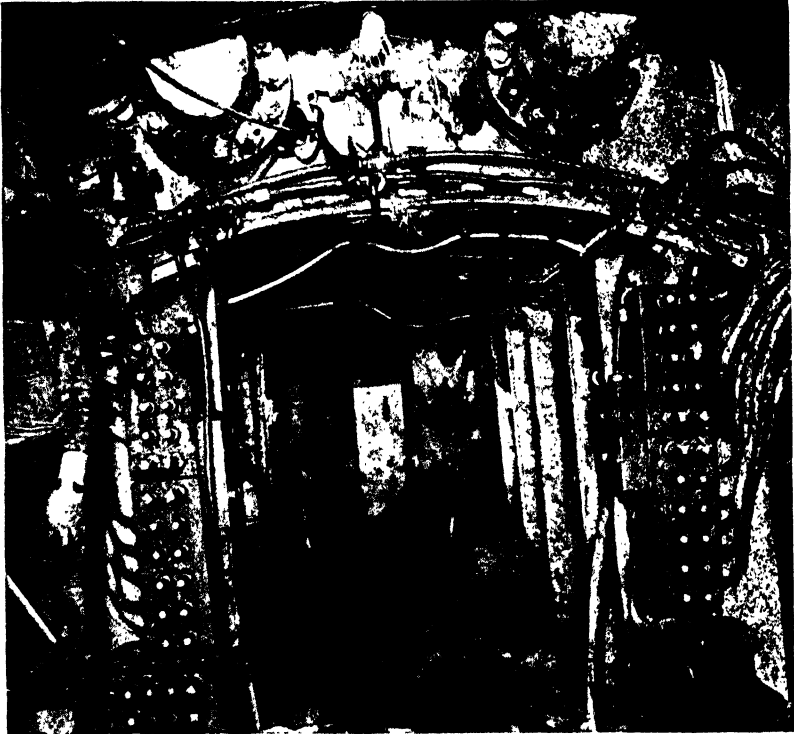
FIG. 233.—Valves for controlling shoving jacks on a shield. Valves are arranged in two banks, one for each side of the shield; master valves are at lower left.
