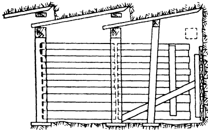
FIG. 182.—Use of the false set in forepoling.
