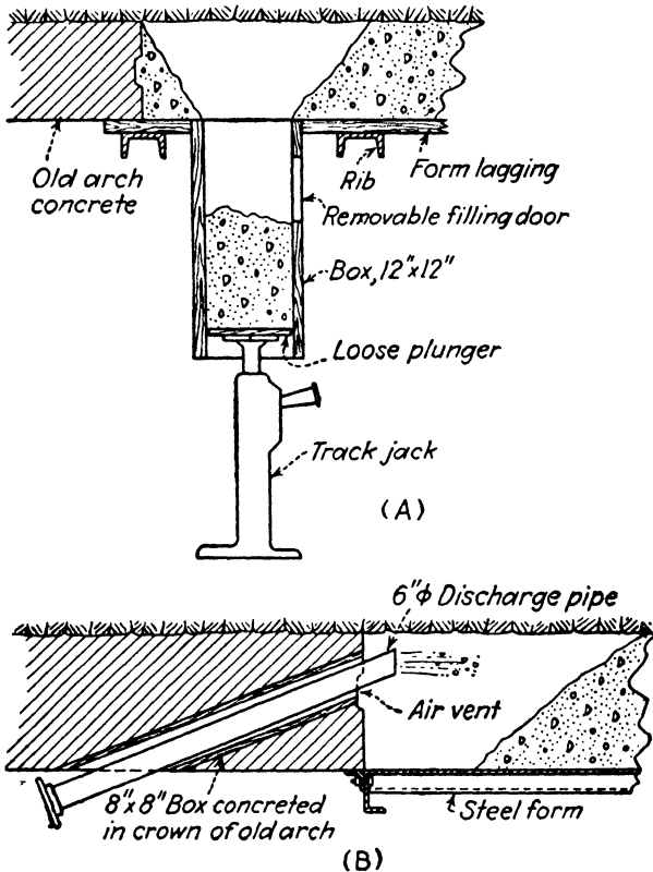
FIG. 358.—Two methods of making the closure between concreted sections. A , method for hand placing; B , method used with pneumatic placers.
