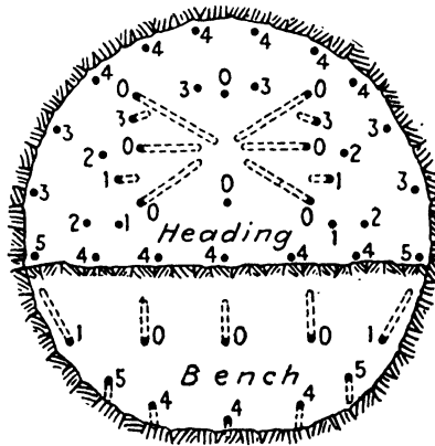
FIG. 301.—Drilling and shooting diagram for a 17-ft. tunnel driven by heading-and-bench method. Bench is shot with the heading. Numbers refer to blasting-cap delays.
