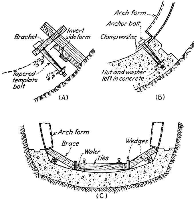
FIG. 341.—Methods of fastening and bracing forms at the invert. A, template for setting anchor bolts in the invert; B, clamp for holding bottom of arch form; C, typical bracing at invert for telescoping forms.
