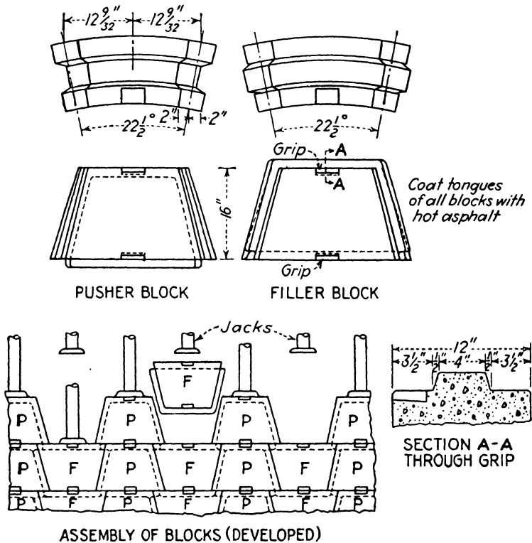
FIG. 220.—Details of the T. & M. type of concrete block for small shield-driven tunnels.
