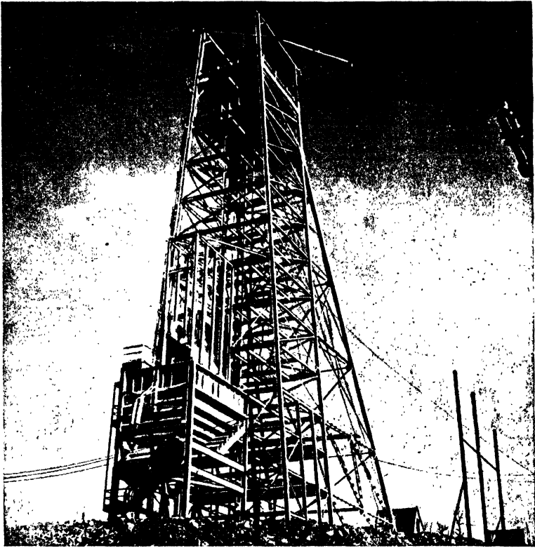
FIG. 135.—Headframe and muck storage bin, Shaft 6, Delaware Aqueduct, Pleasantville Constructors, Inc. Note the hydraulically operated bin gates. Hoist is in the house to the rear of the shaft, beyond the tower backstays.
