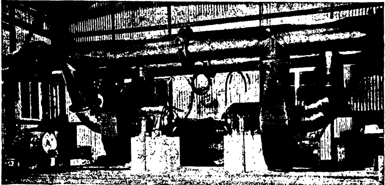
FIG. 140.—Flexible fan and piping arrangement, Colorado River Aqueduct. Fans were nonreversing, but the direction of air flow could be changed and the volume varied by manipulating the pipe valves and changing the speed and size of impellers.
