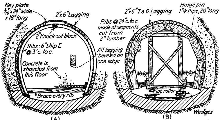
FIG. 334.—Wood forms for small tunnels. A, hand-handed and hand-filled form; B, traveling form, mechanically filled.
