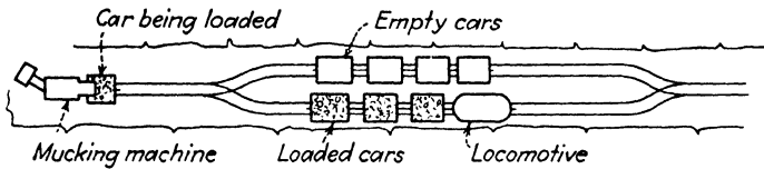
FIG. 88.—Passing track.
