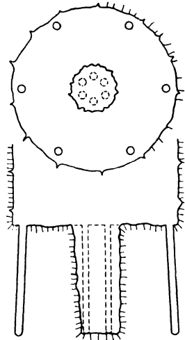
FIG. 63.—Burnt cut for sinking small shafts.
