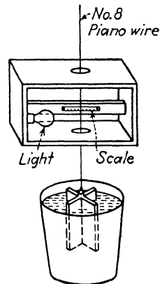
FIG. 34.—Plumb bob and light box at foot of shaft.
