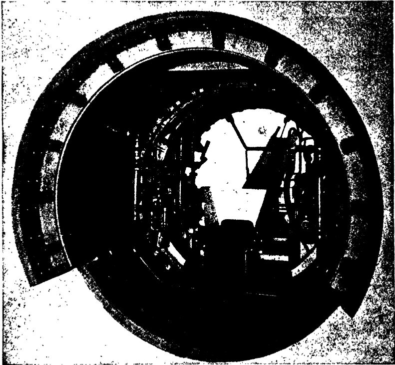
FIG. 235.—Articulated T. & M. shield for 6-ft. concrete-block-lined tunnel. The air-operated hydraulic pumps are mounted within the shield. Muck cars are loaded by the belt conveyor. (Courtesy of Link-Belt Co.)
