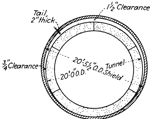
FIG. 221.—Shape of the annular void under tail of the shield.
