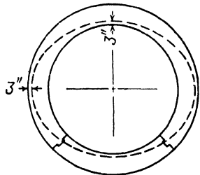
FIG. 26.—General location of reinforcing steel for tension in soft-ground tunnel lining.
