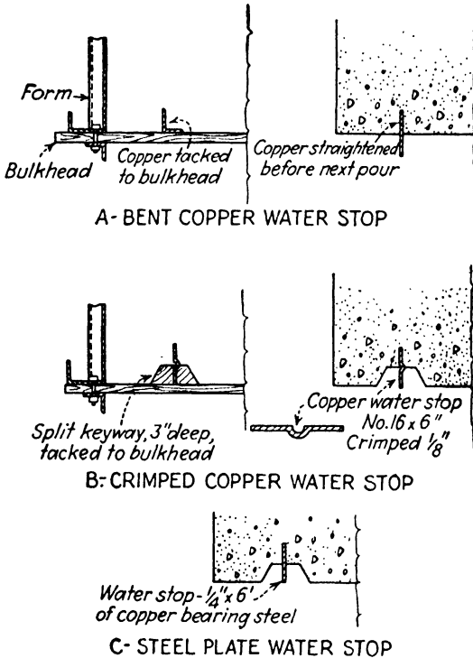
FIG. 343.—Various types of water stops in concrete lining.
