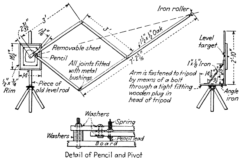
FIG. 42.—Pantograph for direct recording of cross section of a tunnel.
