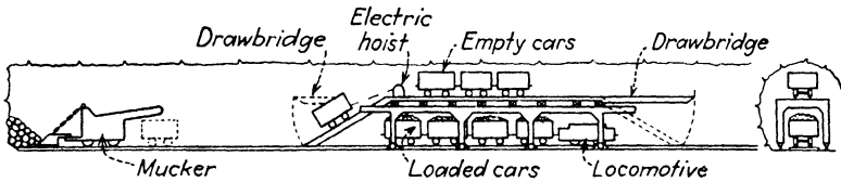
FIG. 96.—The Grasshopper car changer. Empty cars are stored on the upper level; loads are hauled back at main track level; the ramps to upper level lift up to clear passing cars below.
