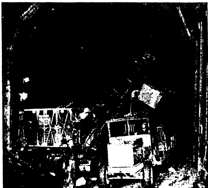
Fig. 124.—Linn tractor-truck hauling muck at Parker Dam diversion tunnel.
