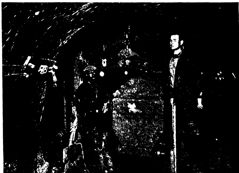
FIG. 367.—Intersection of shaft and tunnel in marl, Charleston water tunnel. This material is soft enough to cut with spades, yet stands without timbering, and the water tunnel was left unlined.
