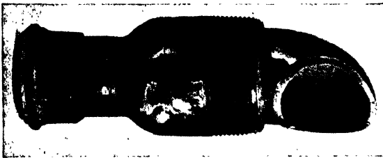
FIG. 225.—Special nozzle to direct flow of gravel shot behind tail of shield, used on Union Tunnel, Pennsylvania R.R., Baltimore.
