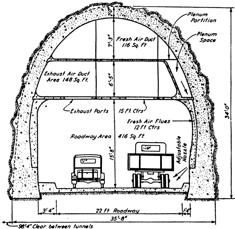
FIG. 20.—Broadway Low Level Tunnel, Oakland, Calif. Note unusual arrangement of ventilation ducts. (From "Western Construction News.")
