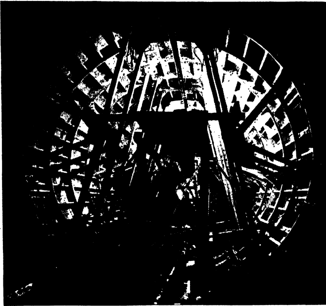
FIG. 333.—Nontelescoping steel forms, Crooked Creek Dam diversion tunnel, 15½ ft. in diameter. Note that the bottom of the form is clamped to anchors cast into the invert concrete. (Courtesy of Blaw-Knox Co.)
