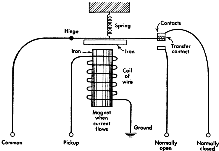
FIG. 1. Relay.
