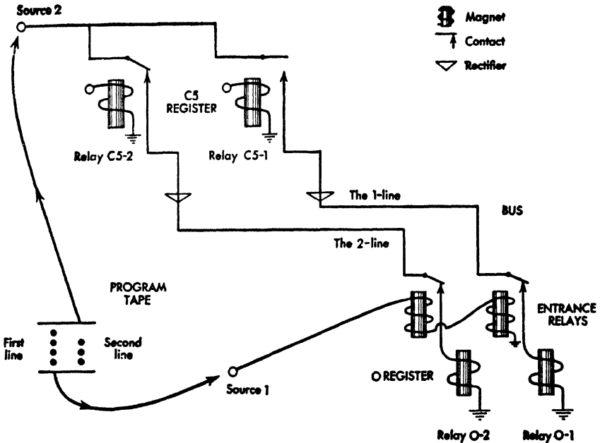
FIG. 5. Transfer circuit.
