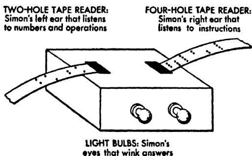
FIG. 1. Simon, the very simple mechanical brain.
