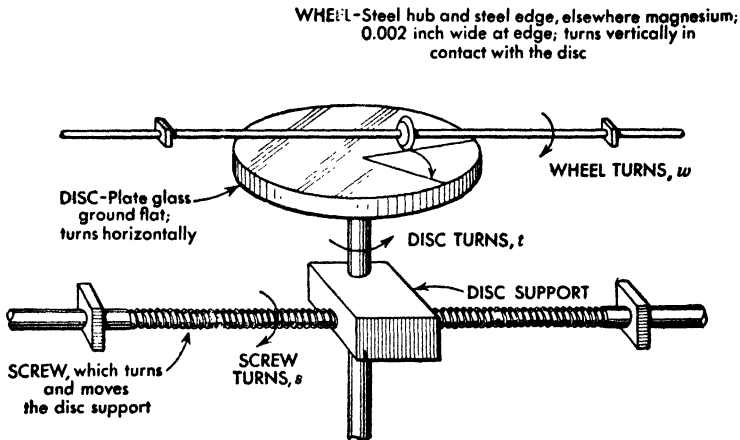
FIG. 19. Mechanism of integrator.
