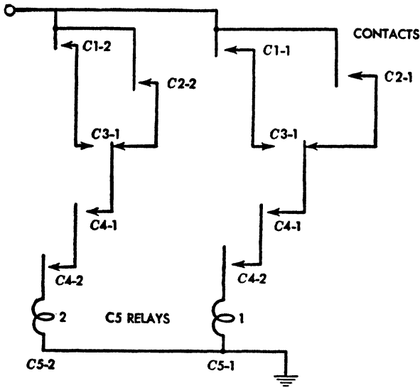
FIG. 11. Selection circuit.
