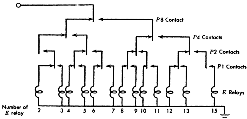
FIG. 12. Select-Receiving-Register circuit.
