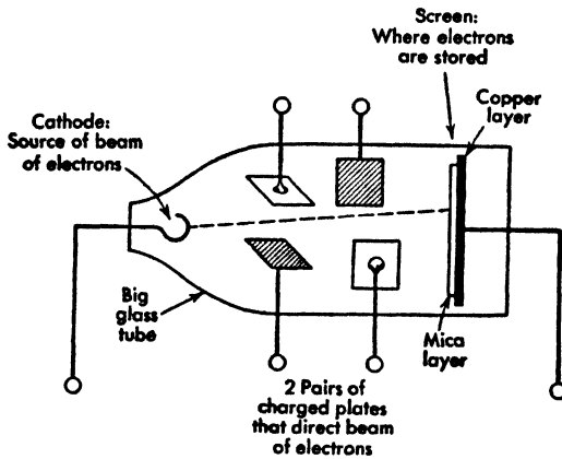
FIG. 4. Electrostatic storage tube.
