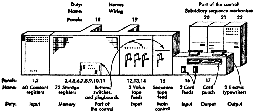
FIG. 1. Scheme of Harvard IBM Automatic Sequence-Controlled Calculator.
