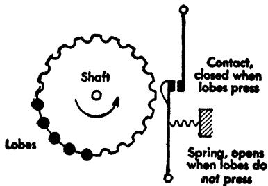
FIG. 8. Cam, with 5 lobes and contact.
