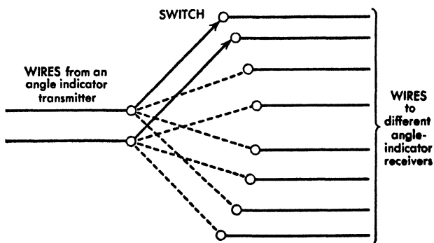
FIG. 13. Switchboard.
