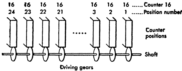
FIG. 6. Scheme of counter 16.
