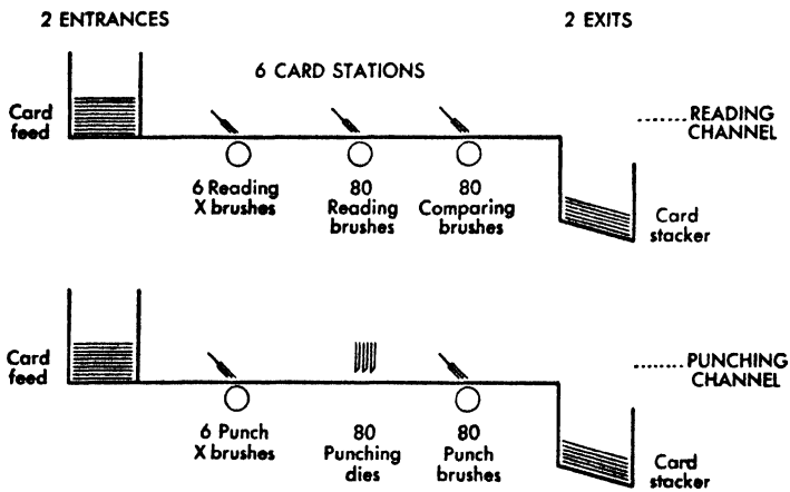
FIG. 9. Reproducer.
