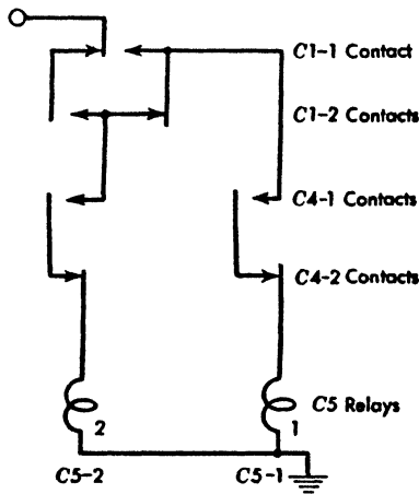
FIG. 8. Negation circuit.
