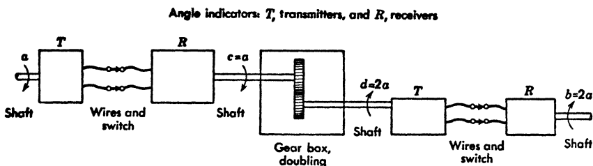
FIG. 16. Another example of a doubling mechanism.
