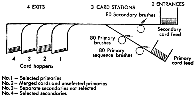
FIG. 10. Collator.
