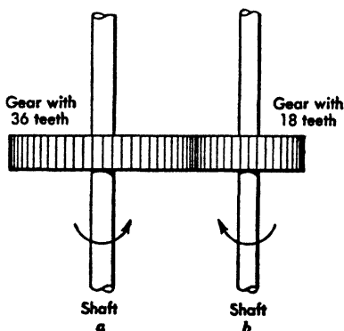
FIG. 15. Example of a doubling mechanism.
