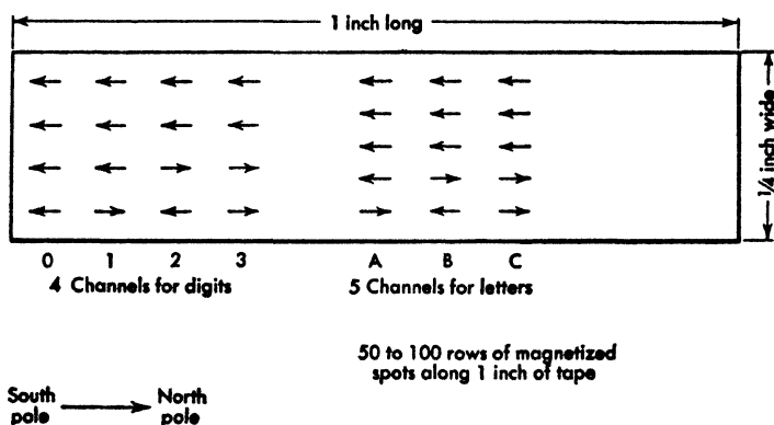
FIG. 1. Magnetic tape.
