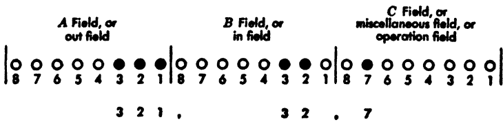
FIG. 10. Sequence-control tape code.
