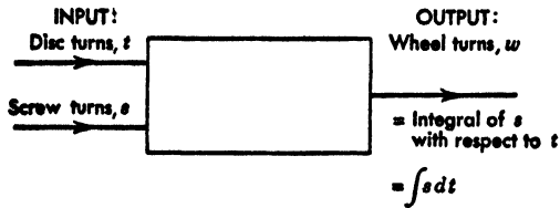
FIG. 20. Scheme of integrator.
