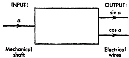
FIG. 10. Scheme of angle-indicator transmitter.
