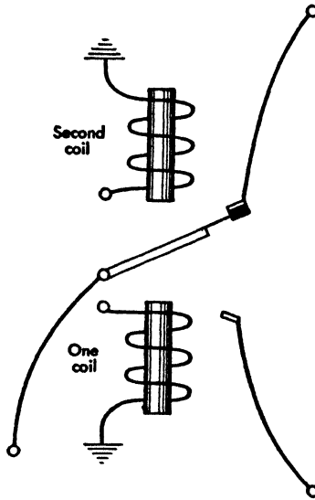
FIG. 13. Latch relay.
