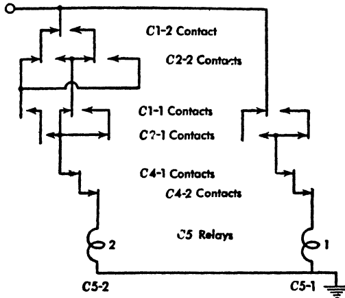
FIG. 9. Addition circuit.
