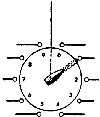
FIG. 3. Dial switch.
