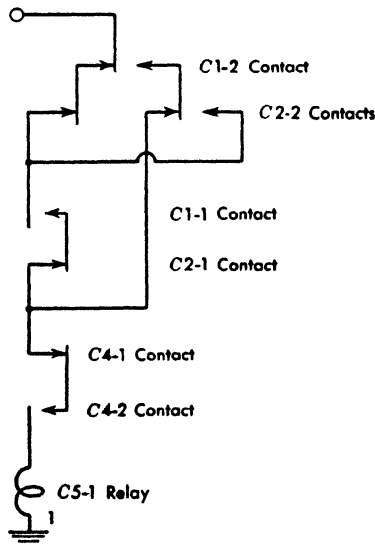
FIG. 10. Greater-than circuit.
