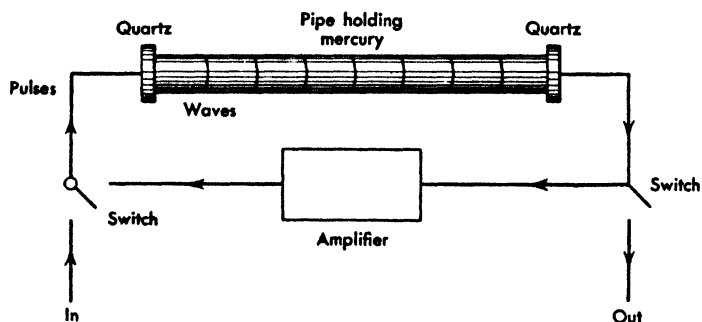
FIG. 3. Mercury tank.
