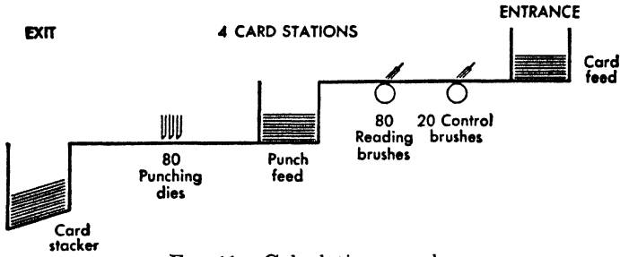
FIG. 11. Calculating punch.
