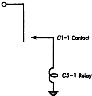
FIG. 6. Negation—right-hand digit.
