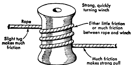
Fig. 9. Increasing turning force; winch, or torque amplifier.
