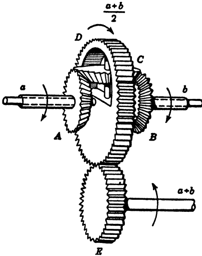
FIG. 18. Example of an adding mechanism (differential gear assembly).
