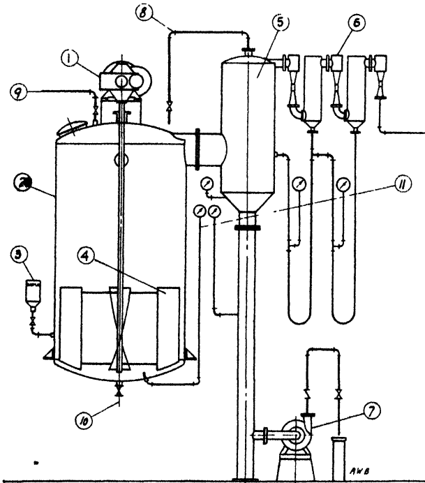
Fig. 54-A. Sweetened condensed milk vacuum cooler
