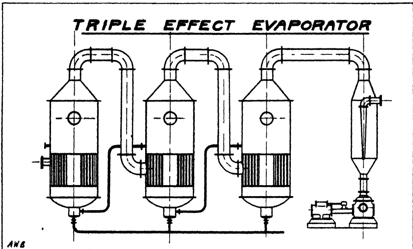
Fig. 31. Multiple-effect evaporator Courtesy of Arthur Harris & Co.
