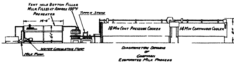
Fig. 77. New Chapman continuous pressure process sterilizer Courtesy of Berlin Chapman Company
