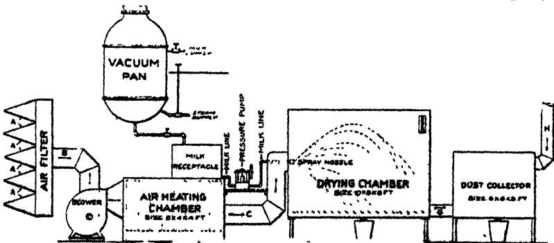
Fig. 102. The Merrell-Soule spray dryer
