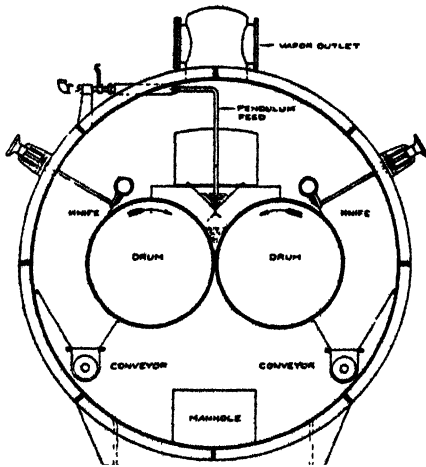
Fig. 99. The Buffovak Double-drum vacuum dryer Courtesy of Buffalo Foundry & Machine Co.
