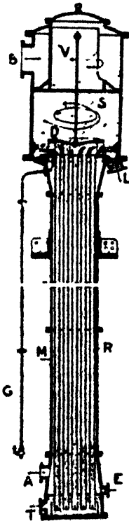
Fig. 21. Kestner tubular evaporator By Permission of Wehre and Robinson 8
