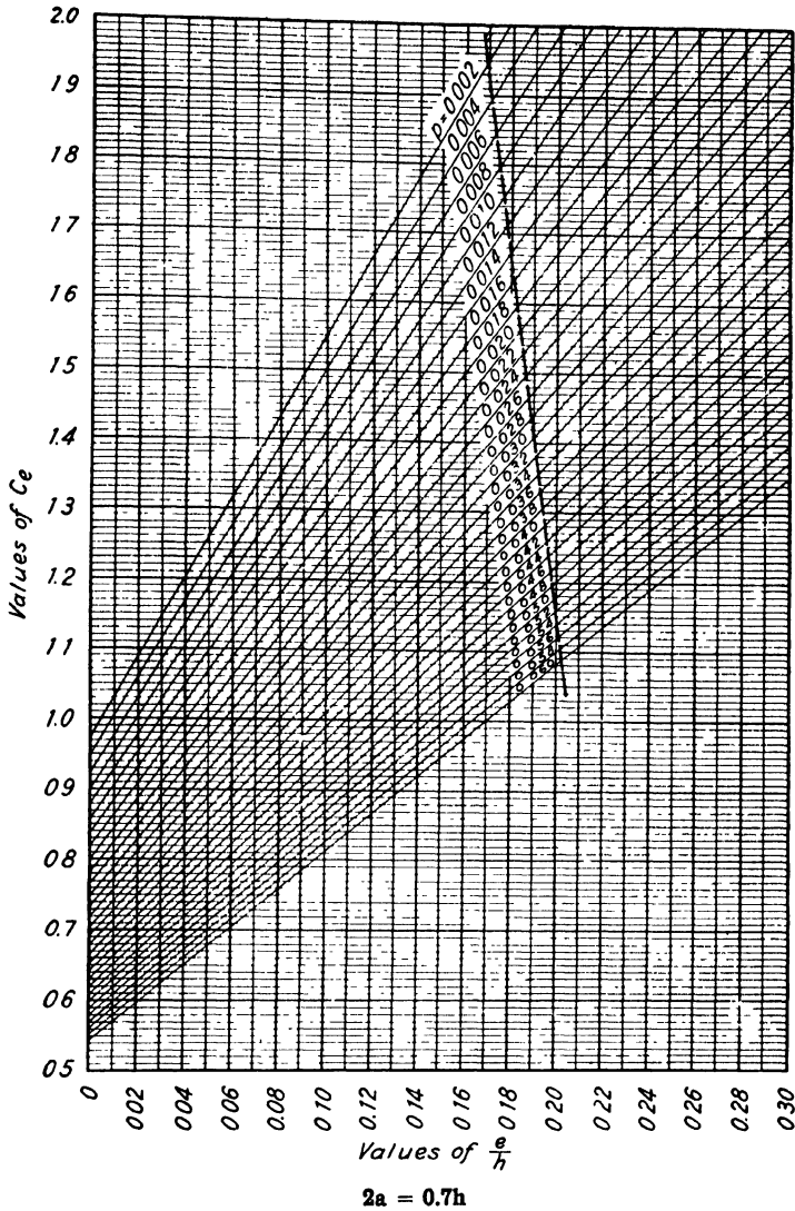
DIAGRAM 21.—Constants C_c for Members Subjected to Direct Compression and Flexure. (See p. 177.)
