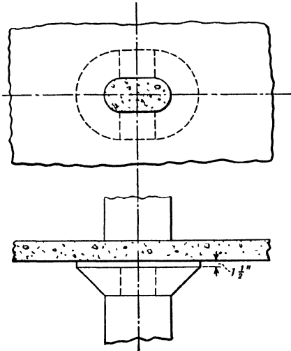
FIG. 111.—Column Head for Oblong Column. (See p. 319.)
