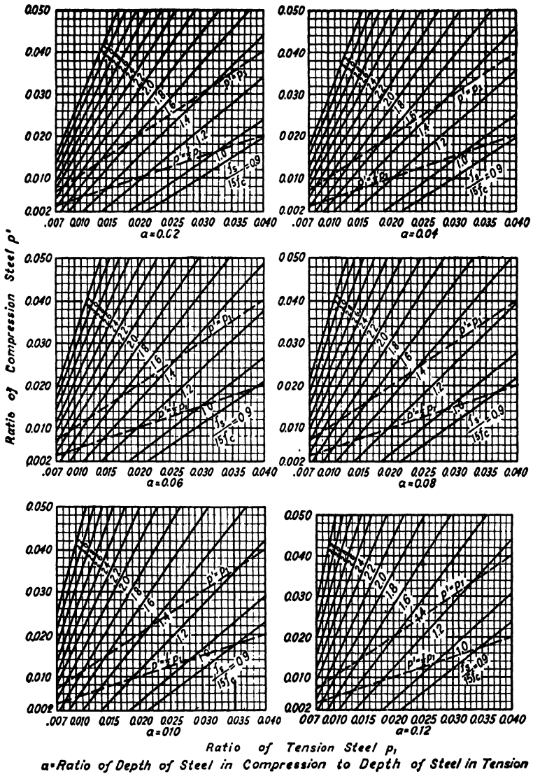
DIAGRAM 11. —Relation between Tensile and Compressive Steel in Beams with Steel in Top and Bottom. (See pp. 238 and 903.)
