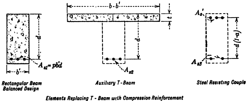
FIG. 76.—T-Beam with Compression Reinforcement. (See p. 230.)
