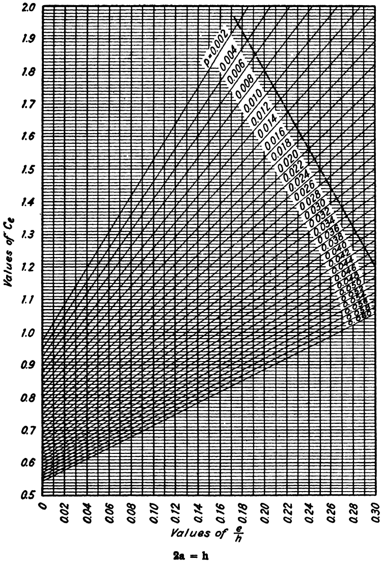
DIAGRAM 18.—Constants C_c for Members Subjected to Direct Compression and Flexure. (See p. 177.)
