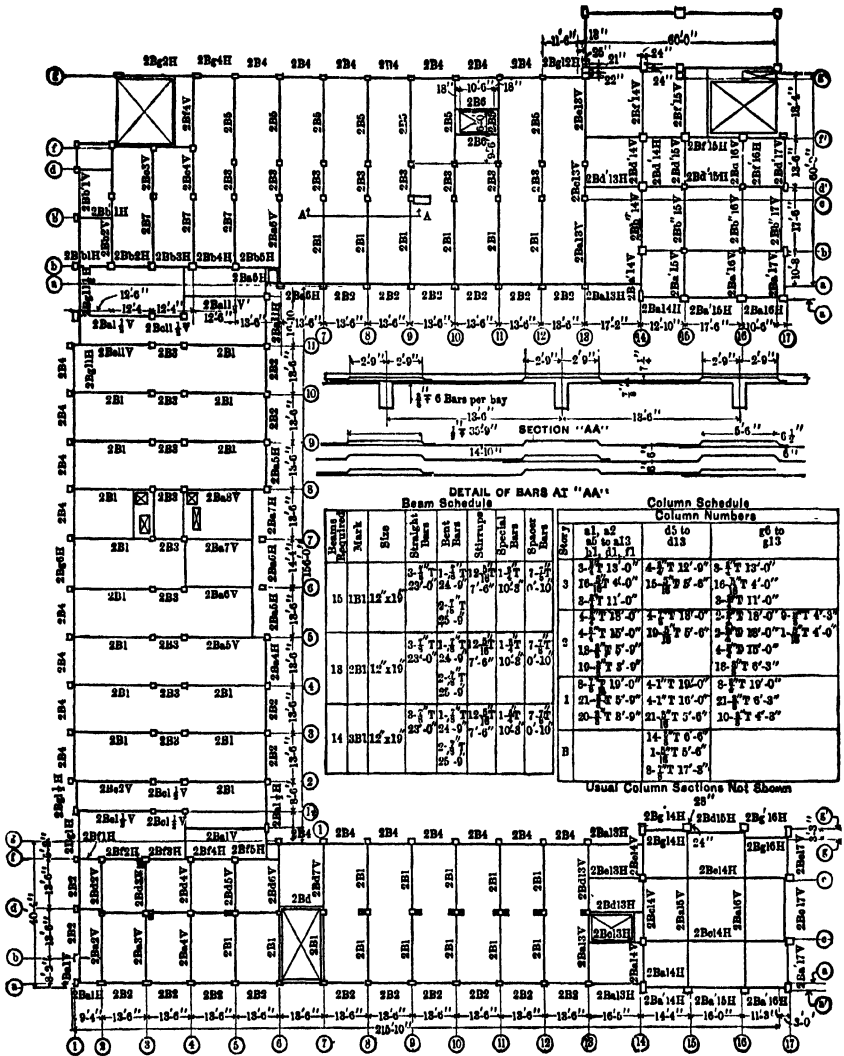
Fig. 239.—Typical Framing Plan and Steel Schedule. (See p. 711.) Buildings 1, 3 and 5, Massachusetts Institute of Technology, Cambridge, Mass. Stone & Webster, Builders. Sanford E. Thompson, Consulting Engineer.
