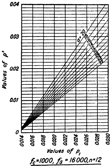
DIAGRAM 8.—Ratio of Compression Steel p' for Given Ratio of Tension Steel p_1 . (See p. 903.)
