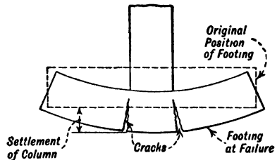
FIG. 157.—Failure of Footing. (See p. 479.)
