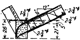
Intermediate Sawtooth Frame Supported by Girder
