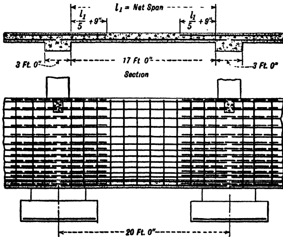
FIG. 206.—Detail of Basement Wall Supported at the Columns. (See p. 645.)
