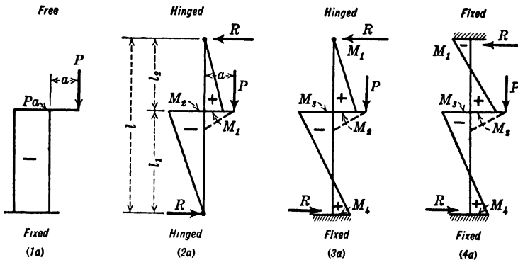
FIG. 156.—Columns Carrying Load on Brackets, b = 0 . (See p. 466.)
