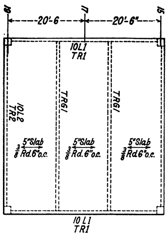
Tower Roof Framing
