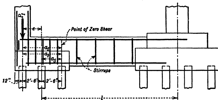
FIG. 176.—Straps for Footings on Piles. (See p. 536.)
