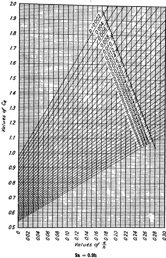
DIAGRAM 19.—Constants C_c for Members Subjected to Direct Compression and Flexure. (See p. 177.)
