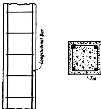
FIG. 140.—Typical Design of Column with Vertical Steel only. (See p. 405.)
