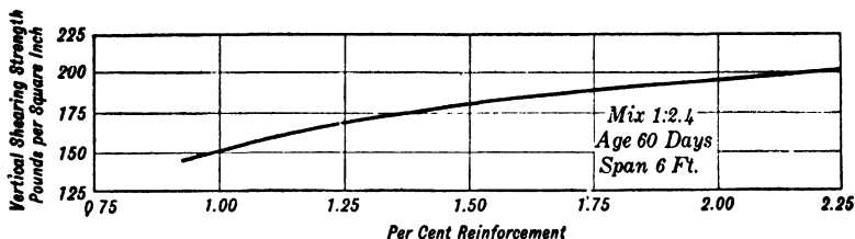
FIG. 16.—Effect of Percentage of Horizontal Steel upon Web Resistance. (See p. 47.)
