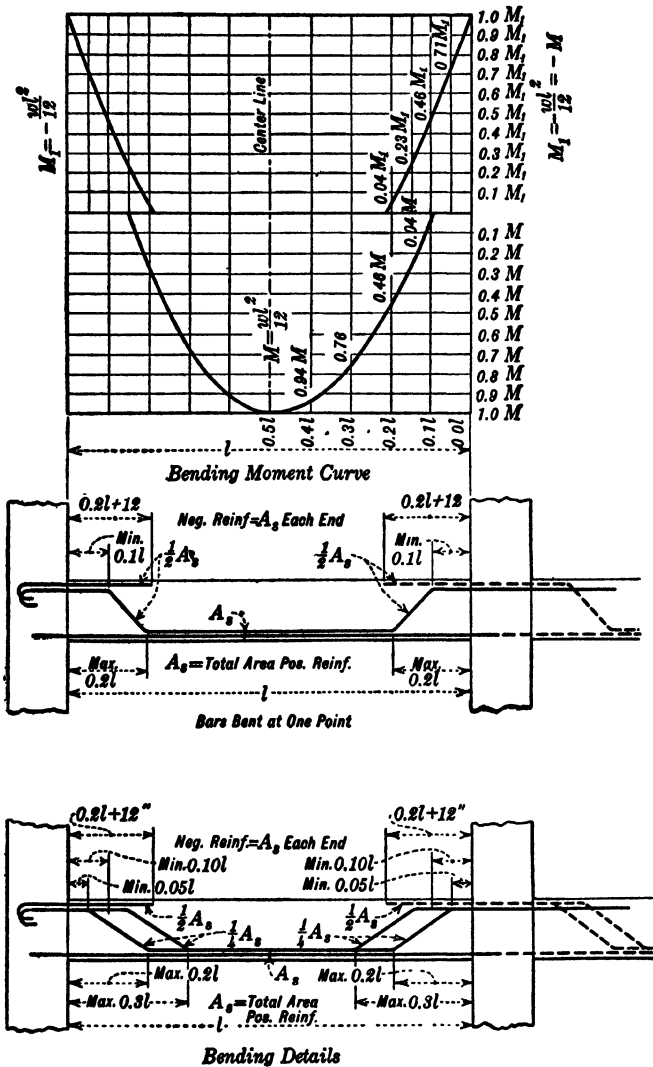
FIG. 102.—End Span of Building Frame. End Fully Restrained. (See p. 290.)
