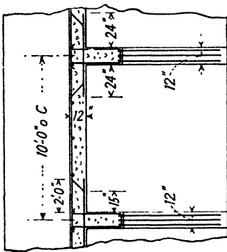
Horizontal Section
