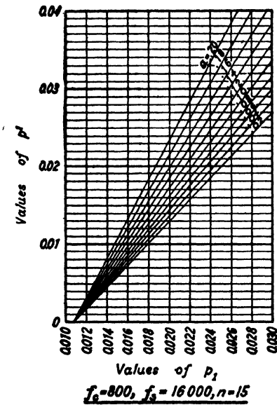
DIAGRAM 7.—Ratio of Compression Steel, p' for Given Ratio of Tension Steel p_1 . (See p. 903.)
