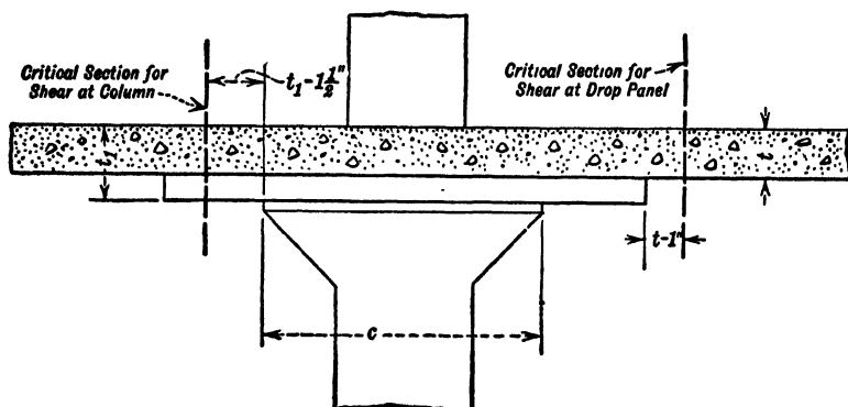
FIG. 120.—Section of Critical Shearing Stresses. (See p. 347.)
