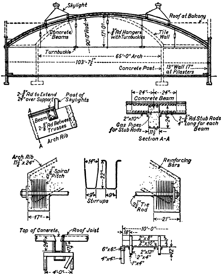
FIG. 218.—Details of Arch Roof. (See p. 669.)
