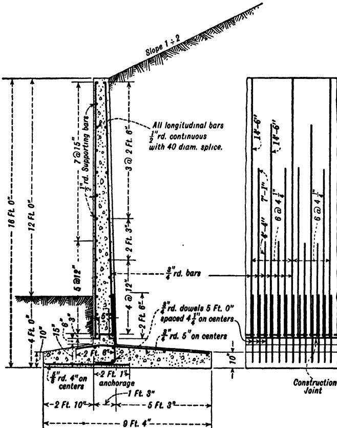
FIG. 305.—Details of T-wall designed in Example. (See p. 862.)
