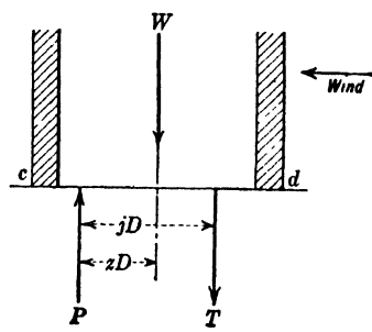
FIG. 293.—External and Internal Forces Acting upon a Chimney. (See p. 817.)
