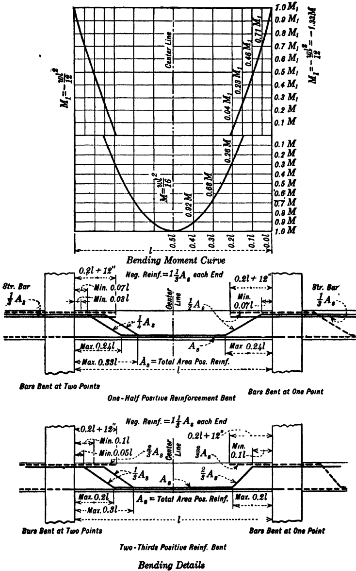
FIG. 103.—Interior Span of Building Frame. (See p. 290.)
