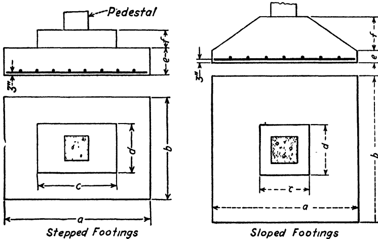
FIG. 238.—Method of Showing Independent Footings. (See p. 713.)
