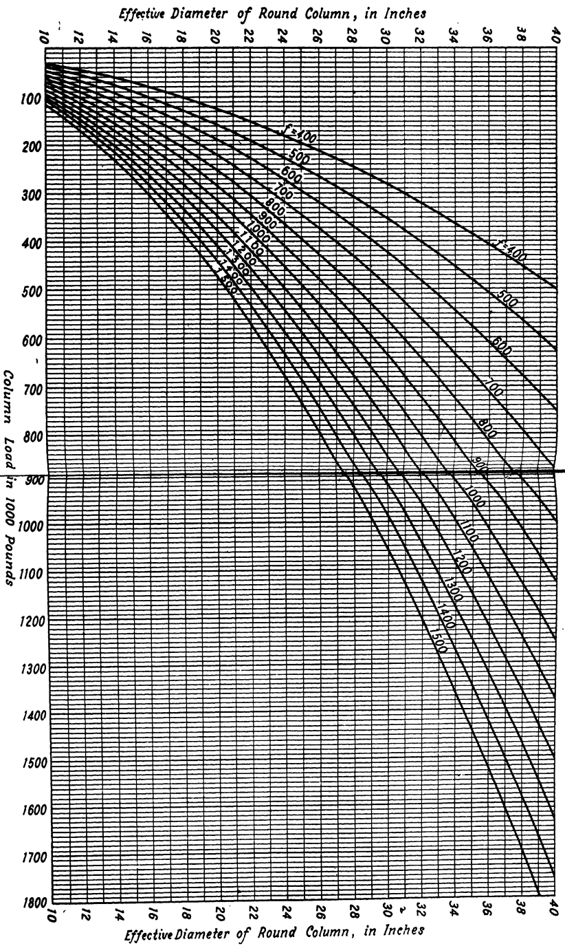
Diagram 16.—Total Loads on Round Columns for Different Average Stresses, f . Based on Formula P = Af . (See p. 406.)
