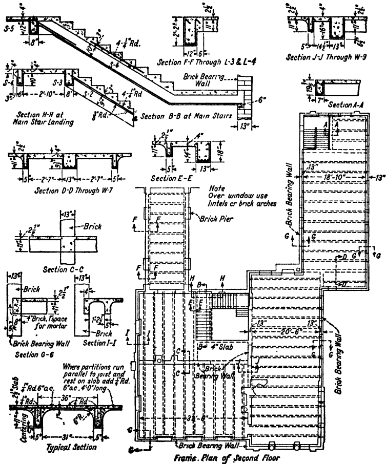
FIG. 204.—Floor Plan and Details of Barnes Foundation Building. (See p. 629.) Paul P. Cret, Architect. William H. Gravell, Engineer.
