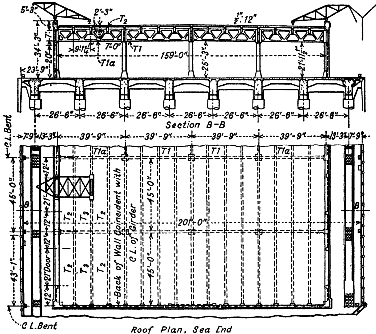
FIG. 224.—Partial Plan and Section of Pier 6 at Cristobal, Canal Zone. (See p. 677.)
