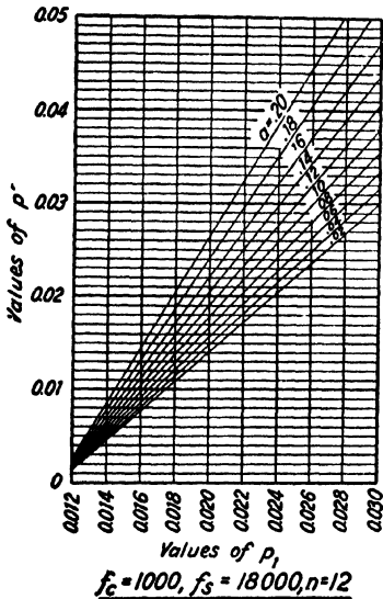
DIAGRAM 10.—Ratio of Compression Steel p' for Given Ratio of Tension Steel p_1 .
