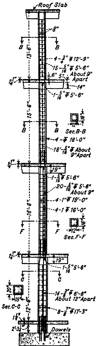
FIG. 146.—Typical Column with Vertical Steel Only. (See p. 418.)
