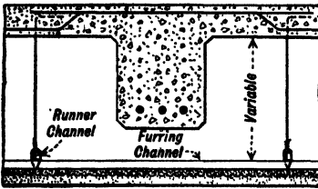
Ceiling Suspended below Beam from Concrete Slab
