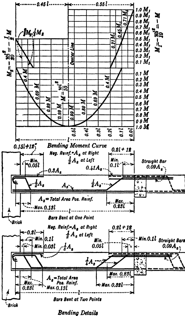
FIG. 99.—End Span of Continuous Beam, Freely Supported or Slightly Restrained at End. (See p. 290.)
