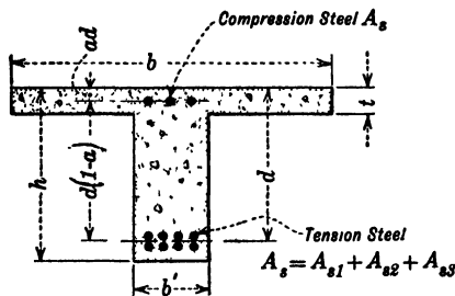
T-Beam with Compression Reinforcement
