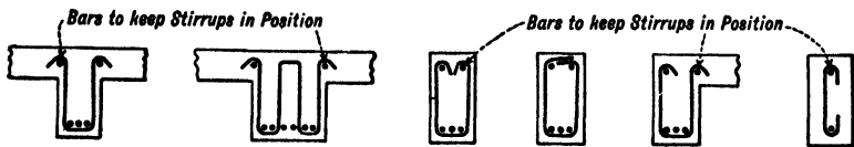
FIG. 78.—Types of Stirrups. (See p. 243.)
