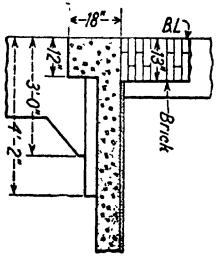
Section 2-2
