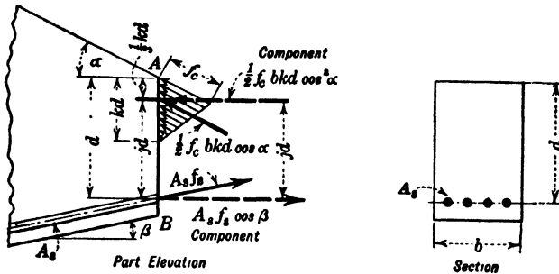
FIG. 47.—Resisting Forces in Wedge Shaped Beam. (See p. 140.)
