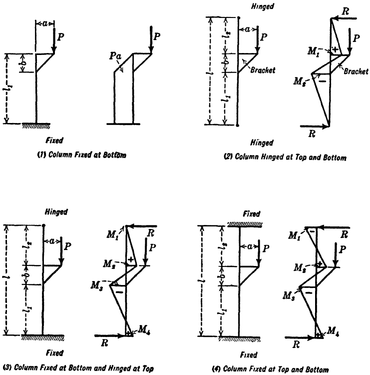
FIG. 155.—Columns Carrying Loads on Brackets. (See p. 464.)
