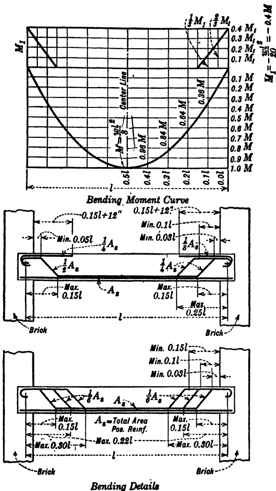
FIG. 98.—Beam Freely Supported or Slightly Restrained at Both Ends. (See p. 290.)
