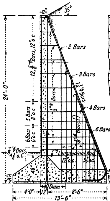
Cross Section
