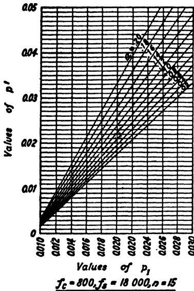
DIAGRAM 9.—Ratio of Compression Steel p' for Given Ratio of Tension Steel p_1 .
