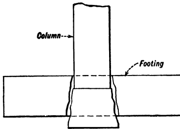
Fig. 165.—Failure Caused by Punching. (See p. 492.)
