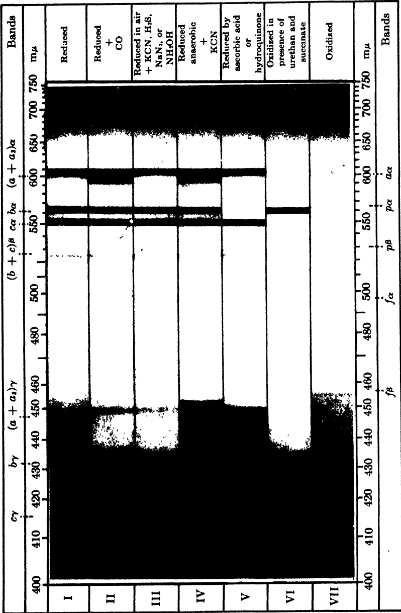
Fig. 4. Cytochromes a and a 3 (according to Keilin, 1953).
