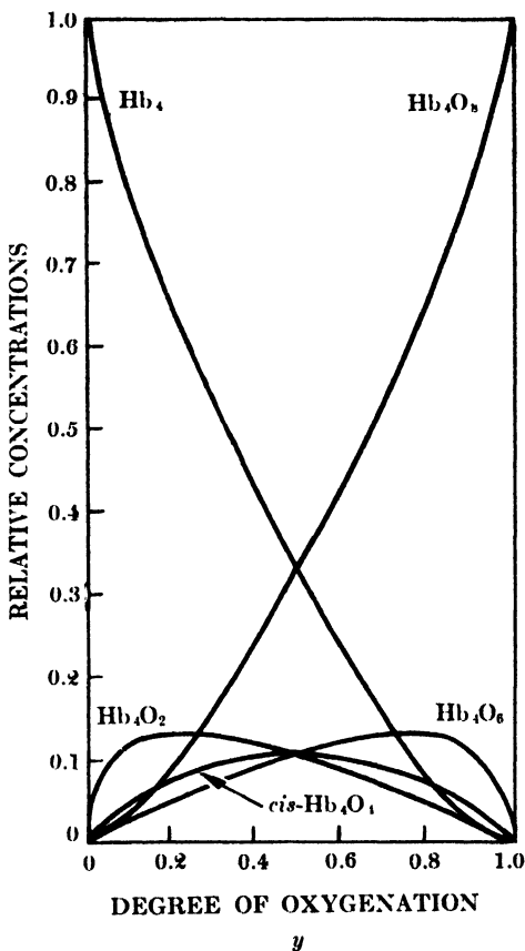
Fig. 7. Relative concentrations of intermediates between \text{Hb}_4 and \text{Hb}_4(\text{O}_2)_4 (after Coryell, Pauling, and Dobson, 500). The curve for \text{trans-Hb}_4(\text{O}_2)_2 is not given; it has 1/24 the height of II throughout.
