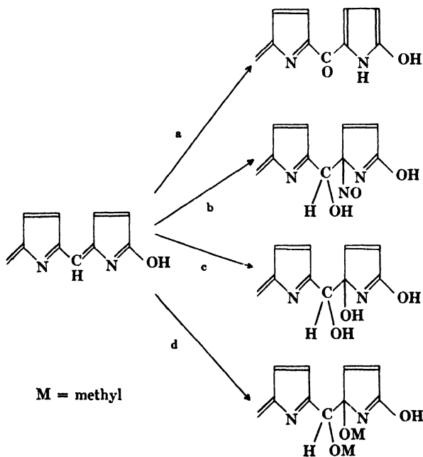
Fig. 10. Gmelin reaction.
