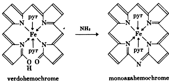
Fig. 4. Reaction of verdohemochrome with ammonia.
