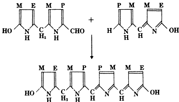
Fig. 16. Synthesis of mesobilerythrin (Siedel).
