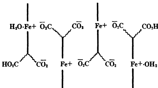
FIG. 4. \beta -Hematin (half-anhydride)
