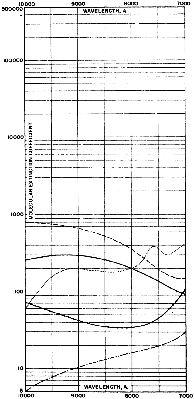
Absorption spectra: oxyhemoglobin, hemoglobin, hemoglobin, carboxyhemoglobin, hemoglobin cyanide. All spectra 10,000-2500 A.
