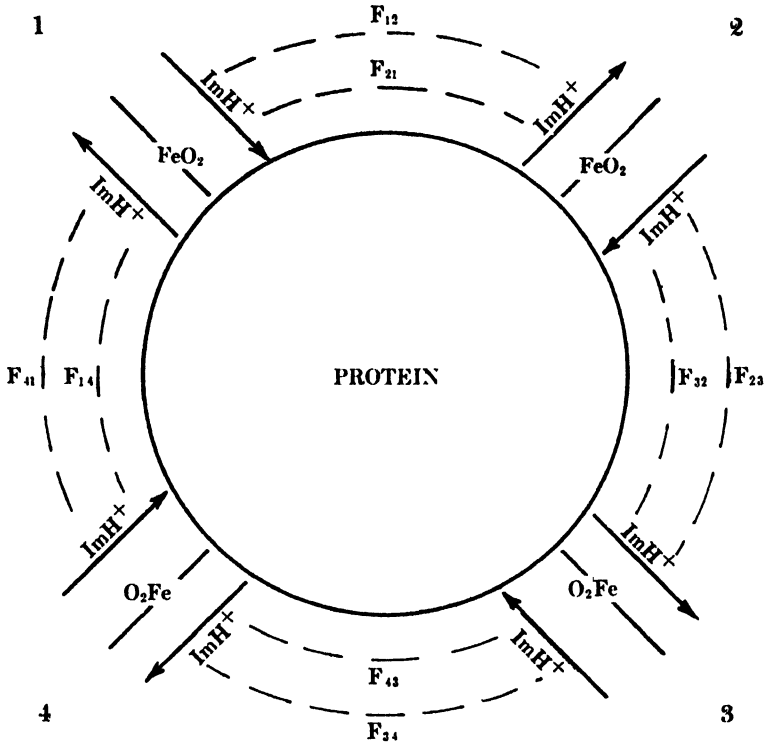
Fig. 13. Heme-heme interaction.
