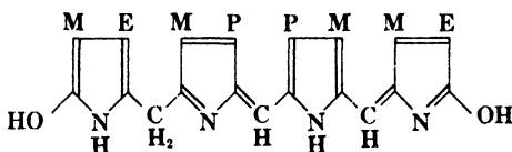
Fig. 17. Mesobiliviolin, differing from mesobilerythrin only in position of double bonds.
