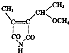
Fig. 7. \alpha -Methoxyethylmethylmaleimide
