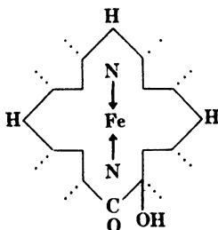
Fig. 7. Possible intermediate.
