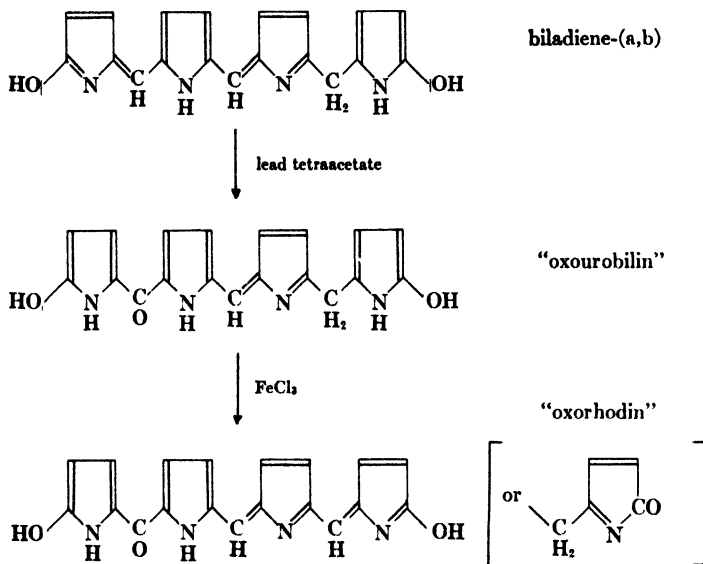
Fig. 22. Bilierythrinoid oxidation product of bilatriene.
