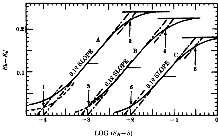
Fig. 3. The solid lines represent the theoretical relation of E_h - E_0' to \log(S_B - S) when q = r = 2 , 0.5S = S_r = S_0 = 1 \times 10^{-4} M . The broken lines represent the same theoretical relation with \log(S_B - 0.5S) as abscissa. Curve A, K_R = 1 \times 10^{-3} , 0.5 \log K_R = -4.00 (point 1); K_0 = 1 \times 10^{-4} , 0.5 \log K_0 = -2.00 (point 2); E_2 - E_0 = 0.2400 (0.06 coefficient). Curve B, K_R = 1 \times 10^{-5} , 0.5 \log K_R = -3.00 , (point 3); K_0 = 5 \times 10^{-3} , 0.5 \log K_0 = -1.15 (point 4); E_2 - E_0 = 0.2219 (0.06 coefficient). Curve C, K_R = 1 \times 10^{-4} , 0.5 \log K_R = -2.00 (point 5); K_0 = 1 \times 10^{-1} , 0.5 \log K_0 = -0.50 (point 6); E_2 - E_0 = 0.1800 (0.06 coefficient). After Clark et al. (453).
