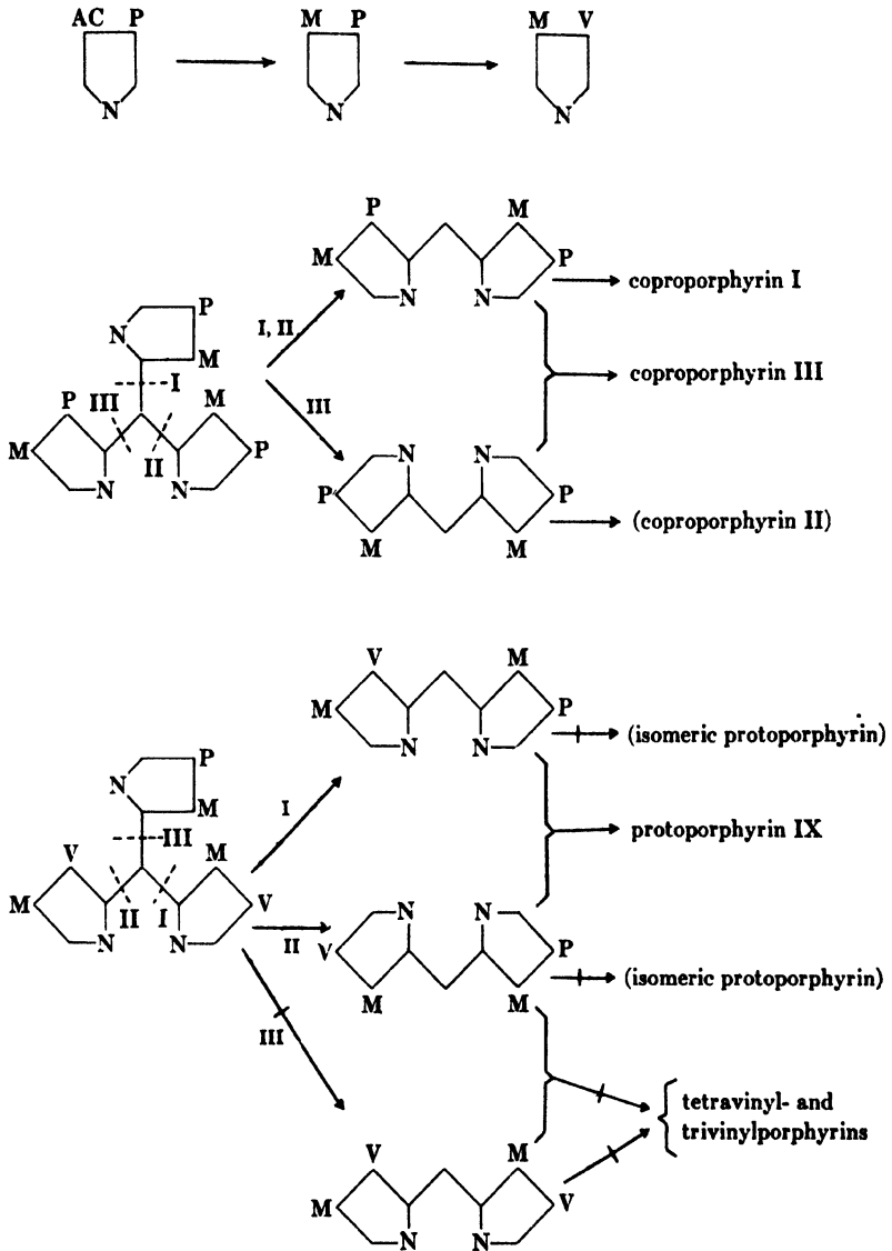
Fig. 3. Theory of porphyrinogenesis of Turner (1940); (→) possibilities not taken into account.
