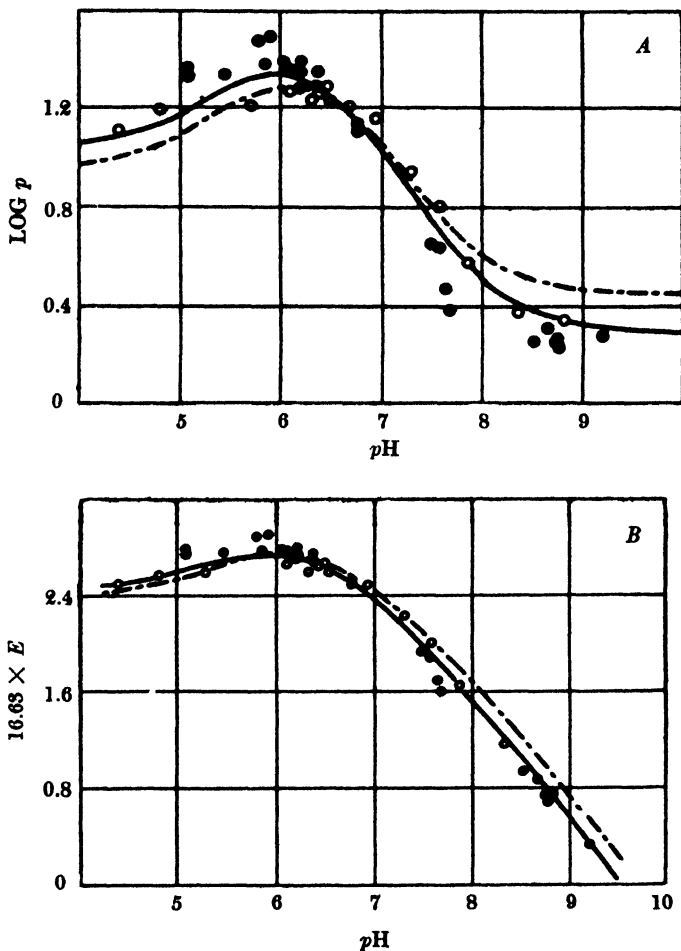
Fig. 10. Wyman's theory and fit of curves describing dependence of gas saturation and oxidation-reduction potential on \text{pH} with observed curves (after Wyman and Ingalls, 3136). A: O, values of \log p , the oxygen dissociation pressure at 50% saturation in relation to \text{pH} , from the data of Ferry and Green; ●, values of \log p calculated from the oxidation-reduction potentials given by Taylor and Hastings. B: ●, oxidation-reduction voltages \times 16.63 for 50% oxidation, from the data of Taylor and Hastings; O, values of the same calculated from the oxygen dissociation pressures given by Ferry and Green. All curves are calculated on the basis of dissociation constants discussed in the text.
