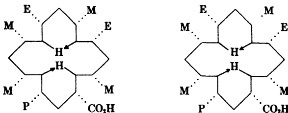
Fig. 20. Prototropic isomerism.
