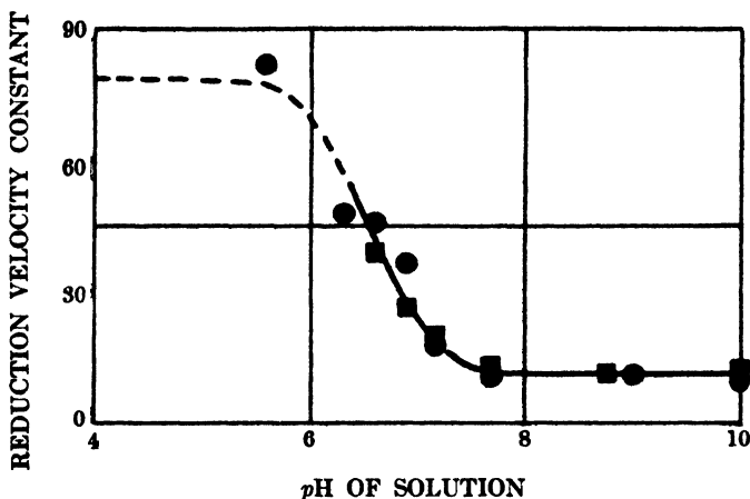
Fig. 11. \text{pH} dependence of rate of dissociation of oxyhemoglobin for two different blood samples (after Hartridge and Roughton, 1148).
