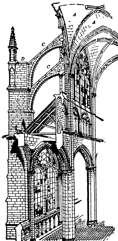
CROSS SECTION OF AMIENS CATHEDRAL
