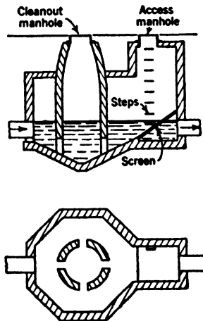
FIG. 75. Grit Chamber for Private Systems.
