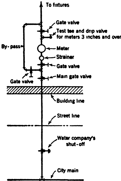
FIG. 27. Service Piping.
