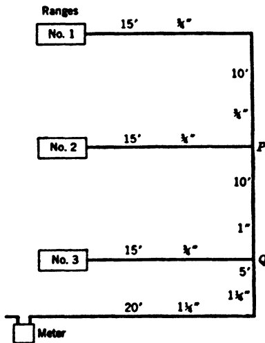
FIG. 87. Layout of Piping for Small Apartment House.
