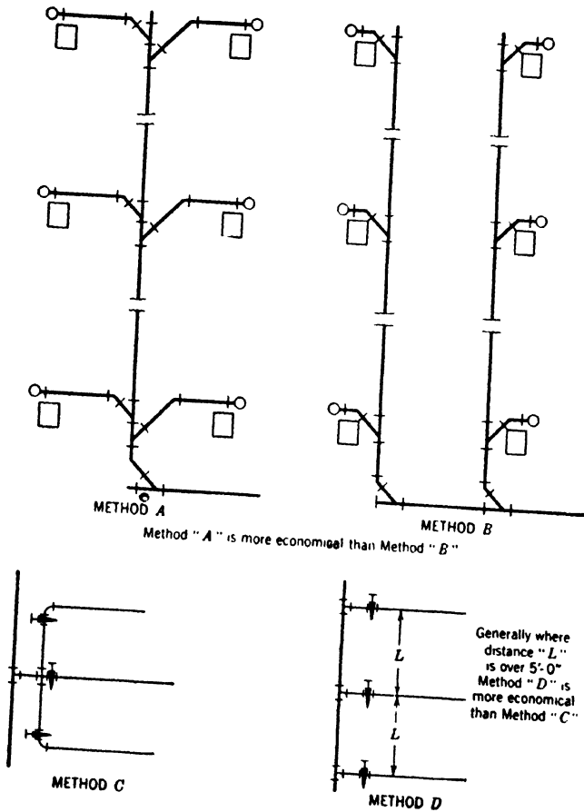
FIG. 23. Piping Economies.
