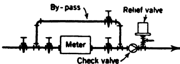
FIG. 37. Water-Meter Connections.
