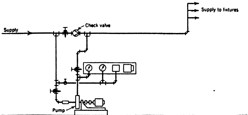
FIG. 31. Booster System.
