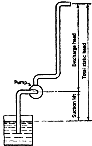
FIG. 21. Pumping Conditions.
