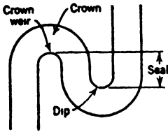
FIG. 57. Parts of Trap.
