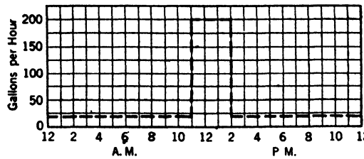
FIG. 108. Hourly Hot Water Demands for Each 1,000 Gallons Daily Hot Water Load. (From Water Heating (20).)
