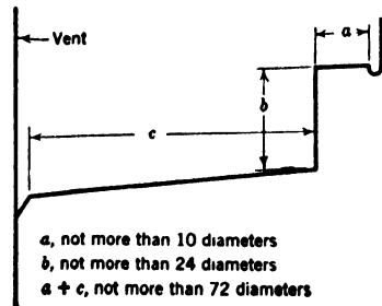
FIG. 67. Limitations to Vents for Flat-Bottomed Fixtures.
