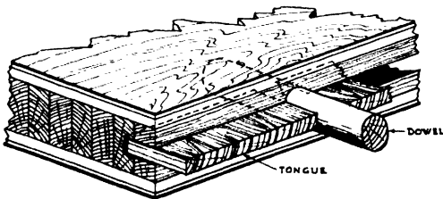
SKETCH SHOWING TONGUE & DOWEL
