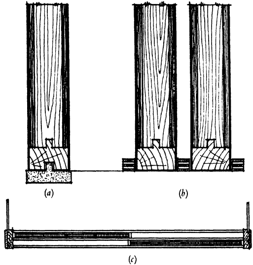
FIG. 197.—SLIDING DOORS.
