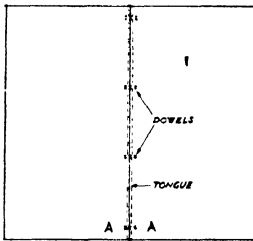
ELEVATION OF PANELS SHOWING POSITION OF TONGUE & DOWELS
