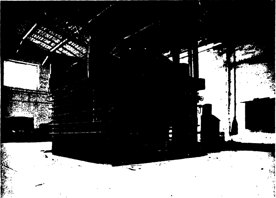
FIG. 54.—A LARGE HOT PRESS CAPABLE OF PRODUCING BOARDS 137"×89".
