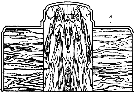
FIG. 203. Settee-end constructed with \frac{3}{4} " Oregon Pine plywood faced with \frac{3}{8} " veneered plywood. The dotted lines indicate line of upholstery.
