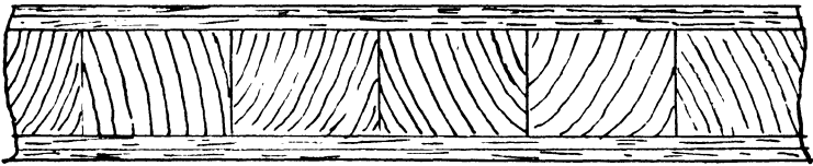
FINNISH TYPE OF BLOCKBOARD BLOCKS ABOUT \frac{5}{8} INCH WIDE
