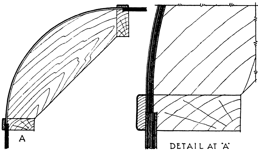
FIG. 194.—CONSTRUCTION OF CURVED CORNERS.
