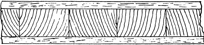
BLOCKBOARD BLOCKS NOT EXCEEDING 1 INCH WIDE
