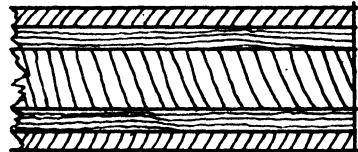
5-ply construction—stout heart.
