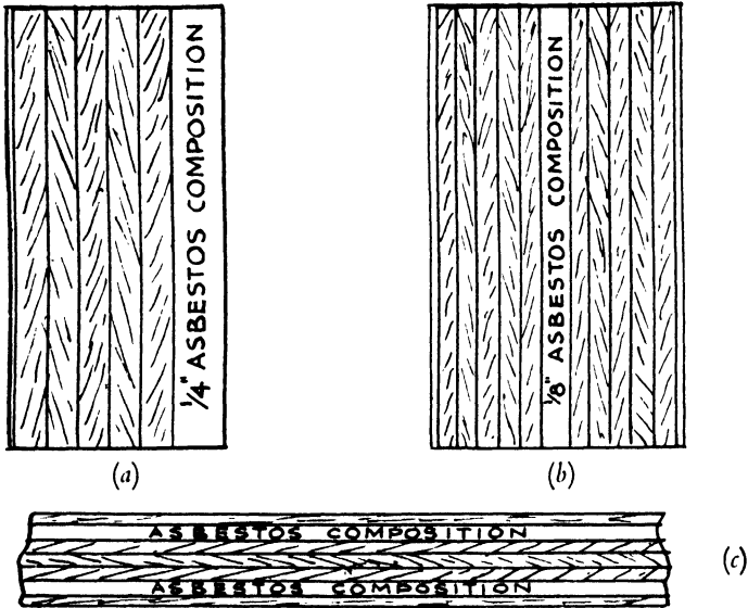
FIG. 78.—COMPOSITE BOARDS.
