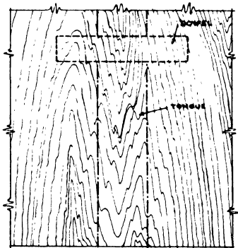
DETAIL ELEVATION AT 'A-A'
