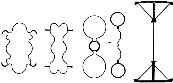
FIG. 71. SPAR SECTIONS
