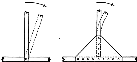
FIG. 25. PIN JOINT AND RIGID JOINT
