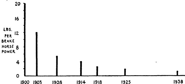
FIG. 17. REDUCTION IN WEIGHT OF INTERNAL COMBUSTION ENGINES
