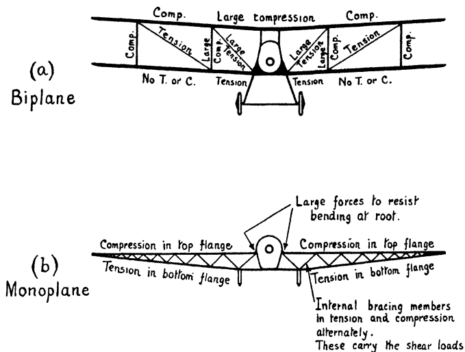
FIG. 72. LOADING IN BIPLANE AND MONOPLANE STRUCTURES
