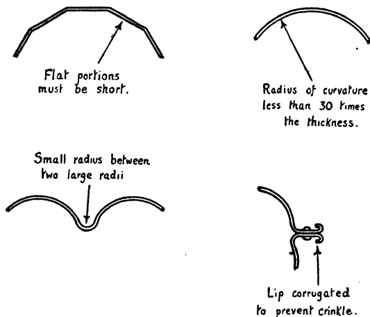
FIG. 67. PRINCIPLES OF CORRUGATION
