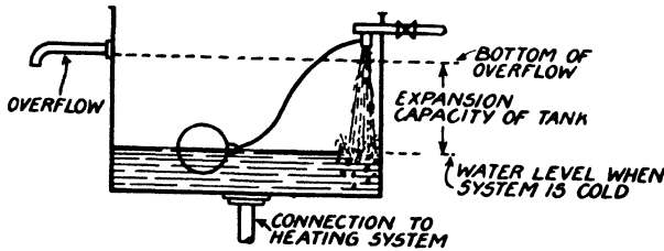
Fig. 39. - A TYPICAL FEED AND EXPANSION TANK
