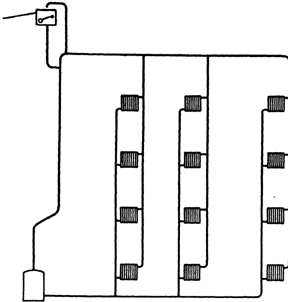
Fig. 15.- TWO-PIPE DROP SYSTEM
