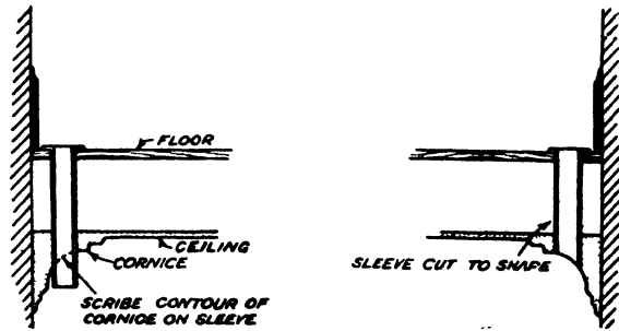
Fig. 12.—WHEN A SLEEVE PASSES THROUGH A CORNICHE The shape of the cornice should be scribed on it; the sleeve can then be cut to fit the curve as shown on the right.
