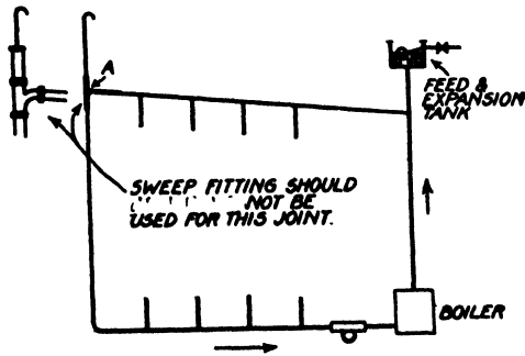
Fig. 43.—THE DRAWBACK OF THE ARRANGEMENT IN FIG. 42 IS ALMOST COMPLETELY OBIVIATED BY THE ABOVE ARRANGEMENT
