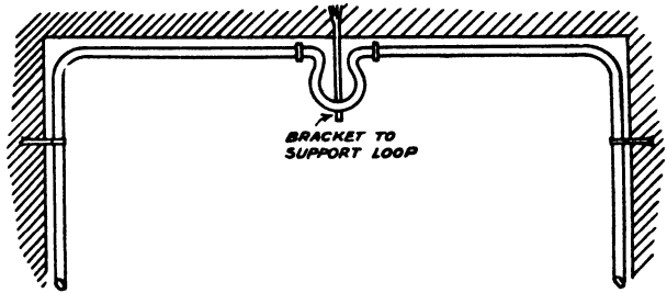
Fig. 6. - WHEN A LOOP IS USED A SPECIAL BRACKET SHOULD BE PROVIDED TO SUPPORT IT
