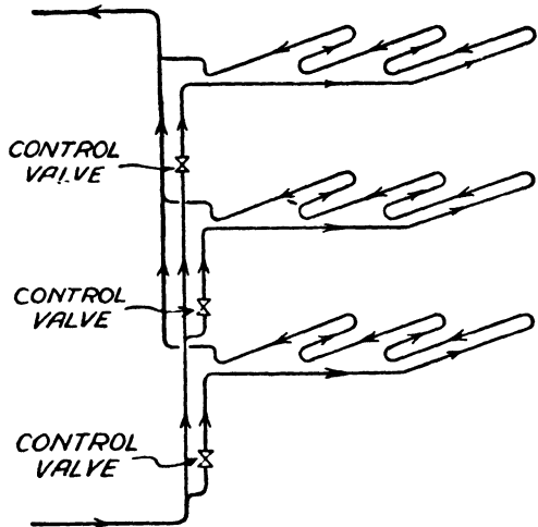
Fig. 30.—A TYPICAL ARRANGEMENT OF PIPE CIRCUIT FOR EMBEDDED PANEL WARMING
