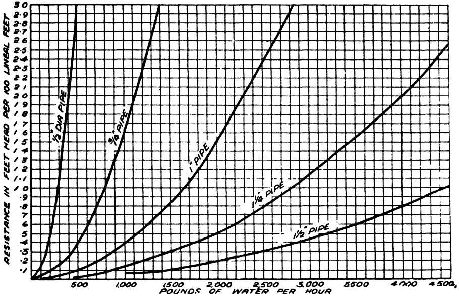
Fig. 9. CHART SHOWING FLOW OF WATER FOR ACCELERATED SYSTEMS
