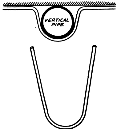
Fig. 18.—PASSOVER BEND FOR CROSSING VERTICAL PIPE First make the centre bend almost a hairpin shape.
