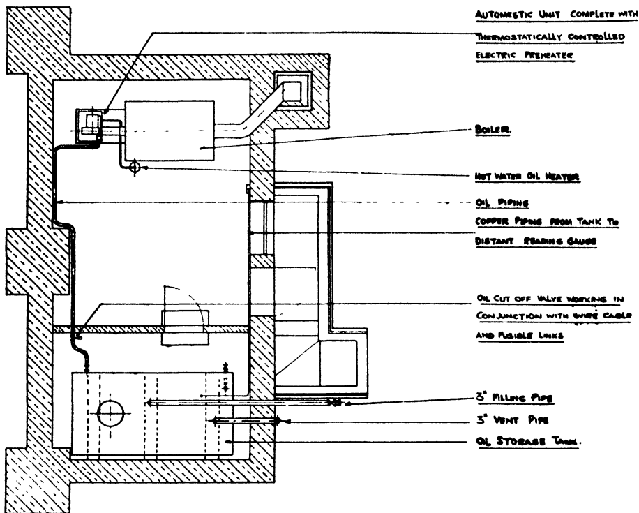
Fig. 24.—LAYOUT OF AUTOMATIC OIL-BURNING EQUIPMENT FOR A HEATING BOILER Designed to burn heavy fuel oil. Scale: \frac{1}{4} in. = 1 ft
