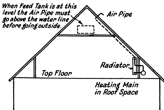
Fig. 16. DROP SYSTEM HORIZONTAL MAIN IN SMALL ROOF SPACE ON TOP FLOOR LEVEL
