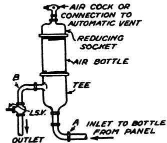
Fig. 47.—METHOD OF VENTING EMBEDDED PANEL
