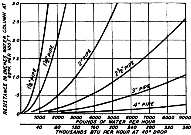
Fig. 4.—PIPE CAPACITIES FOR GRAVITY WATER-HEATING SYSTEM
