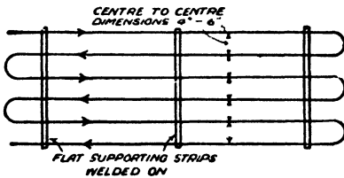
Fig. 28.—HAIRPIN TYPE OF EMBEDDED PANEL
