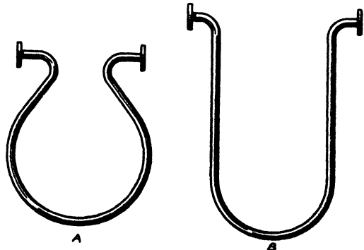
Fig. 1.—EXPANSION LOOPS
