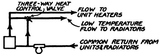
Fig 11.--COMBINED HOT-WATER UNIT HEATER AND RADIATOR SYSTEM
