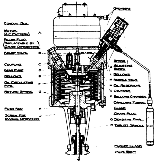
ELECTRO-MECHANIC POWER UNIT MODEL HQ (TEMPERATURE SENSITIVE INSIDE) (SERIES I) 11673
