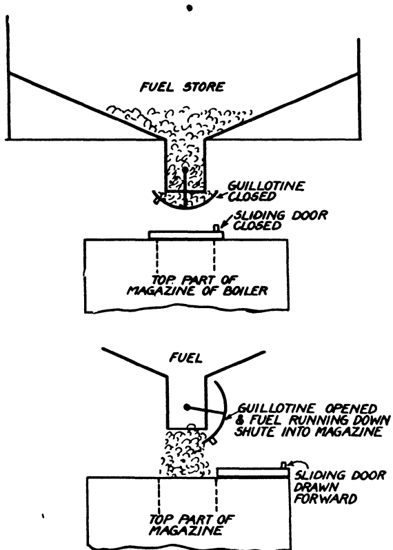
Fig 13. -- FUEL STORE FOR GRAVITY-FED BOILER
