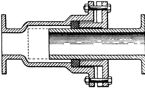
Fig. 4.—SLIDING EXPANSION JOINT
