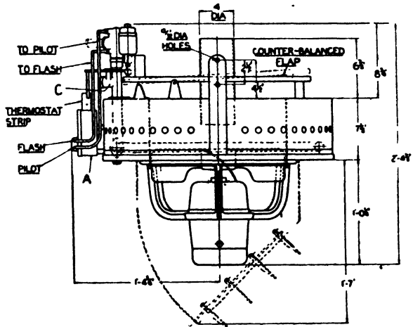
Fig. 14.- VERTICAL SECTION THROUGH GAS UNIT HEATER
