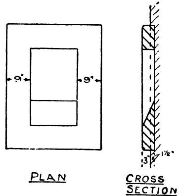
Fig. 1.—TYPICAL ARRANGEMENT OF BASE FOR HEATING-BOILER
