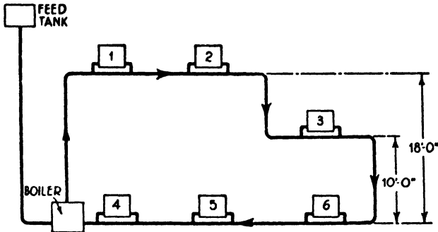
Fig. 2. - IN A SIMPLE SINGLE-PIPE CIRCUIT THE MEAN HEIGHT OF THE SYSTEM MUST BE ASCERTAINED
