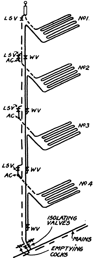
Fig. 38. —A BETTER ARRANGEMENT FOR EMBEDDED PIPE PANEL HEATING SYSTEM Note flow of water is upward through each panel. Note air cock to each panel and arrangement of valves.
