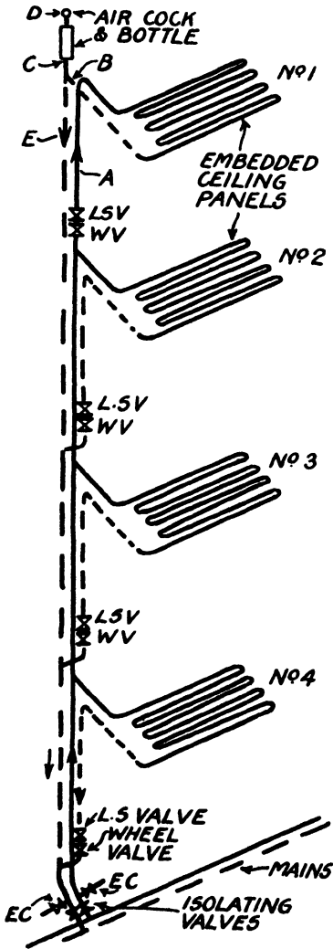
Fig. 37. —A SMALL SECTION OF AN EMBEDDED PIPE PANEL HEATING SYSTEM The above is a common arrangement of piping but one with which air troubles are likely. L.S.V., lock-shield valve.
