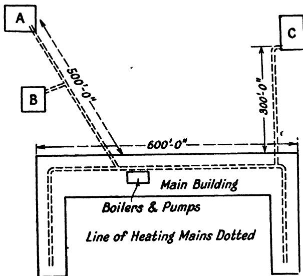
Fig. 18.-- TYPICAL EXAMPLES OF AN ACCELERATED SYSTEM
