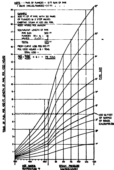
Fig. 1. —FUEL WASTAGE ON EXPOSED PIPES WITH SURROUNDING TEMPERATURE 70° F.
