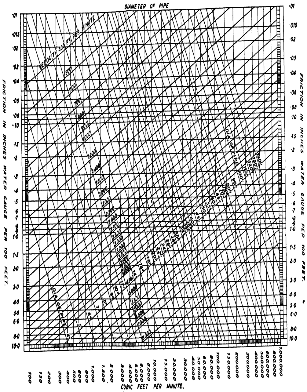
Fig. 15.—CAPACITIES AND RESISTANCES OF GALVANIZED IRON DUCTWORK
