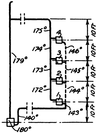
Fig. 23 —TWO-PIPE DROPPING SYSTEM
