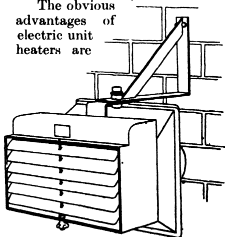
Fig. 13.—WALL BRACKET MOUNTING OF ELECTRIC HEATER
