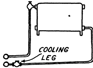
Fig. 15.—A SUPERIOR METHOD OF CONNECTION
