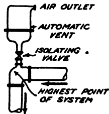
Fig. 45.—UNSATISFACTORY CONNECTION TO AUTOMATIC VENT
