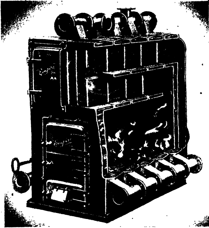
Fig. 5 —ANOTHER TYPE OF SECTIONAL STEEL BOILER IN WHICH THE SECTIONS ARE HELD TOGETHER BY MEANS OF FLANGED FLOW AND RETURN HEADERS
