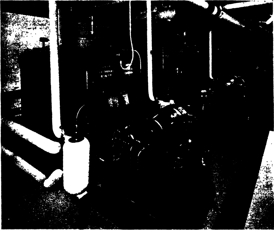
Fig. 23. — AUTOMATIC HEAVY OIL BURNERS FITTED TO TWO DAVEY PAXMAN STEEL SECTIONAL BOILERS, EACH RATED AT 1,250,000 B.T.U. HOUR AND ONE CRANE DOMESTIC SUPPLY BOILER RATED AT 250,000 B.T.U.
