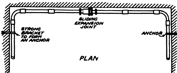
Fig. 5.—FIXING FOR LONG LENGTH ALONG A WALL
