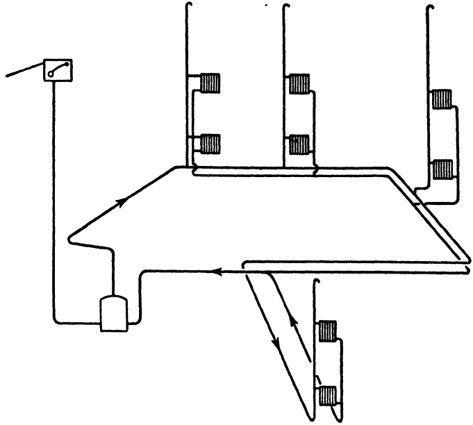
Fig. 13. — TWO-PIPE UP-FEED SYSTEM.— 3
