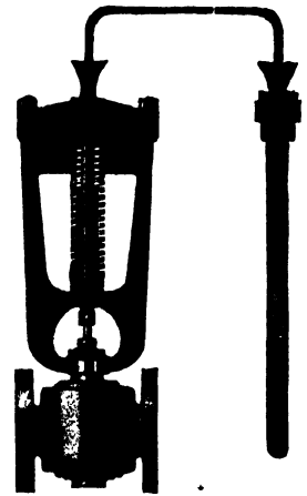
By courtesy of the Drayton Regulator and Instrument Co., Ltd. Fig. 3.—SECTIONED VIEW OF STEAM VALVE DIRECTLY OPERATED BY VAPOUR PRESSURE SYSTEM
