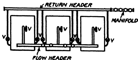
Fig. 9.—METHOD OF COUPLING BOILERS
