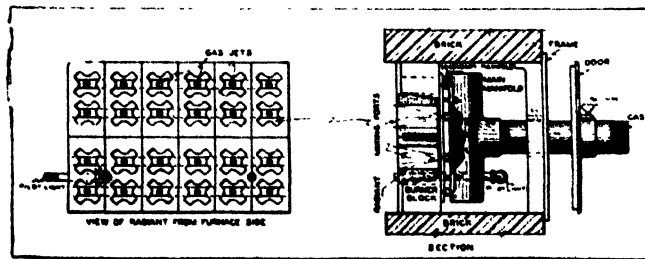
Fig. 19.—GAS COMBUSTION CHAMBER AND MIXING PORTS
