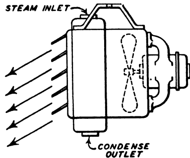
Fig. 2.—TYPE OF UNIT HEATER SUSPENDED FROM CEILING
