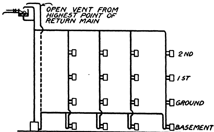
Fig. 27.—RADIATORS AT OR BELOW LEVEL OF BOILER CONNECTED TO AN OVERHEAD RETURN MAIN
