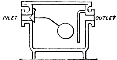
Fig. 2.—CLOSED-FLOAT TRAP
