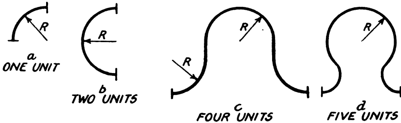
Fig. 2. - FOUR TYPES OF EXPANSION BENDS
