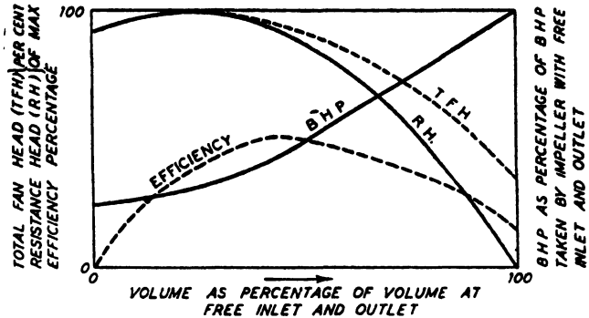
Fig. 7.—CHARACTERISTIC CURVES FOR CENTRIFUGAL FANS
