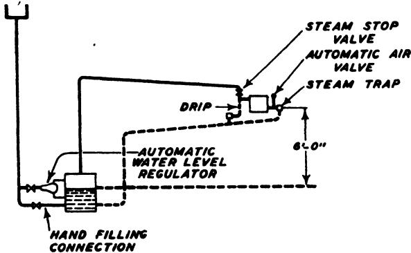
Fig. 9.—THE ESSENTIAL FEATURES OF A GRAVITY STEAM SYSTEM FOR UNIT HEATERS
