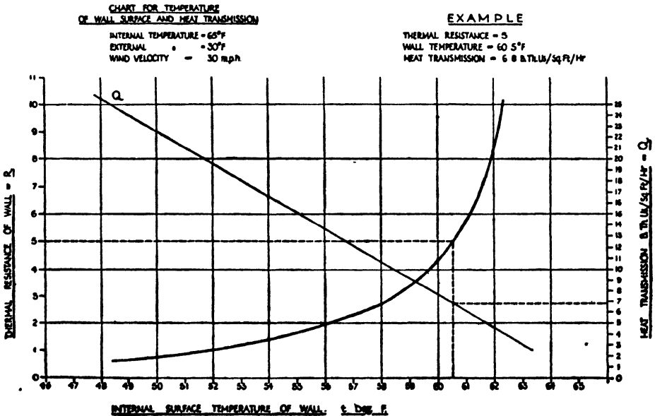
Fig. 3.—INNER SURFACE TEMPERATURE IN RELATION TO THE THERMAL RESISTANCE OF A WALL, ETC.
