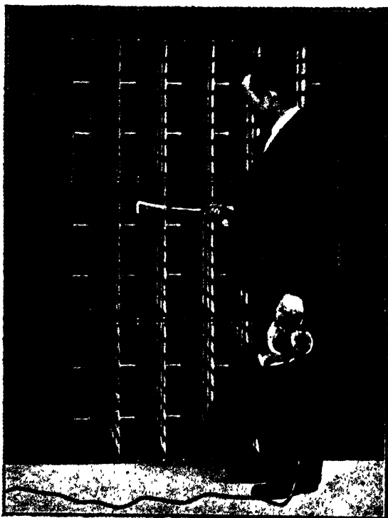
Fig. 2. —15,000 C.F.M. INSTALLATION OF SIX FOUR SQUARE FOOT UNITS SHOWING SIMPLE CLEANING EQUIPMENT AND METHOD OF CLEANING (Messrs. Vokes, Ltd.)
