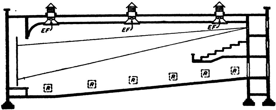
Fig. 16.—A SMALL CINEMA
