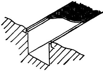
Fig. 3.—CHEQUER-PLATE TRENCH COVER AND RAILS
