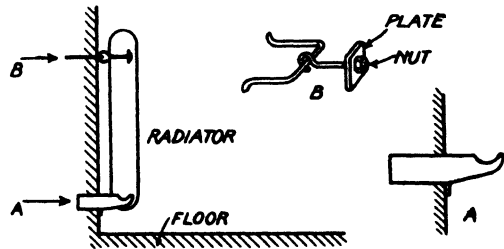
Fig. 3.—METHOD OF FIXING RADIATORS TO WALLS
