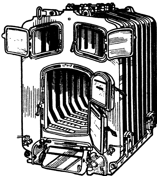
Fig. 1.—CAST-IRON BOILER BUILT UP IN SECTIONS
