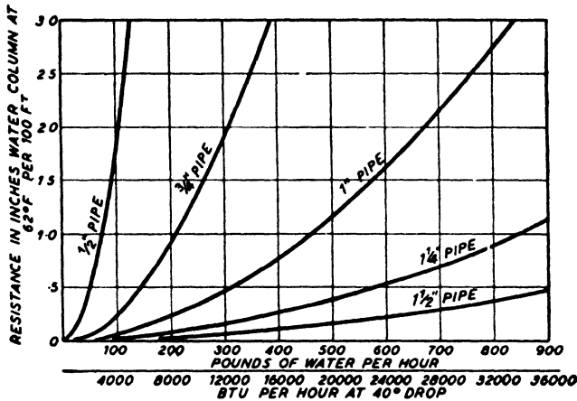
Fig. 5. — PIPE CAPACITIES FOR GRAVITY WATER-HEATING SYSTEMS
