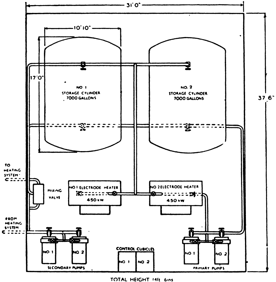
Fig. 17.—TYPICAL BOILER-HOUSE LAYOUT OF ELECTRODE THERMAL STORAGE PLANT FOR HEATING BUILDINGS
