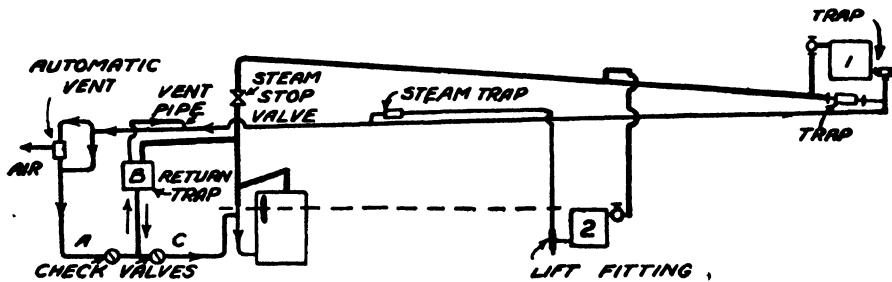
Fig. 17.—SYSTEM WITH RADIATOR ON SAME LEVEL AS BOILER
