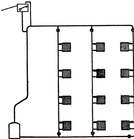
Fig. 14. — DROP SYSTEM
