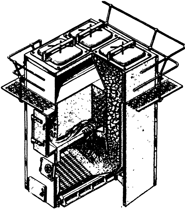
Fig. 2.—TYPICAL EXAMPLE OF MAGAZINE OR GRAVITY FEED BOILER
