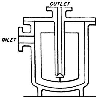
Fig. 3.—OPEN-FLOAT TRAP
