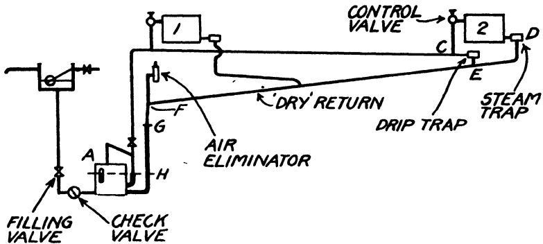
Fig. 9 - SIMPLE ARRANGEMENT OF STEAM BOILER, RADIATORS AND PIPING
