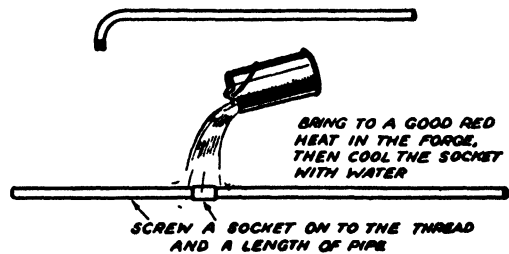
Fig. 19.—SHOWING SHORT BEND CLOSE UP TO THE THREAD AND HOW TO MAKE IT
