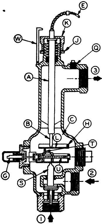
FIG. 6-1. — Sarcotherm valve. (Sarcotherm Controls, Inc.)
