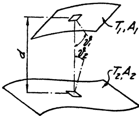
FIG. 10-6.—A general case of heat exchange between areas.
