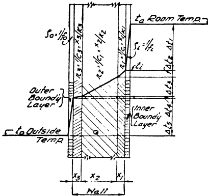
FIG. 10-2.—Temperature gradient in wall.
