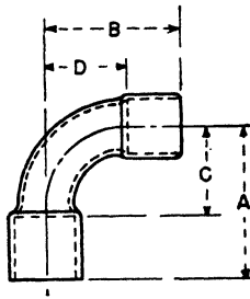
Wrought 90-deg. elbow. Roughing-in Measurements
