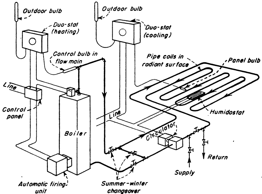
FIG. 9-4.—Control system for radiant heating and cooling.
