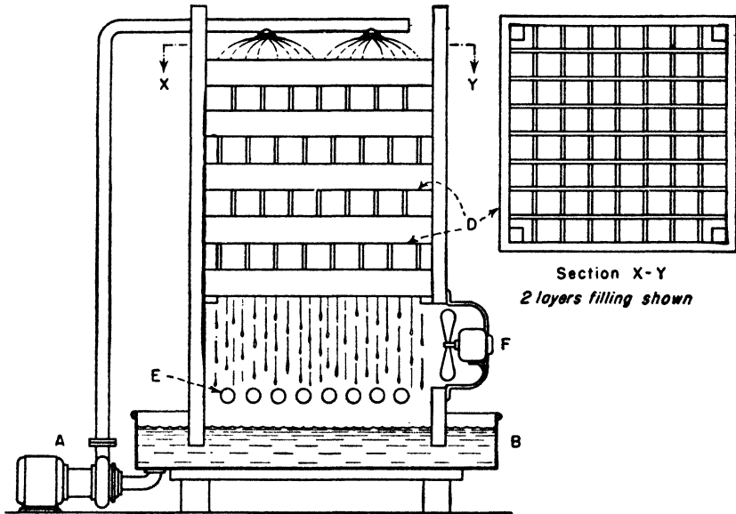
FIG. 9-3.—Cooling-tower design.
