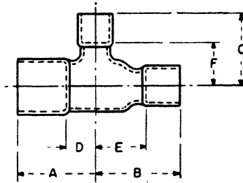
Wrought tee.
