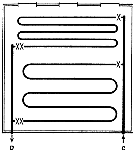
FIG. 8-2.—Sinuous coil.
