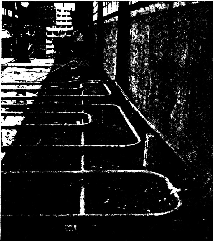
FIG. 8-4.—Welded wrought-iron pipe connections. (A. O. Smith Corporation.)
