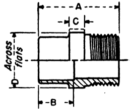
Wrough male adapter.
