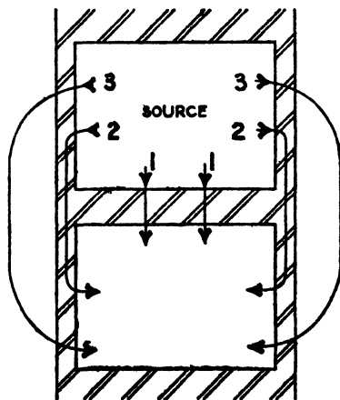
FIG. 10 FLANKING TRANSMISSION
