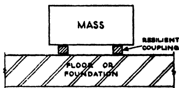
FIG. 11 MECHANICAL LOW PASS FILTER
