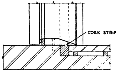
FIG. 48 SEAL TO SILL ON FLOATING FLOOR
