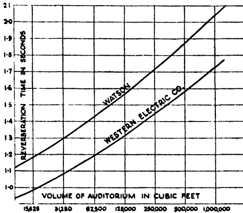
OPTIMUM REVERBERATION TIME OF AUDITORIA FOR 512 C.P.S.
