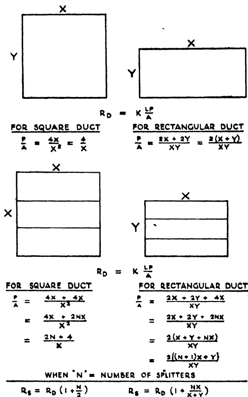
FIG. 68 EFFICIENCY OF SPLITTERS
