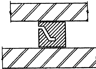
FIG. 14. DIFFERENTIAL COUPLING HAVING TWO VALUES OF COMPLIANCE
