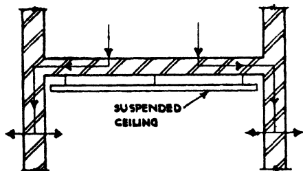
FIG. 32 SUSPENDED CEILING
