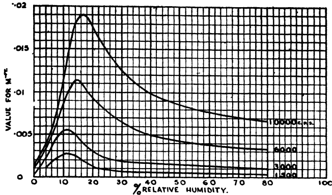
FIG. 77 PLOT OF M AGAINST RELATIVE HUMIDITY (AFTER KNUDSEN)
