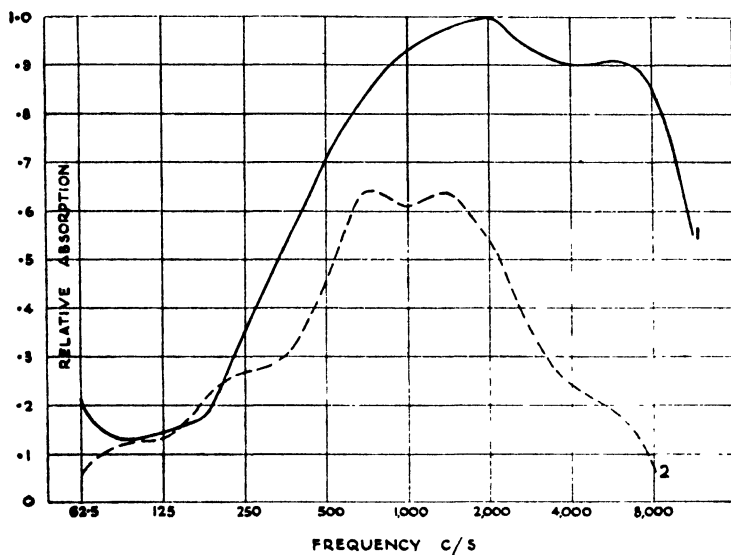
FIG. 86 VARIATION OF ABSORPTION WITH PERFORATION IN OIL-CLOTH STUCK TO 1 IN. FELT
