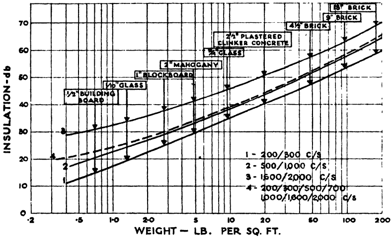
FIG. 18A INSULATION v. LOGARITHM OF MASS
