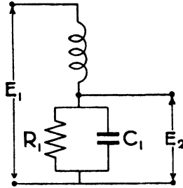
FIG. 98 EQUIVALENT DIVIDING NETWORK FOR DAMPED MASS MOUNTING
