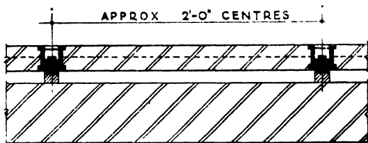
FIG. 29 B.R.S. FLOATING FLOOR
