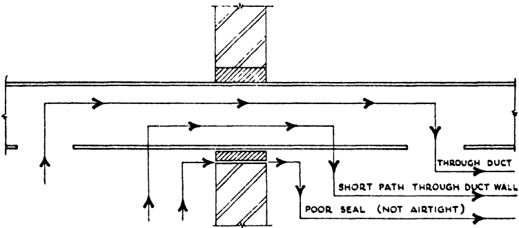
FIG. 62 CROSS TALK THROUGH DUCTS
