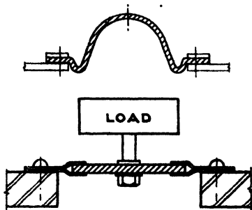
FIG. 102 VERTICAL MOUNTING ISOLATOR
