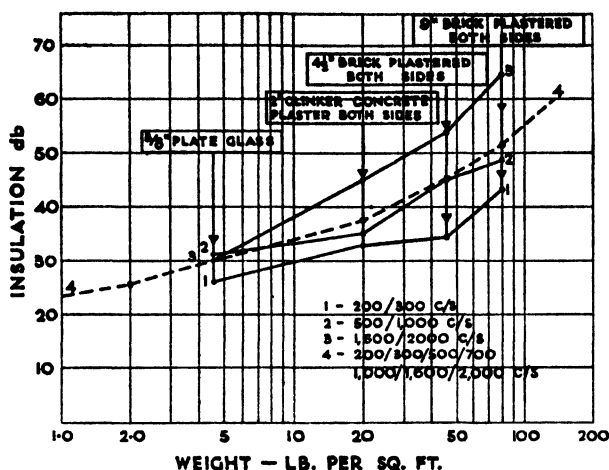
FIG. 18B INSULATION v. LOGARITHM OF MASS
