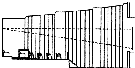
FIG. 80 ELEVATION OF A REVIEW ROOM (M.G.M. ELSTREE STUDIOS)
