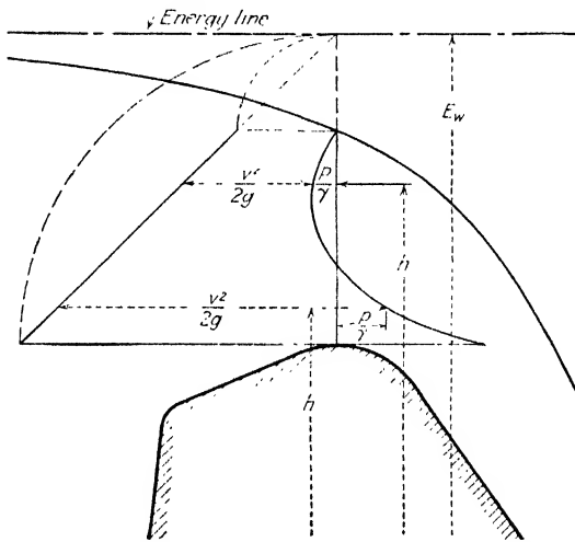
FIG. 10.—Non-hydrostatic pressure distribution in curvilinear motion.
