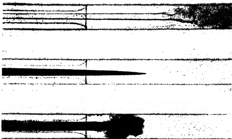
FIG. 78.—Instability of laminar flow at a boundary expansion, the point of disruption moving upstream with increasing Reynolds number. The form of the dye cloud in the center photograph is evidence of parabolic velocity distribution.
