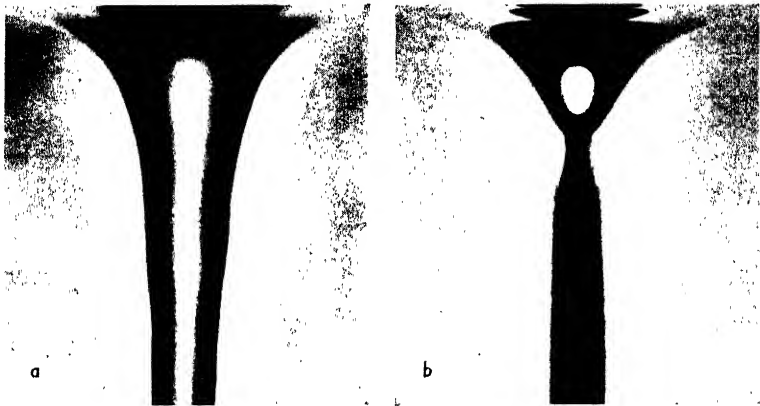
FIG. 27.—Profiles of (a) the potential and (b) the combined vortex, occurring above an orifice in the bottom of a tank. The central portion of the combined vortex has been colored by dye.
