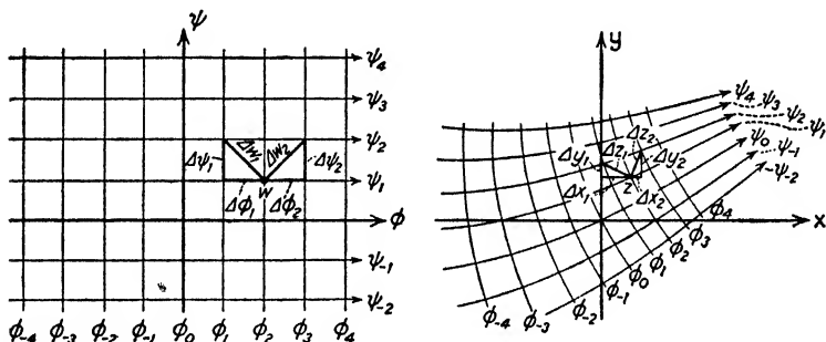
FIG. 42.—Conformal transformation.
