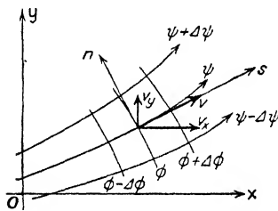
Fig. 36.—Stream and potential lines.
