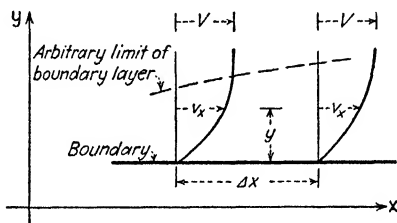
FIG. 84.—Boundary-layer growth in the direction of flow.
