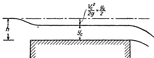
Fig. 171.—Customary treatment of the broad-crested weir.
