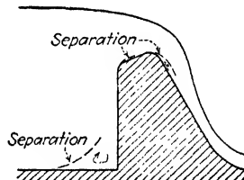
FIG. 65.—Separation at a spillway.
