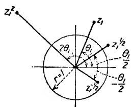
FIG. 40.—Powers of complex numbers.
