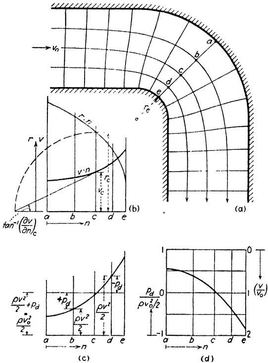
FIG. 11.—Application of the flow net.
