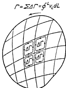
FIG. 22.—Circulation.
