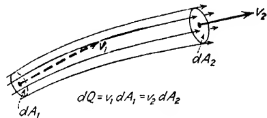
FIG. 2.---Stream filament.
