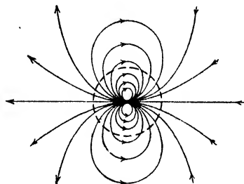
FIG. 32.—Three-dimensional doublet.
