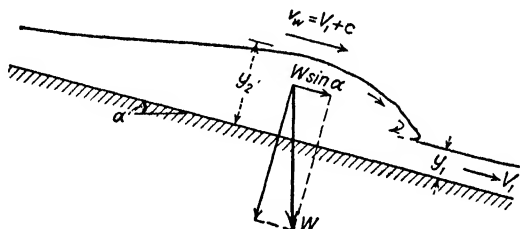
FIG. 223.—Profile of a roll wave.
