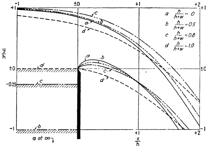
FIG. 168.—Variation in the weir nappe with \frac{h}{h+w} .
