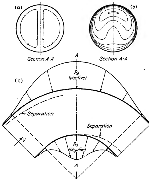
FIG. 139.—Flow at a conduit bend.
