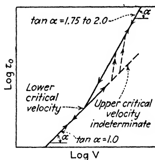
FIG. 80.—Boundary shear versus mean velocity in the critical region.
