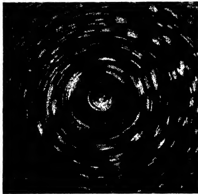
FIG. 28.—Velocity distribution of the combined vortex as indicated by the paths of aluminum particles during a short time exposure.
