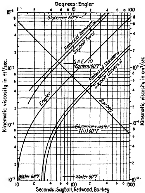
FIG. 242.—Viscometer characteristics.
