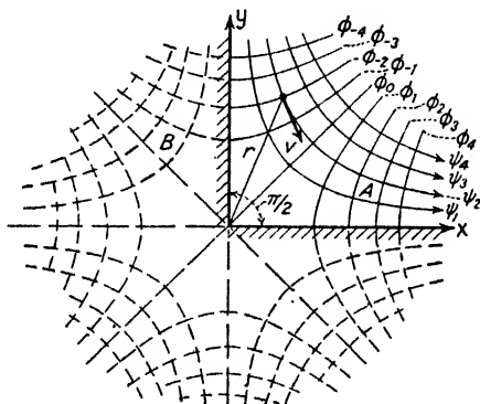
FIG. 44.—Potential flow at a 90^\circ boundary angle.
