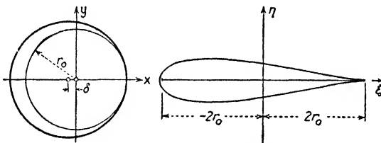
FIG. 57.—Streamlined foil.
