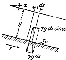
FIG. 143.—Definition sketch—boundary shear in an open channel.
