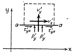
FIG. 82. - Apparent stresses resulting from momentum transport.
