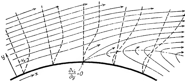
FIG. 93. - Separation of flow from a curved boundary; vertical scale is enlarged.
