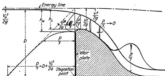
FIG. 167.—Pressure distribution at a spillway designed after the ventilated nappe of a weir.
