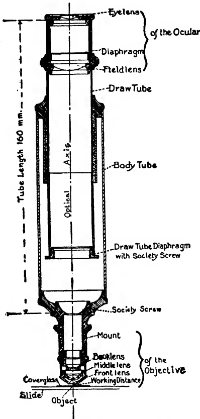
FIG. 55.—Sectional View of Microscope Tube Including Ocular and Objective.
