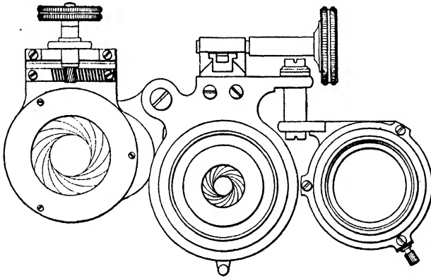
FIG. 67.—Top view of a Substage Attachment with Condenser and Lower Iris Diaphragm Thrown out of Optical Axis.
