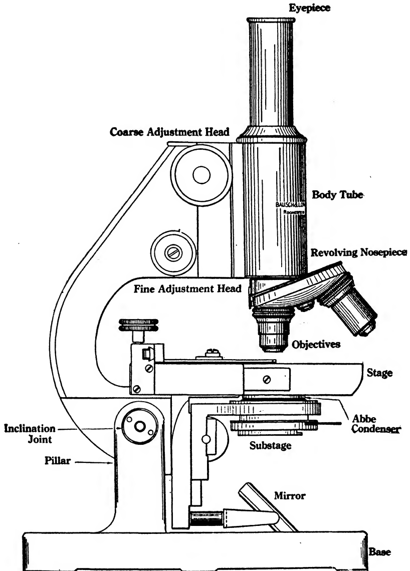
FIG. 54.—A Compound Microscope with Parts Named
