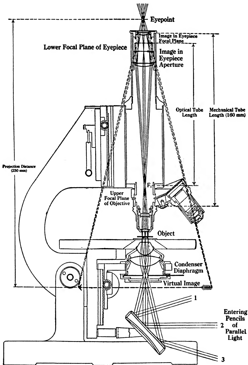
FIG. 58.—Diagram Showing Path of Light Rays through the Compound Microscope, Together with Images (Courtesy the Bausch & Lomb Optical Company)
