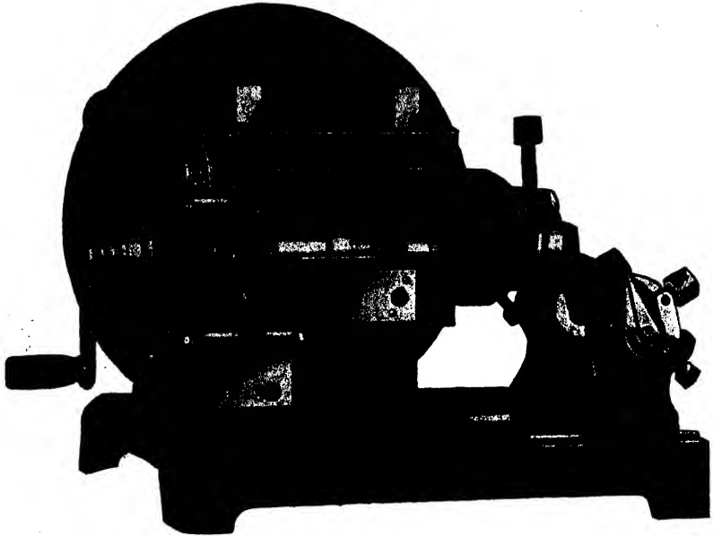
FIG. 28.—Spencer Rotary Microtome
