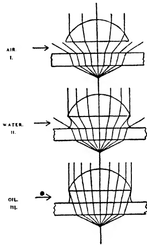
FIG. 70.—Diagram to Illustrate the Relative Amounts of Light Utilised with Dry, Water Immersion, and Homogeneous Oil Immersion Objectives, Respectively (after Bausch).
