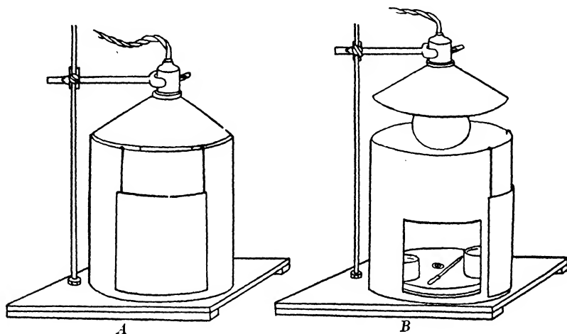
FIG. 25.—Wisconsin Paraffin-melting Oven
