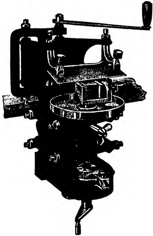
FIG. 32.—Freezing Microtome
