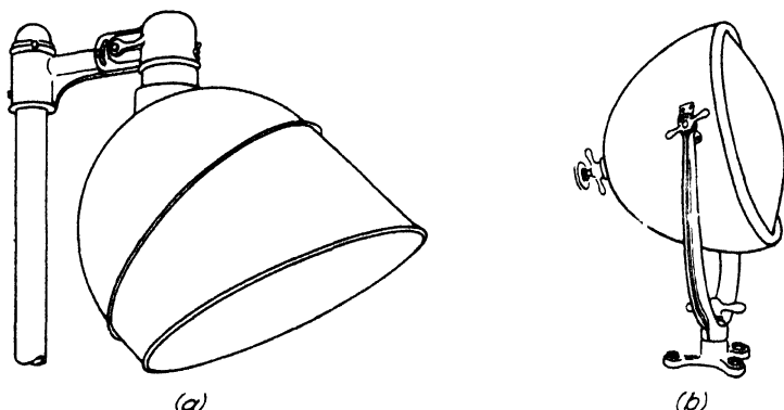
FIG. 5-10. 2 Types of floodlight equipment. (a) Open floodlight. (b) Projector.
