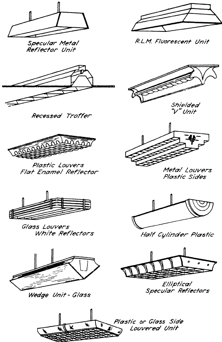
FIG. 14-7. Typical fluorescent lamp luminaires.
