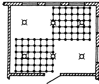
(c)-Unsymmetrical Lighting • - Test Stations
