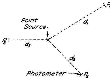
FIG. 4-2. Intensity is independent of distance and position when a point source of light is considered.
