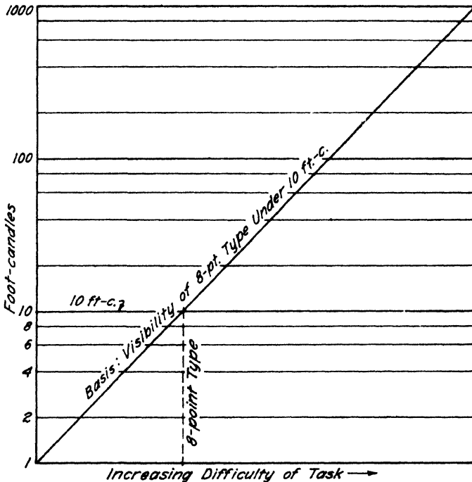
FIG. 6-3. 13 Relative foot-candle prescription of light based on the task.
