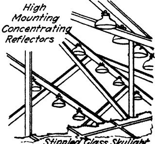
FIG. 5-7. 3 Typical direct lighting luminaires.
