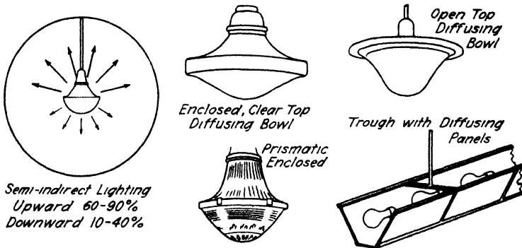
FIG. 8-7: Typical semi-indirect lighting luminaires.
