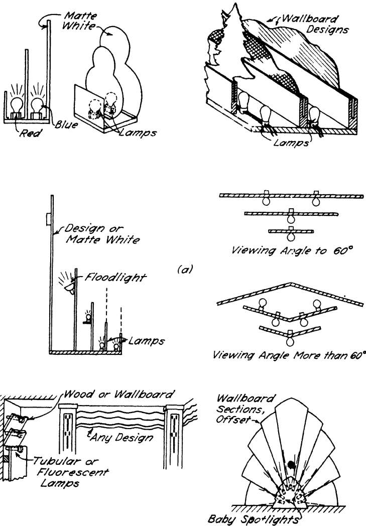
FIG. 11-11A. 1, 6, 22 Setbacks.
