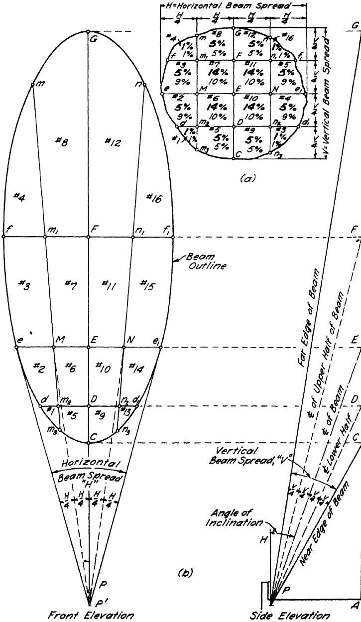
FIG. 10-10. 4 (a) Per cent lumens falling into various parts of the floodlight pattern. Lower figures for accurate parabolic reflectors with C 7-A filament lamp. Bold-face type figures for general floodlights. (b) Problem in offset lighting.
