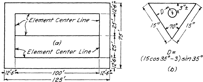
FIG. 4-9. Figure for problem in luminous elements.
