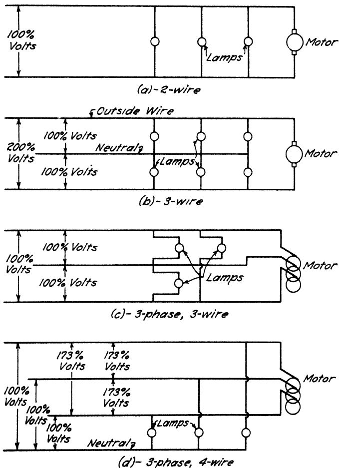
FIG. 4-13. Different types of distribution systems, (a) and (b) for direct current and single-phase alternating current; (c) and (d) for three-phase alternating current.
