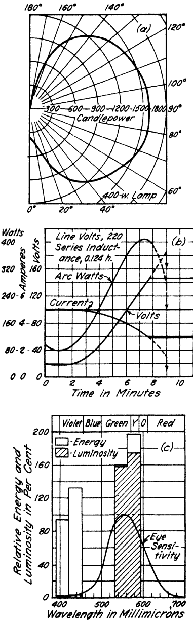
FIG. 14-6. 5 (a) Candlepower distribution curve for a 400-w. Type-H lamp. (b) Characteristics of the lamp at starting. (c) Spectral energy distribution.
