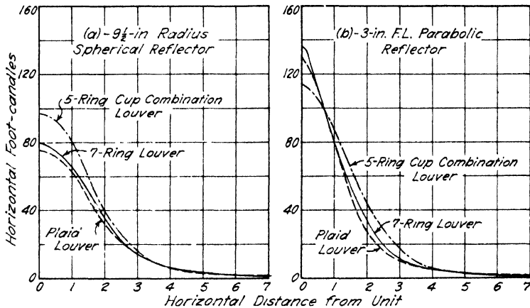
FIG. 7-8. 4 Effect of shape of louver upon the efficiency.
