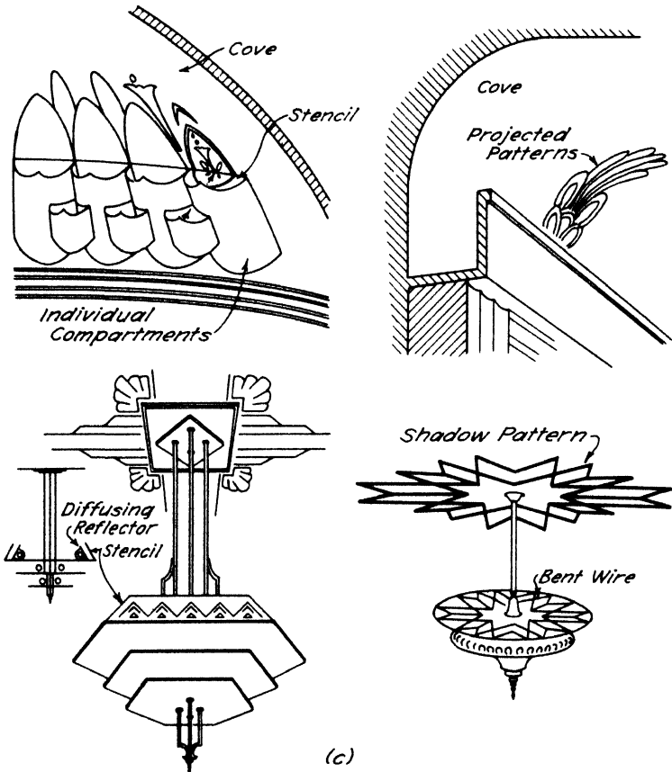
FIG. 9-11B.4. 23 Projected patterns.
