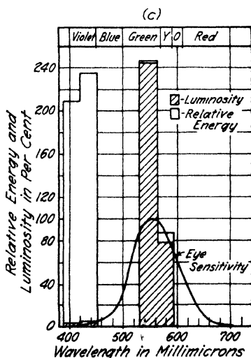
FIG. 12-6. 5, 23 Characteristics and circuit for a low-pressure mercury vapor lamp. (a) A modern power factor corrected circuit. (b) Characteristics of the lamp with respect to voltage. (c) Spectral energy distribution.
