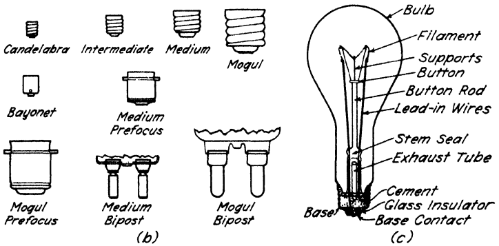
FIG. 5-6. (a) Incandescent lamp bulb designs. (b) Incandescent lamp base designs. (c) Parts of the incandescent lamp.
