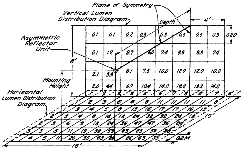
FIG. 16-5. Information from Fig. 15-5 shown in the horizontal and vertical plane of the show window.
