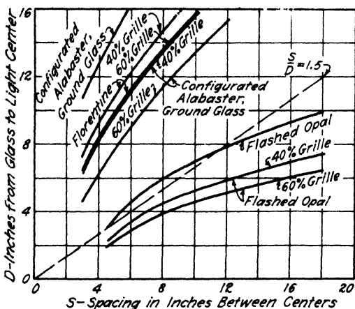
Fig. 1-9. 1 Lamp spacing for acceptable uniformity of brightness.
