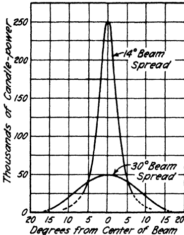
Fig. 1-10. 3 Characteristic beam spreads.
