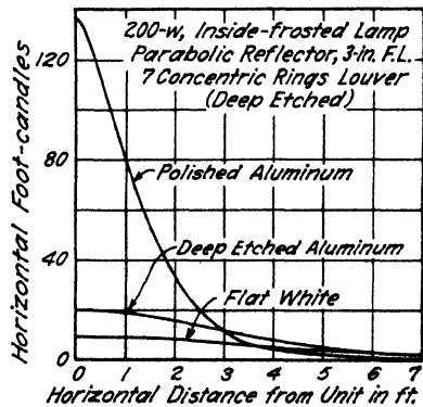
FIG. 8-8. 5 Effect of reflector finish upon the efficiency of louver equipment.
