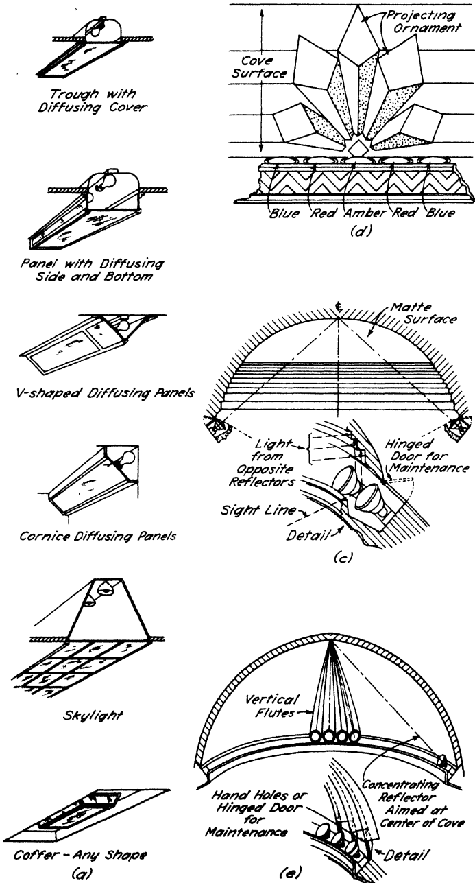
Fig. 1-11A. 4,22 Lighting equipment and covers may be converted for novelty lighting.
