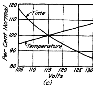
FIG. 6-13. 11 Effect of voltage variation on (a) lamps, (b) motors, (c) heaters.
