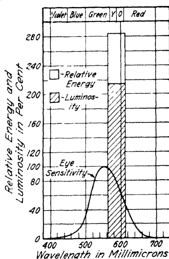
FIG. 15-6. 5 Spectral energy distribution and visual utilization of light from a sodium lamp.
