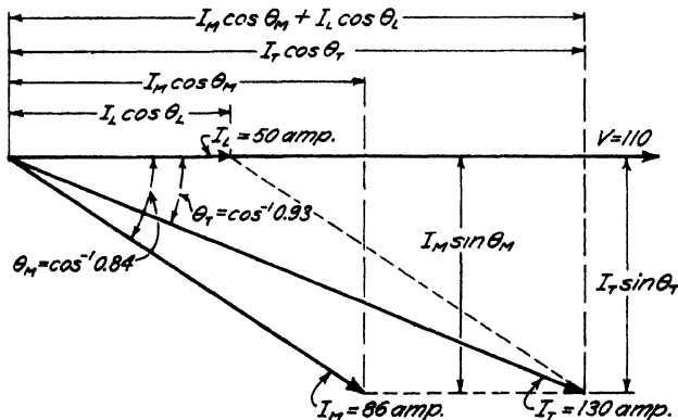
FIG. 5-13. Vector diagram for combining currents of different power factors.
