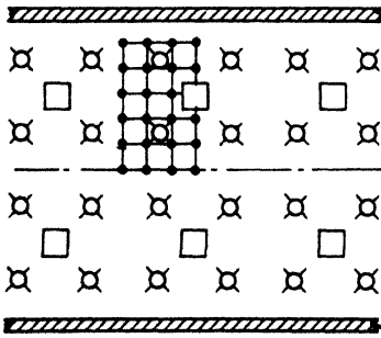
(b)-Large Room - Symmetrical X - Lighting Units • - Test Stations
