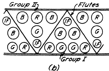
FIG. 8-11A. The colorama and its construction.
