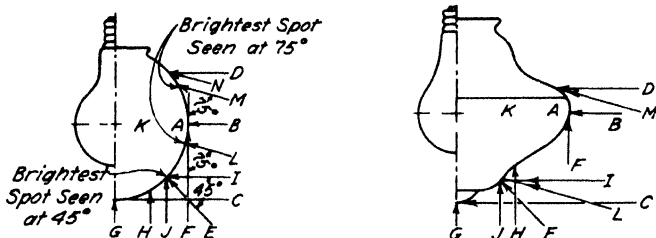
FIG. 3-5. 2 Points on the luminaire which are measured for brightness.
