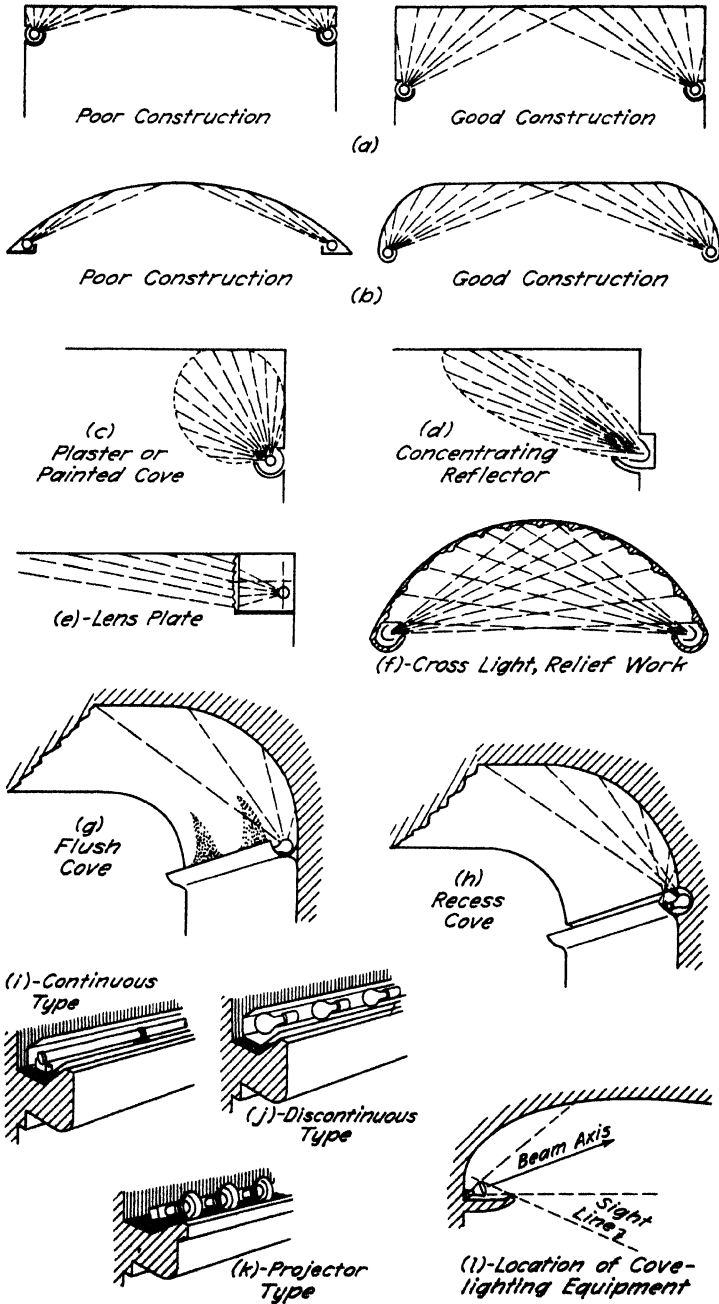
FIG. 2-8.1 Cove lighting
