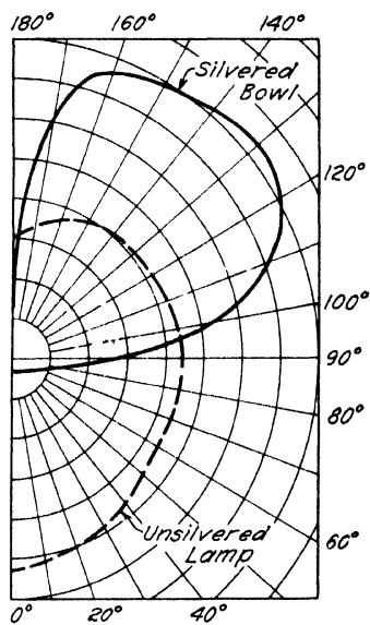
FIG. 6-6. 4 Candlepower distribution curves for the unsilvered and the silver-bowl incandescent lamps.
