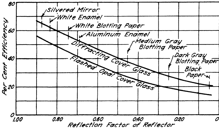
FIG. 3-9. 1 Relation between reflection factor of reflector and efficiency of the unit.
