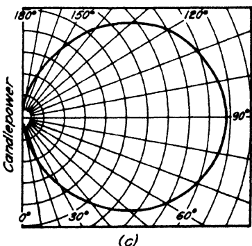
FIG. 16-6. 30 (a) Circuits for fluorescent lamps. (b) The characteristics of fluorescent lamps with voltage change. (c) Candlepower distribution curve for fluorescent lamps.
