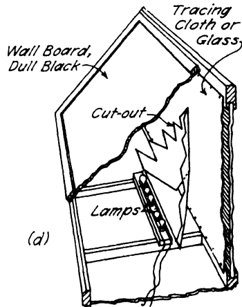
FIG. 8-11B. 1,4 The colorama and its construction.
