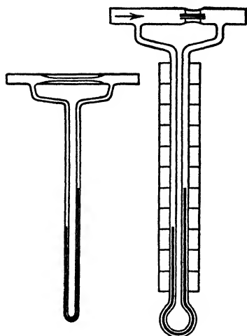
FIG. 8-3. Capillary flowmeter
