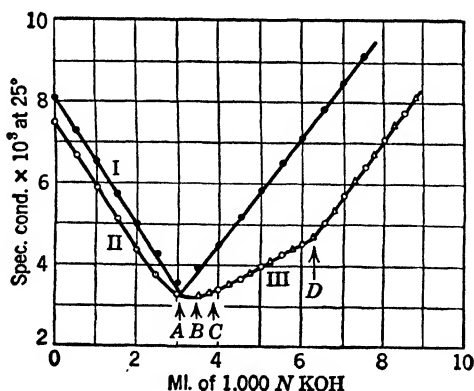
FIG. 5-2. Conductimetric titrations of aqueous fluoboric acid solutions I, ●, unhydrolyzed \text{HBF}_4 solution. II, ○, hydrolyzed \text{HBF}_4 solution. III, △, solution of \text{KBF}_4 + \text{KBF}_3\text{OH} + \text{KHF}_2 . (Courtesy Journal of the American Chemical Society )
