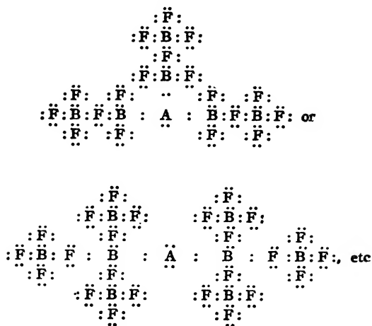
FIG. 4-2. Suggested coordination of argon with polymerized molecules of boron trifluoride
