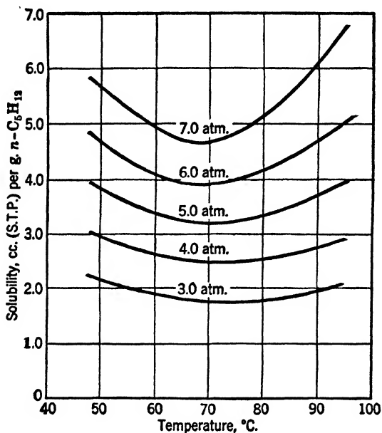
FIG. 2-3. Solubility of boron trifluoride in n -pentane at constant partial pressure of boron trifluoride
