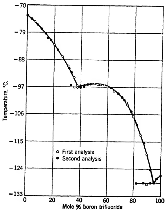
FIG. 4-10. The system sulfur dioxide-boron trifluoride (Courtesy Journal of the American Chemical Society )
