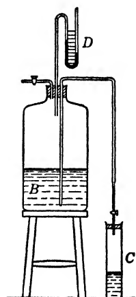
FIG. 8-5. Volume-displacement bottle
