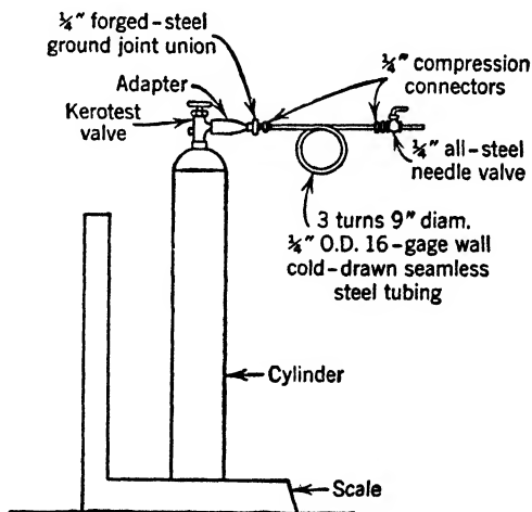
FIG. 8-6. Measuring boron trifluoride from cylinder by weight
