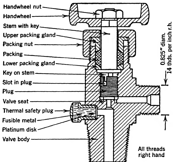
FIG. 8-1. Valve—stem seated (Courtesy The Harshaw Chemical Co.)
