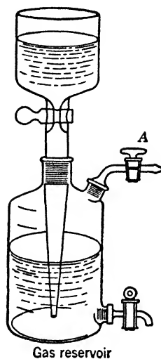
FIG. 8-4. Gas reservoir
