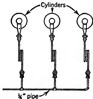
FIG. 8-7. Cylinders connected by means of copper refrigeration fittings (Courtesy The Harshaw Chemical Co.)
