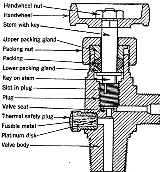
FIG. 8-2. Valve—stem not seated (Courtesy The Harshaw Chemical Co.)
