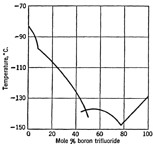
FIG. 4-9. The system hydrogen sulfide-boron trifluoride (Courtesy Journal of Physical Chemistry )
