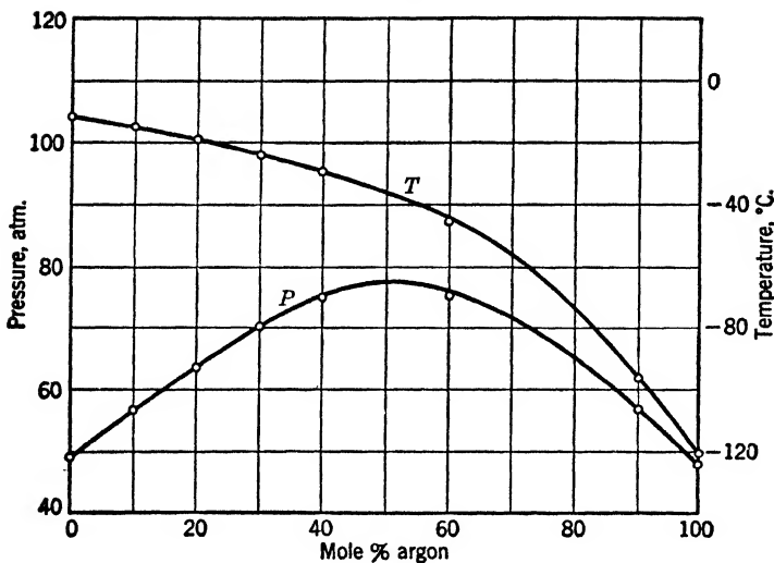
FIG. 2-1. Maximum temperature of liquefaction and corresponding pressures of argon-boron trifluoride mixtures (Courtesy Journal of the American Chemical Society )
