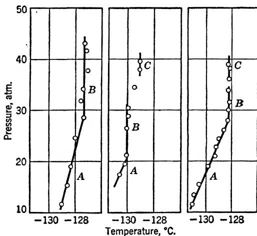
FIG. 4-3. Evidence for existence of compounds of argon and boron trifluoride above the freezing point. Dissociation products of the argon-boron trifluoride compounds lower the freezing point of the solution (Courtesy Journal of the American Chemical Society )
