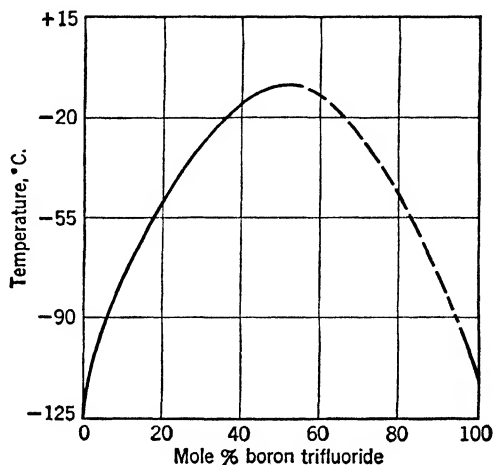
FIG. 4-13. The system dimethyl ether-boron trifluoride
