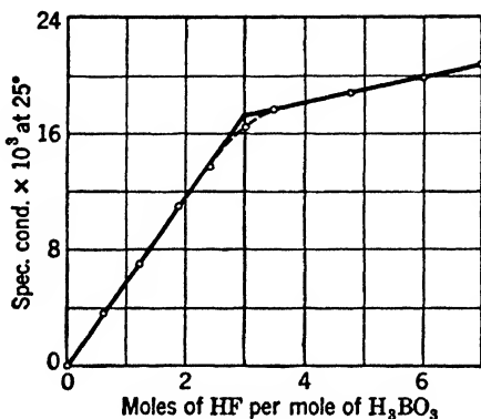
FIG. 5-1. Conductance of \text{H}_3\text{BO}_3 - \text{HF} mixtures immediately after mixing (Courtesy Journal of the American Chemical Society )
