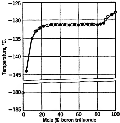
FIG. 4-15. The system tetrafluoromethane-boron trifluoride (Courtesy Journal of the American Chemical Society )
