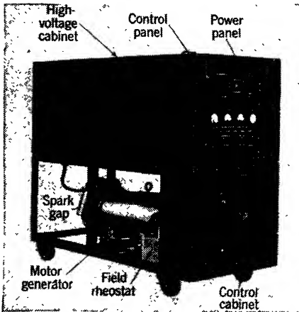
FIG. 11-17.—Photograph of the Model 16 pulser.
