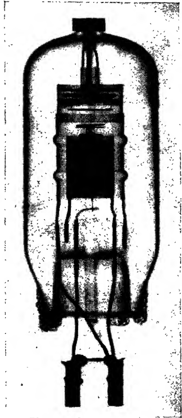
FIG. 8-38.—X-ray photograph of a hydrogen thyatron.
