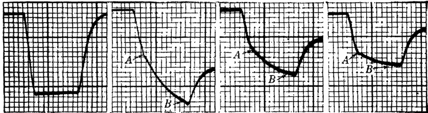
(e) 0.5 μsec voltage pulse. (f) 525 pps. (g) 1000 pps. (h) 2000 pps. Incremental condenser voltage.
