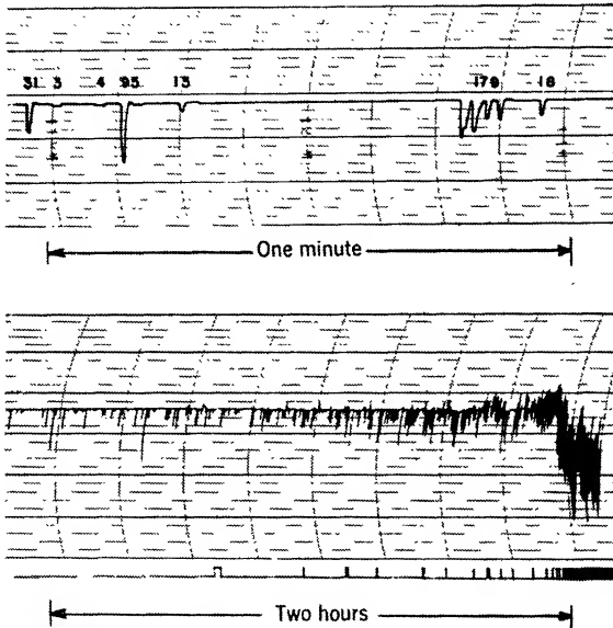
FIG. A-43.—Records of average magnetron current showing sparking as a function of time.
