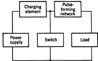
FIG. 9-1.—Block diagram of a line-type pulser.
