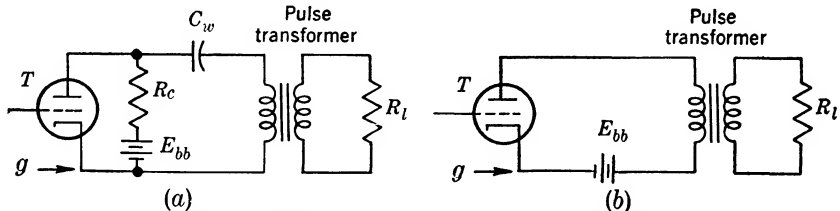
FIG. 2-42.—Two possible arrangements for the use of a pulse transformer with a hard-tube pulser.
