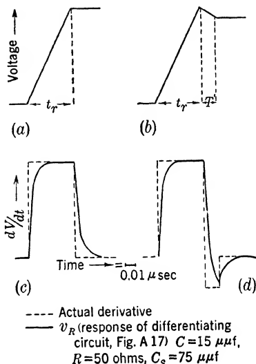
FIG. A-20.—Hypothetical voltage pulses and corresponding time derivatives. (a) Trapezoidal voltage wave front. (b) Trapezoidal voltage wave front with a spike. (c) Time derivative of (a). (d) Time derivative of (b).
