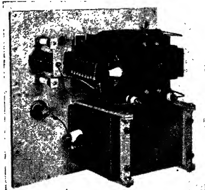
FIG. 11-4.—Compartment for the high-voltage components of high-power pulser.
