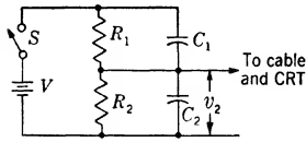
FIG. A-3.—Parallel RC -divider circuit for pulse-voltage measurements with a synchroscope.
