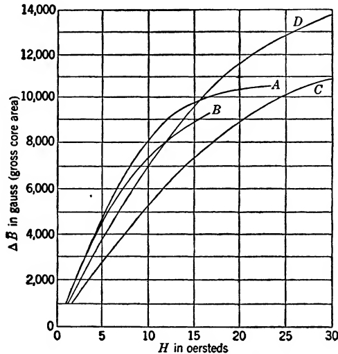
FIG. 15-9.—Loci of the tips of pulse B - H loops taken on butt-joint cores, with 1- \mu sec pulses. Curve A is for Monimax 0.003-in., \frac{1}{2} in. by \frac{1}{2} in. leg section. Curve B is for silicon Nicaloi 0.003 in., \frac{1}{2} in. by \frac{1}{2} in. leg section. Curve C is for silicon Nicaloi 0.004 in., \frac{1}{2} in. by \frac{3}{4} in. leg section. Curve D is for Hipersil 0.002 in., \frac{1}{2} in. by \frac{3}{4} in. leg section.
