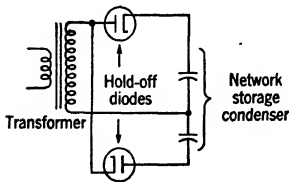
FIG. 9-30.—Two-diode charging circuit.
