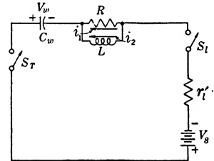
FIG. 5-16.—Simplified output circuit of a hard-tube pulser with a biased-diode load and an LR -network to minimize the change in load current during the pulse.
