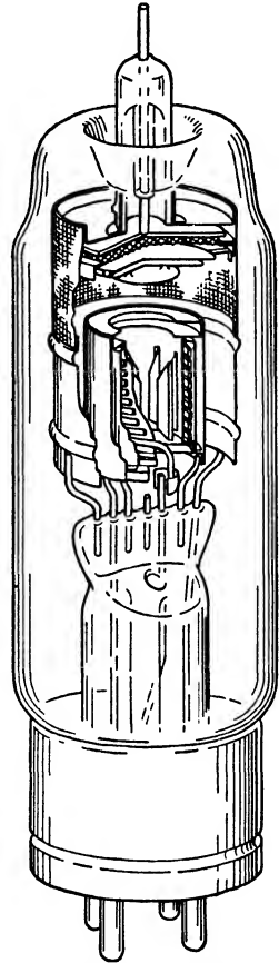
FIG. 8-37.—Cut-away perspective view of the 5C22 hydrogen thyratron.
