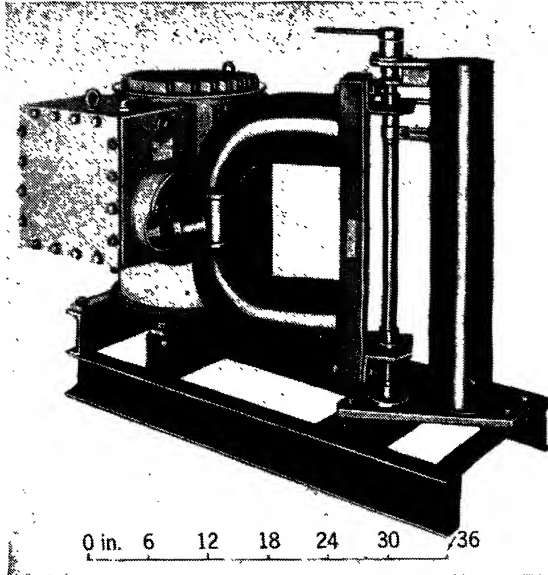
Fig. 15-35.—A high-power magnetron plugged into the gasketed melamac well of a 10-Mw 1- \mu sec pulse transformer.
