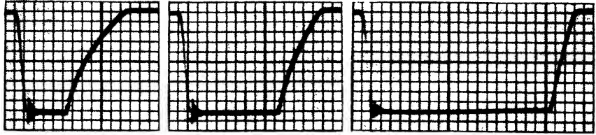
(a) 0.5 \mu\text{sec} (b) 1 \mu\text{sec} . (c) 2 \mu\text{sec} . Magnetron voltage pulses of amplitude = 10 kv.
