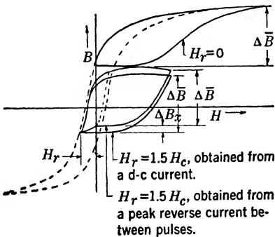
FIG. 15-31.—Pulse B - H loops superimposed on a d-c loop to show the difference between obtaining H_r from a peak reverse current between pulses and from a d-c current.
