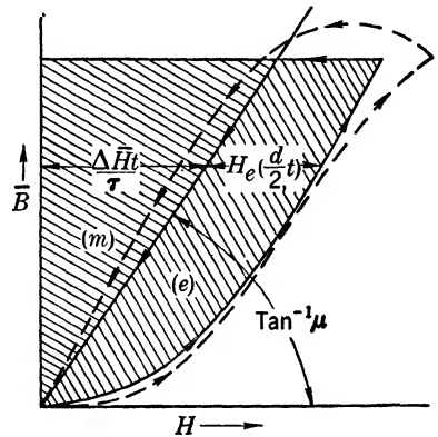
FIG. 15-18.—Idealized and actual pulse B - H loops.
