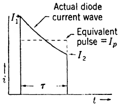
FIG. A-31.—Approximate shape of the current pulse in the diode of Fig. A-28.
