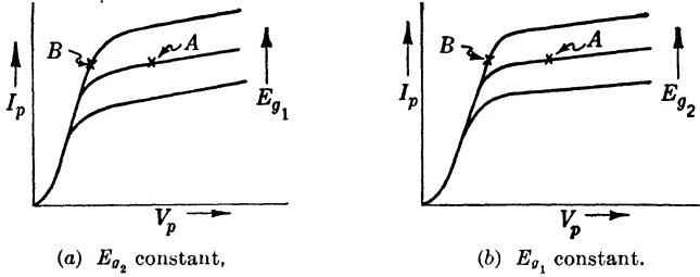
FIG. 3-15.—Idealized current-voltage characteristics of a tetrode.
