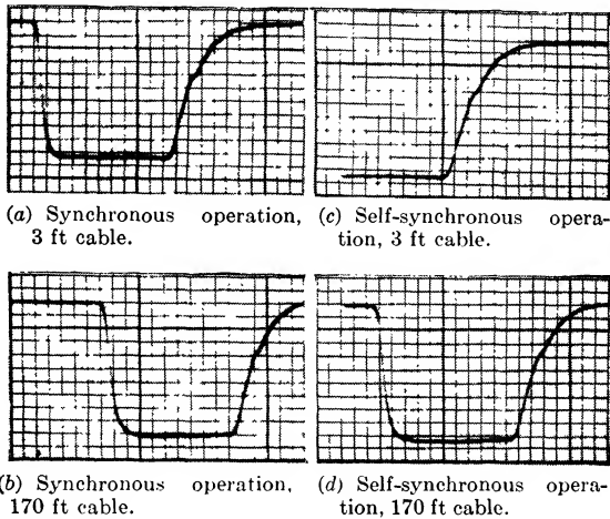
FIG. A-24.—Photographs of voltage pulses showing the delay in the start of the sweep in self-synchronous operation, and the effect of a long 100-ohm cable on the observed pulse shape.
