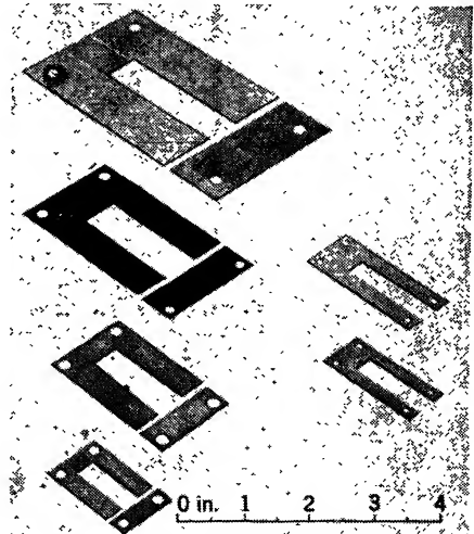
FIG. 15-8.—Various nickel steel punchings. Light-colored punchings are of 0.004-in. silicon Nicaloi, the dark punching of 0.003-in. Monimax.
