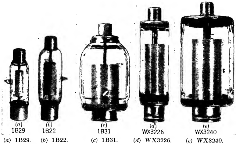
FIG. 8-26.—Photographs of various aluminum-cathode gaps. (Parts (a) and (b) courtesy of the Bell Telephone Laboratories.)
