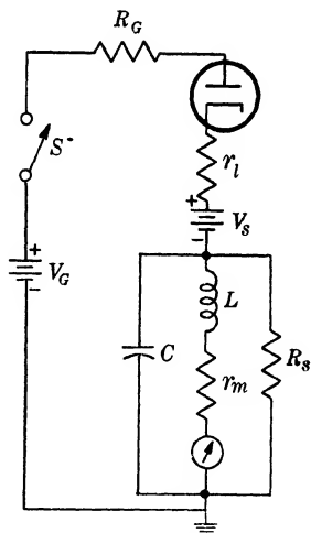
FIG. A-40.—Schematic diagram of pulse-discharging circuit including the equivalent circuit for a magnetron and an average-current meter.
