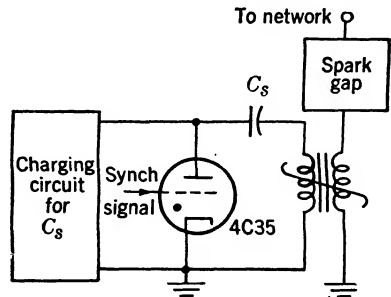
FIG. 8-20.—Trigger circuit using a saturable-core transformer.
