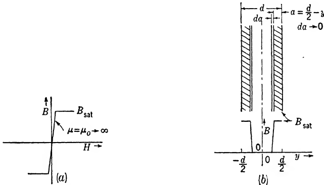
FIG. 15.23.—(a) Idealized B - H loop for a material of \mu = \mu_0 = \infty and H_c = 0 . (b) Instantaneous distribution of flux density within the lamination for nonlinear magnetization where \mu = \mu_0 = \infty and H_c = 0 .
