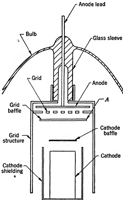
FIG. 8-36.—Structure of a hydrogen thyratron.
