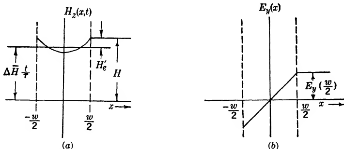
FIG. 15-25.—Steady-state distribution throughout the core of (a) H_z(x,t) , where H_e' = \frac{10^{-9}\mu\pi\omega^2\Delta\bar{H}}{3r\left(\frac{r_s}{d}\right)} oersteds, and (b) E_y(x) , where E_y\left(\frac{w}{2}\right) = \frac{10^{-9}\mu\Delta\bar{H}w}{2r} volts.
