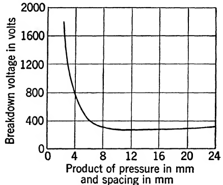
FIG. 8-35.—Plot of breakdown voltage in hydrogen as a function of the product of spacing and pressure.
