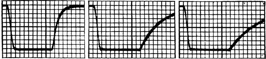
(d) R_l = 1000 ohms. (e) R_l = 5000 ohms. (f) R_l = 10,000 ohms. Capacitance in parallel with the load = 140 \mu\text{f} .
