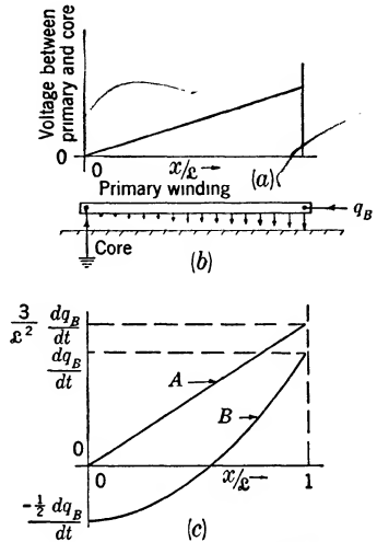
FIG. 12-21.—(a) Voltage distribution between primary and core for a pulse transformer.
