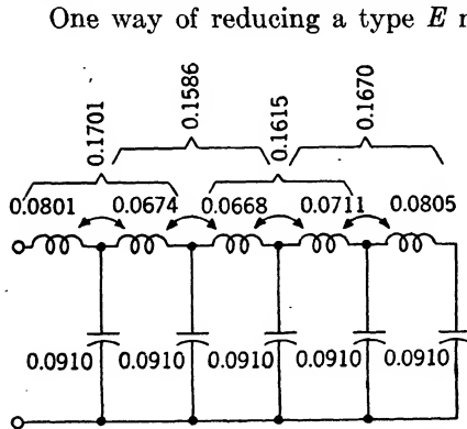
FIG. 6-28.—Equal-capacitance mutual-inductance network equivalent to the equal-capacitance network in Fig. 6-22. The inductances are in henrys and the capacitances in farads if the pulse duration is expressed in seconds and network impedance in ohms.
