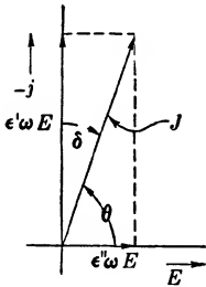
FIG. 15-34.— Vectors showing the relationship of the displacement current to the loss current.
