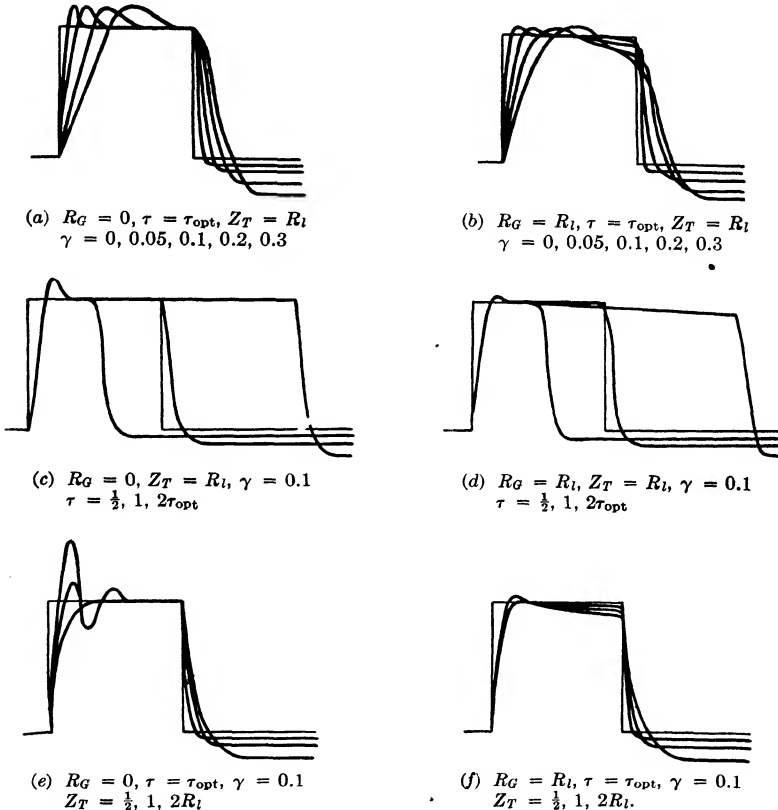
FIG. 14-13.—Pulse shapes on a resistance load calculated for various values of the parameters. (\alpha + \beta)_{opt} = \gamma; \frac{Z_T}{R_l} = \frac{1}{R_l} \sqrt{\frac{L_L}{C_D}}; \frac{\tau}{\sqrt{2LLC_D}} = \frac{\tau}{\tau_{opt}}; \frac{R_G}{R_l}
