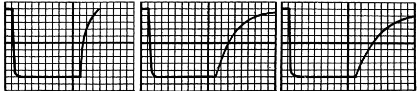
(j) R_l = 1000 ohms. (k) R_l = 5000 ohms. (l) R_l = 10,000 ohms. Pulse shapes calculated from equivalent circuit (m) for shunt capacitance = 80 \mu\text{f} .
