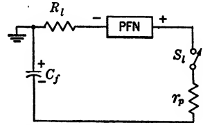
FIG. 11.19.—Equivalent circuit at the start of the pulse.
