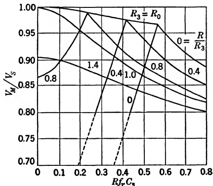
FIG. 8-22.—Ratio V_M/V_S as a function of RfC_3 for the series-gap circuit of Fig. 8-9a.
