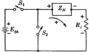
FIG. 11-41.—Equivalent circuit for a double-switch single-network pulser.
