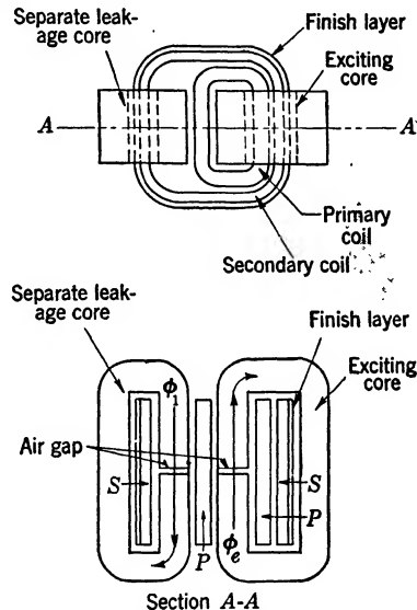
FIG. 9-20.—Sketch of an a-c resonant-charging transformer with separate leakage core; \phi_e is the exciting flux and \phi_1 is the reactance flux. (Courtesy of General Electric Co.)
