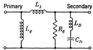
FIG. 7·12.—Equivalent circuit for a pulse transformer.
