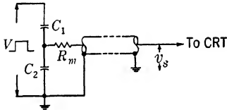
FIG. A-11.—Capacitance divider approximately matched to a cable by a series resistor R_m = Z_0 ; v_s = \frac{C_1}{C_1 + C_2 + C_c + C_s}
