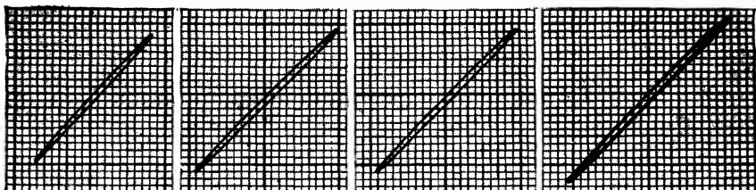
(e) I_{c_{rms}} = 0.215 amp, L_L = 2.94 henrys. (f) I_{c_{rms}} = 0.435 amp, L_L = 2.98 henrys. (g) I_{c_{rms}} = 0.870 amp, L_L = 2.92 henrys. (h) I_{c_{rms}} = 1.000 amp, L_L = 2.89 henrys. Primary short-circuited, no d-c in secondary
