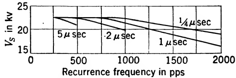
FIG. 8-10.— V_s as a function of recurrence frequency.
