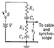
FIG. A-12.—Series RC -divider circuit for pulse-voltage measurements with a synchroscope.
