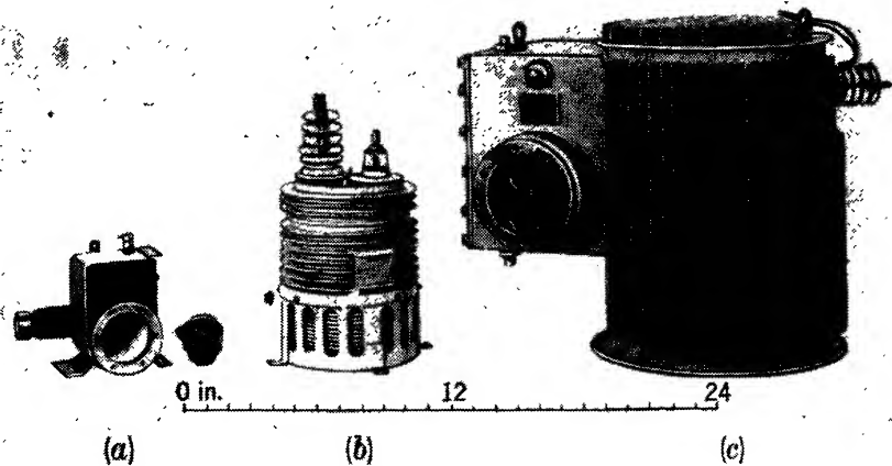
FIG. 13-11.—Three pulse transformers designed for operation at different power levels. (a) 120 kw (232 BW2) with well for magnetron (Westinghouse). (b) 2 Mw (GE) (c) 10 Mw (377 BW2) with form-fitting well for magnetron (GE).
