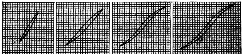
(m) V_{sec} = 1730 volts, L_L = 54.0 henrys. (n) V_{sec} = 3460 volts, L_L = 52.0 henrys. (o) V_{sec} = 7500 volts, L_L = 48.4 henrys. (p) V_{sec} = 8600 volts, L_L = 46.6 henrys. Primary open-circuited, no d-c in secondary.
