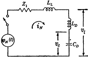
FIG. 7-18.—Simplified equivalent circuit of a line-type pulser for the analysis of the leading edge of the pulse.
