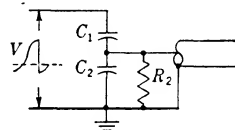
FIG. A-27.—Unbalanced RC -divider for measurements of post-pulse voltages of either polarity across the pulser switch.
