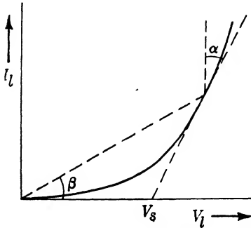
FIG. 3-16.—Current-voltage characteristic of a nonlinear load.
