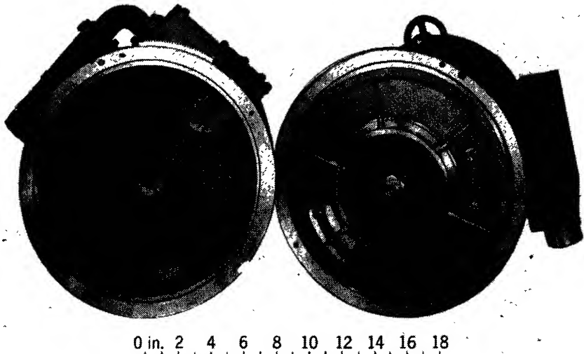
FIG. 8-7.—Photograph of a radial-pin rotary gap.
