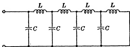
FIG. 6-32.—Current-fed pulse-forming network of the uniform-line type.
