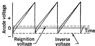
FIG. 8-48.—Anode-voltage waveform showing the removal of inverse voltage by means of a shunt diode.
