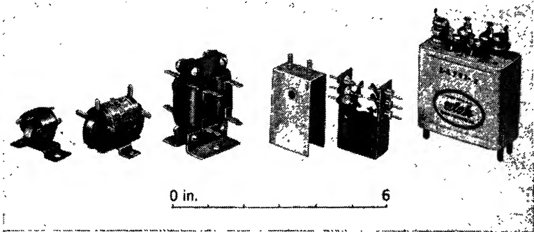
FIG. 13-9.—Some examples of low-power regenerative-pulse-generator pulse transformers.
