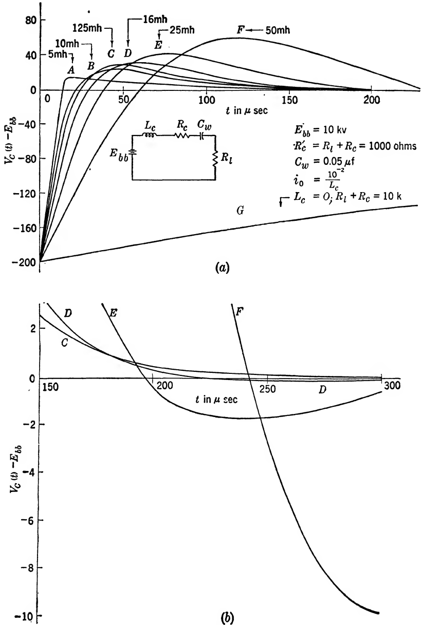
FIG. 2-39.—Storage-condenser voltage as a function of time during the recharging interval for an inductive element in series with the power supply; large values of R'_c/L_c . The portion of the curves C, D, E, and F beyond t = 150 \mu sec are plotted on expanded scales in (b) in order to show the transition from the aperiodic to the oscillatory conditions.
