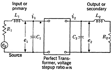
FIG. 12-2.—A source-load system employing a perfect transformer.
