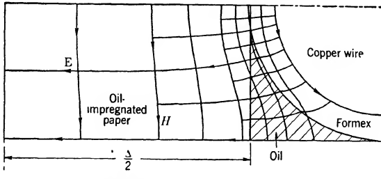
FIG. 15-39.—Flux plot showing lines of E and H for a typical pulse-transformer winding. No. 25 quadruple formex wire, dia = 0.0219 in., bare Cu dia = 0.0179 in. Spacing between windings \Delta = 0.040 in.
