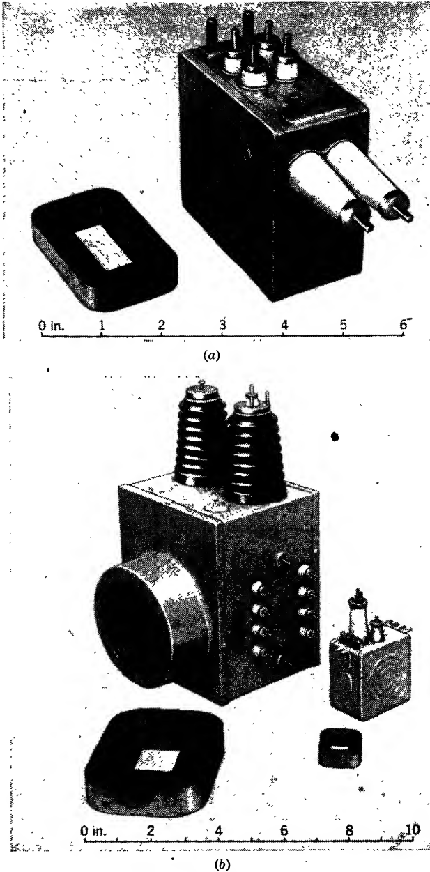
FIG. 13-12.—Three pulse transformers constructed with continuously wound permalloy cores (Western Electric Company). (a) Rectangular core of 1-mil 4-79 molybdenum permalloy and pulse transformer in which it is used. Pulse power: 100 kw. (b) 3-lb. rectangular core of 2-mil 45 permalloy and \frac{1}{4} -lb. core of 1-mil 4-79 molybdenum permalloy with the pulse transformers in which they are used.
