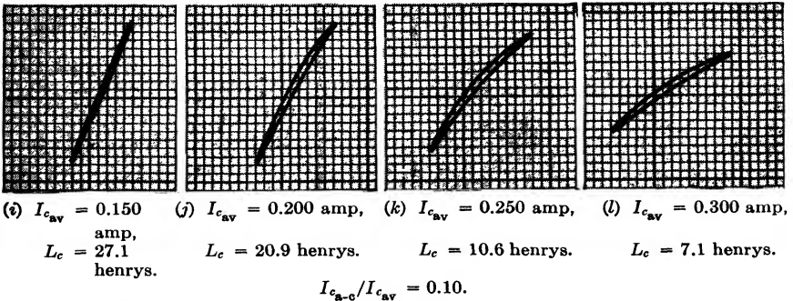
FIG. 9-9.— B-H oscillograms for a typical d-c charging reactor rated at I_{c_{av}} = 0.19 amp, B is vertical and H is horizontal.
