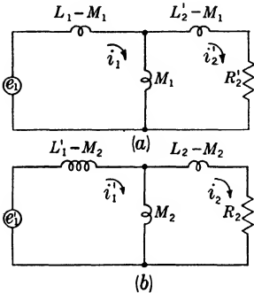
FIG. 12-4.—Circuits equivalent to those shown in Fig. 12.3.
