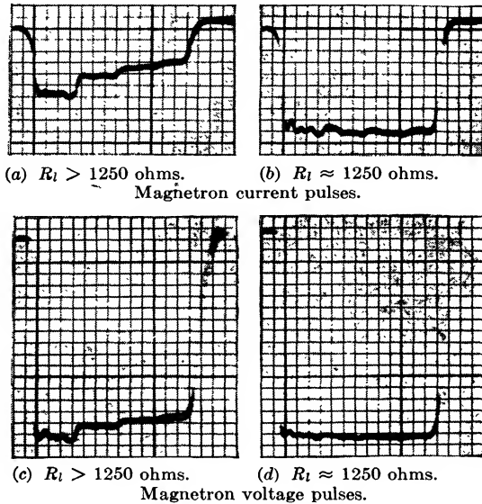
FIG. 2-47.—Oscilloscope traces for 2- \mu\text{sec} pulses of magnetron current and voltage for a hard-tube pulser using the 232AW and 232BW pulse transformers with 100 ft of 50-ohm pulse cable. The transit time for transformers and cable is 0.25\mu\text{sec} .
