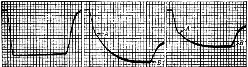
(i) 1 μsec voltage pulse. (j) 525 pps. (k) 1000 pps. Incremental condenser voltage.
