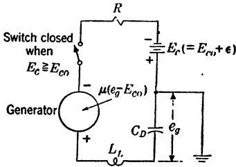
FIG. 14-16.—Simplified equivalent circuit for a regenerative pulse generator in which the effects of C, C_{op}, r_p, L_p (and L_L ) are neglected.
