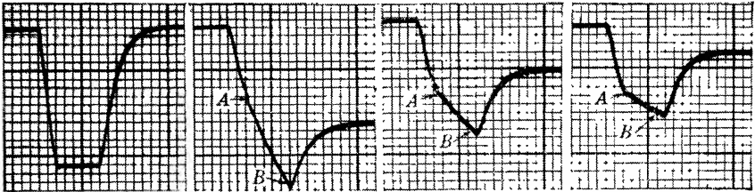
(a) 0.25 μsec voltage pulse. (b) 525 pps. (c) 1000 pps. (d) 2000 pps. Incremental condenser voltage.
