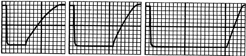
(j) 0.5 \mu\text{sec} . (k) 1 \mu\text{sec} . (l) 2 \mu\text{sec} . Voltage pulses calculated from the equivalent circuit (m).
