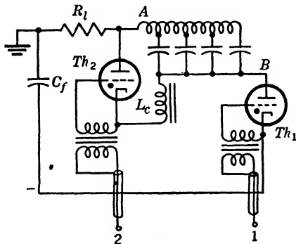
FIG. 11-18.—The Anger circuit with a hold-off thyatron.
