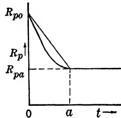
FIG. 7-27.—Assumed switch-resistance characteristics.
