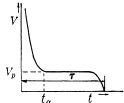
FIG. 7-10.—Typical switch drop as function of time.
