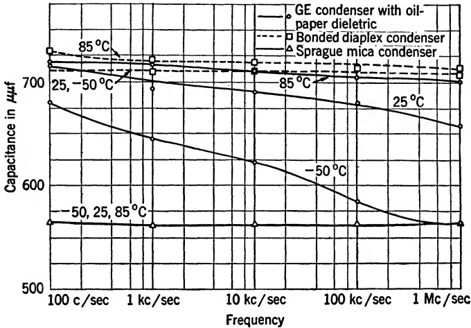
FIG. 6-42.—Variation of capacitance with frequency and temperature.
