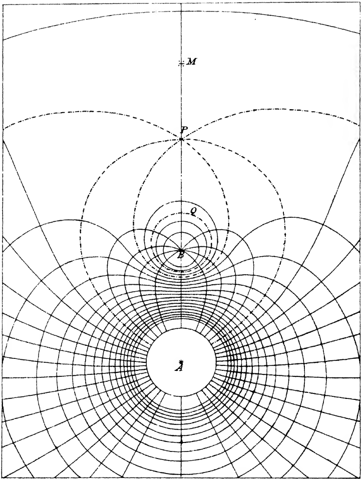
Lines of Force and Equipotential Surfaces.
