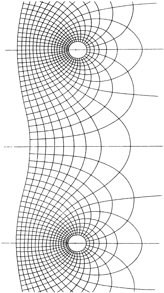
Lines of Force near a Grating.
