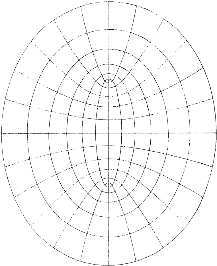
Confocal Ellipses and Hyperbolas
