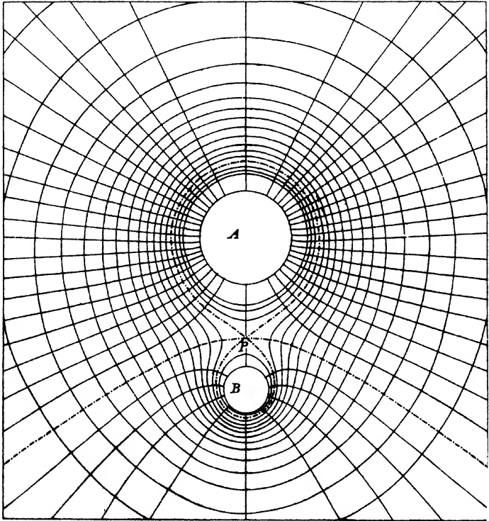
Lines of Force and Equipotential Surfaces.
