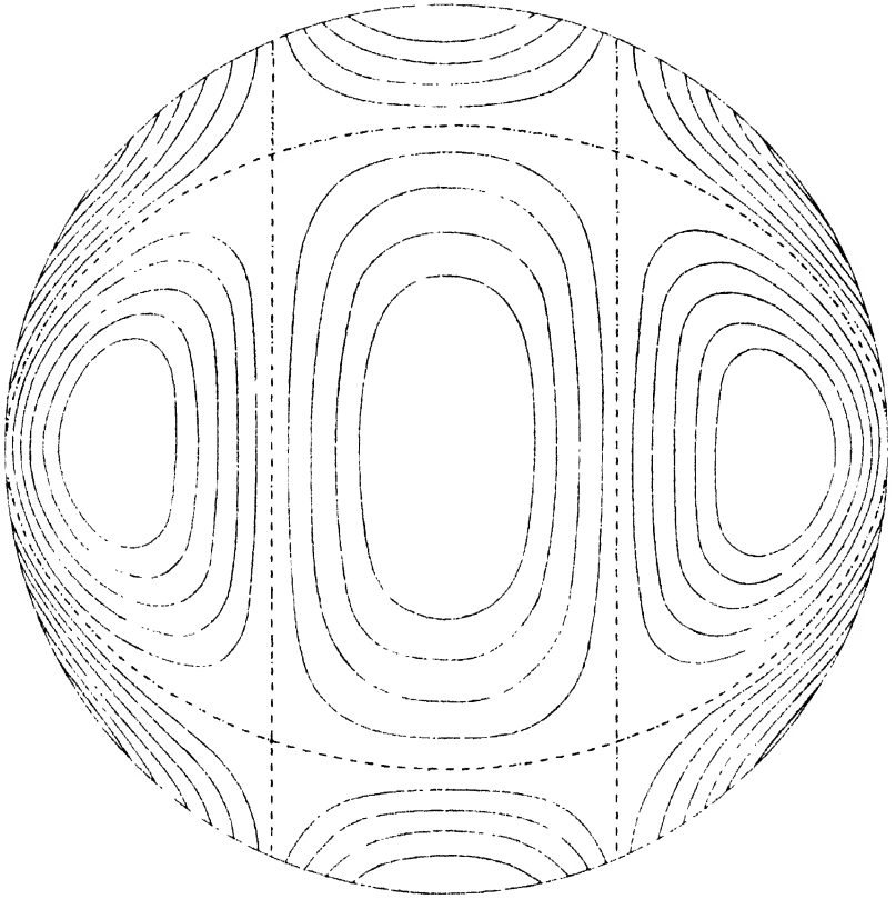
Spherical Harmonic of the fourth order
