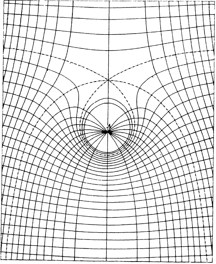
Lines of Force and Equipotential surfaces
