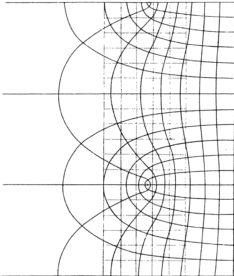
Lines of Force near the edge of a Plate.
