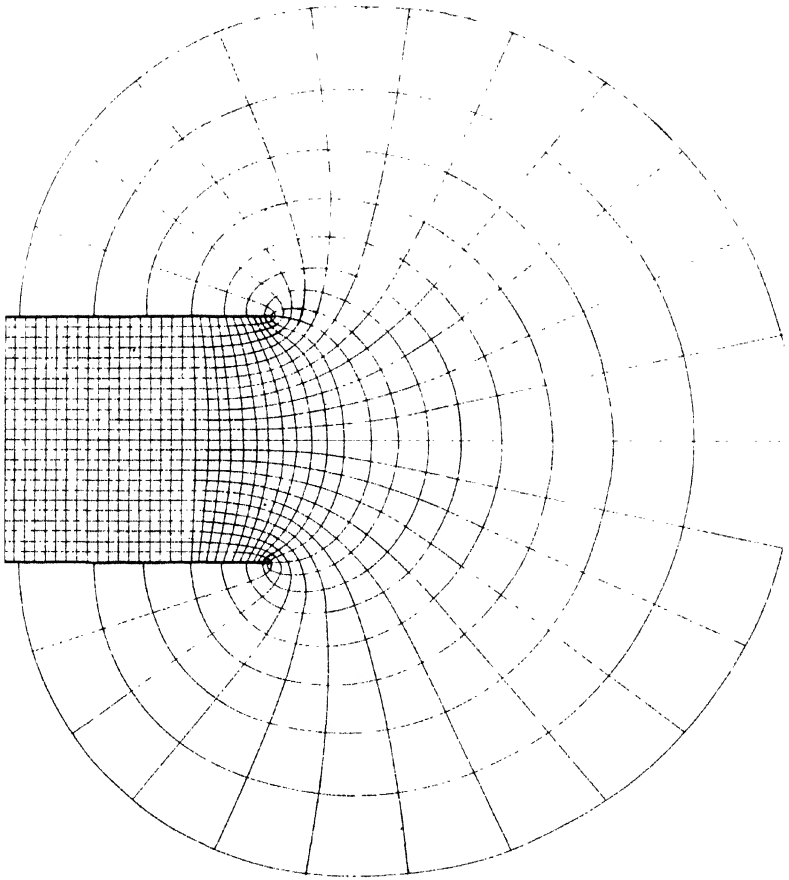
Lines of Force between two Plates
