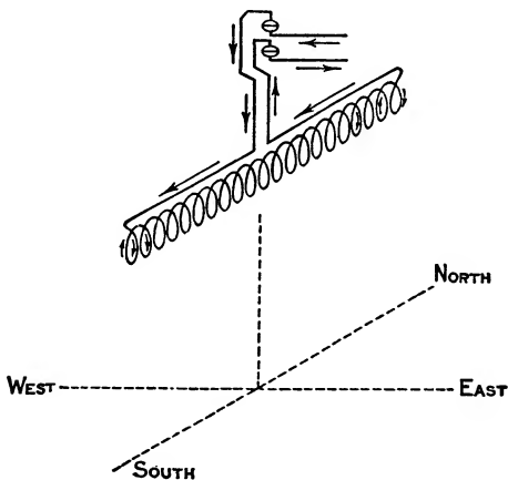
Fig. 67.—Orientation of Solenoid
