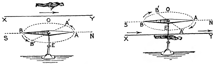
Fig. 63.—Ampère's Rule
