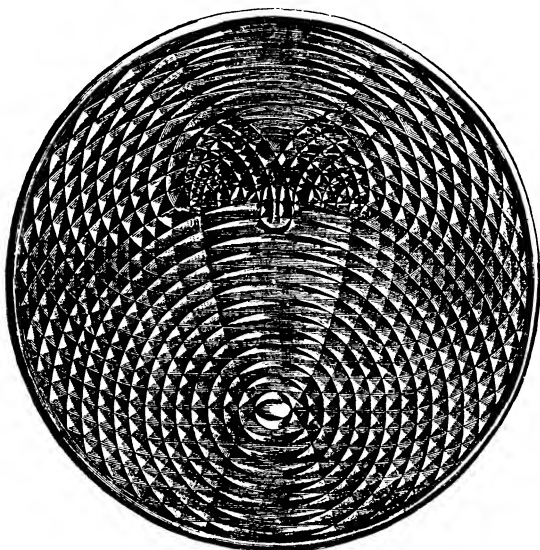
Fig. 82.—Interference Waves
