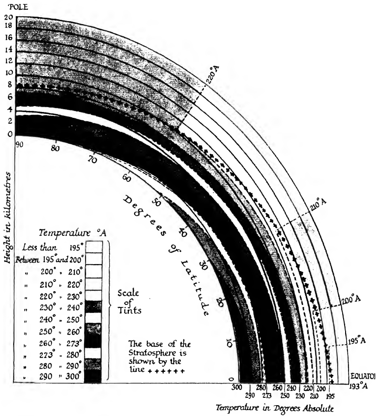
Diagrammatic Representation of the vertical distribution of air temperature
