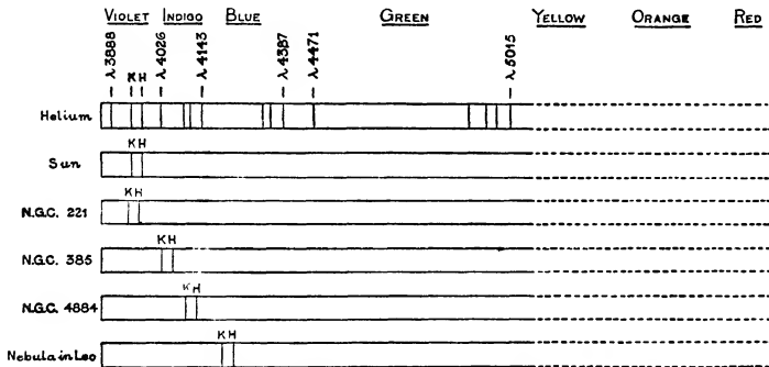
Fig. 136.—Dotted sections not to scale. Red extends to \lambda 7600
