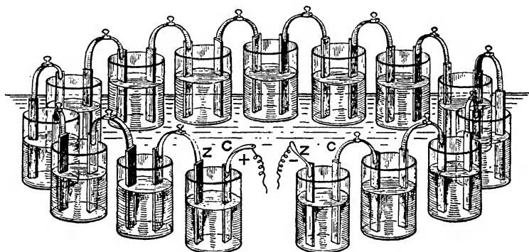
Fig. 60.—Volta's "Crown of Cups"
