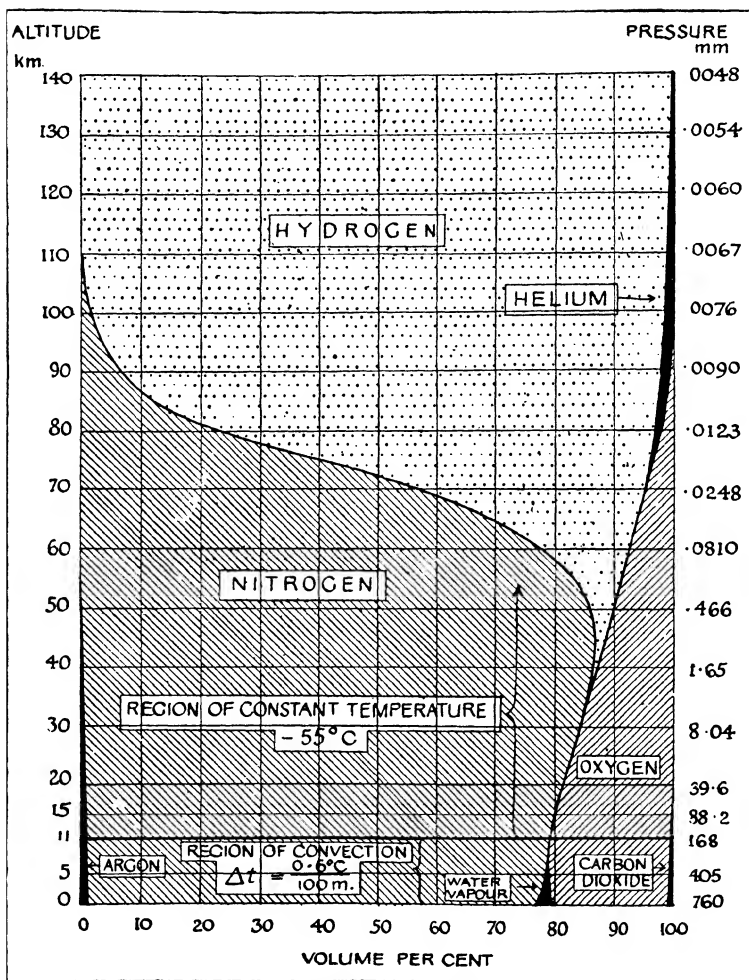
Fig. 151.—Distribution of the gases in the atmosphere (after Humphreys in the Mount Weather Bulletin , Vol. II)
