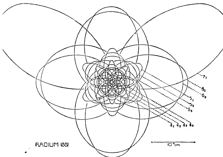
Fig. 110.—Diagram of the Radium Atom
