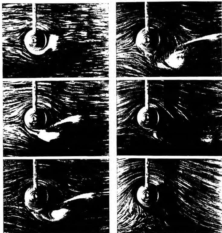
Successive Stages of the Flow round a Rotating Cylinder
