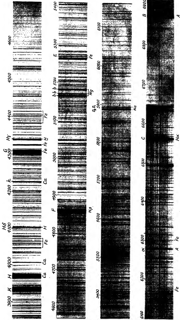
Spectrum of the Sun, \lambda\lambda 3900-6900, with 13-ft. Spectrograph Mount Wilson Observatory
