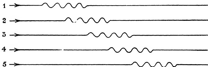
Fig. 123.—Travelling wave-packet. Positions at successive minute intervals of time.
