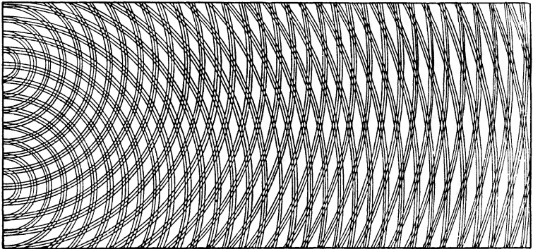
Fig. 81.—Interference or superposition drawn for two sets of ripples originating at A and B
