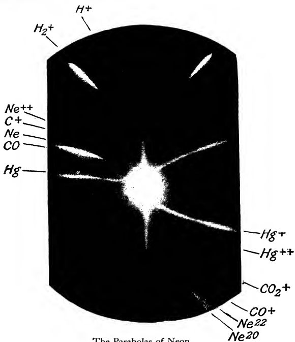
The Parabolas of Neon
