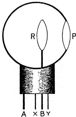
Fig. 131.—Photo-electric cell
