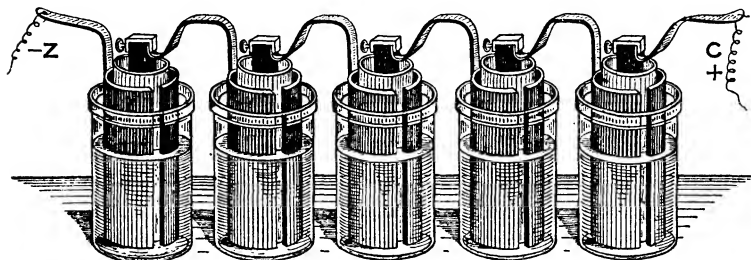
Fig. 61.—Bunsen's Battery
