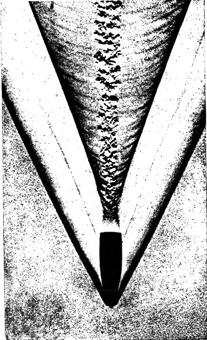
Photograph of an 8-mm. Bullet moving with Velocity of about 880 M./S. C. Cranz ( Berlin , 1917)
