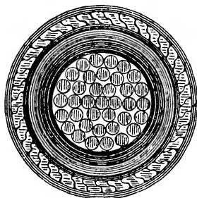
Fig. 129.—Lock-coil steel armoured cable
