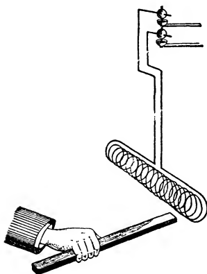
Fig. 68.—Action of Magnet on Solenoid
