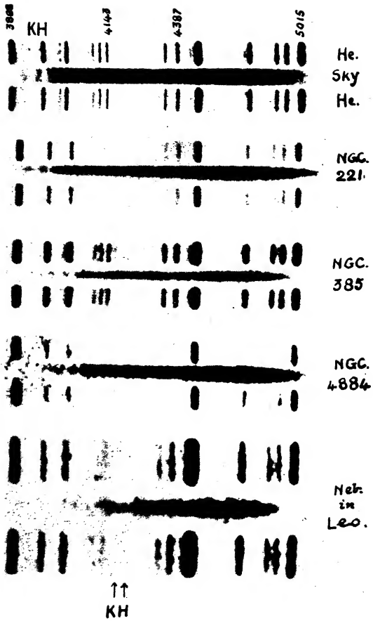
Nebular Spectra, showing Red Shift Increasing with Distance Mount Wilson Observatory
