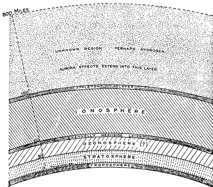
Fig. 155.—Diagram showing succession of atmospheric layers. Heights are rough approximations
