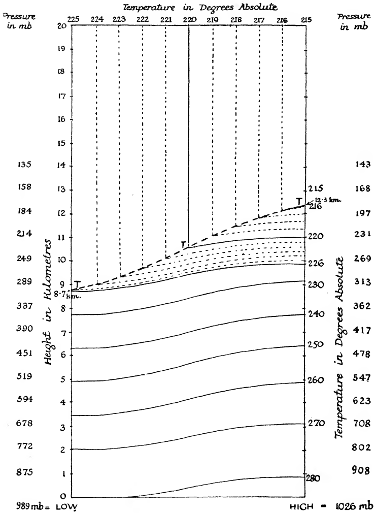
Fig. 149.—Tropopause and Stratopause
