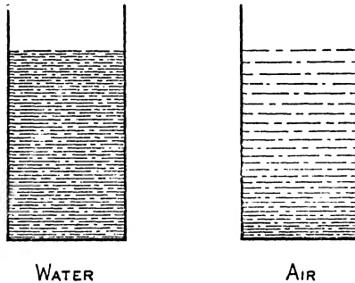
Fig. 146.—Diagrammatic representation of layers of water and air
