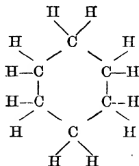
Hexa-hydro-benzene ( C_6H_{12} )
