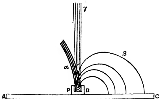
Fig. 99.—Curie Rays
