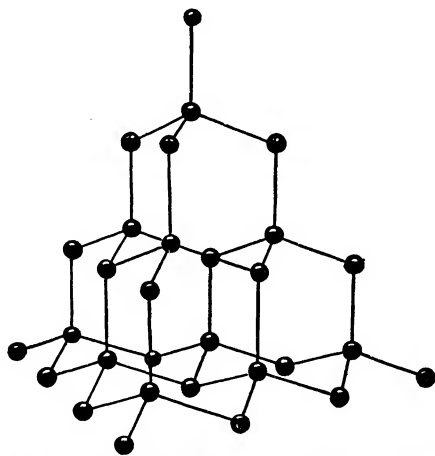
Fig. 118.—Diamond model
