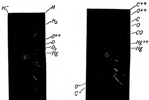
Photographs of Typical Positive Ray Parabolas
