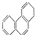
Phenanthrene.
