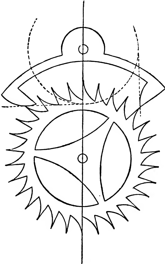
FIG. 10.—ANCHOR ESCAPEMENT.
