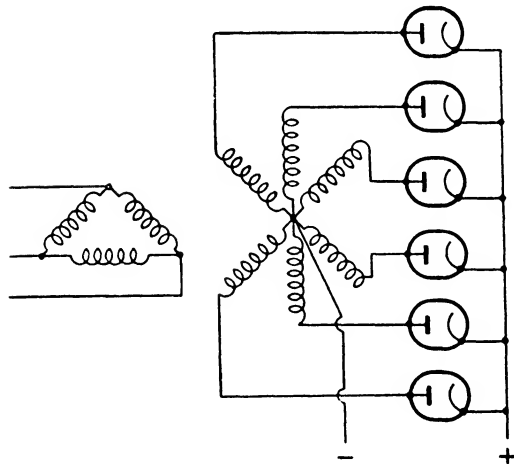
FIG. 68. SIX-PHASE HALF-WAVE RECTIFIER
