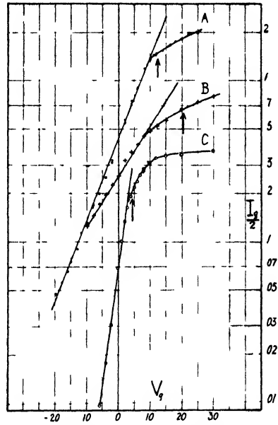
Fig. 9—Collector characteristics showing extension of linear portion into region of positive potentials. Curve A, space-charge limited, V_p=300 . Curve B, not space-charge limited, V_p=300 . Curve C, space-charge limited, V_p=150 , I_s divided by 2.45 before plotting. Tube II.
