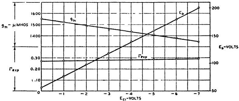
Fig. 12—Reduction of shot effect in cathode current of RCA-57 operated as a triode, for I = 2.5 ma, T = 990^\circ K, and various control-grid biases.
