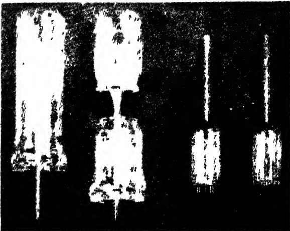
Fig. 4—(Left Half)—Conventional type tube before and after sealing, with discarded collet. (Right Half)—Miniature-type tube before and after sealing, with no collet.
