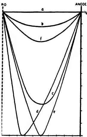
Fig. 12—Potential distribution for several values of space current. \frac{V_a}{V_g} = 1.
