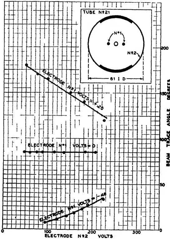
Fig. 6—Beam width and anode potential
