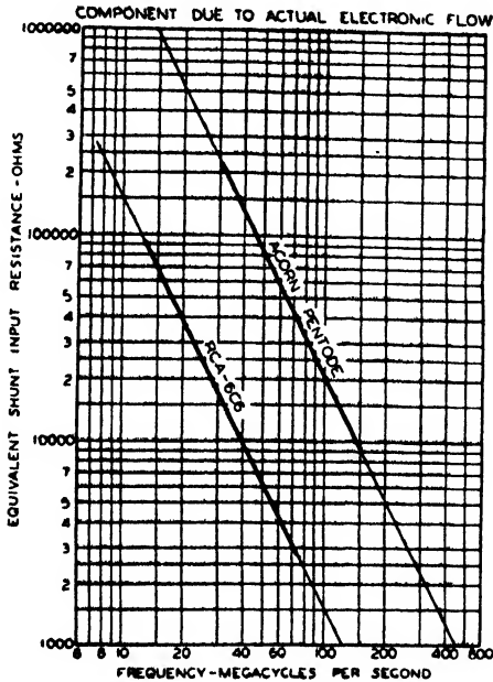
Fig. 9—The equivalent shunt input resistances of the “acorn” pentode and the RCA-6C6 as a function of the frequency. This is the component of resistance which is due to the actual electronic flow past the control grid.
