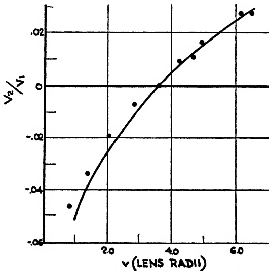
Fig. 8—Focusing relation (variable focus).
