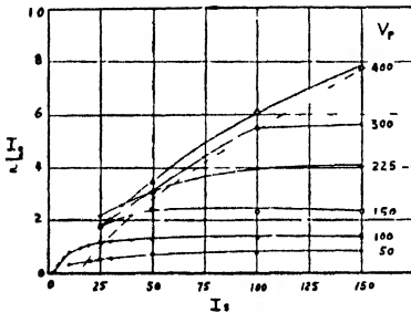
Fig. 3—Variation of probe current (milliamperes) with temperature-limited emission (milliamperes) and plate potential (volts). I_p/2 is the current actually indicated by meter A , Fig. 2, because of the use of a commutator it must be multiplied by two to get the total probe current. Tube I.
