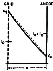
Fig. 1—Potential distribution between grid and anode typical of the case when neither potential minimum nor virtual cathode exist. All of the electrons which pass through the grid are collected at the anode.
