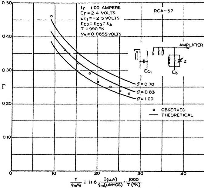
Fig. 10—Reduction of shot effect in cathode current of RCA-57 operated as a triode. The cathode current ranges from 1/2 to 4 milliamperes.
