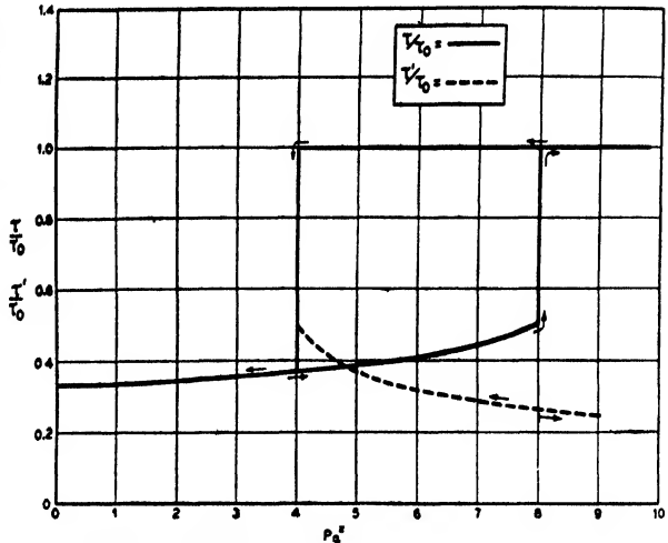
Fig. 13—Variation of electron transit time with space current. \frac{V_a}{V_g} = 1.
