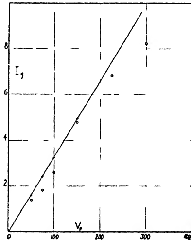
Fig. 11—Probe currents for V_g = 0 . Experimental (O) from data of Fig. 10; computed (+) from (9).
