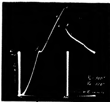
Fig. 19 — Transfer-characteristic oscillogram of special pentode showing the hysteresis and instabilities characteristic of the curve marked \frac{V_a}{V_c} = 0.4 of Figure 11.
