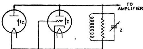
Fig. 9—Schematic shot-effect test circuit using comparator diode.
