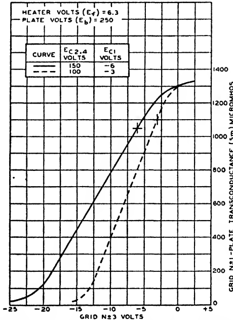
Fig. 3—First grid-to-plate transconductance characteristics for the 6L7. E_{e1} held constant.
