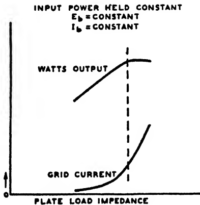
Fig. 6—Power amplifier performance with constant power input.
