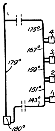
Fig. 24.— SINGLE-PIPE DROPPING SYSTEM
