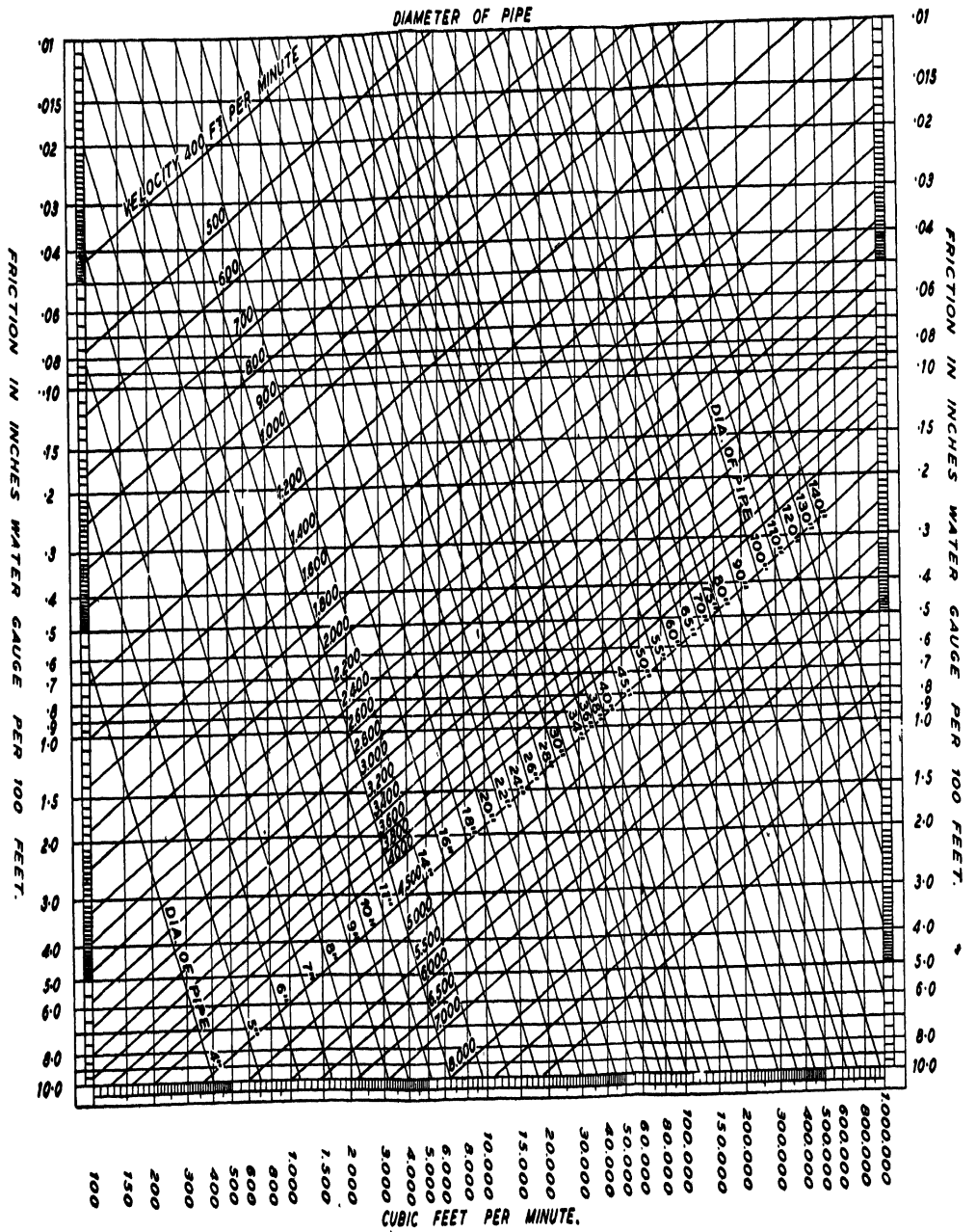
Fig. 15.—CAPACITIES AND RESISTANCES OF GALVANIZED IRON DUCTWORK
