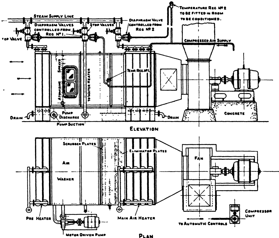
Fig. 19.—GENERAL ARRANGEMENT OF AIR CONDITIONING PLANT
