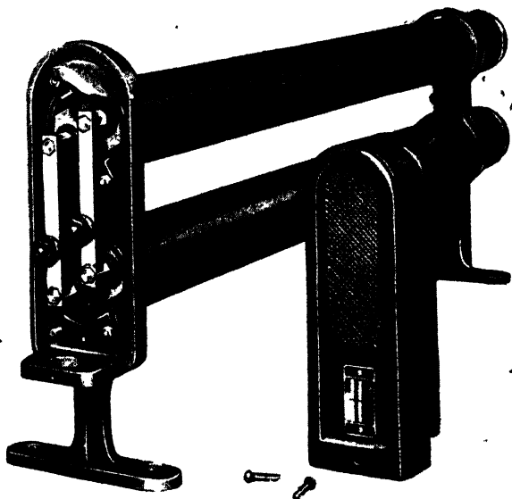
Fig. 2.—TWO-TIER TUBULAR HEATER Showing the terminal box. Note the hole at the base of the box to allow entry of the electric cables. ( General Electric Co. )
