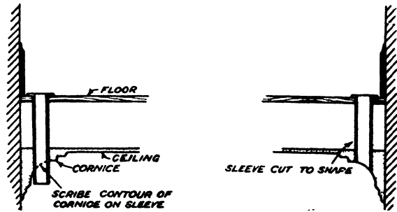
Fig. 12.—WHEN A SLEEVE PASSES THROUGH A CORNICE The shape of the cornice should be scribed on it; the sleeve can then be cut to fit the curve as shown on the right.
