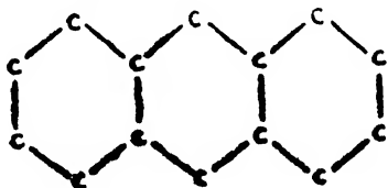
Anthracene skeleton
