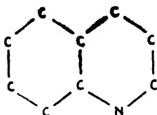
“ Quinoline ” skeleton
