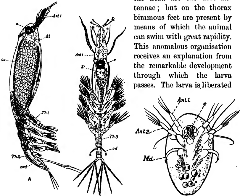
FIG. 30.— Haemocera danae , \times 40 . A , Side view ♀; B , ventral view ♂. Ant. 1 , 1st antenna; e , eye; or , ovary; ovd , oviduct; St , stomach; Th. 1 , 1st thoracic appendage; Th. 5 , 5th thoracic segment; vd , vas deferens. (After Malaquin.)
