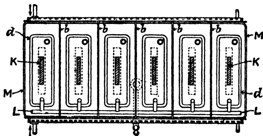
FIG. 2.—The Griesheim Cell.
