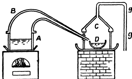
FIG. 1.—Small Still for Hydrofluoric Acid.
