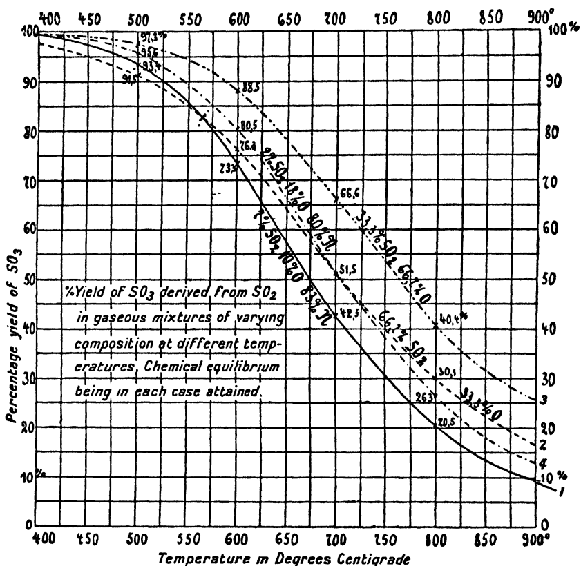
FIG. 30.—Conversion of Sulphur Dioxide into Sulphur Trioxide (Bodenstein and Pohl).
