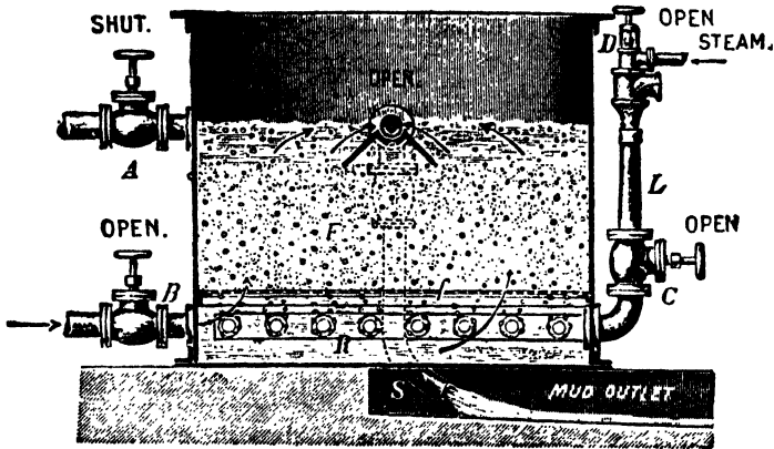
FIG. 4.—Royle's Gravity Filter, cleansing operation.
