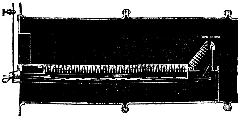
FIG. 4.—Gal'oway-Hill Smoke-Preventing Furnace (Longitudinal Section). (Galloways Ltd., Manchester.)
