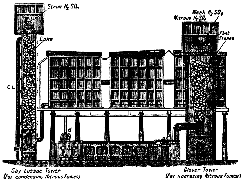
FIG. 13.—Three-Chamber Sulphuric Acid Plant (Diagrammatic).
