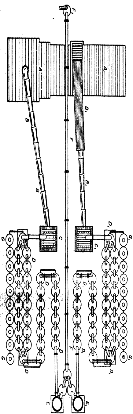
FIG. 1.—Plant for Manufacture of Hydrochloric Acid.
