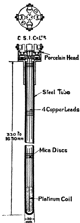
FIG. 6.—Thermo-Element of Electric Resistance Pyrometer.
