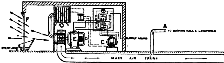
FIG. 14.—Ozonising Installation for Air Treatment of the Central London Railway.
