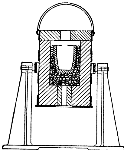
FIG. 7.—Crucible Furnace.
