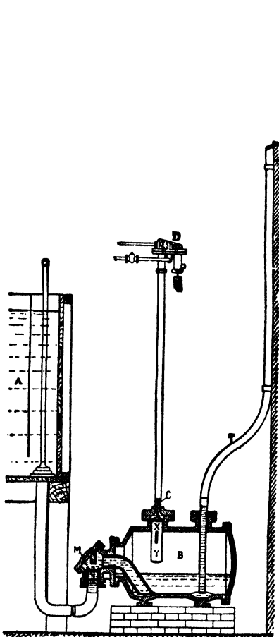
FIG. 22.—Kestner's Acid Elevator.
