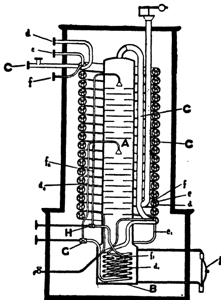
FIG. 16.—Linde Nitrogen Separator. (From Thorpe's "Dictionary of Applied Chemistry." By the courtesy of Messrs Longmans & Co.)
