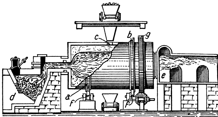
FIG. 2.—Revolving Black Ash Furnace.
