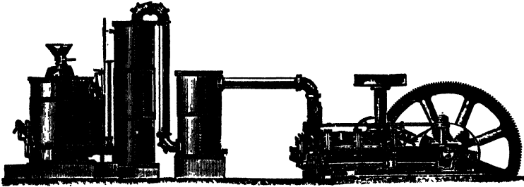
FIG. 11.—Mond Suction Plant and Engine.
