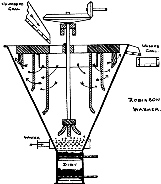
FIG. 3.—Robinson's Coal Washer.
