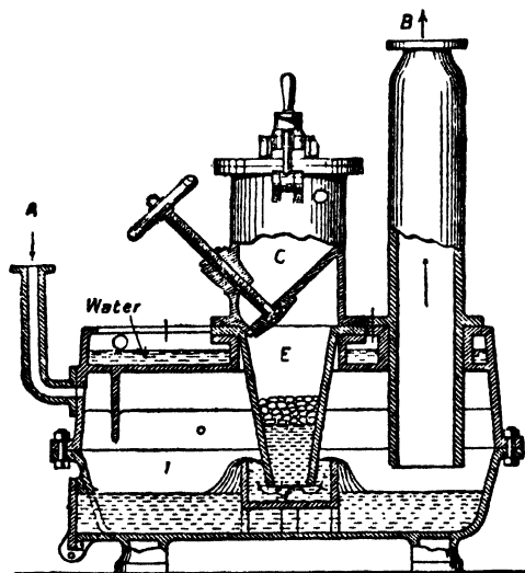
FIG. 2.—Sachsenberg Sulphur Burner.
