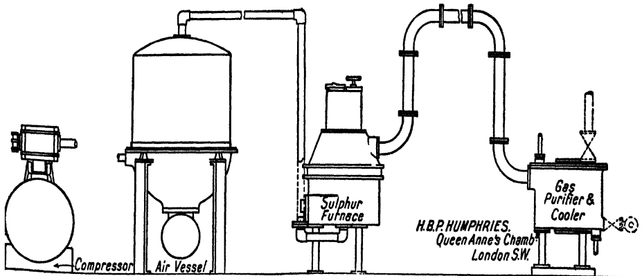
FIG. 4.—Humphries' Plant for making Sulphur Dioxide.
