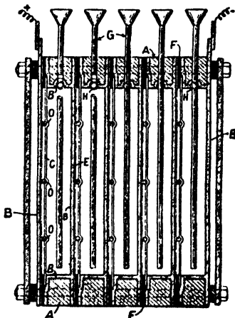
FIG. 1.—Gibb's Electrolytic Cell for Chlorate.
