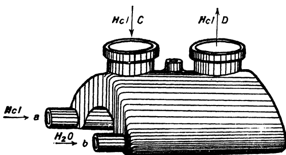
FIG. 3.—Cellarius Receivers.
