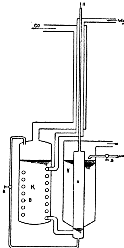
FIG. 24.—Linde-Frank-Caro Process for producing Hydrogen from Water-Gas.
