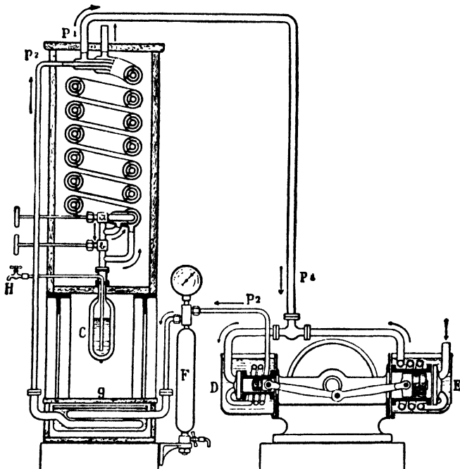
FIG. 8.—Linde's Apparatus for Liquefying Air. Laboratory Type.
