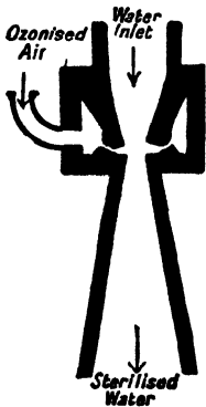
FIG. 11.—Otto's Apparatus for Ozone Treatment of Water.
