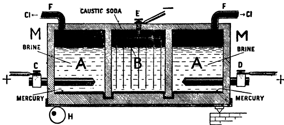
FIG. 8.—The Castner-Kellner Cell.
