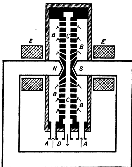
FIG. 5.—Section through the Birkeland-Eyde Furnace.
