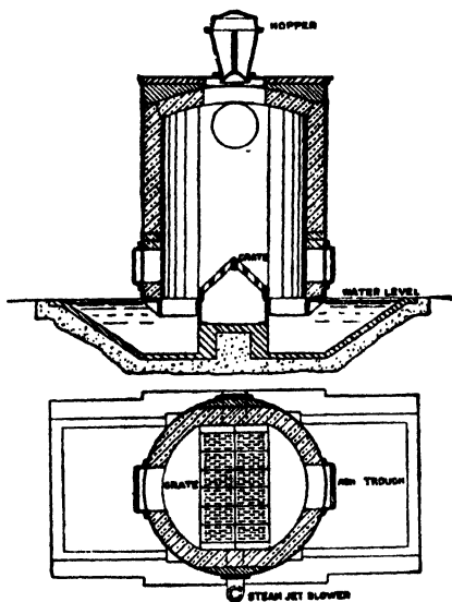
FIG. 5.—The Duff Producer (two views).
