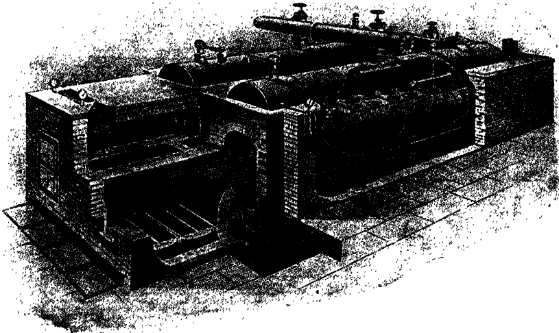
FIG. 2.—Galloway Boiler with External Furnace. (Galloways Ltd., Manchester.)
