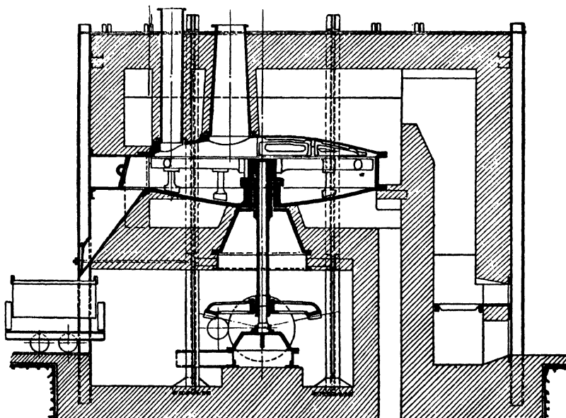
FIG. 4.—Mechanical Salt Cake Furnace.
