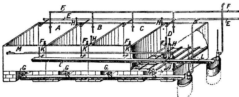
FIG. 3.—Shank's Black Ash Lixiviating Tank.
