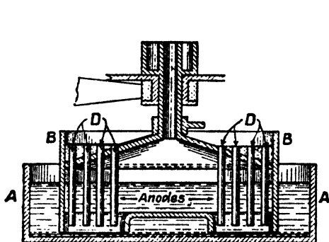
FIG. 10.—The Rhodin Cell.
