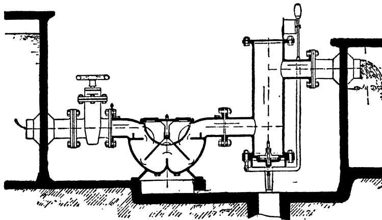
Section Through "R.U.V." Steriliser. Type C. 3.
