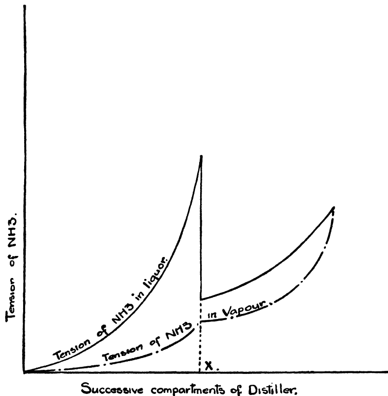
FIG. 12.—Tension of NH 3 in Liquor during Process of Distillation.
