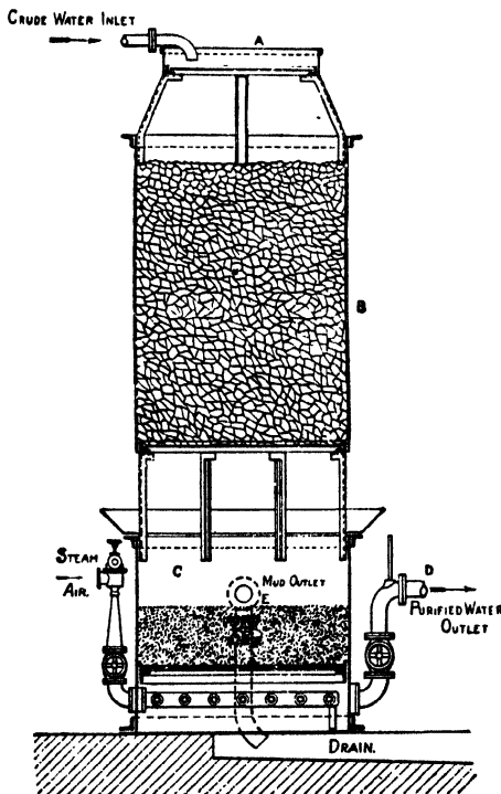
FIG. 12.—Royle's Reiser's Type "FO" Iron-removing Filter.
