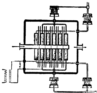
FIG. 6.—Abraham-Marmier System.
