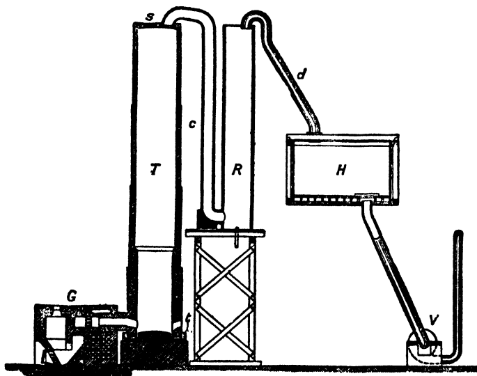
FIG. 29.—Gaillard Towers.
