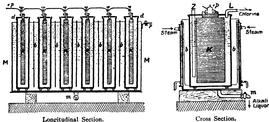
FIG. 1.—The Griesheim Cell.
