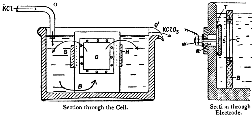
FIG. 2.—Lederlin-Corbin Electrolytic Cell for Chlorate.
