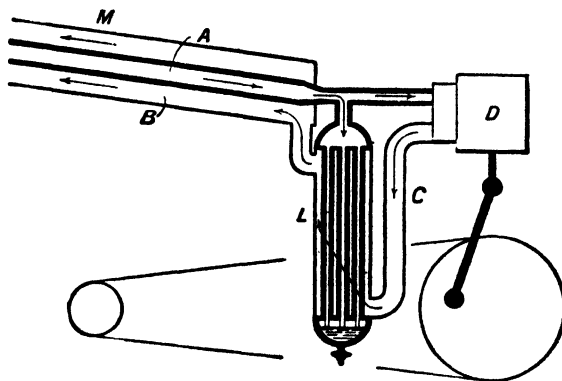
FIG. 10.—Claude Process.
