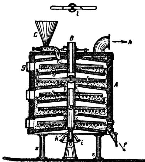
FIG. 2.—Herreshoff Mechanical Furnace for Pyrites.
