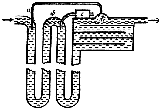
FIG. 12.—Howard-Bridge System for Treatment of Water.
