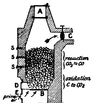
FIG. 2.—Section through a Producer.
