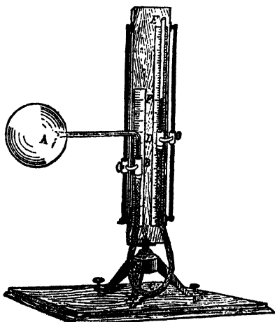
FIG. 5.—Air Thermometer.
