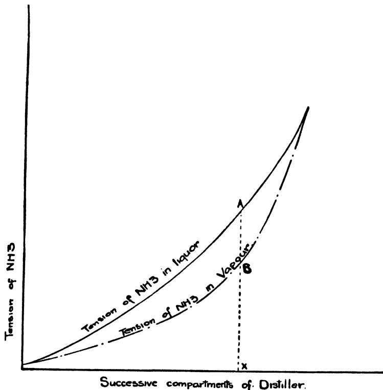
FIG. 11.—Ideal Conditions for Ammonia Distillation.
