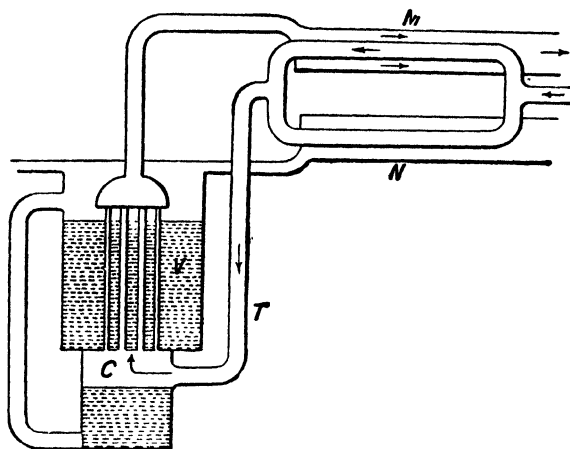
FIG. 18.—Claude's Apparatus for Pure Oxygen and Nitrogen.
