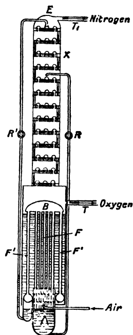
FIG. 19.—Claude's Complete Apparatus, combining the Process of Rectification with Backward Return.
