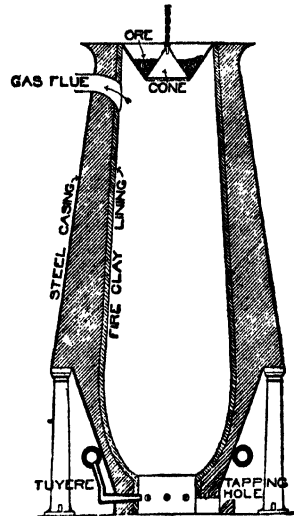
FIG. 12.—Blast Furnace.
