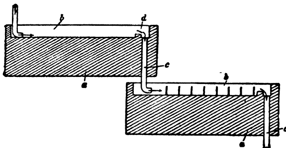
FIG. 8.—Schoop's Electrolyser.
