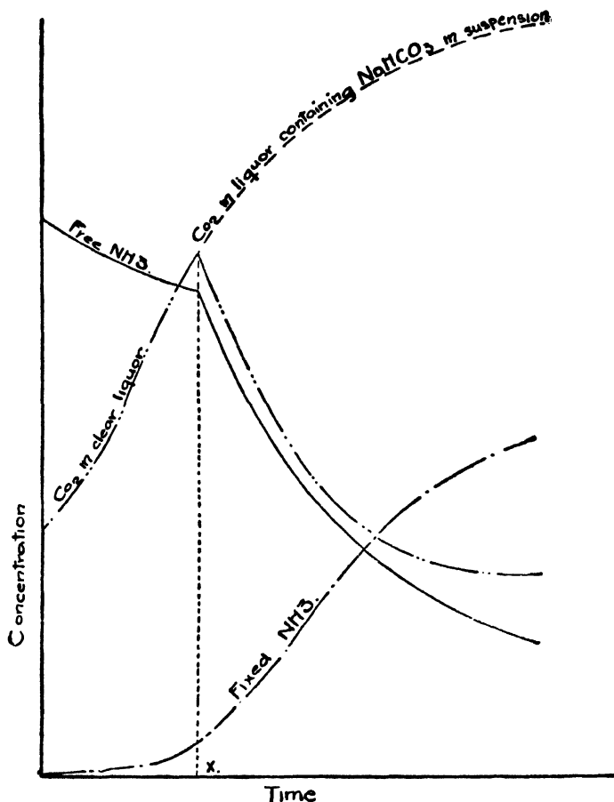
FIG. 6.—Absorption of CO 2 by Ammoniacal Brine.
