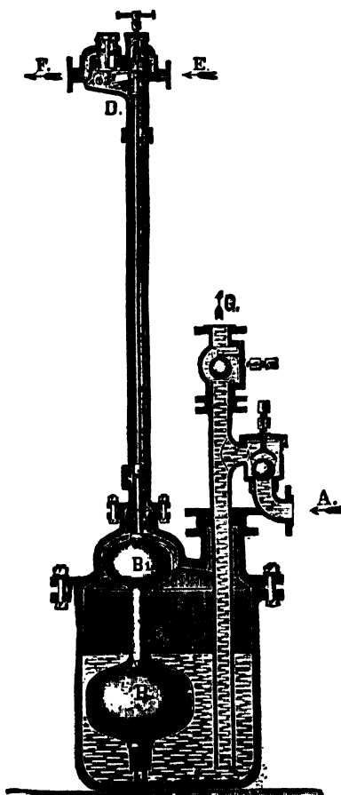
FIG. 23.—Schütze's Acid Elevator.
