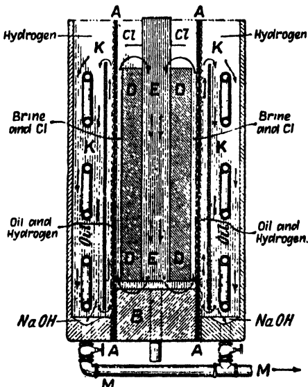
FIG. 4.—The Townsend Cell.
