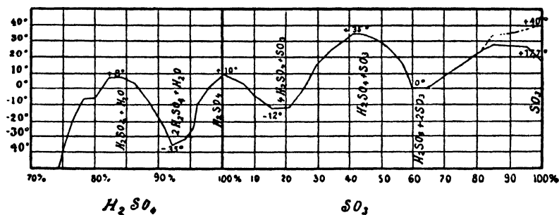
FIG. 33.—Mixtures of H_2SO_4 and SO_3 (after Knietzsch).
