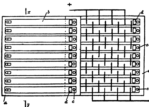
FIG. 9.—Schoop's Electrolyser.
