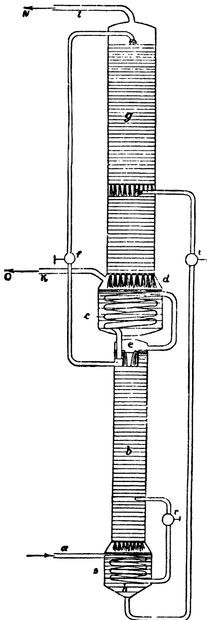
FIG. 17.—New Linde Apparatus for Oxygen and Nitrogen.
