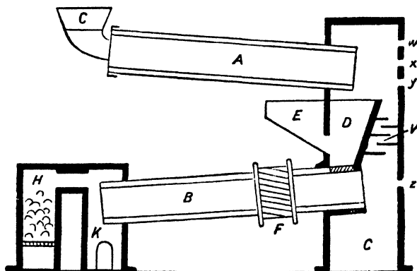
FIG. 3.—The Serpek Process.
