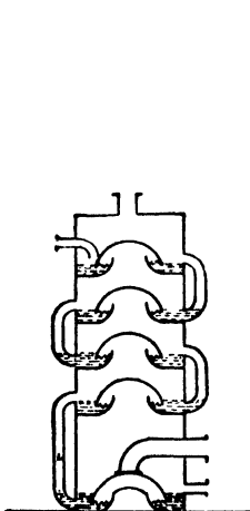
FIG. 1.—Ammonia Absorber.
