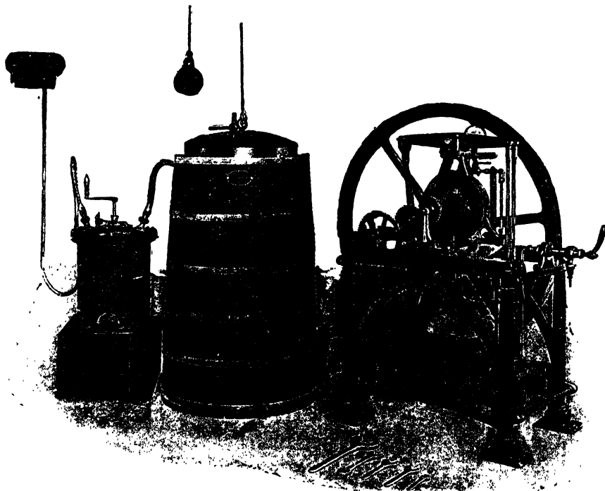
FIG. 2.—Hayward Tyler's Continuous Process Machine.
