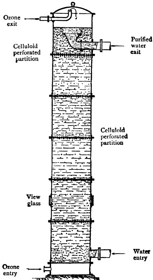
FIG. 13.—Siemens-de Vrise Water Ozonising Tower.
