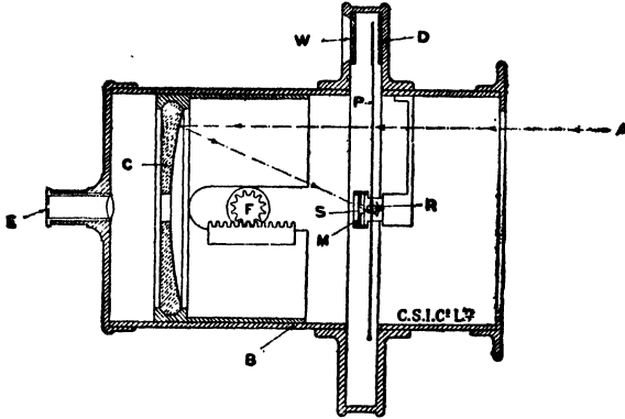
FIG. 14.—Section through Fery Radiation Pyrometer. (Cambridge Scientific Instrument Co. Ltd.)
