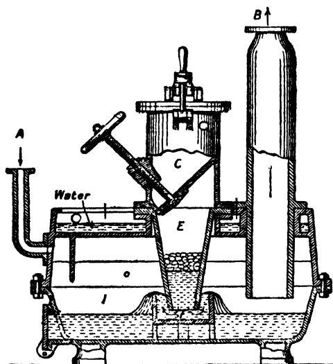
FIG. 11.—Sachsenberg Sulphur Burner.
