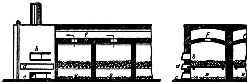
FIG. 1.—Lump Pyrites Kilns.
