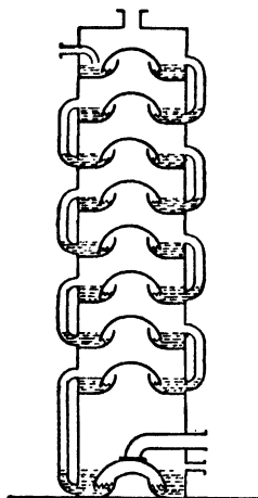
FIG. 2.—Ammonia Recovery Tower.
