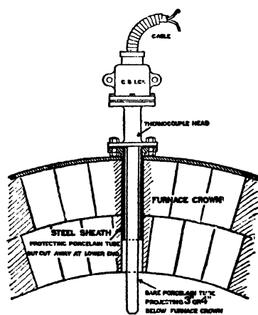
FIG. 7.—Thermo-Element in Furnace. (Cambridge Scientific Instrument Co. Ltd.)
