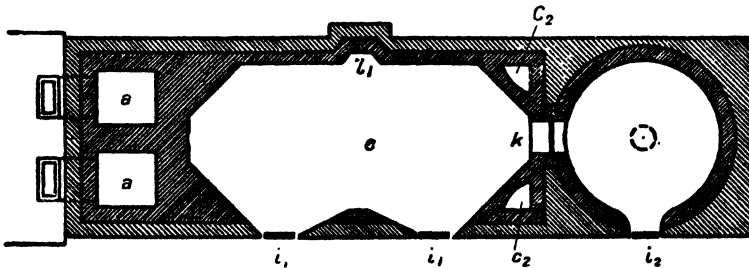
FIG. 2.—Salt Cake Muffle Furnace—Horizontal Section.
