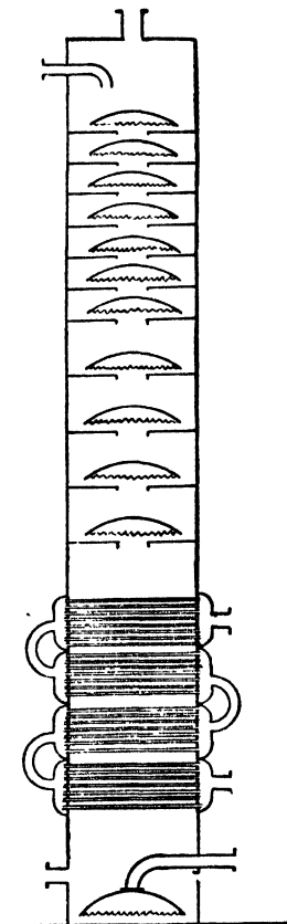
FIG. 4.—Solvay Tower.
