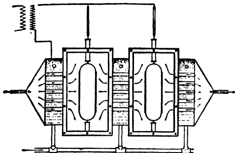
FIG. 5.—Tindal's System.
