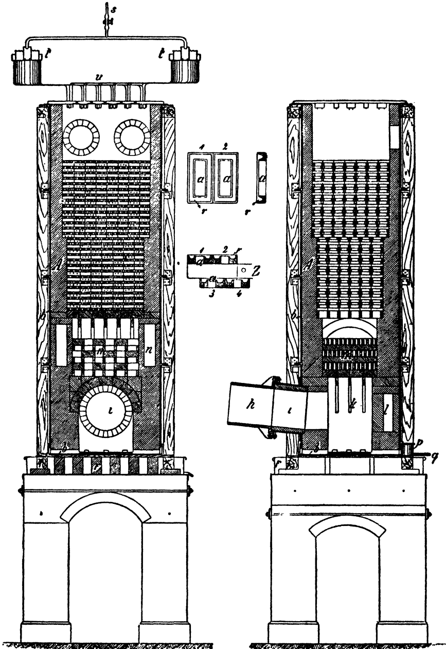
FIG. 17.—Glover Towers. Employing the Niederführ-Rohrman System of Packing. The Two Vertical Sections above shown are cut at Right Angles to each other. (See p. 227.)
