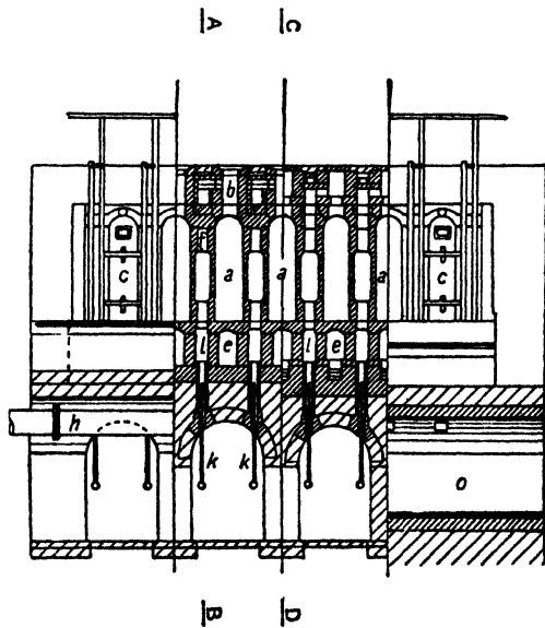
FIG. 4.—The Otto Oven (Cross Section).
