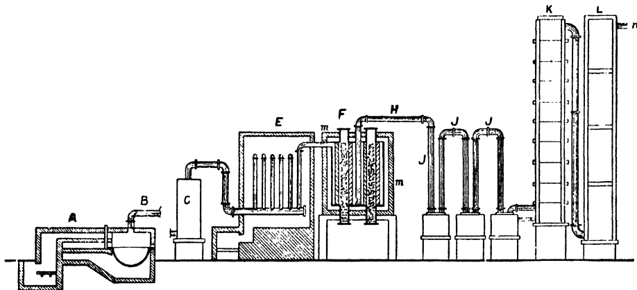
FIG. 4.—Deacon Process of Chlorine Manufacture.
