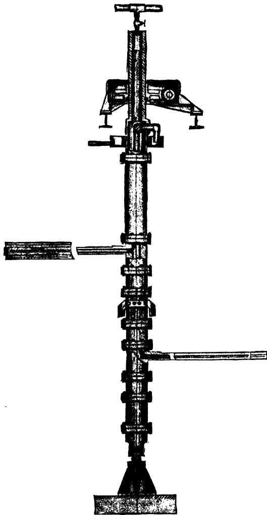
FIG. 3.—The "Harris" Patent Water-cooled Flanged Aim and Shaft for the Wedge Furnace. (See p. 212.)
