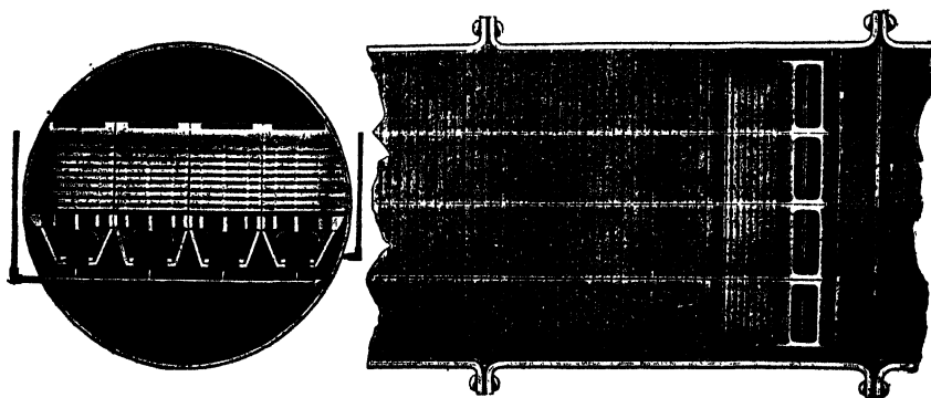
FIG. 5.—Transverse Section and Plan of Fig. 4. (Galloways Ltd., Manchester.)
