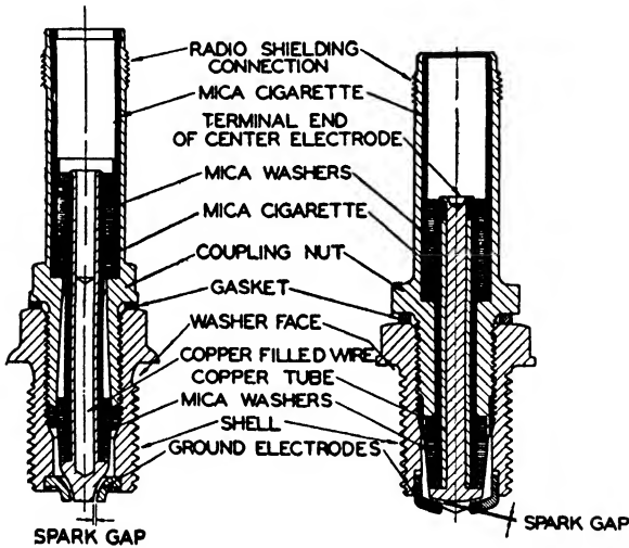
FIG. 296. Typical American mica insulated sparking plugs.
