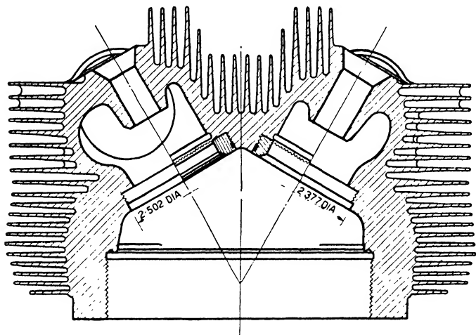
FIG. 181. Sectional view of Bristol aluminium alloy cylinder head.
