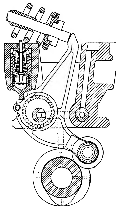
FIG. 225. Hydraulic automatic adjustment device applied to rocker arm.
