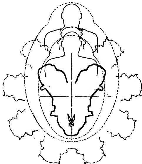
FIG. 5. Comparison of twelve-cylinder vee and nine-cylinder radial type engines of similar output.
