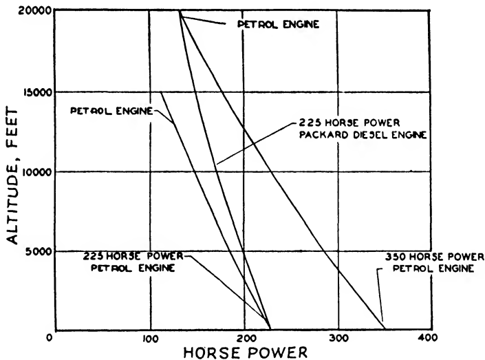
FIG. 149. Flight test results with aircraft C.I. and petrol engines.
