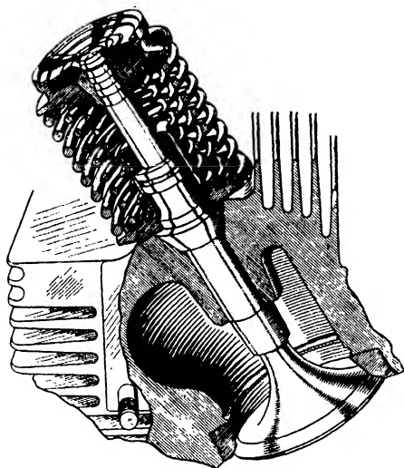
FIG. 220. The assembled Bristol valve in its working position.
