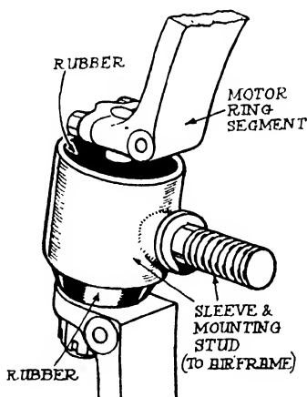
FIG. 243. Detail of one of the Bristol flexible engine mounting members.
