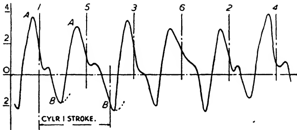
FIG. 316. Exhaust pressure curves for six-cylinder engine.
