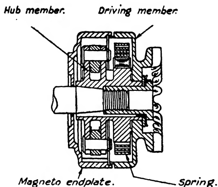
FIG. 334. Sectional view of B.T.H. Type Z impulse starter.
