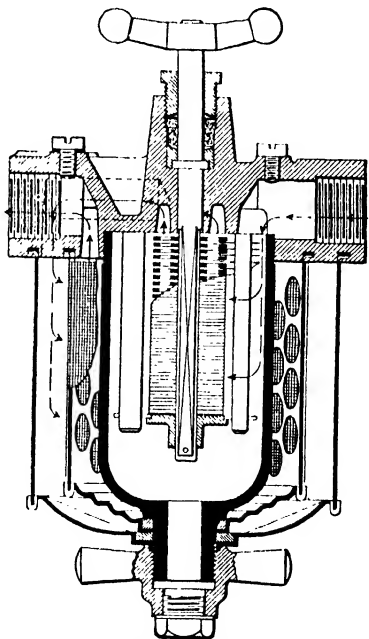
FIG. 248. The Autoclean type of filter.
