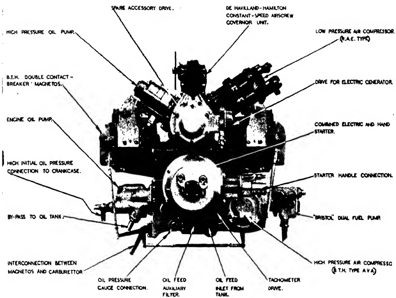
FIG. 329. The Bristol "Pegasus" engine accessory arrangement.
