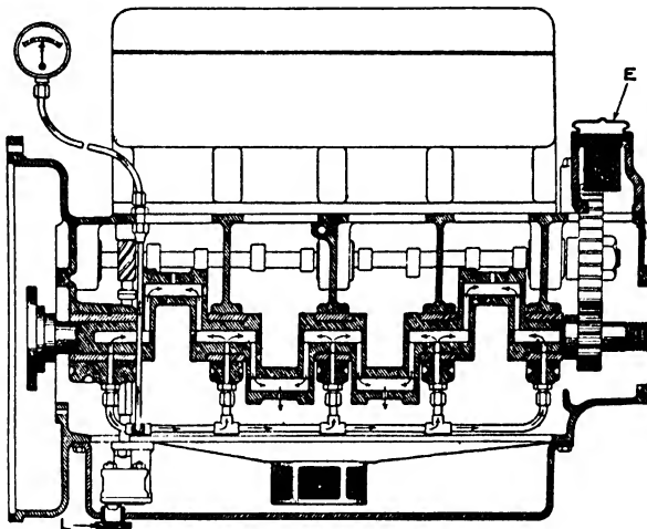
FIG. 245. The pressure-splash lubrication system. E denotes the oil filler with strainer. The pressure gauge is on the delivery side of the oil pump.
