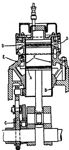
FIG. 145. Single-sleeve valve two-cycle C.I. engine.
