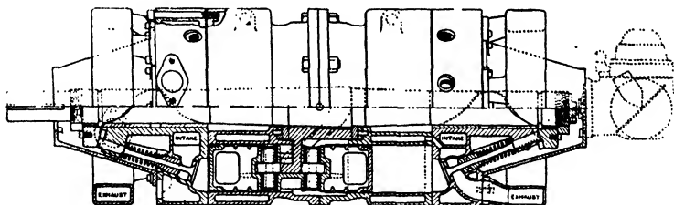
FIG. 174. The Herrmann barrel engine with twelve cylinders (140 h.p.).
