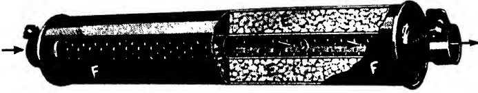
FIG. 318. The Burgess silencer.
