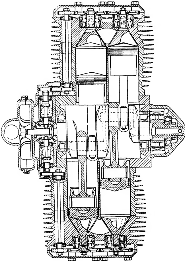
FIG. 50. The Aspin rotary valve opposed cylinder engine.
