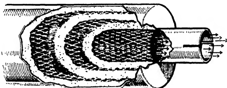
FIG. 319. The Servais absorption type silencer.
