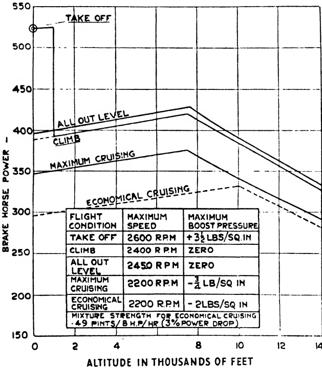
FIG. 55. Performance curves for Gipsy Twelve engine.
