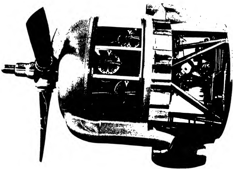
FIG. 133. Installation of Bristol "Hercules" engine complete with cowling and cooling gills.
