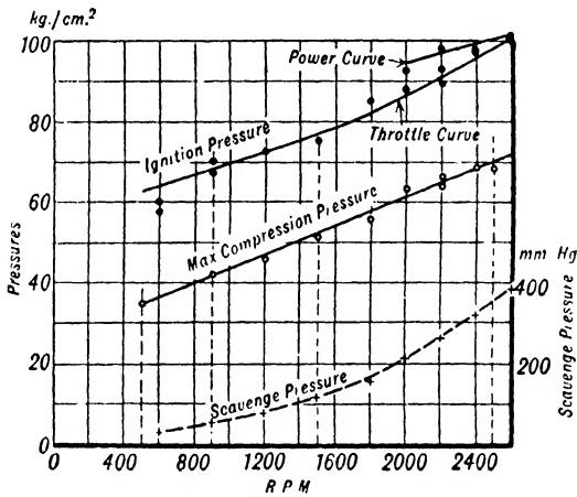
FIG. 165. Pressure values for the Jumo 205 engine at various speeds.
