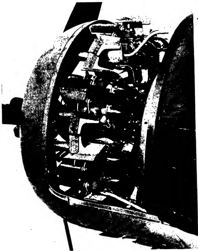
FIG. 89. The inter-cylinder baffles on the Bristol "Mercury" engine as installed in an aircraft.
