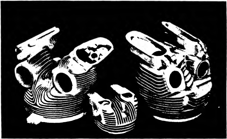
FIG. 182. Some typical cylinder head castings in Hiduminium alloy. ( High Duty Alloys Ltd. )
