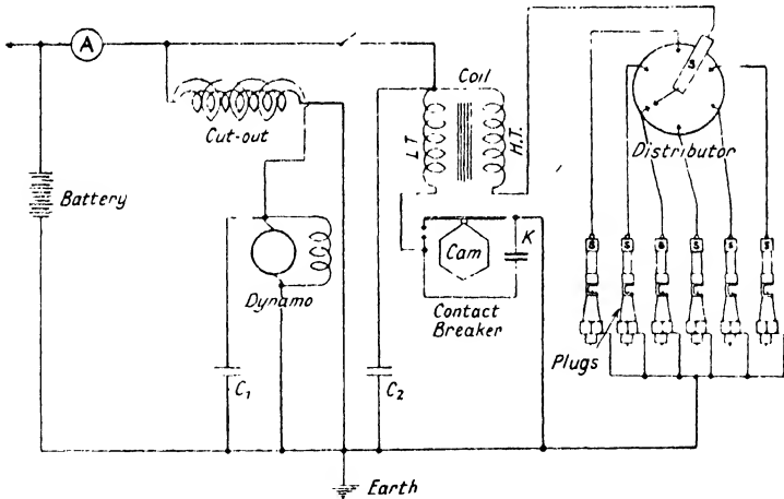
FIG. 294. A typical screened coil ignition system for six-cylinder engine.
