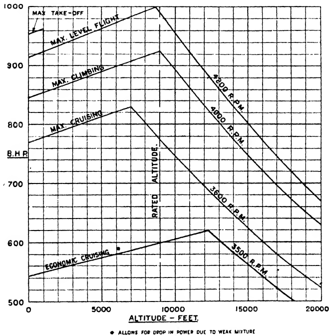
FIG. 76. Performance curves of Napier "Dagger VIII" engine.
