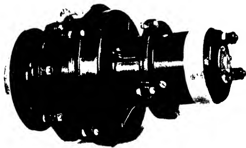
FIG. 341. Rotax-Eclipse combined hand and electric inertia starter. This operates off a 12 v. accumulator and weighs 30\frac{1}{2} lb.
