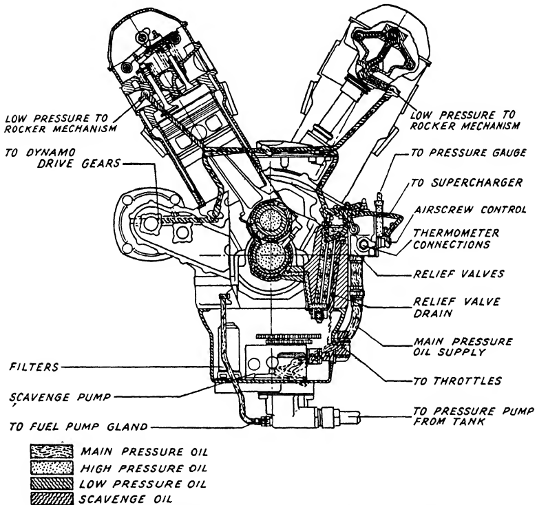
FIG. 270. The Rolls Royce "Merlin" engine lubrication system in front sectional view.
