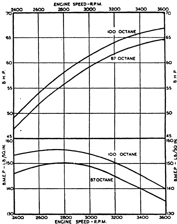
FIG. 116. Performance curves for Bristol "Aquila" size single-sleeve valve cylinder.
