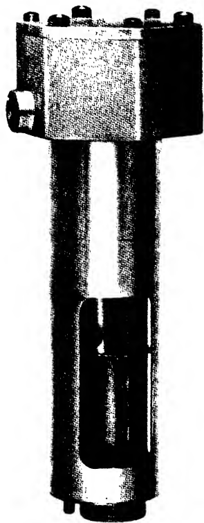
FIG. 249. The Cuno self-cleaning oil filter used in Wright engines
