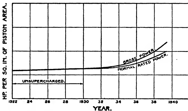
FIG. 65. Illustrating progress in liquid-cooled Vee-type engines.
