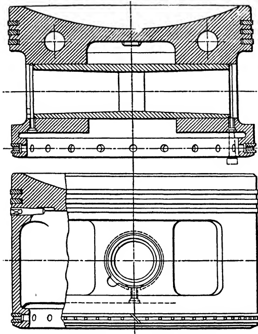
FIG. 195. Typical aircraft engine piston. ( Rolls Royce. )
