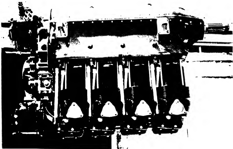
FIG. 30. The Menasco "Pirate" D.S.4 supercharged four-cylinder engine (150 h.p.).
