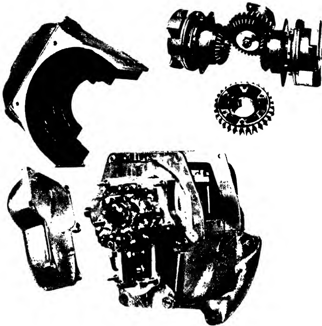
FIG. 291. One of the Bristol shielded magnetos and details of the engine drive.
