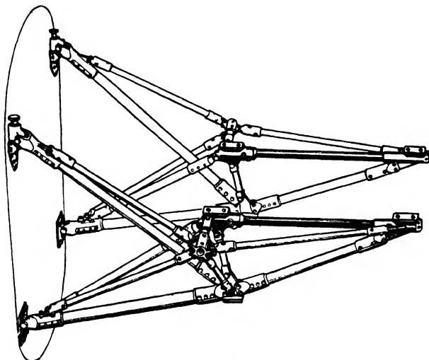
FIG. 235. Mounting for Vee-type engine. ( The Aeroplane. )
