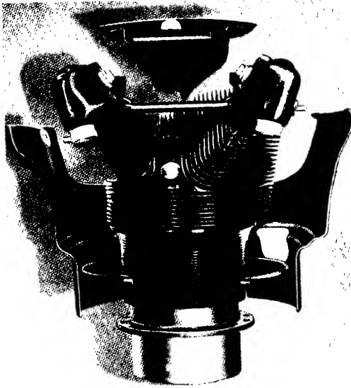
FIG 92. Cylinder and baffles of "Wasp" engine.
