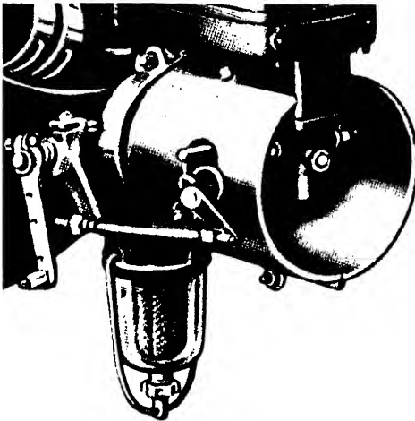
FIG. 48. The Continental fuel injector having cylindrical plungers which reciprocate for pumping and rotate for positive valving.
