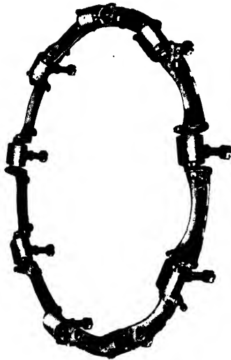
FIG. 242. Flexible mounting for Bristol radial engines.
