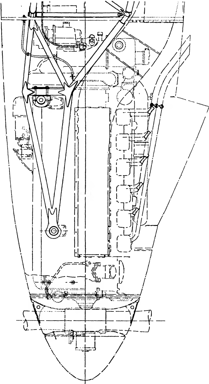
FIG. 57. Side view showing typical installation of Gipsy Twelve engine in aircraft.
