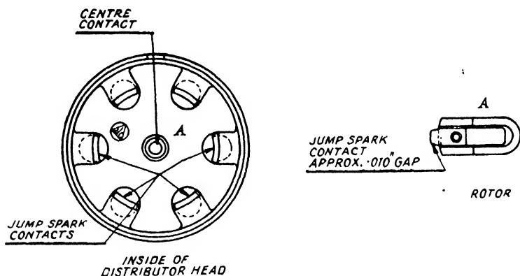
FIG. 276. The "jump spark" type of distributor. The rotor on right is attached to shaft at A (left).
