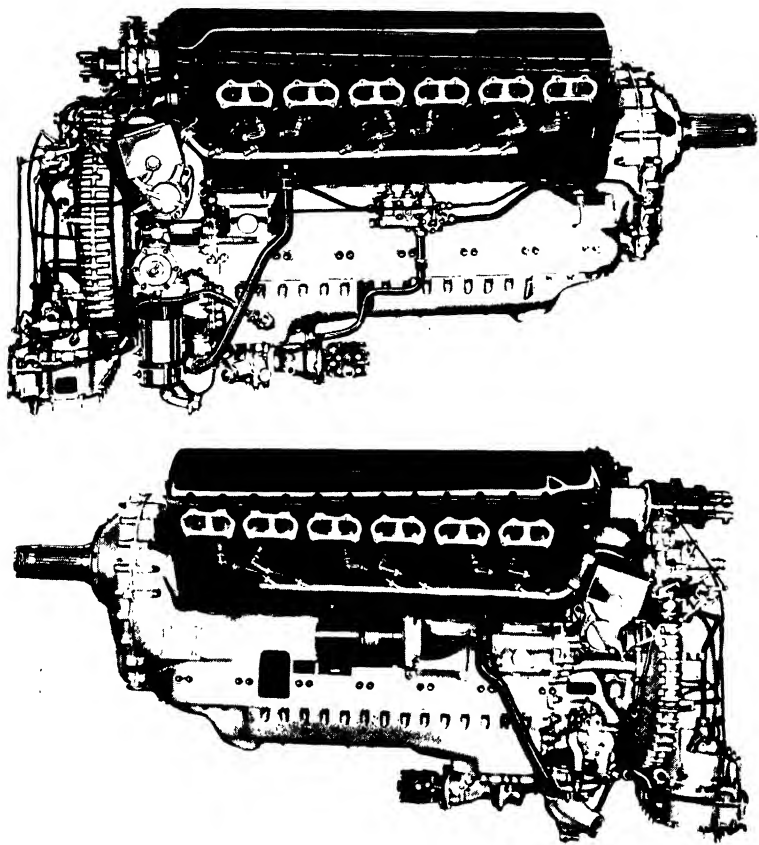
FIG. 67. The Rolls Royce "Merlin" engine.
