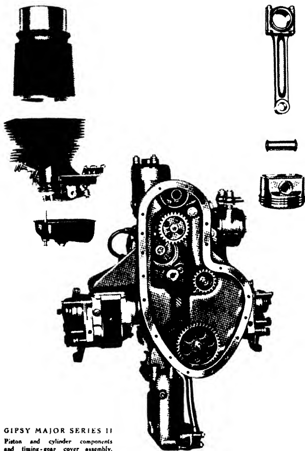
FIG. 183. Piston and cylinder components and timing gear cover of "Gipsy Major" Series II engine.
