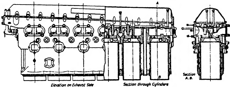
FIG. 187. Cylinder block of Rolls Royce "Merlin" engine. ( Machinery. )
