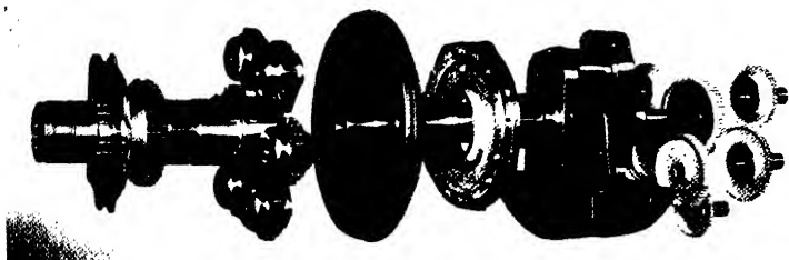
FIG. 212. The Wright "Cyclone" (G.100) crankshaft arrangement showing concentric airscrew reduction gear on left and accessory drive gears on right. The components are shown separated for clearness.
