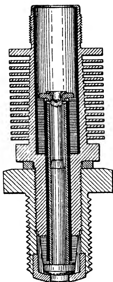
FIG. 304. Bendix aircraft engine sparking plug.
