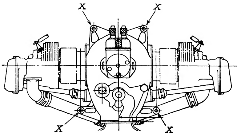
FIG. 234. Mounting of opposed-cylinder engine.
