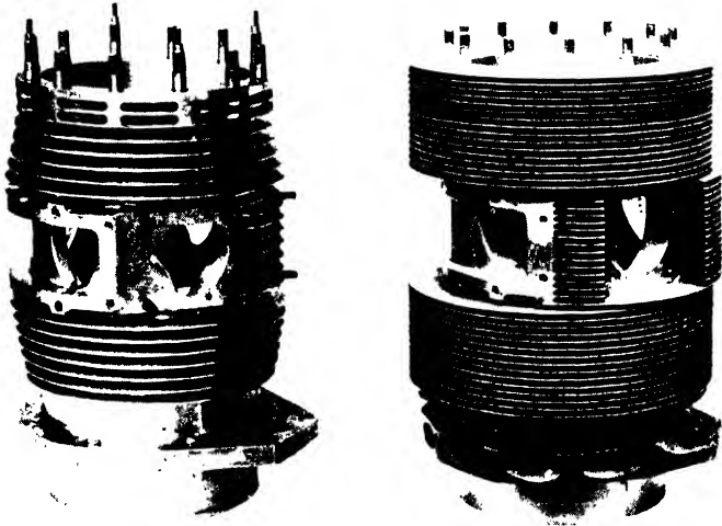
FIG. 126. The original "Perseus" cylinder ( left ) and that of the latest production type ( right ).
