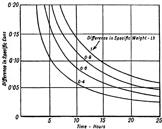
FIG. 141. Curves showing flying time necessary for equal total weight of engine, fuel and fuel tanks of engines of different specific weight and consumption.
