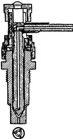
FIG. 62. One of the fuel-injection nozzle units.
