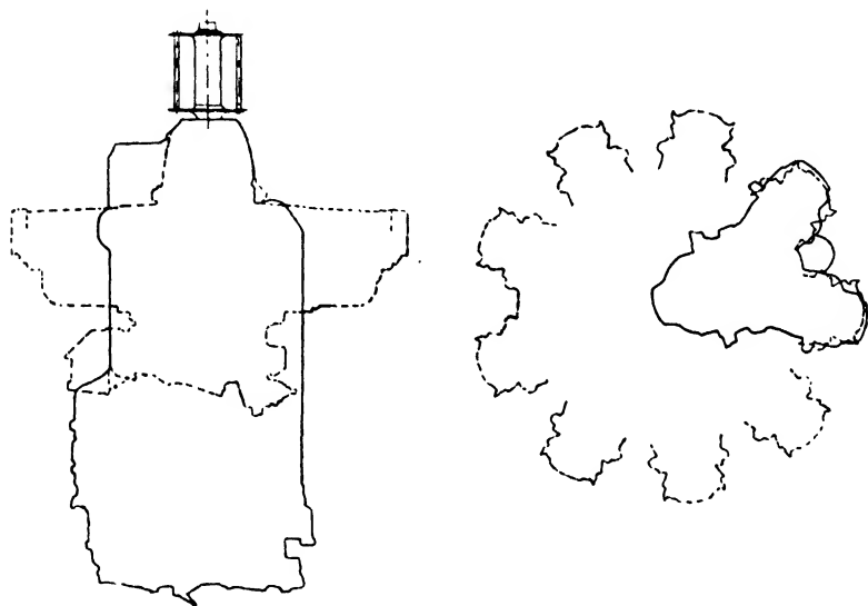
FIG. 6. Plan and frontal areas of twelve-cylinder vee and nine-cylinder radial engines of similar outputs.
