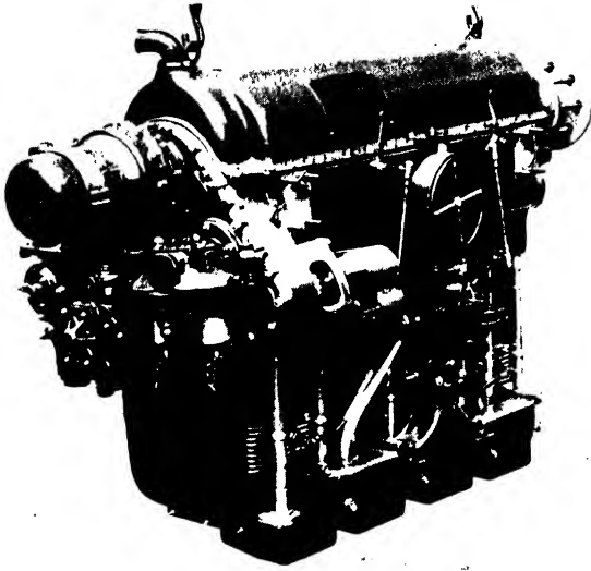
FIG. 33 The "Cirrus Major" engine showing carburettor and rear-end accessories.
