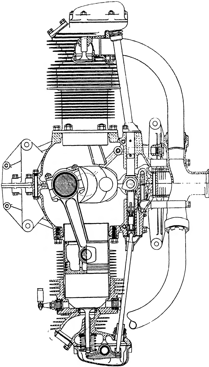
FIG 45. The Continental four-cylinder opposed engine in sectional view.
