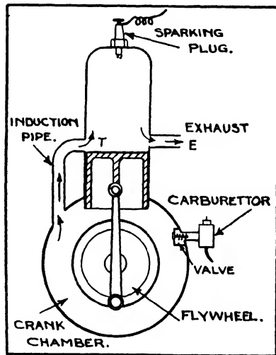
FIG. 134. Principle of the two-cycle engine.
