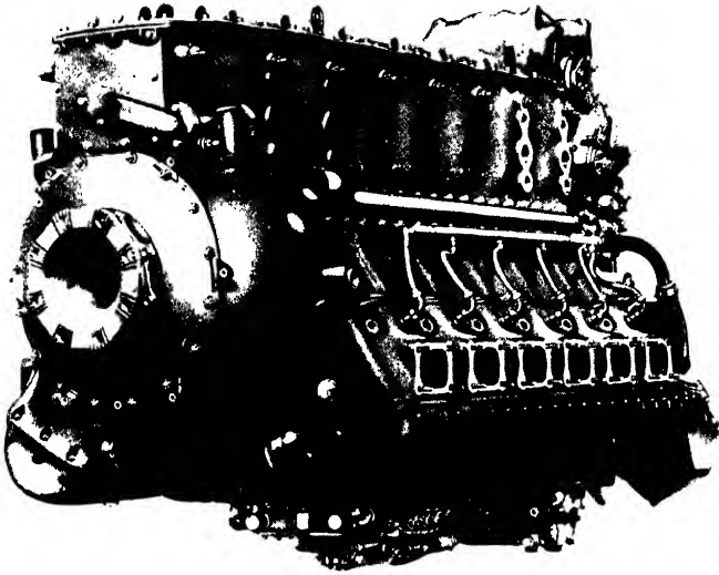
FIG. 50. The Junkers "Juno 211A" inverted twelve-cylinder liquid-cooled engine (1,200 h.p.). (Courtesy "The Aeroplane.")
