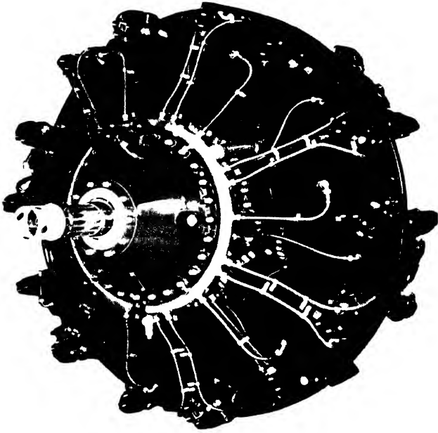
FIG. 106. Wright Double Row "Cyclone 14" fourteen-cylinder radial engine (1,600 h.p.).
