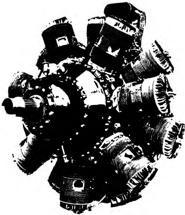
FIG. 131. Bristol "Taurus II" medium supercharged sleeve valve engine.
