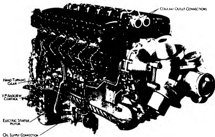
FIG. 69. Three-quarters front end view of "Merlin" engine, showing starting gear, variable pitch airscrew and other details.
