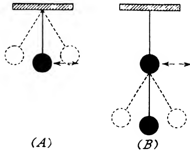
FIG. 16. Principle of pendulum-type damper.
