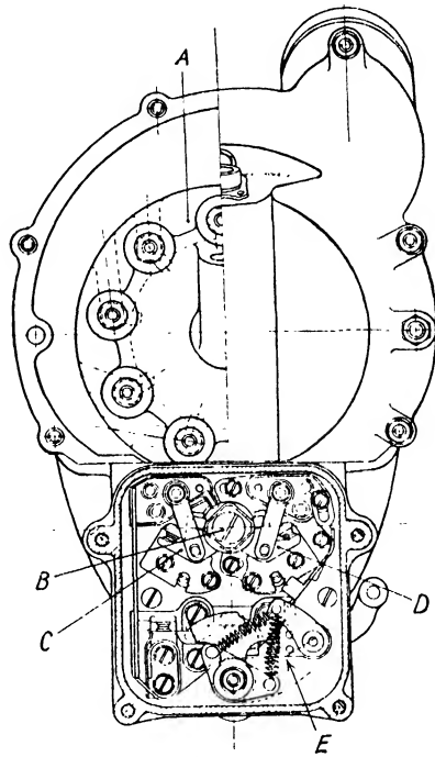
FIG. 285. End View of Rotax "Watford."
