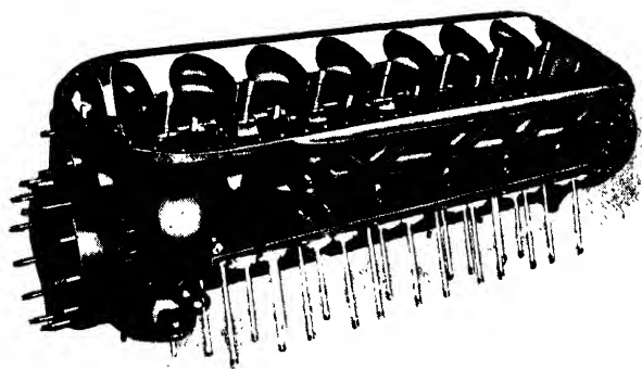
FIG. 193. Crankcase unit of the "Gipsy Twelve" inverted Vee-type engine. Showing cover and cylinder joints, etc.
