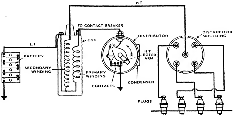
FIG. 293. General lay-out scheme for four-cylinder engine coil ignition system.
