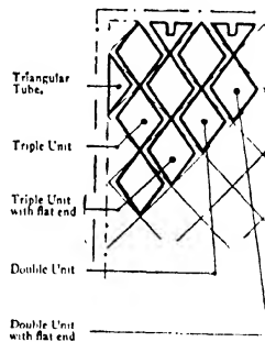
FIG. 262. Detail of Galley radiator illustrating method of construction.
