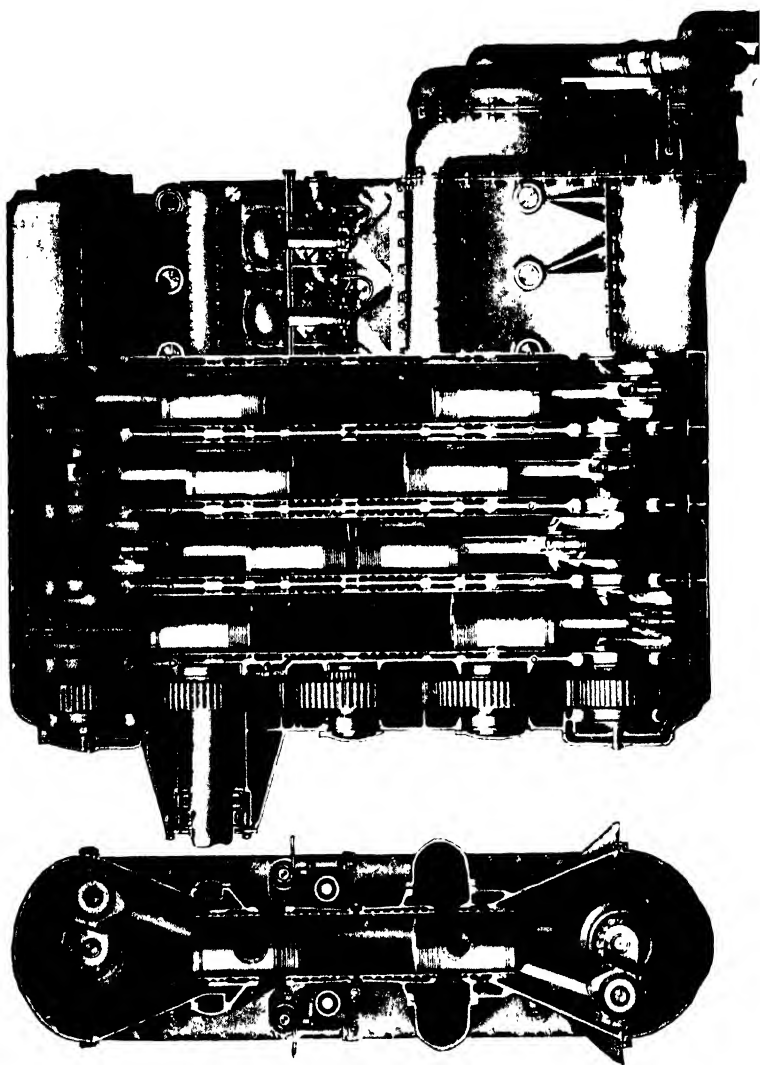
FIG. 166. Pictorial part-sectional view of the Junkers "Jumo" engine.
