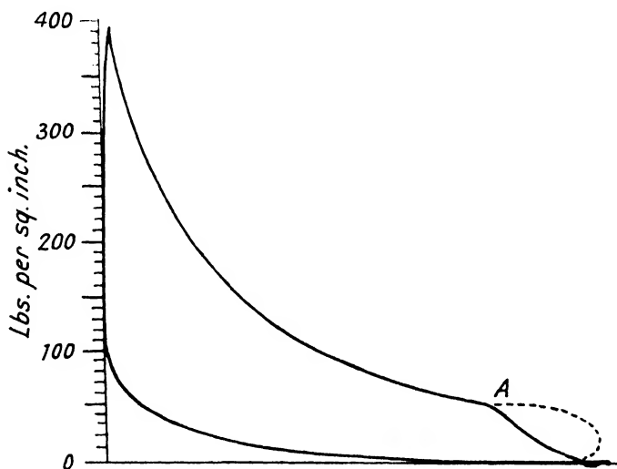
FIG. 135. Two-cycle engine indicator diagram. Dotted line shows four-cycle engine exhaust process, for comparison purposes.
