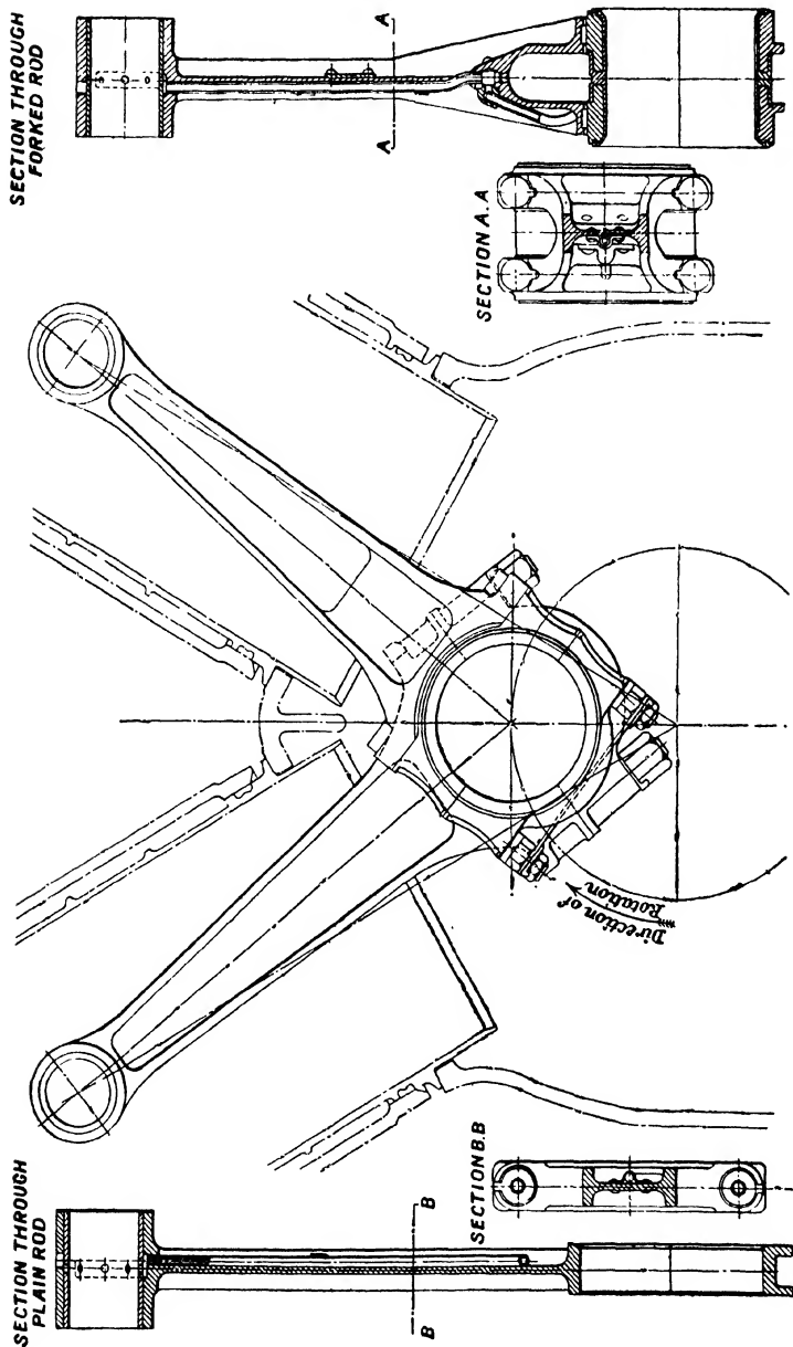
FIG. 201. Connecting-rod system of Vee-type engine. (Engineering.)
