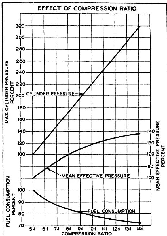
FIG. 4. Compression ratio effect on maximum and mean cylinder pressures and upon fuel consumption.
