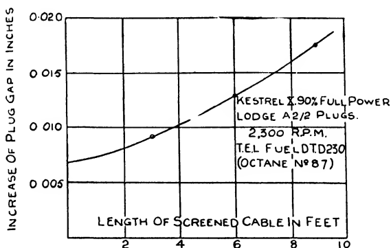
FIG. 308. Variation of erosion of sparking plug electrodes with length of screened cable.
