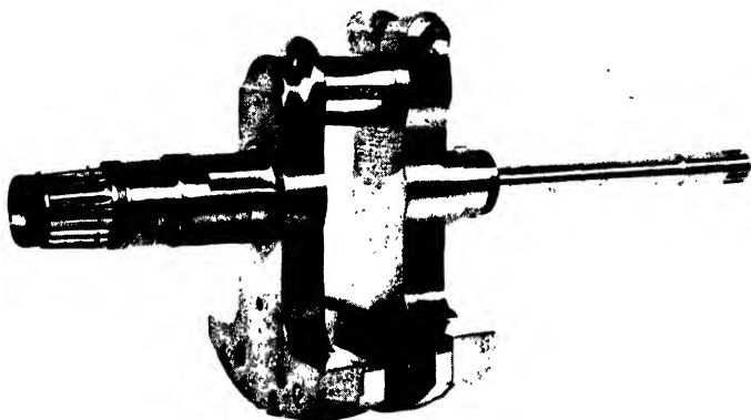
FIG. 211. The Bristol single-row radial engine crankshaft.
