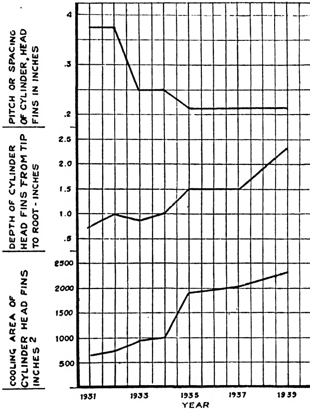
FIG. 99. Illustrating improvement in engine cooling for the Wright Cyclone engine.
