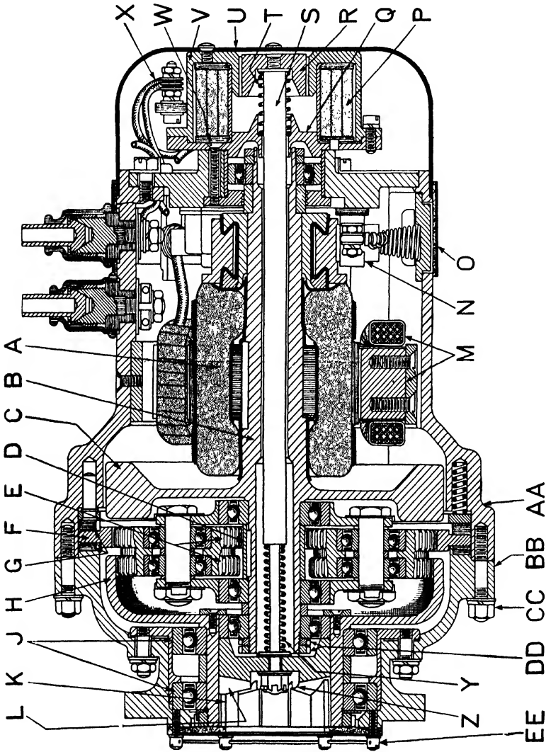
Fig. 339. The B.T.H. electric inertia starter with horizontal motor.
