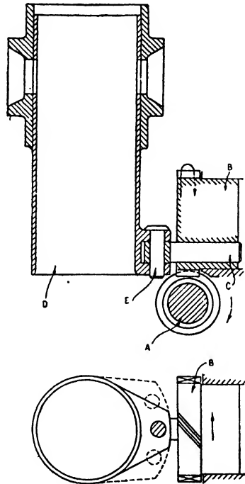
FIG. III. Principle of the single sleeve-valve engine.
