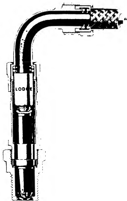
FIG. 303. The Lodge screened aircraft engine sparking plug.
