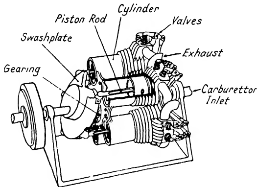
FIG. 172. Barrel-type rotary engine.
