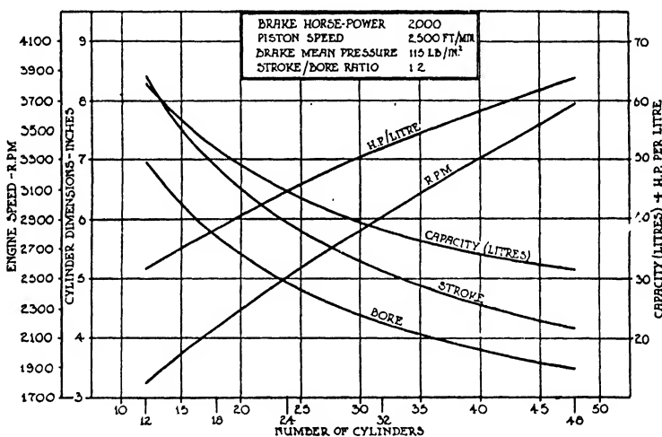
FIG. 3. Alternative cylinder choice for 2,000 B.H.P. engine.
