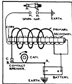
FIG. 292. Illustrating principle of the coil ignition system.
