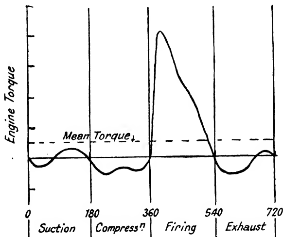
FIG. 12. Single-cylinder engine torque diagram.
