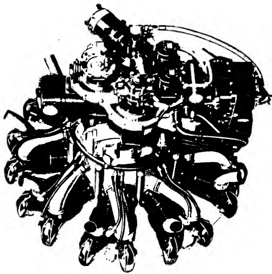
FIG. 82. The Alvis nine-cylinder radial "Leonides" engine (430 h.p.).
