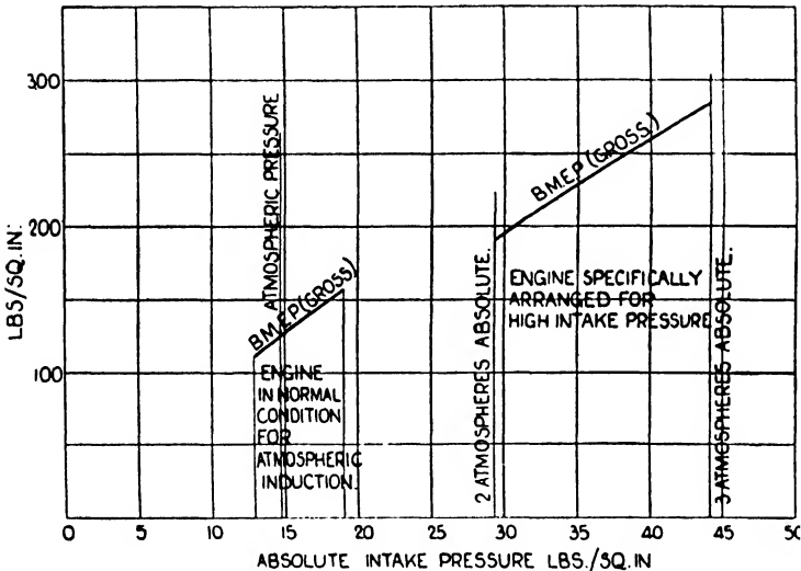
FIG. 147. Brake mean effective pressures with different degrees of supercharging C.I. engine.
