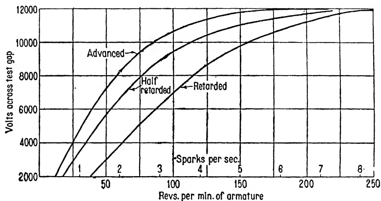
FIG. 289. Voltage curves for cobalt steel magneto.
