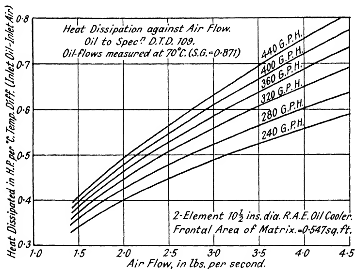
FIG. 257. Performance graphs for R.A.E. oil cooler. (J. Marston Ltd.).
