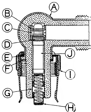
FIG. 309. The K.L.G. elbow resistor for screened sparking plugs.
