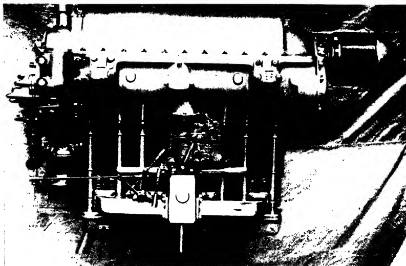
FIG. 31. The "Cirrus Minor" four-cylinder inverted engine.
