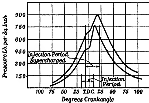
FIG. 146. Supercharging of C.I. engine.
