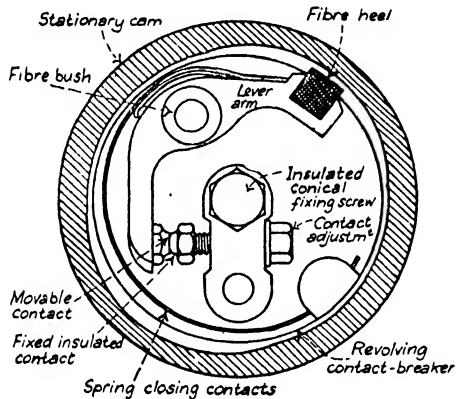
FIG. 277. Contact breaker of rotating armature magnetos.
