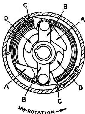
FIG. 333. Section through B.T.H. type Z impulse starter. A, pawls; B, hub member arms; C, stops on magneto end plate; D, arms on driving member.
