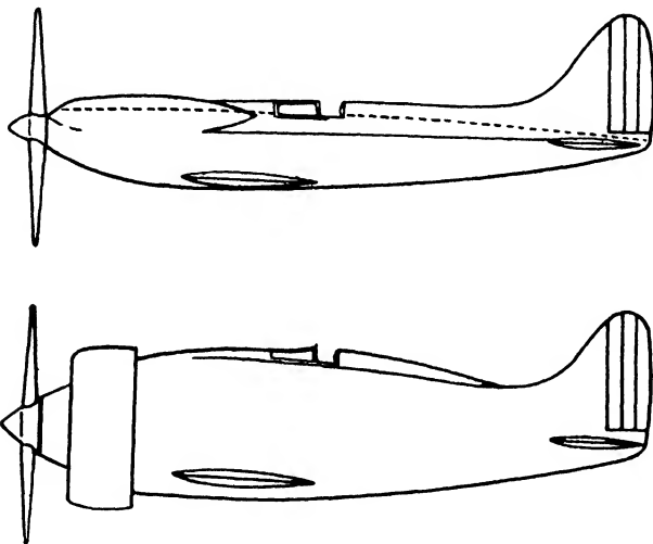
FIG. 7. Illustrating the dimensions of fuselages of the twelve-cylinder vee and nine-cylinder radial engines of similar outputs.
