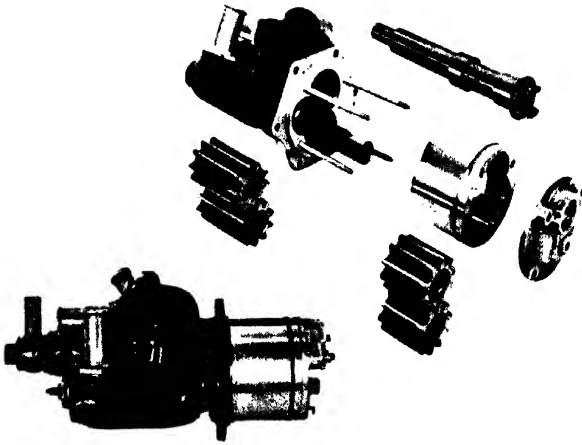
FIG. 268. The Bristol oil pump and its components.
