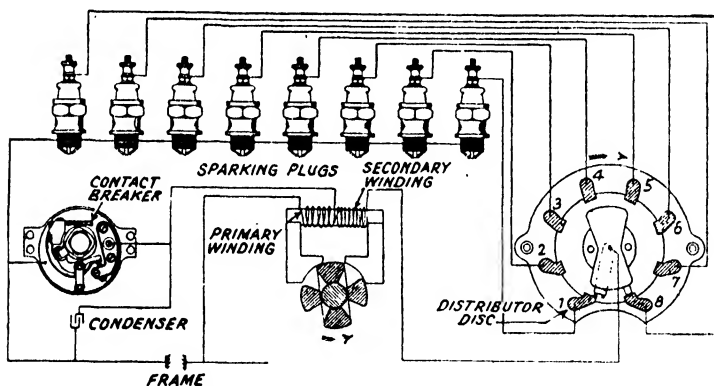
FIG. 283. Lay-out for eight cylinder polar inductor magneto circuit.
