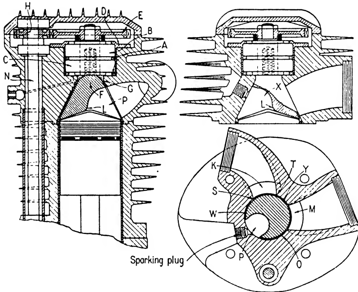
FIG. 51. Cylinder head showing rotary valve and piston of the Aspin engine.
