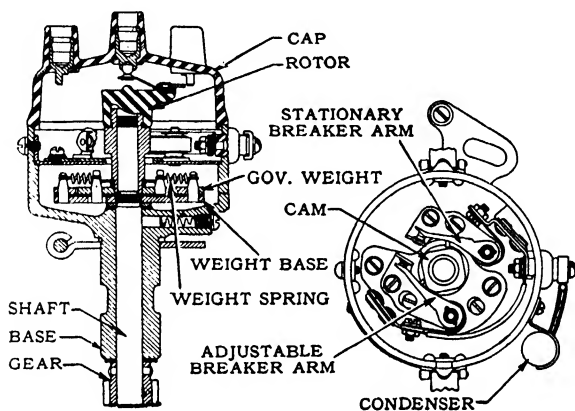
FIG. 279. Four-lobed contact breaker unit with two contact breakers, for eight-cylinder engine.
