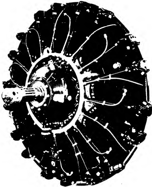
FIG. 100. Wright "Cyclone" G-100, nine-cylinder single-row radial engine (1,100 h.p.)
