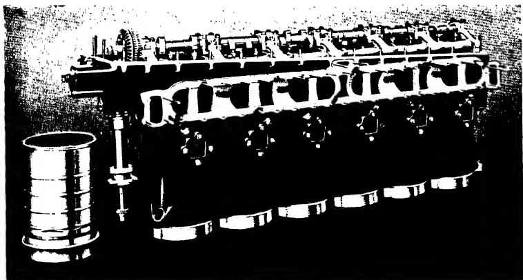
FIG. 72. Cylinder block and one cylinder barrel of "Merlin" engine.
