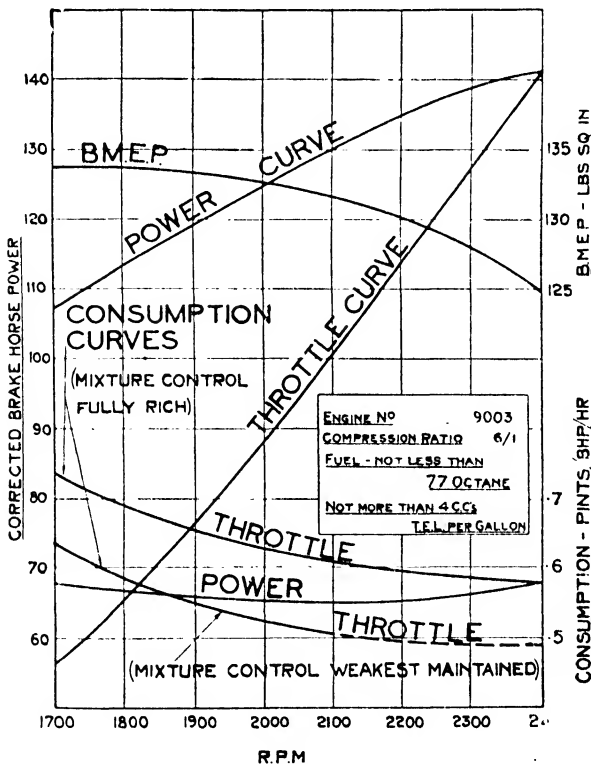
FIG. 30. Power and throttle curves for Gipsy Major Series II engine.
