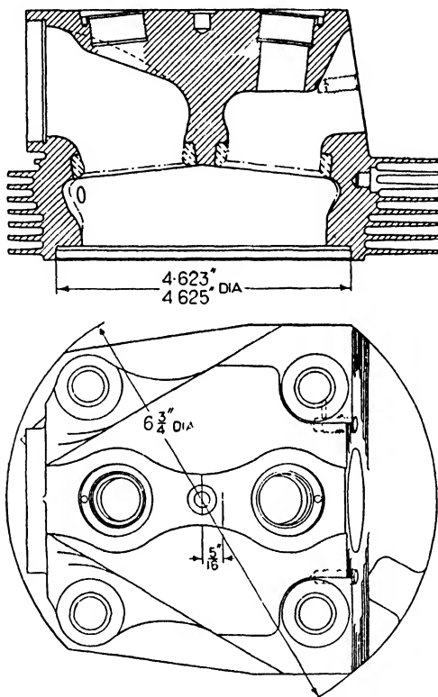
FIG. 184. Cylinder head of Napier "Dagger" engine. ( Aircraft Production. )
