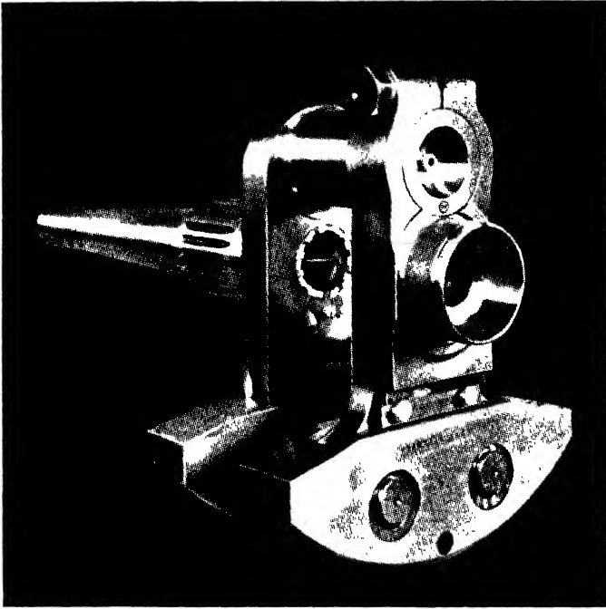
FIG. 18. The Wright radial engine pendulum damper.
