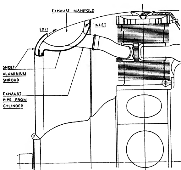
FIG. 327. Bristol shrouded exhaust manifold.
