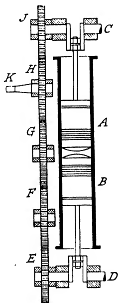
FIG. 22. The Junkers opposed piston engine principle.
