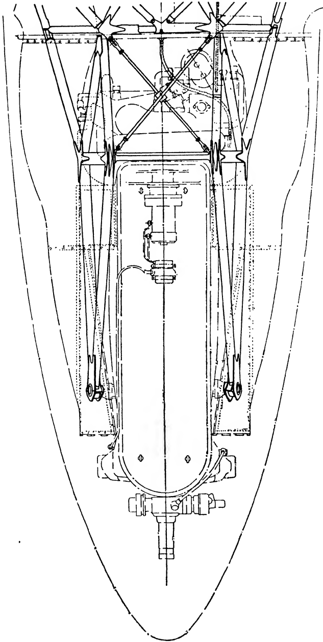
FIG. 58. Plan view of Gipsy Twelve installation in aircraft.
