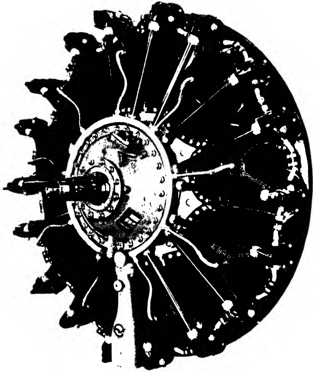
FIG. 91. Pratt and Whitney H.I. "Wasp" engine (550 h.p.).
