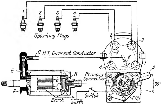
FIG. 275. Rotating armature magneto for four cylinder engine.
