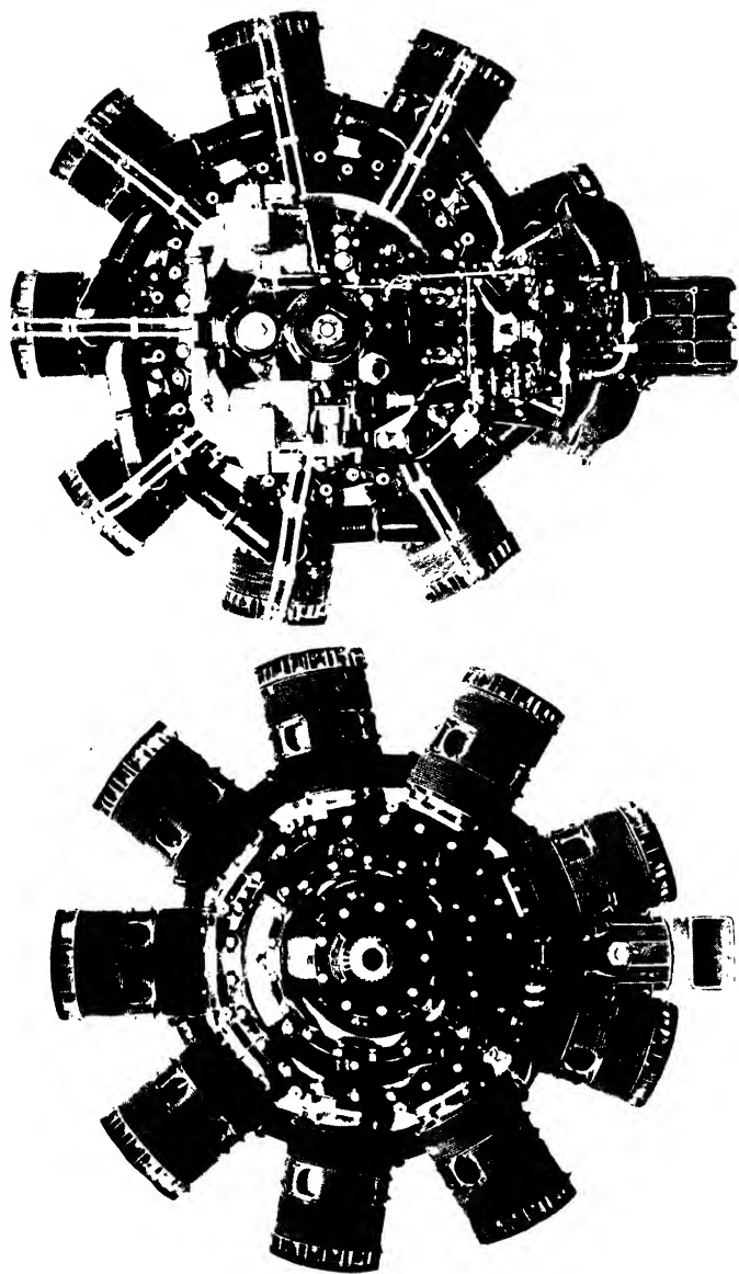
FIG. 130. Front and rear views of Bristol "Perseus XII" sleeve valve engine.
