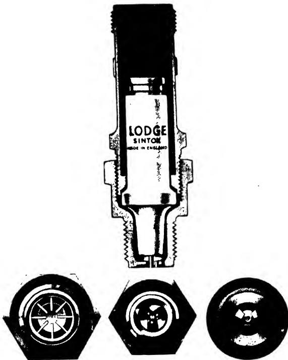
FIG. 298. The Lodge Sintox insulator sparking plug. (Below) Three alternative electrode arrangements, showing on left platinum-iridium electrode model.
