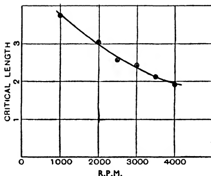
FIG. 313. Critical length of exhaust pipe for different speeds.
