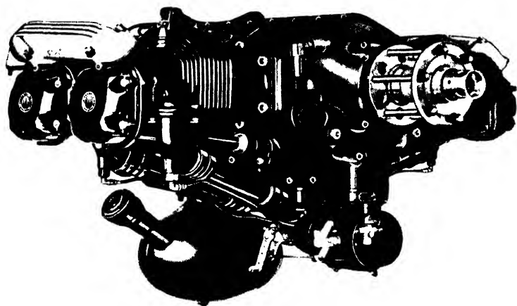
FIG. 46. The Continental four-cylinder opposed engine.
