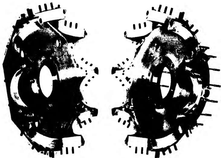
FIG. 194. Crankcase components of Bristol radial nine-cylinder engine.
