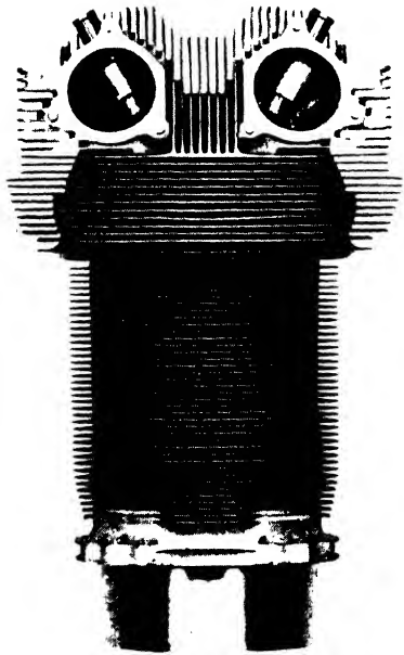
FIG. 177. The complete cylinder and head of Bristol "Mercury" and "Pegasus" engines.
