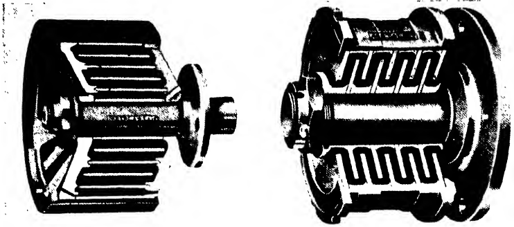
FIG. 241. "Metallastik" rubber-steel engine mountings.
