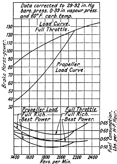
FIG. 38. Performance curves for the Menasco "Pirate" C.4 engine.
