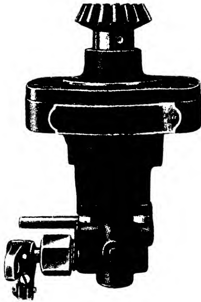
FIG. 48. The Continental fuel injector having cylindrical plungers which reciprocate for pumping and rotate for positive valving.
