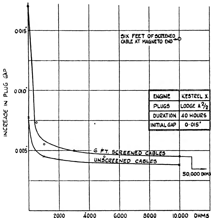
FIG. 307. Graphs showing effect upon erosion of sparking plug electrodes of resistances in series with the plugs.
