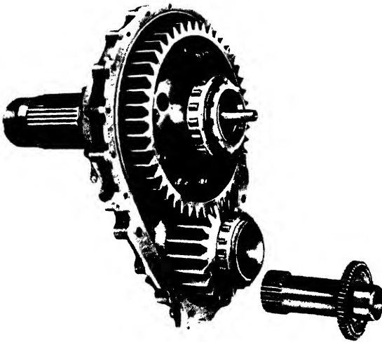
FIG. 232. The Rolls Royce "Merlin" engine airscrew reduction gear, which is similar in principle to that shown in Fig. 233.
