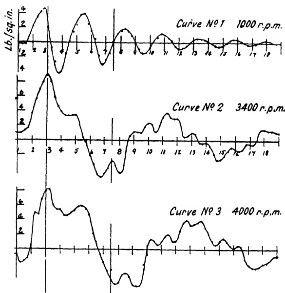
FIG. 311. Exhaust pressure curves for single cylinder engine.
