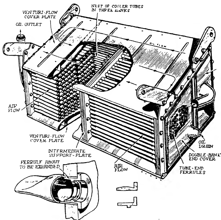
FIG. 256. The Robertson oil cooler, showing below (left) details of ferrule joint for the tubes.
