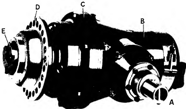
FIG. 343. The Rotax-Eclipse direct cranking electric starter. A—Hand starting connection. B—Electric motor. C—Gear wheel housing. D—Mounting flange. E—Engine engagement dogs.
