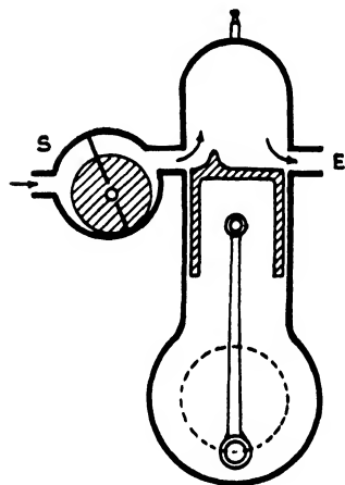
FIG. 136. Compressor-charged two-cycle engine. S, compressor; E, exhaust port. Fuel is injected after cylinder ports are closed.
