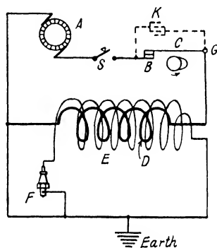
FIG. 273. Principal of rotating armature magneto.
