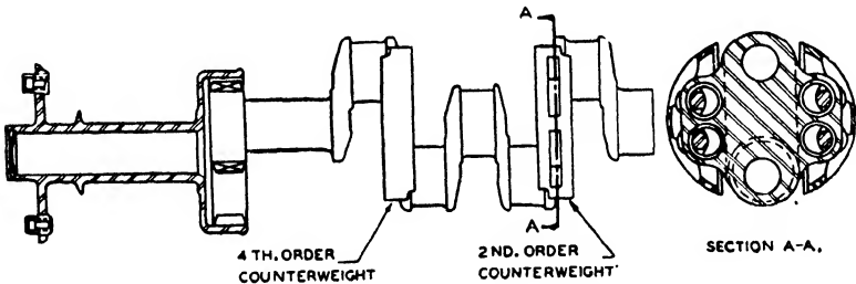
FIG. 214. Lycoming four-cylinder opposed engine crankshaft.
