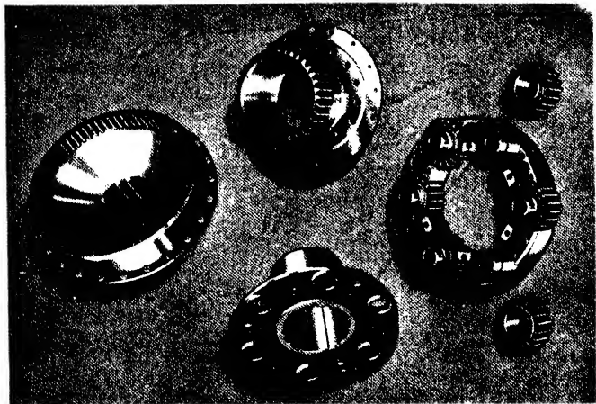
Fig. 97. Details of the airscrew reduction gear for Twin "Wasp" engine.
