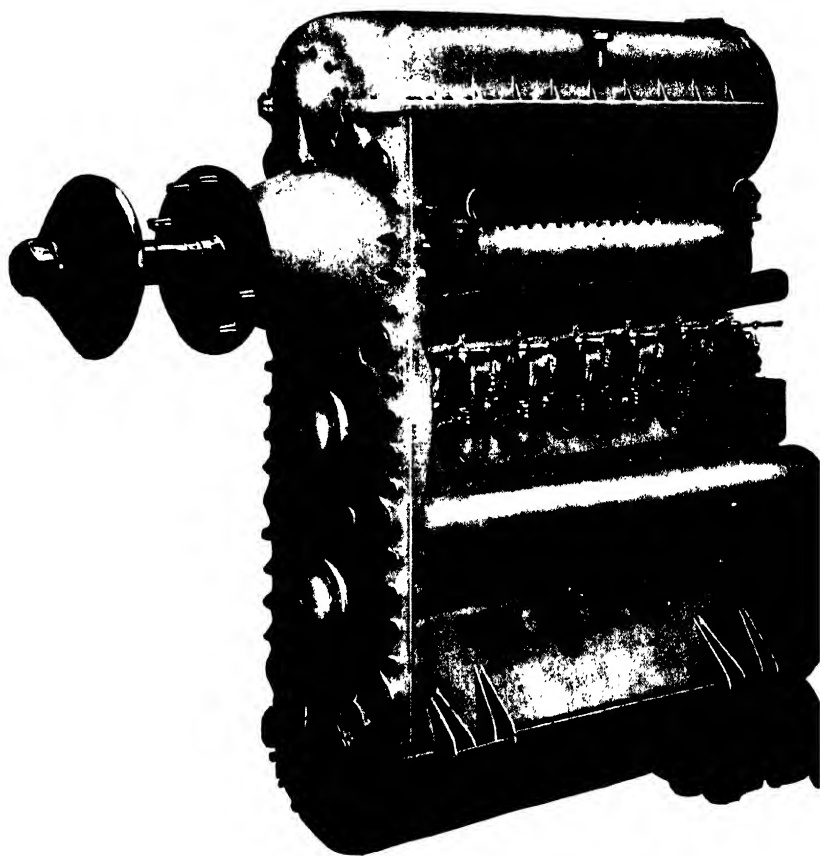
FIG. 169. Outside view of the Junker's "Jumo" six (double) cylinder engine, showing aircrew shaft.
