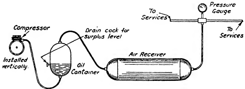
FIG. 335. Compressed air engine starting equipment.
