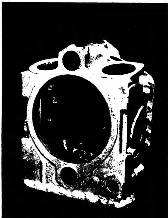
FIG. 190. Aircraft engine timing gear case cast in magnesium alloy. ( Magnesium Castings Product Co. )
