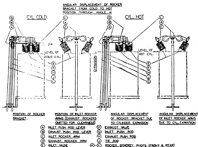
FIG. 221. The Bristol valve stem clearance compensation device.
