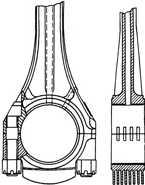
FIG. 200. Big end portion of typical light design of connecting rod.
