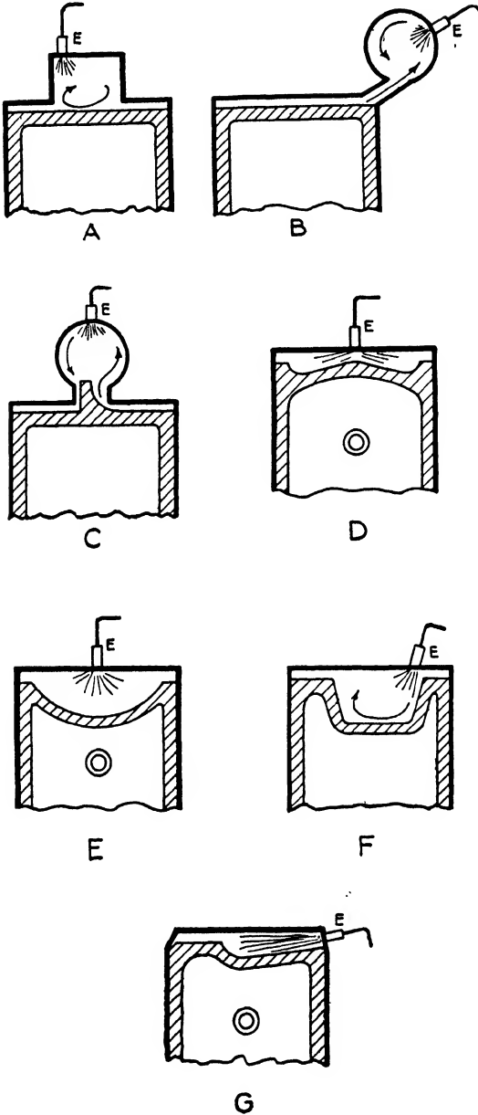
FIG. 152. Compression ignition engine combustion systems.
