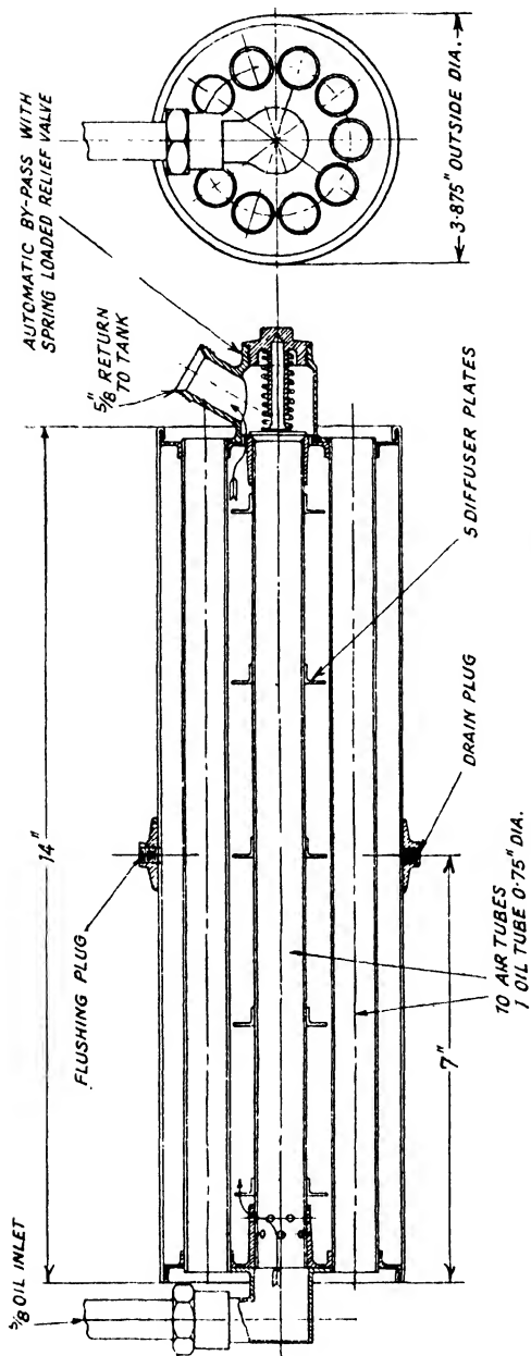
FIG. 255. The Bristol oil cooler. [R. and M. No. 1486. Courtesy the Air Ministry.]
