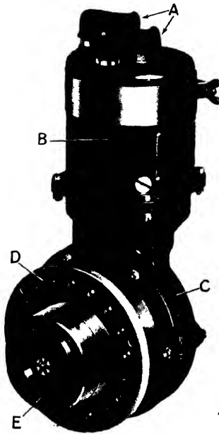
FIG. 342. Direct cranking electric starter for engines up to 200 h.p. A—Battery cable connections. B—Electric motor. C—Gear housing. D—Mounting flange. E—Engine engagement dogs.
