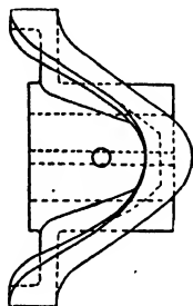
FIG. 175. The sine wave-shaped cam plate.
