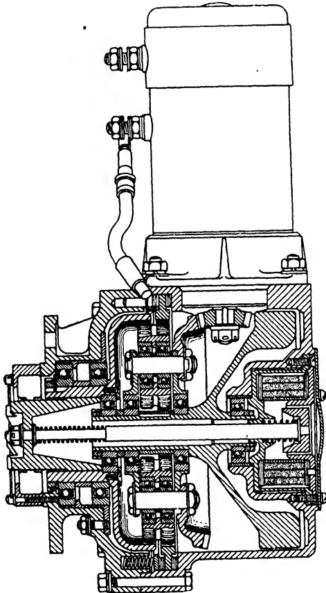
FIG. 340. The B.T.H. electric inertia starter with vertical motor.
