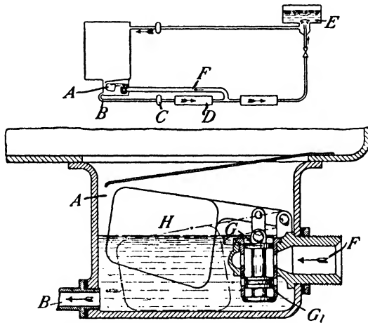
FIG. 253. Method of preventing frothing of the engine oil.
