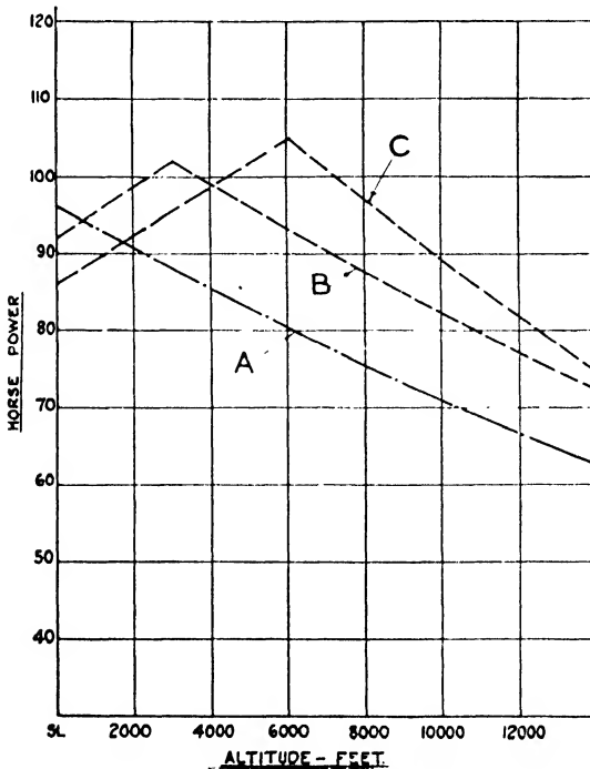
Fig. 29. Performance curves for Gipsy Major Series II engine.
