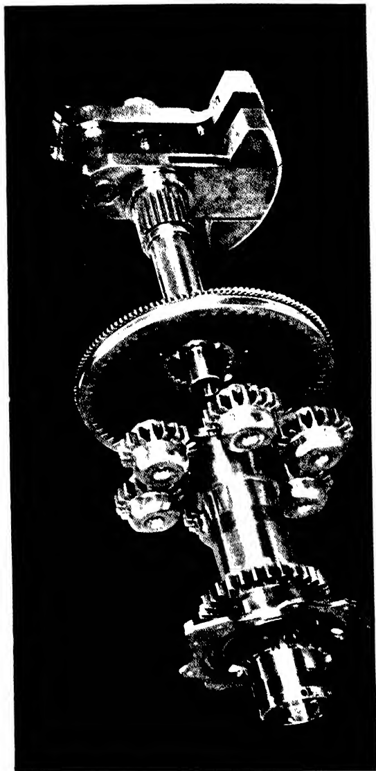
Fig. 103. The Wright "Cyclone" G.100 crankshaft and reduction gear for airscrew drive.
