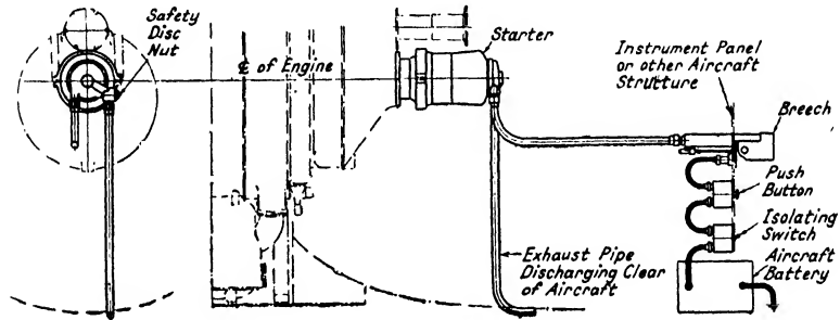
FIG. 337. Bristol cartridge starting system.
