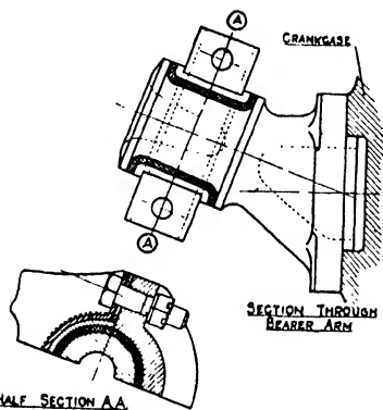
FIG. 237. Trunnion pin mounting of Gipsy Twelve engine.
