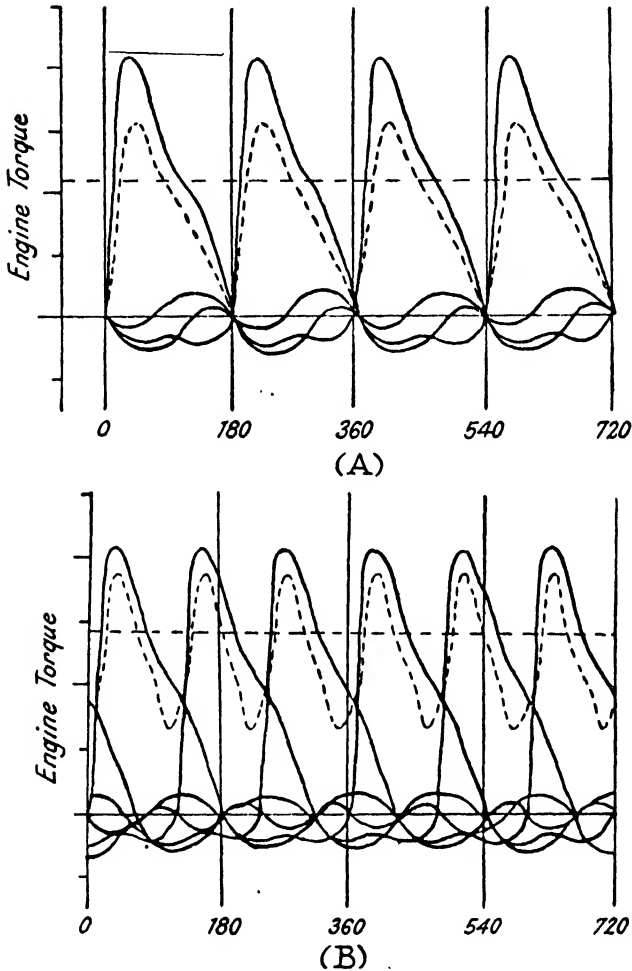
FIG. 13. Four- and six-cylinder in-line engine torque diagrams
