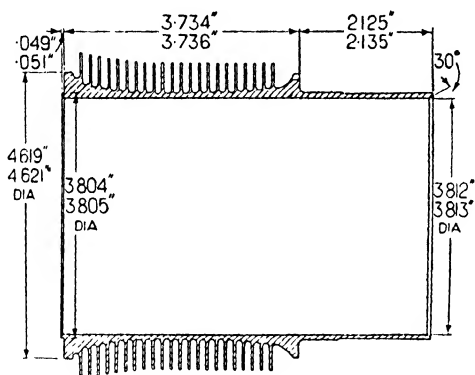
FIG. 178. Section through cylinder barrel of Napier "Dagger" engine. ( Aircraft Production. )
