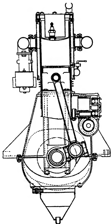
FIG. 114. The Argyll single-sleeve valve aircraft engine.
