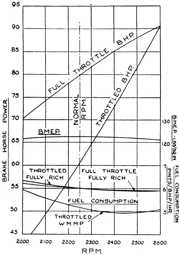
FIG. 28. Performance curves for the Gipsy Minor engine.
