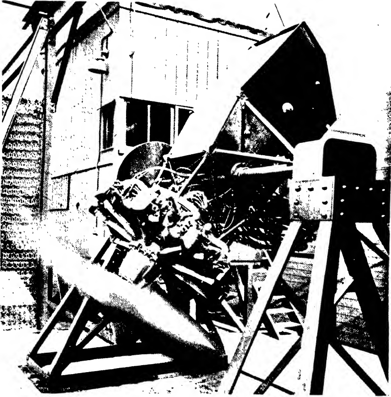
FIG. 351. The Bristol tilting test engine stand.
