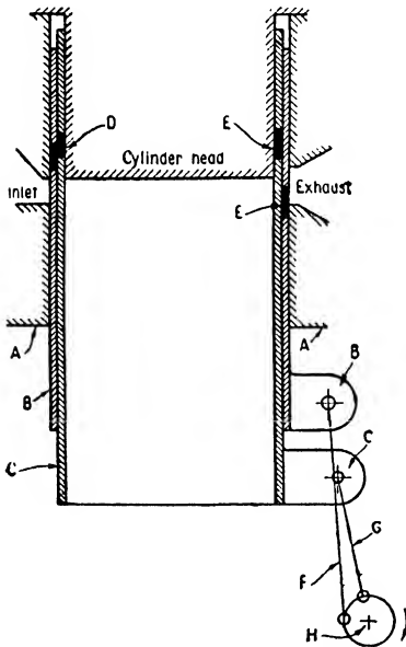
FIG. 109. Principle of the double-sleeve valve engine.
