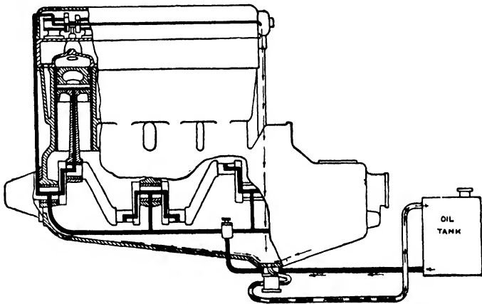
FIG. 246. The dry sump method of lubrication.
