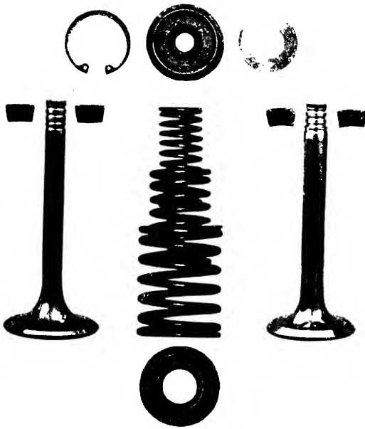
FIG. 219. The Bristol valves and their components.
