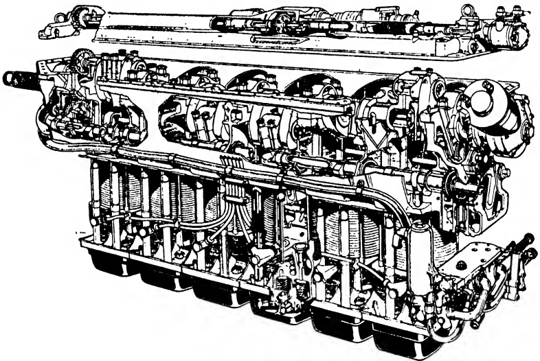
FIG. 40. The Gipsy Six Series II six-cylinder inverted air-cooled engine. (Courtesy "The Aeroplane.")
