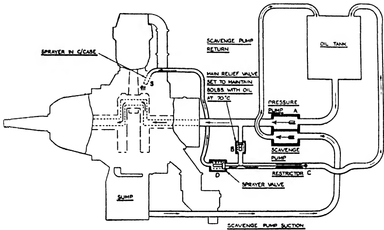
FIG. 264. The Bristol high initial oil pressure system.
