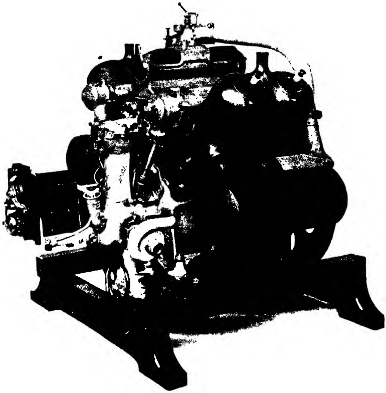
FIG. 137. The N.E.C. four-cylinder two-cycle aircraft engine. ( Courtesy The Science Museum, London. )
