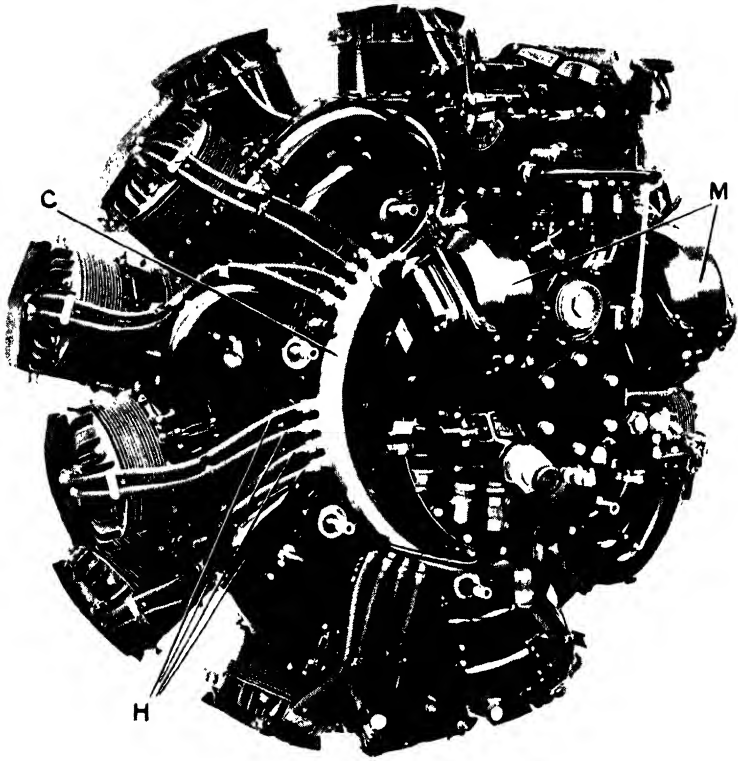
FIG. 310. The Bristol sleeve valve engine ignition harness. C—Ignition harness. H—Sparking plug screened cables. M—Dual magnetos.
