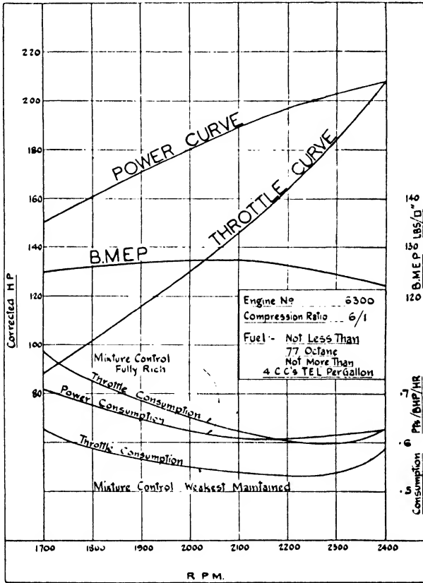
FIG. 41. Performance curves for the Gipsy Series II engine.
