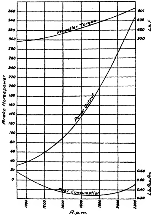
FIG. 162. Performance curves for Guiberson engine.
