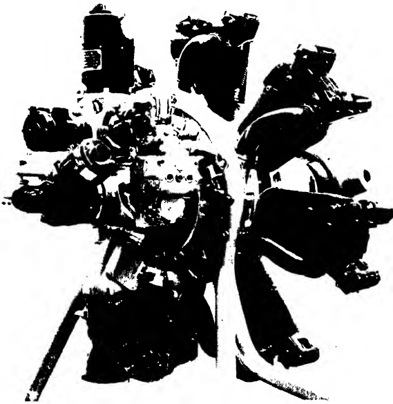
FIG. 80. The Armstrong Siddeley "Cheetah XI" (415 h.p.) engine, showing accessories and engine mounting.
