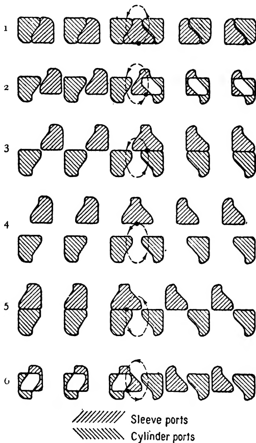
FIG. 113. Sequence of valve port openings and closing in five-port engine.
