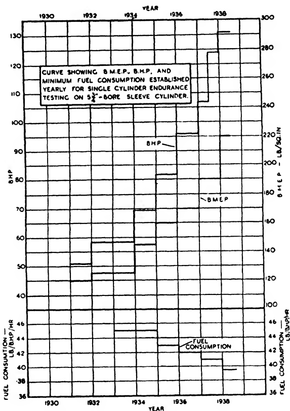
FIG. 115. Illustrating progress in the development of the Bristol sleeve-valve engine.
