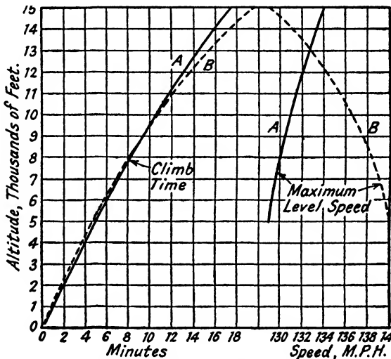
FIG. 156. Comparative flight trials. Bristol "Phoenix" and "Jupiter VIII" in "Wapiti" aircraft.
