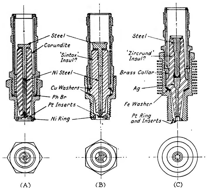
FIG. 299. Typical sparking plugs with sintered aluminum insulators. A—K.L.G., R-C.I; B—Lodge R.S.I; C—Sphinx Mk.I.Y.
