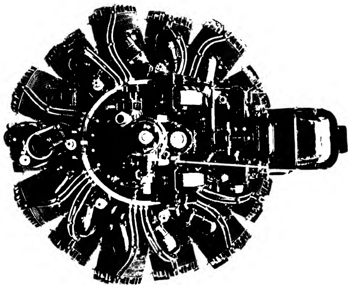
FIG. 132. The Bristol "Hercules" fourteen-cylinder twin row sleeve valve engine.
