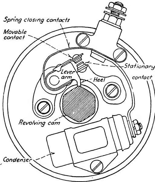
FIG. 278. Improved contact breaker unit.
