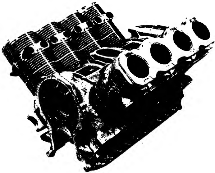
FIG. 191. Cylinder block and crankcase unit for aircraft engine cast in High Aluminium alloy. ( High Duty Alloys Ltd. )
