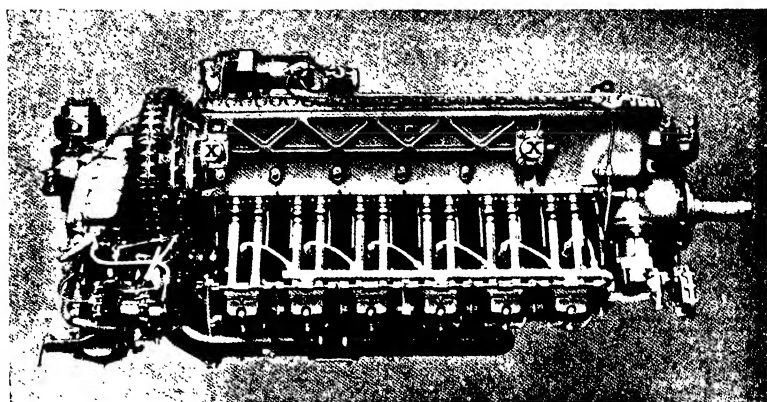
FIG. 236. The "Gipsy Twelve" engine showing trunnion mountings at X, X.
