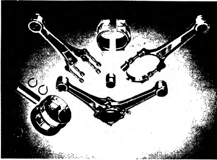
FIG. 202. The Rolls Royce "Merlin" engine connecting rods and piston.
