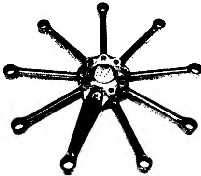
FIG. 203. Connecting-rod system of British "Mercury" and "Pegasus" engines.
