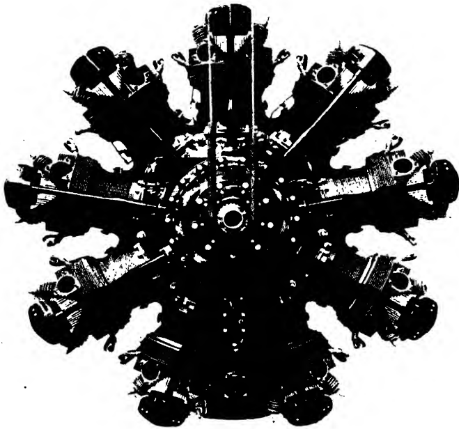
FIG. 86. The Bristol "Mercury" nine-cylinder air-cooled radial engine (840/890 h.p.).
