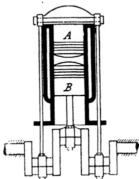
FIG. 21. Example of opposed piston balanced engine.
