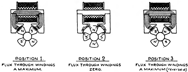
FIG. 281. Principle of polar inductor magneto.
