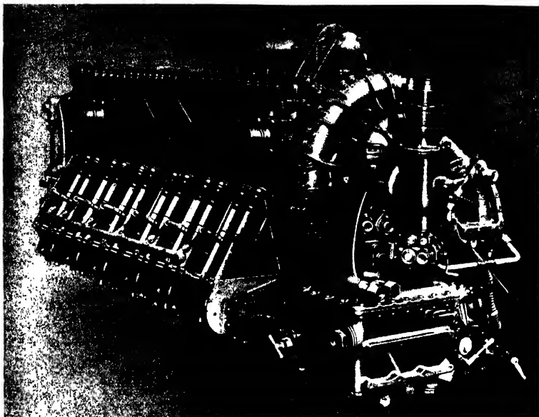
FIG. 53. Rear end view of "Gipsy Twelve" inverted twelve-cylinder Vee engine (400 h.p.).
