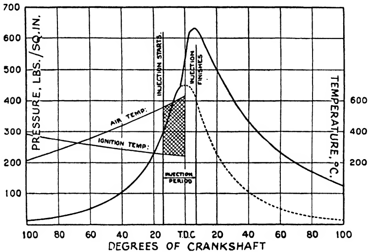
FIG. 139. Cylinder pressure, air and ignition temperature diagrams for C.I. engine.
