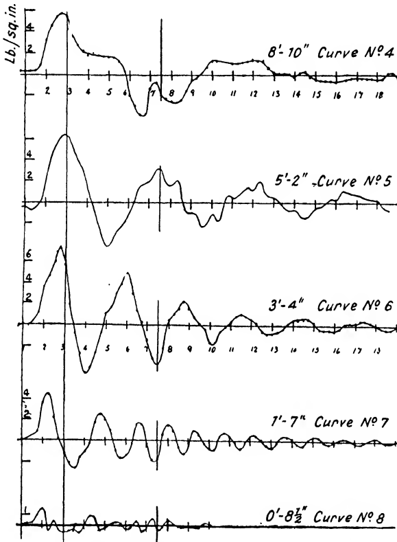
FIG. 312. Effect of exhaust pipe length on pressure valves.
