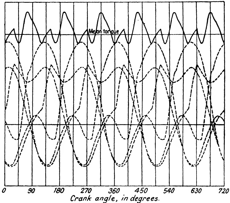
FIG. 14. Torque curves of 400 h.p. twelve-cylinder vee-type engine.
