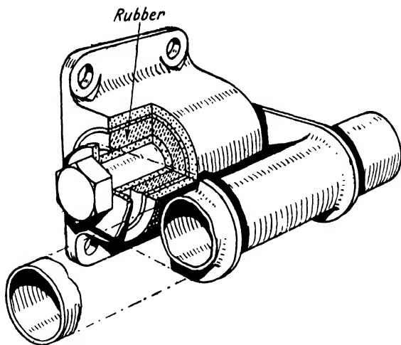
FIG. 244. Silentbloc rubber-type flexible aircraft engine mounting.
