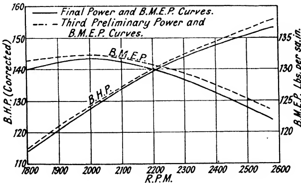
FIG. 36. Power curves for the Cirrus Major engine.
