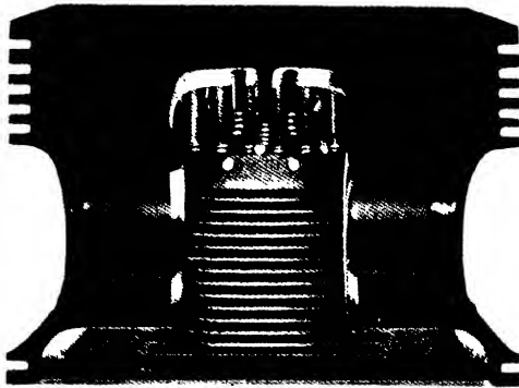
FIG. 198. Wright "Cyclone" engine piston, showing cooling studs.
