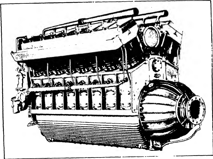
FIG. 104. The sixteen-cylinder 1,200-h.p. Mercedes-Benz compression ignition engine, used on the LZ129 Zeppelin airship.
