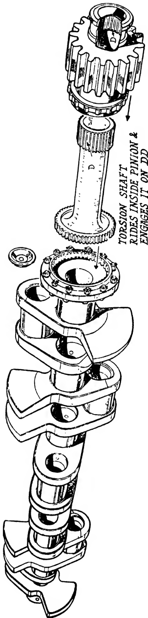
FIG. 208. Rolls Royce "Merlin" crankshaft showing torsion shaft drive for camshaft, supercharger and auxiliaries. ("The Aeroplane.")
