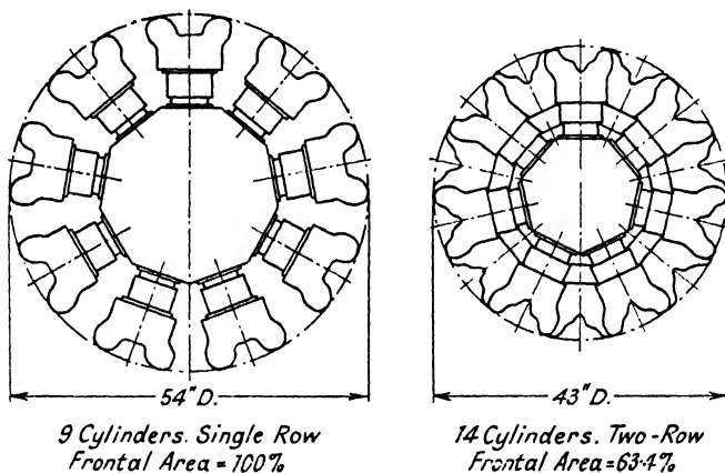
FIG. 1. Comparison of radial engines of equal power.
