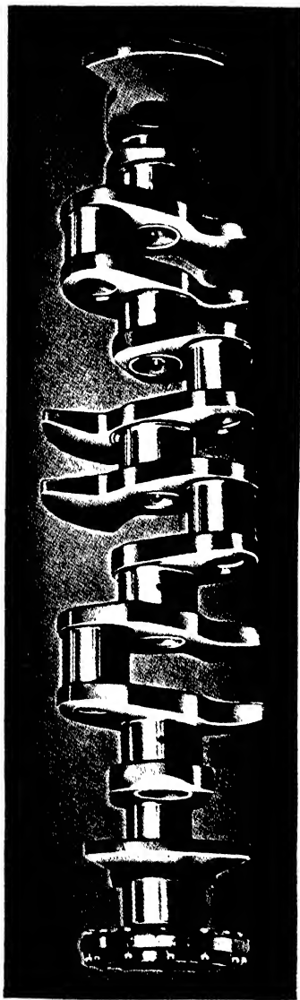
FIG. 207. The Rolls Royce "Merlin" engine six-throw crankshaft, showing balance weights, etc. [To face p. 254.]
