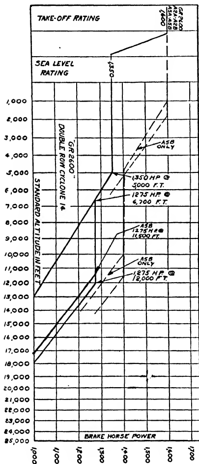
FIG. 107. Performance curves for the Wright Double Cyclone 14 engine.
