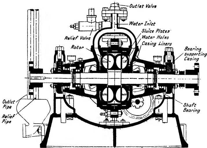
FIG. 351. Heenan and Froude hydraulic dynamometer.
