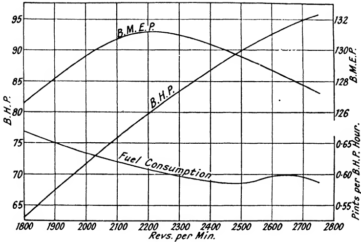
FIG. 35. Performance curves for the Cirrus Minor engine.
