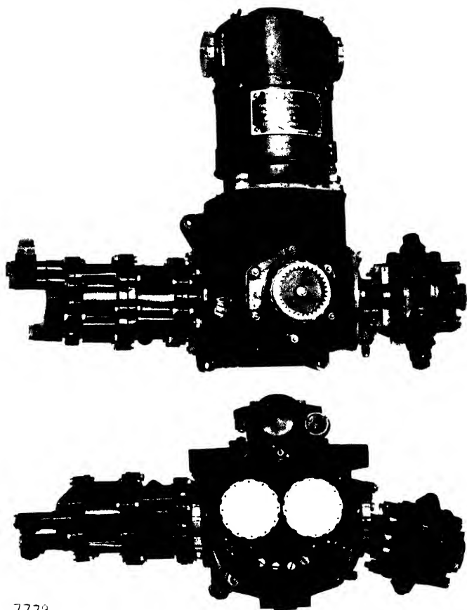
FIG. 331A. The Bristol auxiliary gear box.
