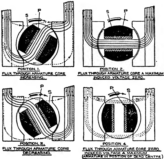
FIG. 274. Illustrating the flux changes in the rotating armature magneto.
