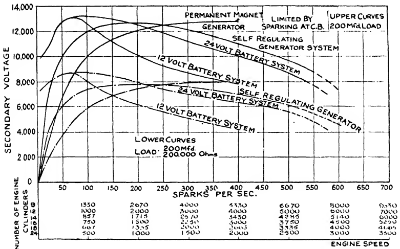
FIG. 295. Voltage-speed characteristics of coil ignition systems under various conditions of load.
