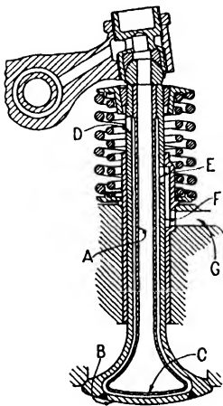
FIG. 216. Air- or liquid-cooling systems for exhaust valves.
