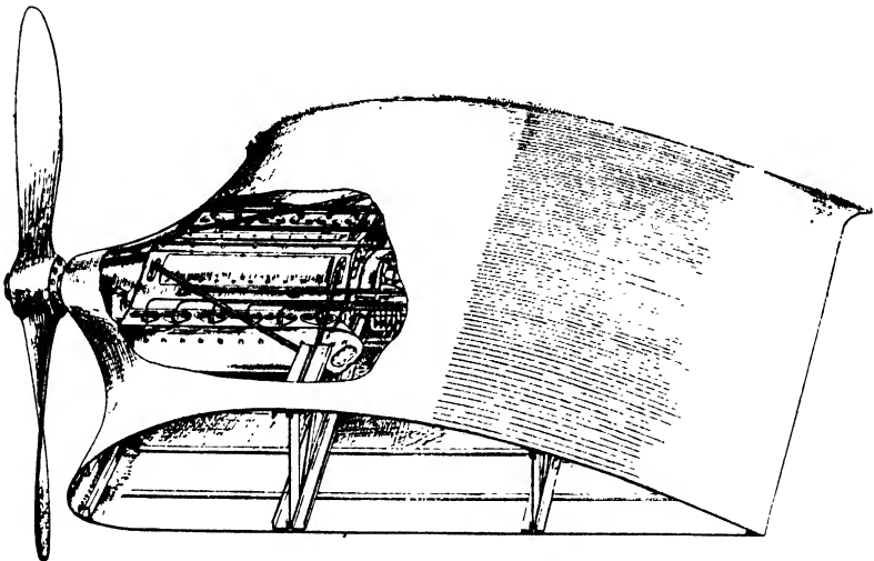
FIG. 43. Illustrating method of housing large opposed cylinder engine in wing of aircraft.
