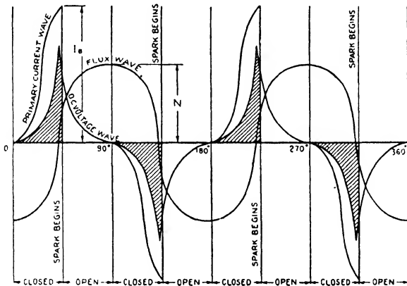
FIG. 282. Flux and voltage curves for polar inductor magneto.
