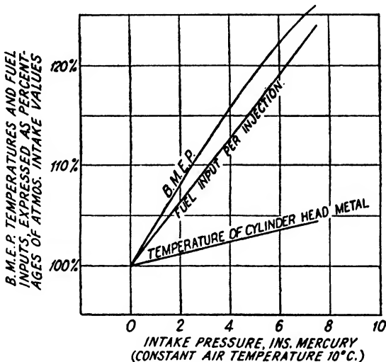
FIG. 148. Effect of supercharging C.I. engine upon B.M.E.P. and cylinder head temperature.
