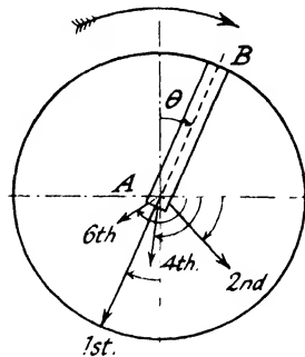
FIG. 20. Vector components of piston acceleration.
