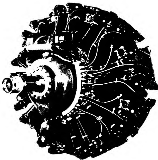
FIG. 108. Wright "Duplex-Cyclone," eighteen-cylinder two-row radial engine (2,000 h.p.).
