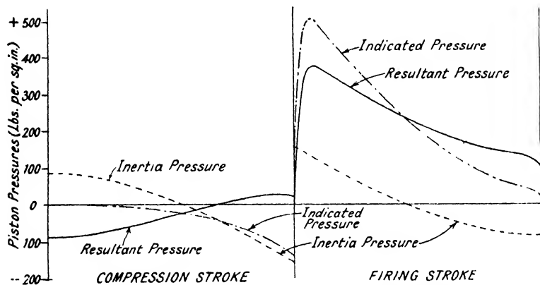
FIG. 10. Modification of gas pressures by inertia effects.
