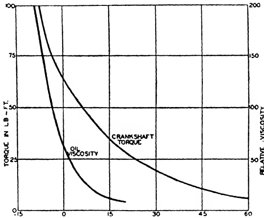
FIG. 344. Effect of temperature on the cranking torque and oil viscosity.
