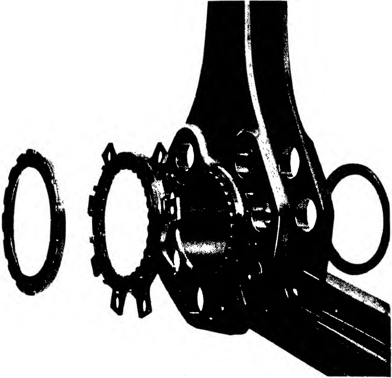
FIG. 205. Wright "Cyclone" master rod and link rod arrangement.
