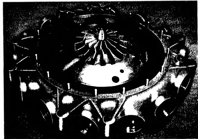
Fig. 96. Supercharger unit of Twin "Wasp" engine.
