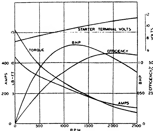
FIG. 346. Starting motor characteristics.
