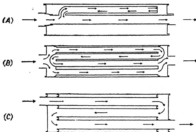
FIG. 324. Interference type silencers.
