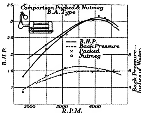
FIG. 321. Absorption silencer test results.
