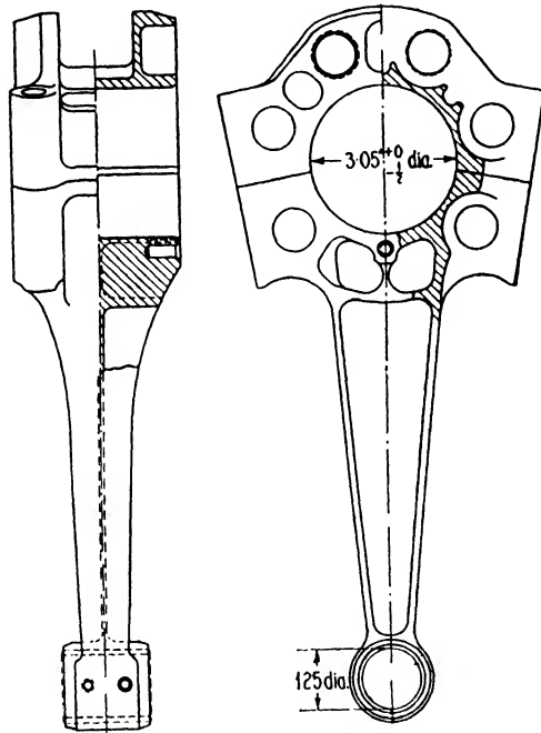
FIG. 204. Master rod for the Armstrong Siddeley "Cheetah" radial engine.
