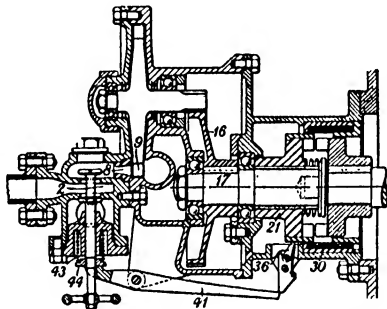
FIG. 338. Explosive cartridge engine starting scheme.
