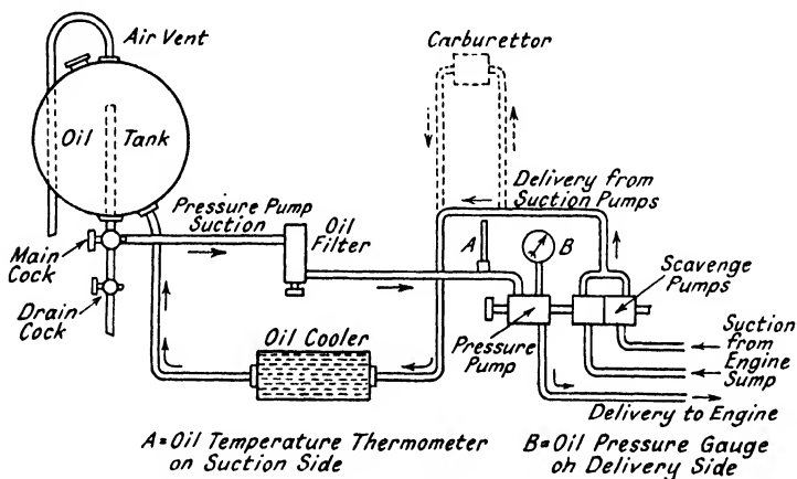
FIG. 247. Typical lay-out of aircraft engine dry sump lubrication system.
