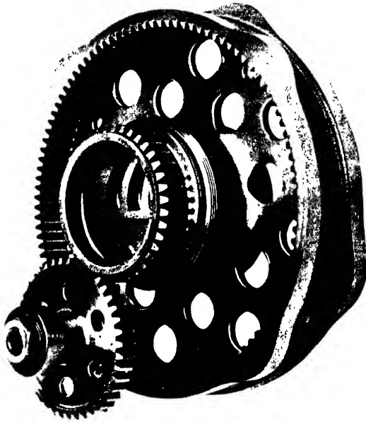
FIG. 230. Bristol "Mercury" engine cam rings and gear drive.
