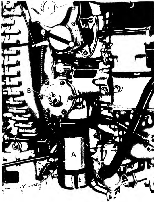
FIG. 317. Rolls Royce "Merlin" engine starting unit.
