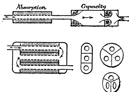
FIG. 317. (Above) Absorption and capacity type silencer. (Below) Examples of absorption silencers.
