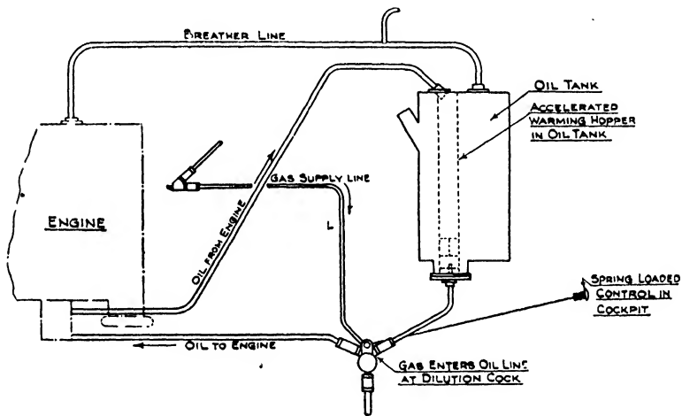
FIG 265. Oil dilution by fuel for starting purposes.
