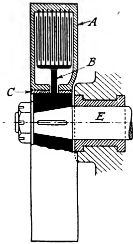
FIG. 15. Torsional vibration damper.
