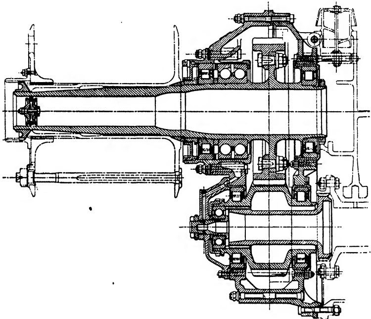
FIG. 233. Airscrew reduction gear unit, showing gears and bearings, etc.
