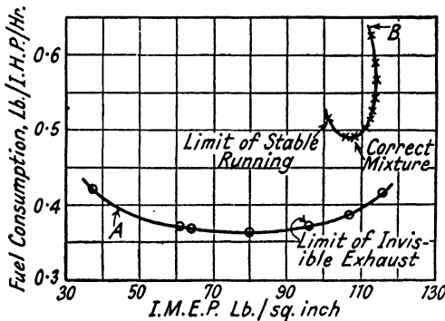
FIG. 142. Fuel consumption ranges of C.I. and petrol engines.
