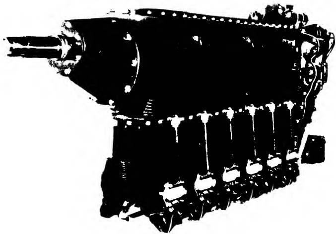
FIG. 42. The Menasco inverted six-cylinder air-cooled engine.
