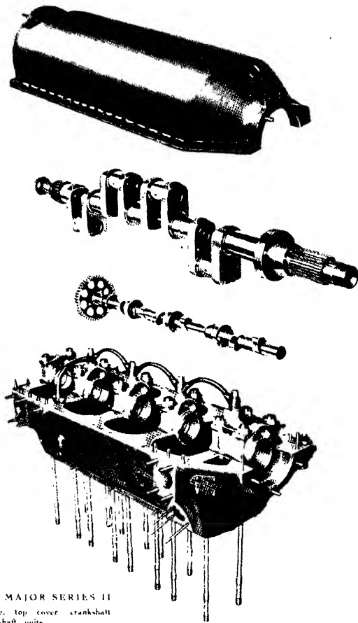
FIG. 192. Crankcase, top cover, crankshaft, and camshaft of "Gipsy Major" engine (inverted four-cylinder type).
