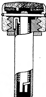
FIG. 223. Automatic valve-stem clearance adjuster.
