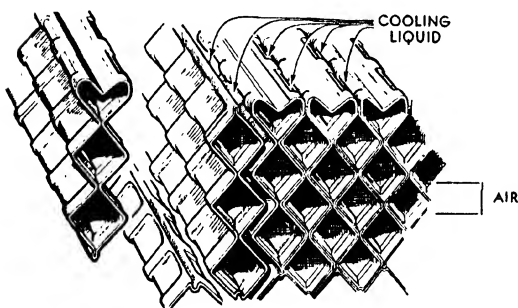
FIG. 261. Illustrating method of construction of Galley radiator for liquid-cooled engines and oil coolers.
