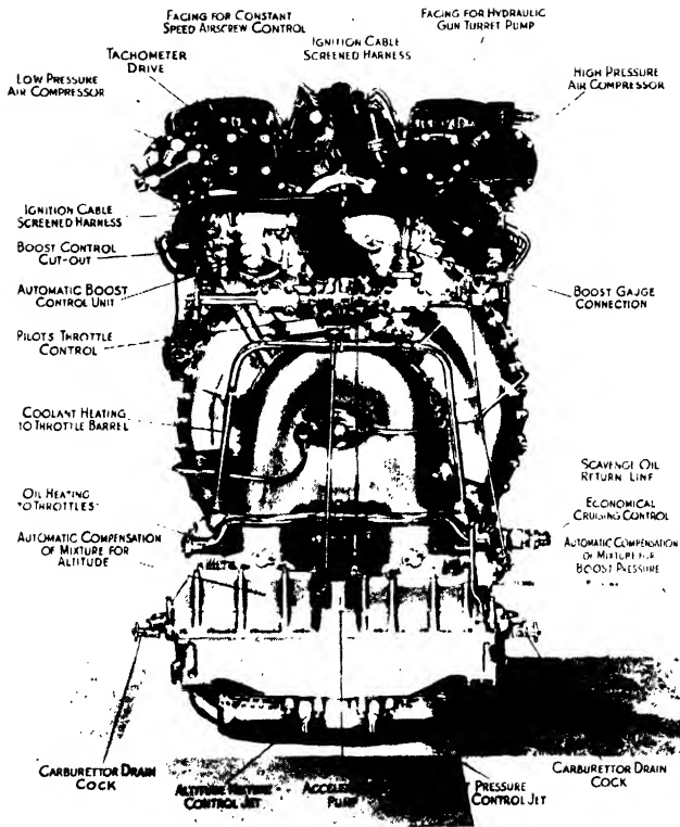
Fig. 68. Rear end view of Rolls Royce "Merlin" engine showing principal components.
