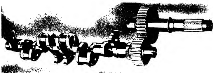
FIG. 210. Crankshaft and airscrew drive of the "Gipsy Twelve" inverted Vee-type engine.
