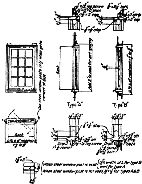
FIG. 158.—Pivoted window.
