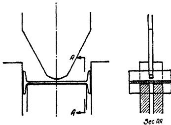
FIG. 2.—Beam shearing.
