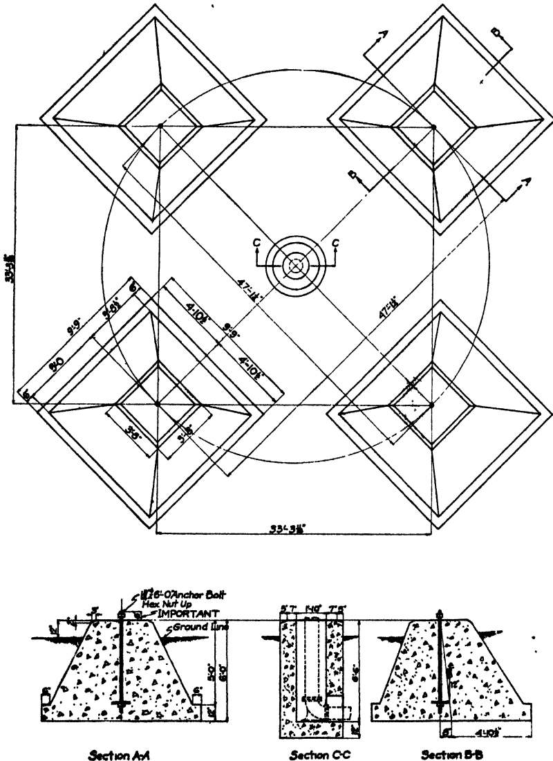
FIG. 13.—Foundation for 100,000-gal. tank, 100 ft.—0 in. to bottom, concrete mixture 1:3:5.
