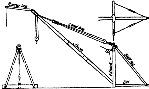
FIG. 9.—Six-ton steel ginnywink.
