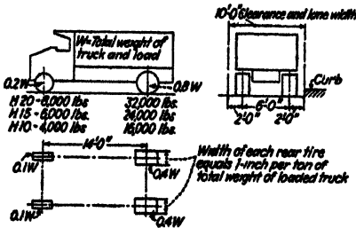
FIG. 65.—Standard H truck loadings.
