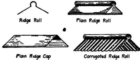
FIG. 115.—Ridge roll.
