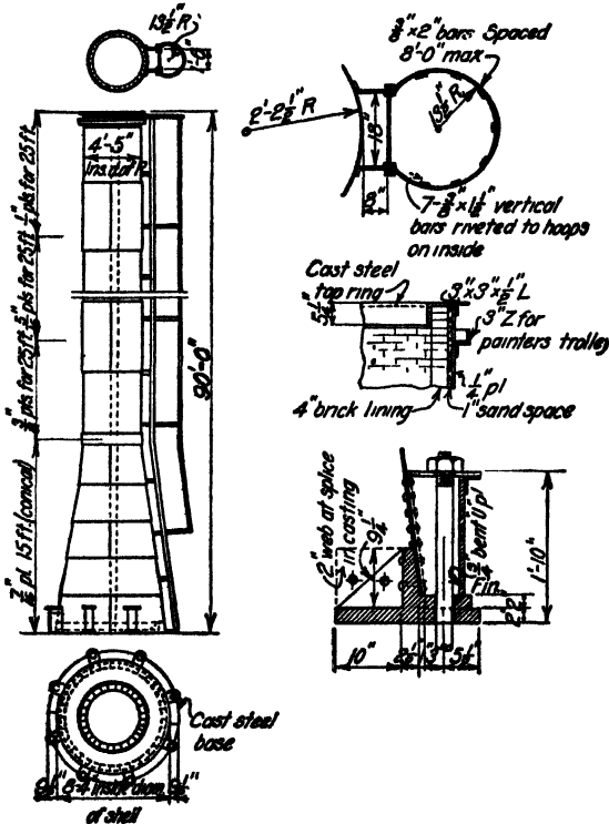
FIG. 112.—Self-supporting stack.
