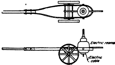
FIG. 35.—Reaming buggy.
