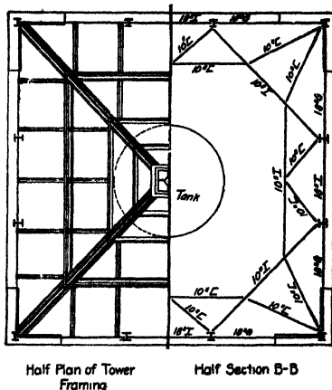
FIG. 80. - Half plan and section of tower.
