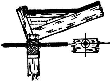
FIG. 188.—Detail of saw-tooth frame— inclined face with pipe ties.
