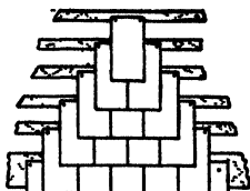
FIG. 148.—Slate on wood purlins.
