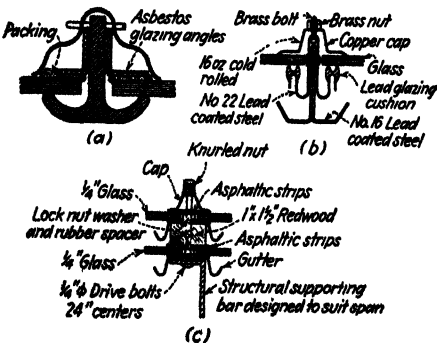
FIG. 167.—Types of skylight bars.
