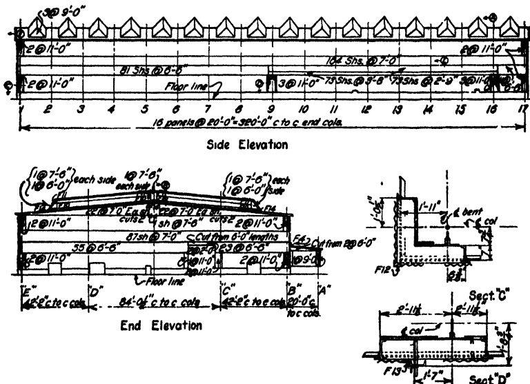
FIG. 122.—Corrugated steel plans for a machine shop (American Bridge Co.).
