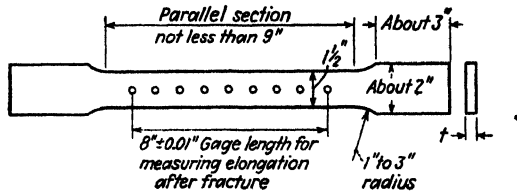
FIG. 1. Standard 8-in. gage length test specimen.
