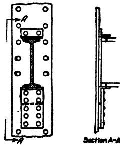
FIG. 39.—Connection with stiffening plate.
