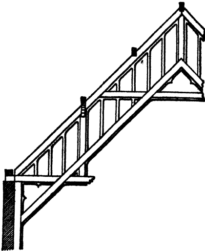
FIG 101 —Laminated truss.
