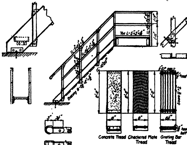
FIG. 110.—Stairs with angle hand rail.
