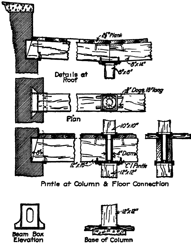
Fig. 198.—Some special details used in framing mill construction.
