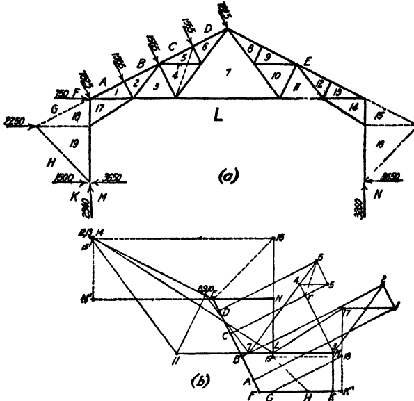
FIG. 65.—Knee-braced trusses.
