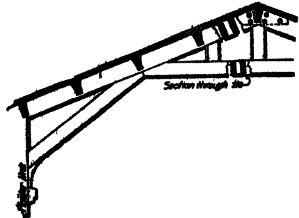
FIG. 105.—Braced rafter.
