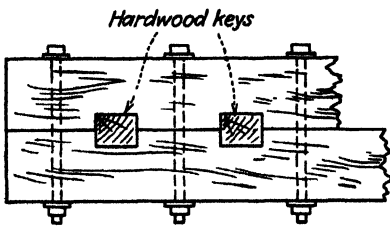
FIG. 23.—Built-up beam with keys.
