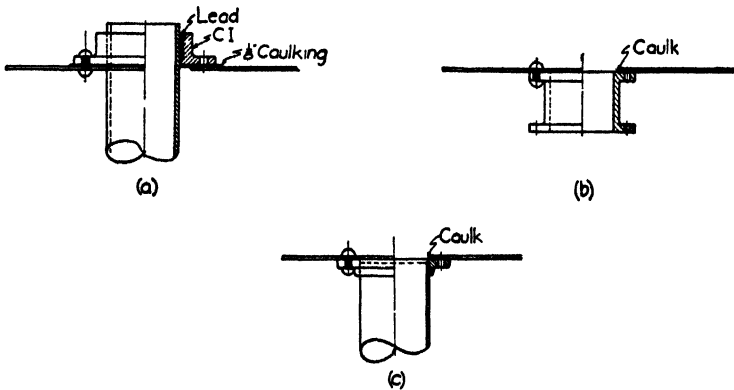
FIG. 6.—Connections to bottom of tank.
