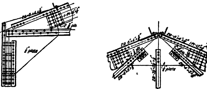
FIG. 105.—Roof truss details.
