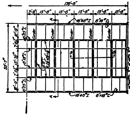
FIG. 77.—Court skylight framing.
