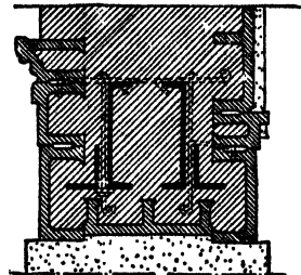
FIG. 68.—Section over entrance showing method of supporting terra cotta.
