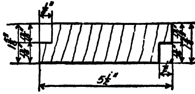
FIG. 182.—Section of 2 × 6-in. shiplap.
