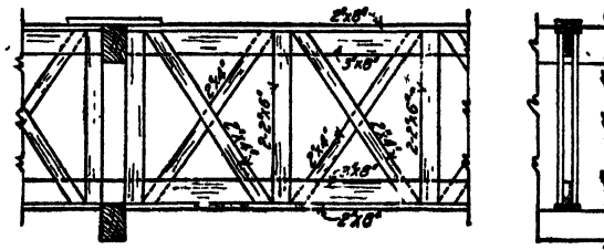
FIG. 183.—Detail of typical roof bracing truss.
