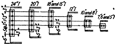
FIG. 28.—Framing of various-size beams.
