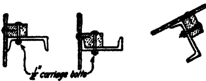
FIG. 119.—Wood nailers.
