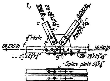
Joint g FIG. 53
