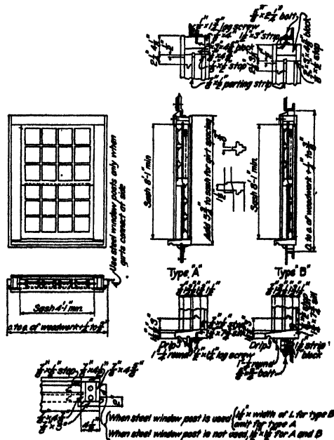
FIG. 163.—Double hung weighted window.
