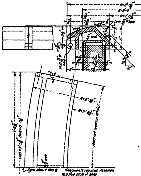
FIG. 9.—Cast-iron top cap details.
