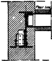
FIG. 65.—Spandrel section for solid wall.
