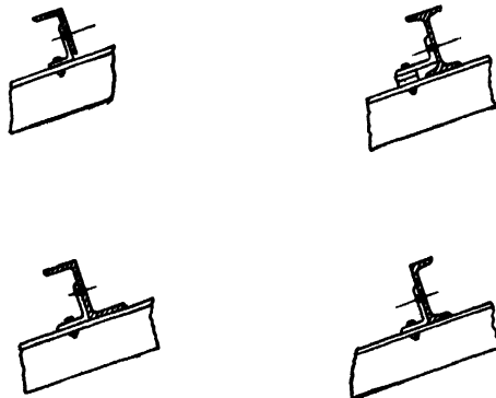
FIG. 108.—Purlins.
