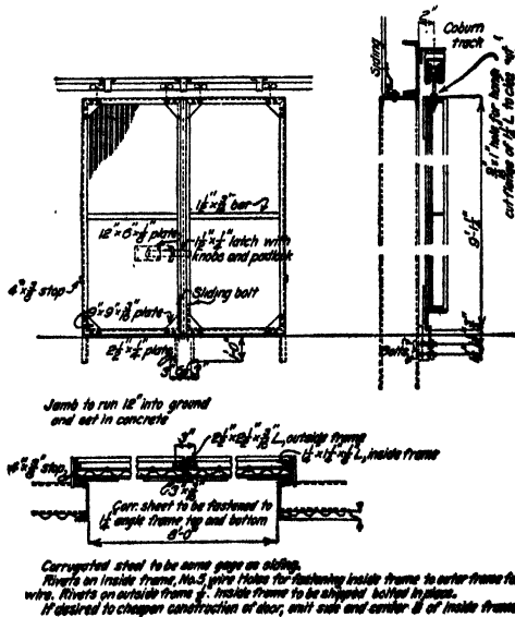
FIG. 155.—Steel sliding door.
