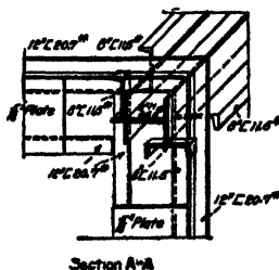
Section A-A FIG. 81.—Section of tower column.
