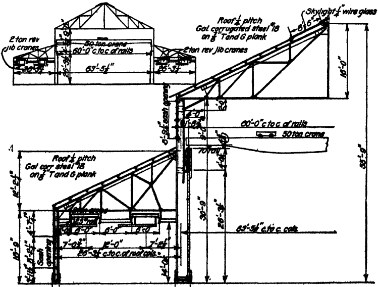
FIG. 94.—Machine shop. Cross-section.
