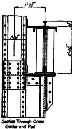
FIG. 101.—Section through crane girder and rail.
