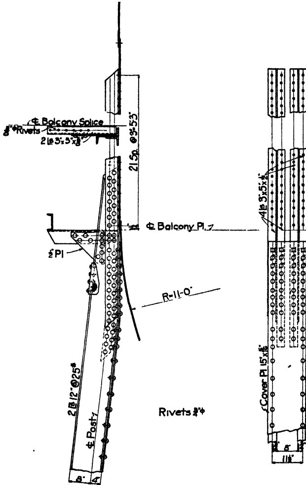
FIG. 8.—Post to tank connection for 100,000-gal. tank.
