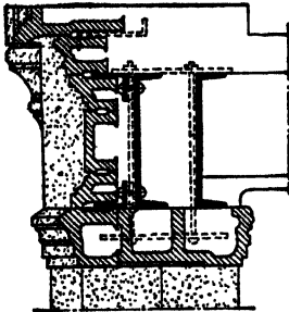
FIG. 67.—Spandrel section showing method of supporting terra cotta.
