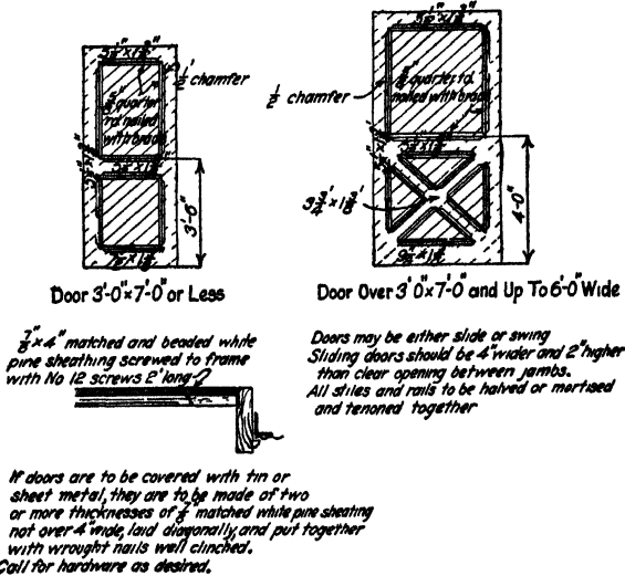
FIG. 152.—Wooden doors under 6 ft. wide.
