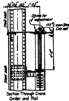
FIG. 102.—Section through crane girder and rail.
