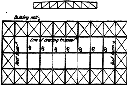
FIG. 185.—Diagrammatic plan of typical roof bracing.
