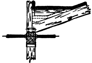
FIG. 189.—Detail of saw-tooth frame— vertical face with pipe ties.
