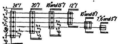
FIG. 29.—Framing of various-size beams.
