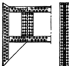
FIG. 62.—Wind-bracing girder.
