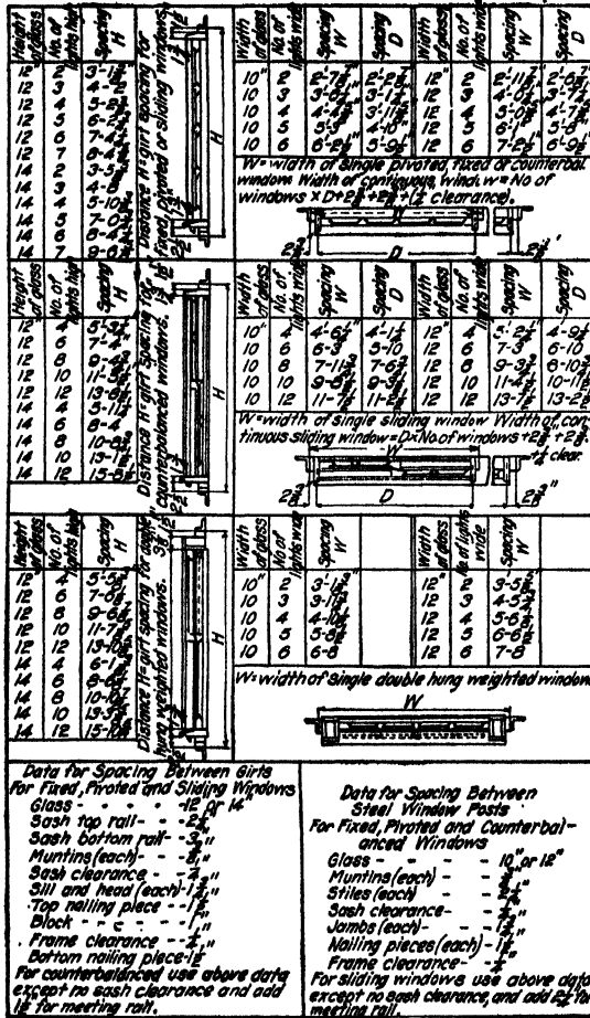
FIG. 165.—Dimensions for wood frames.
