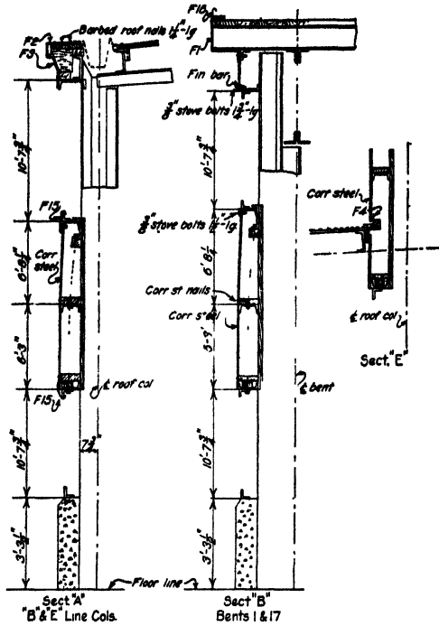
FIG. 123.—Corrugated steel details for machine shop shown in Fig. 122.
