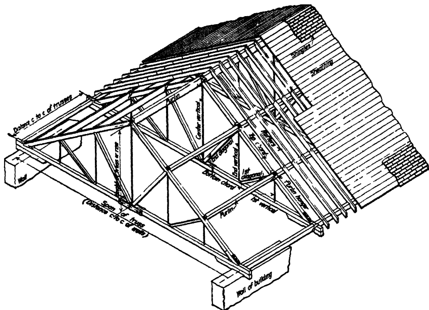
FIG. 22.—Detailed design of a wooden roof truss.
