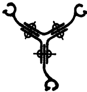
FIG. 14.—Standard fabricated Y steel sheet piling.
