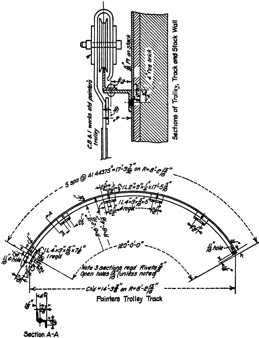
FIG. 10.—Details of painter's trolley and track.
