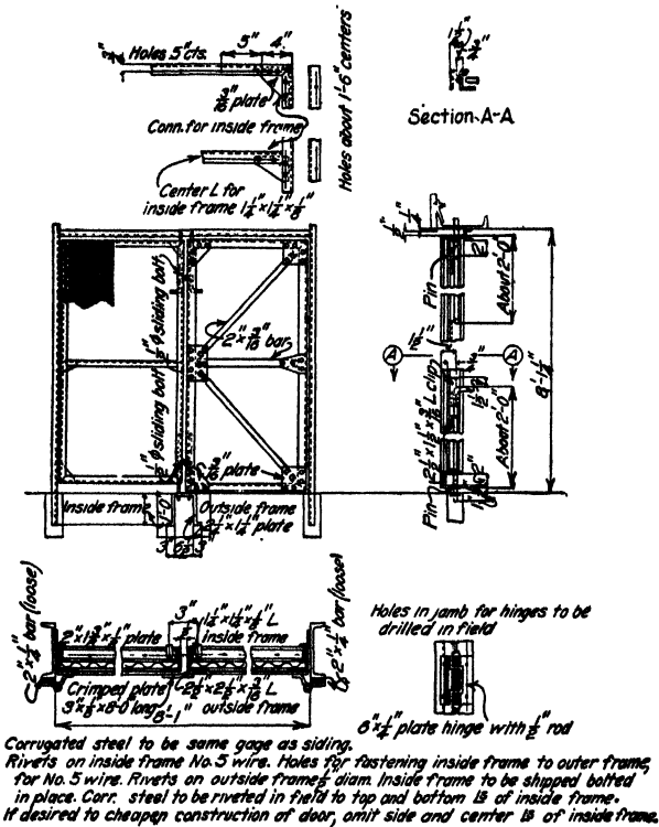
FIG. 156.—Steel swinging door.
