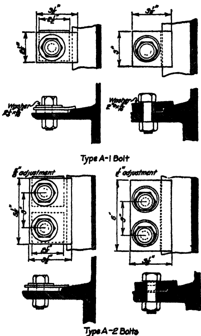
FIG. 106.—Rail clips.
