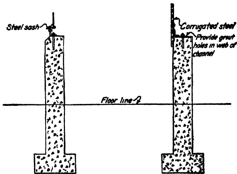
FIG. 134.—Curtain walls.
