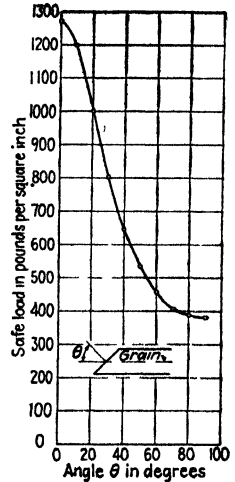
FIG. 6. --Inclined bearing on Douglas fir.
