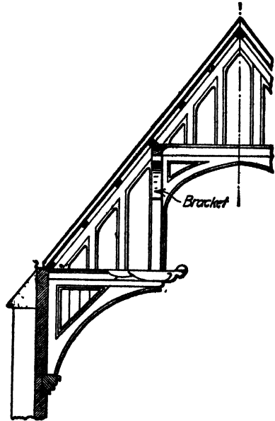
FIG. 100—Hammer beam with A-truss
