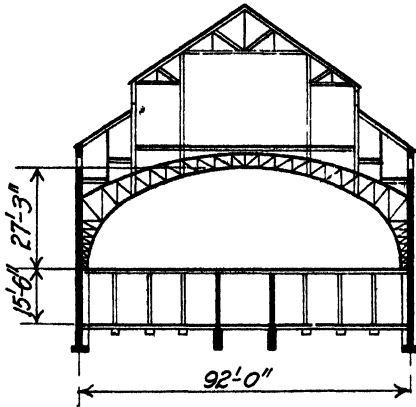
FIG. 77.—Section of gymnasium and armory, University of Wisconsin.
