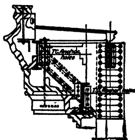
FIG. 72.—Cornice supported by brackets.
