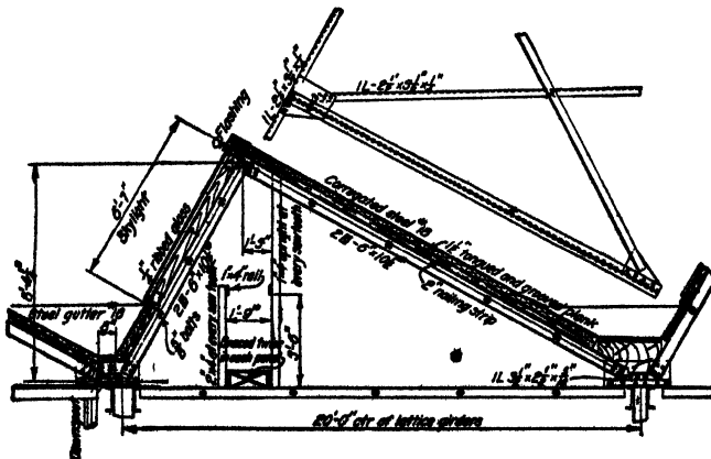
FIG. 98.—Section through saw-tooth skylight.
