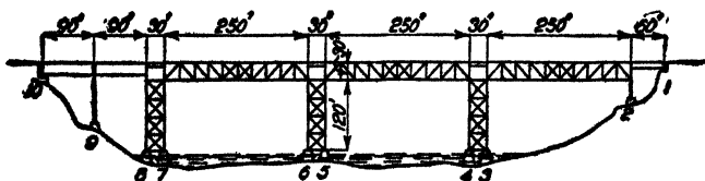
FIG. 37.—Bridge erected by cantilever method.
