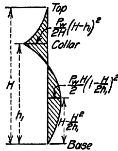
FIG. 3.—Moment diagram for a guyed steel stack with one set of guys
