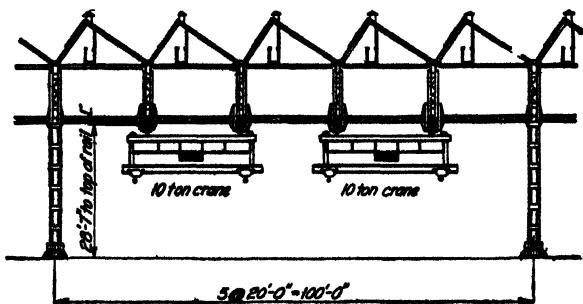
FIG. 96.—Structural steel fabricating shop. Longitudinal section through punching and assembling departments.
