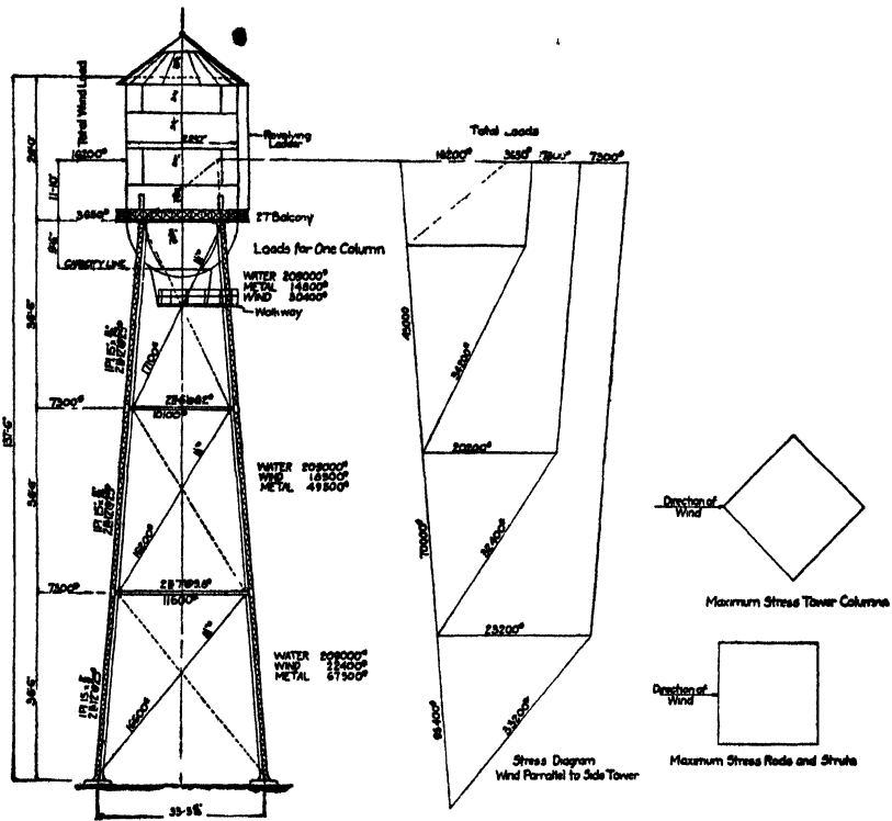
FIG. 14.—100,000-gal. tank 100 ft.—0 in. to bottom.
