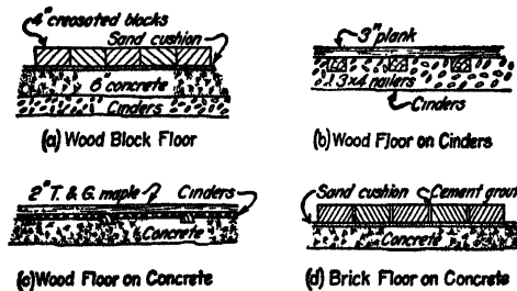
FIG. 150.—Ground floors.
