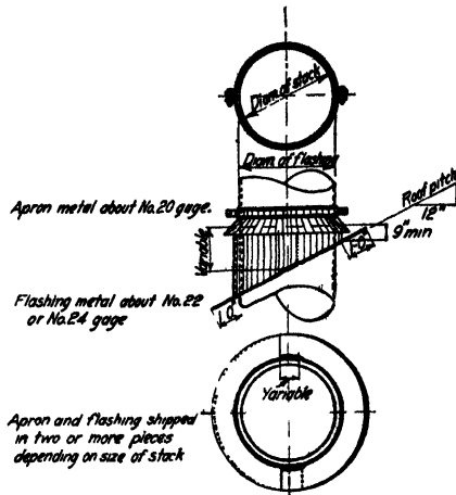
FIG. 133.—Stack flashing.
