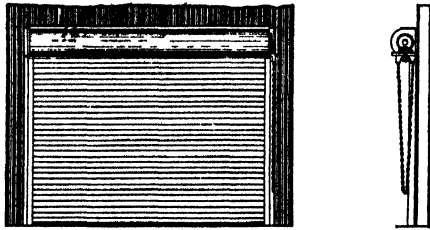
FIG. 157.—Kinnear steel rolling door.
