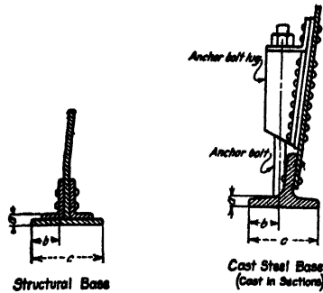
FIG. 6.—Base plates for self-supporting steel chimneys.
