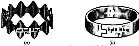
FIG. 12.—(a) Toothed ring. (b) Split ring.
