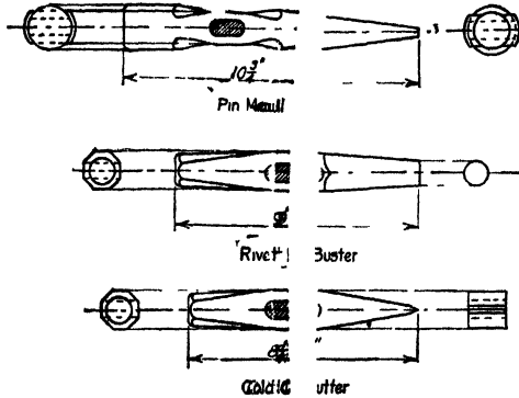
FIG. 30.—Hand tools for cutting out rivets.
