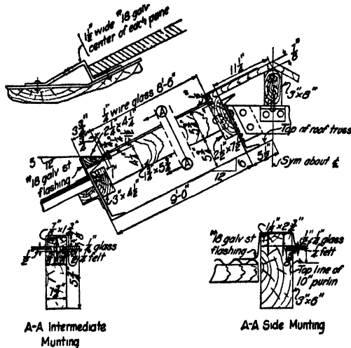
FIG. 168.—Wooden skylight frame.
