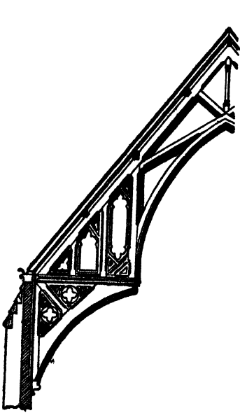
FIG. 99—Hammer beam with scissors truss above.
