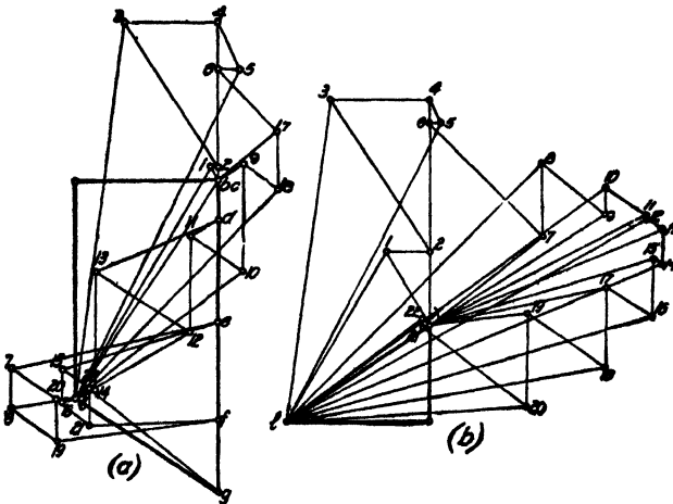
FIG. 93.—Snow load stress diagram.
