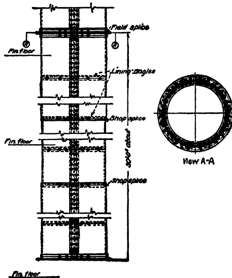
FIG. 82.—Self-supporting stack.
