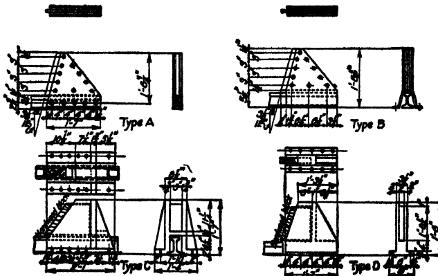
FIG. 107.—Crane stops.
