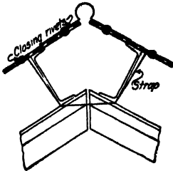
FIG. 125.—Section through ridge roll.
