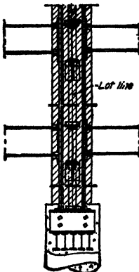
FIG. 54.—Simple party wall.
