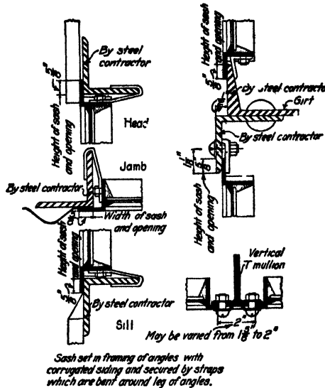
FIG. 166.—Steel sash details.
