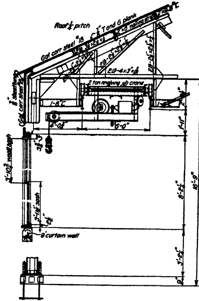
FIG. 93.—Machine shop lean-to. Showing revolving jib crane.
