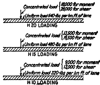
FIG. 66.—H lane loadings.
