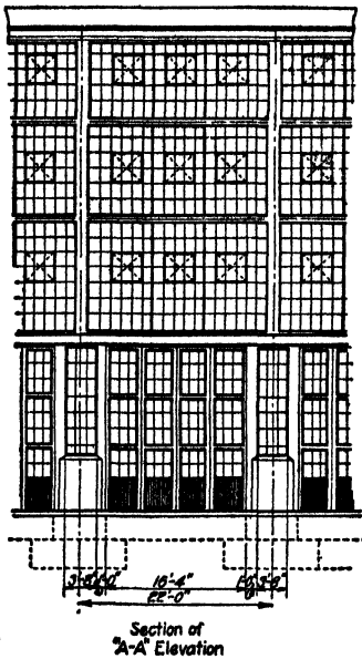
FIG. 87.—Locomotive boiler shop. Outside elevation showing windows and doors in side wall.
