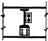
FIG. 31.—Framing into deep beams.
