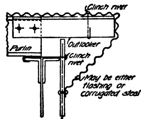
FIG. 130.—Gable finish with outlooker.
