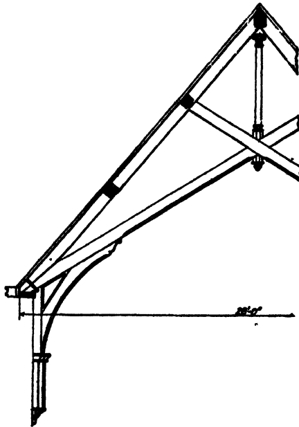
FIG. 106.—Scissors truss.
