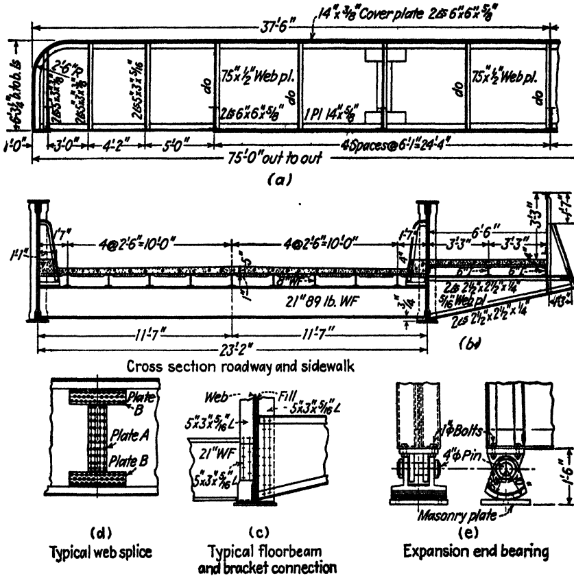
FIG. 67.—General drawing, 75-ft. plate girder highway bridge.
