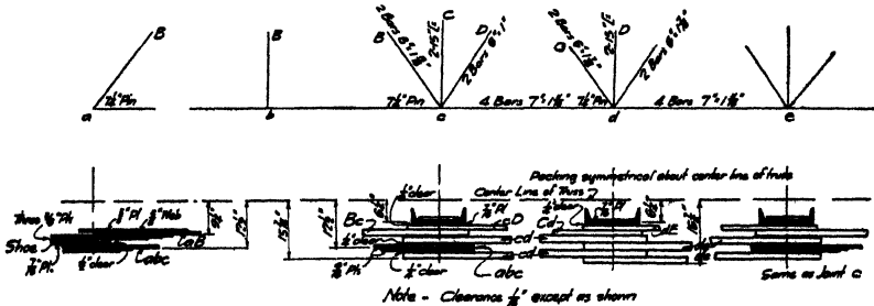
FIG. 59.—Lower chord packing.
