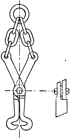
FIG. 14.—I-beam hook for I-beams 15 in. deep and over.
