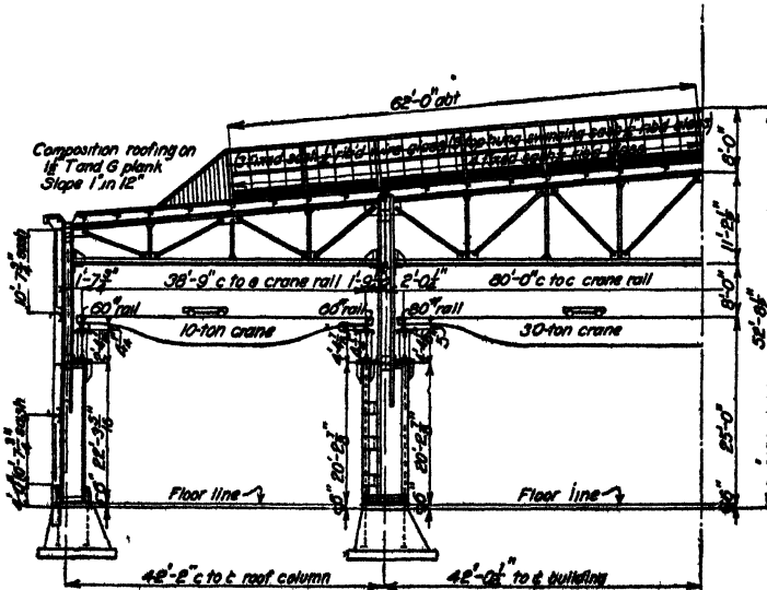
FIG. 91.—Machine shop. Cross-section showing capacity and elevation of cranes.
