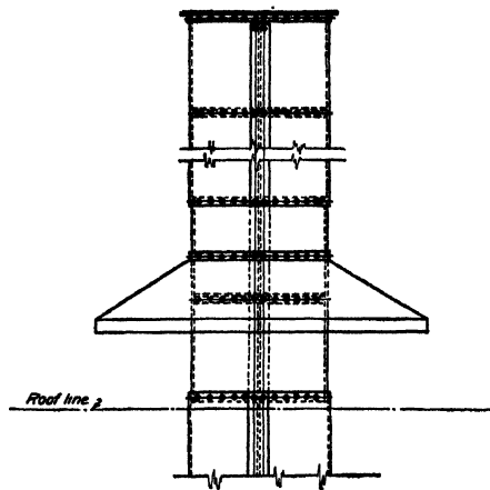
FIG. 84.—Stack hood at roof level.
