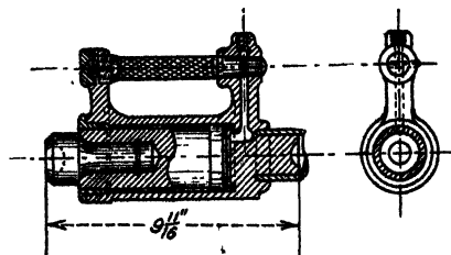
FIG. 30.—Pneumatic buckler-up.
