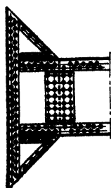
FIG. 63.—Wind-bracing girder.
