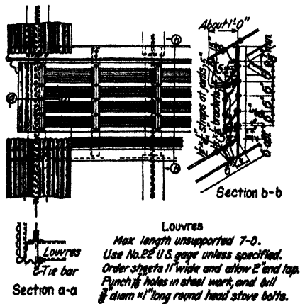
FIG. 135.—Louvre ventilators.
