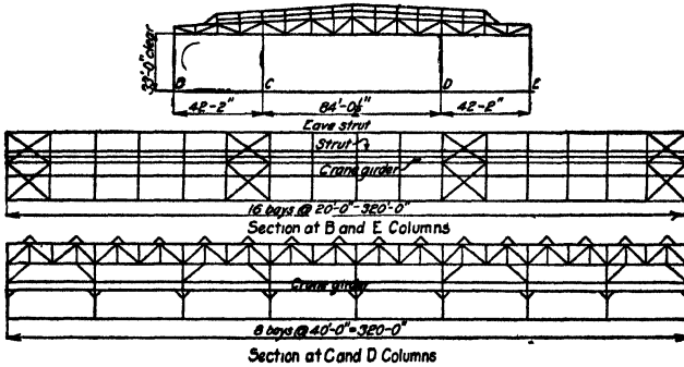
FIG. 90.—Longitudinal and transverse sections through machine shop shown in Fig. 91.
