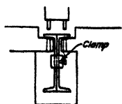
Fig. 11.—Flange punching channels in pairs.
