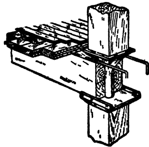
FIG. 196.—Detail of column and girder construction with cast-iron pintle.
