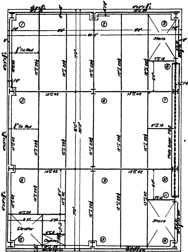
Fourth Floor Framing Plan Scale \frac{1}{4} "=1'0"
