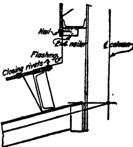
FIG. 131.—Finish of lean-to to main building.
