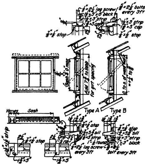
FIG. 159.—Continuous pivoted and fixed sash in monitors.
