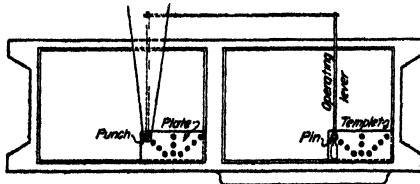
FIG. 7.—Weatherson spacer.
