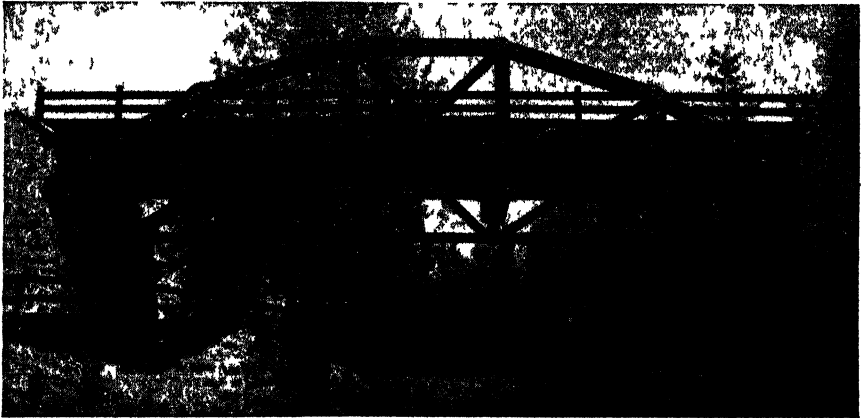
FIG. 35—Ring-connected timber bridge over Johnson Creek near Portland, Ore. Span is 60 ft. 0 in., roadway width 20 ft. 0 in., designed for the H-15 loading (Courtesy of Timber Engineering Co.).
