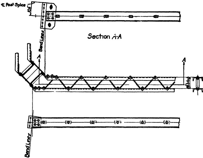
FIG. 12.—Typical strut.
