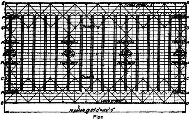
FIG. 89.—Machine shop Plan of skylights and roof bracing.
