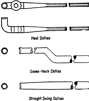
FIG. 26.—Dolly bars.
