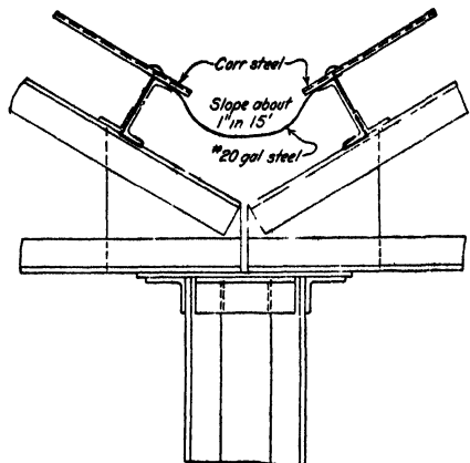
Fig. 143.—Valley gutter.
