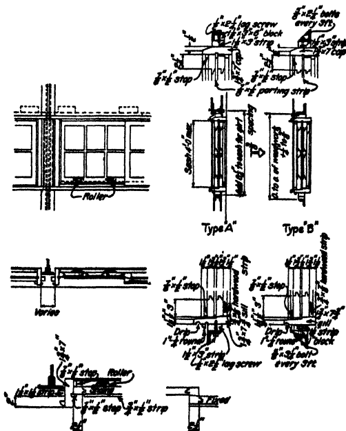
FIG. 161.—Continuous sliding sash.
