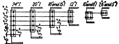
FIG. 30.—Framing of various-size beams.
