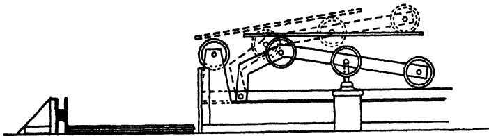
FIG. 23.—Kickoff for plates.
