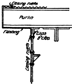
FIG. 129.—Gable finish.
