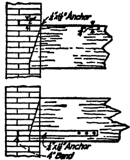
FIG. 170.—Details of connection—timber joists to brick walls.
