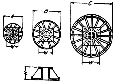
FIG. 10.—Cast-iron column bases.
