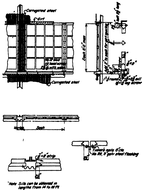
FIG. 160.—Continuous fixed sash.
