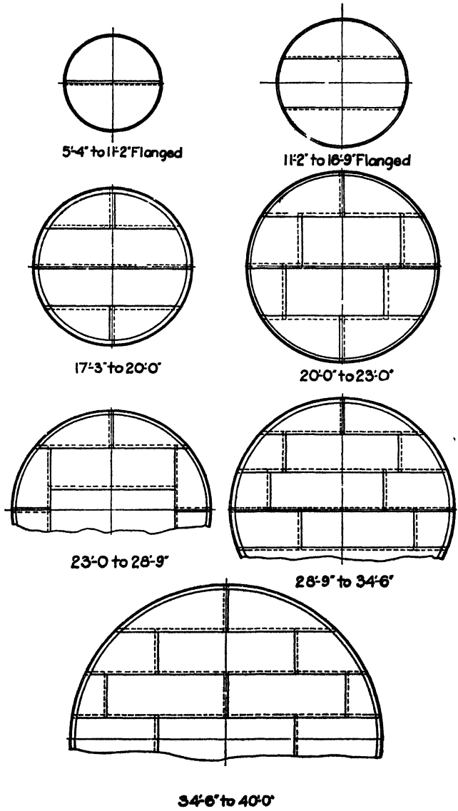
FIG. 3.—Arrangement of bottom plates for various diameter tanks.
