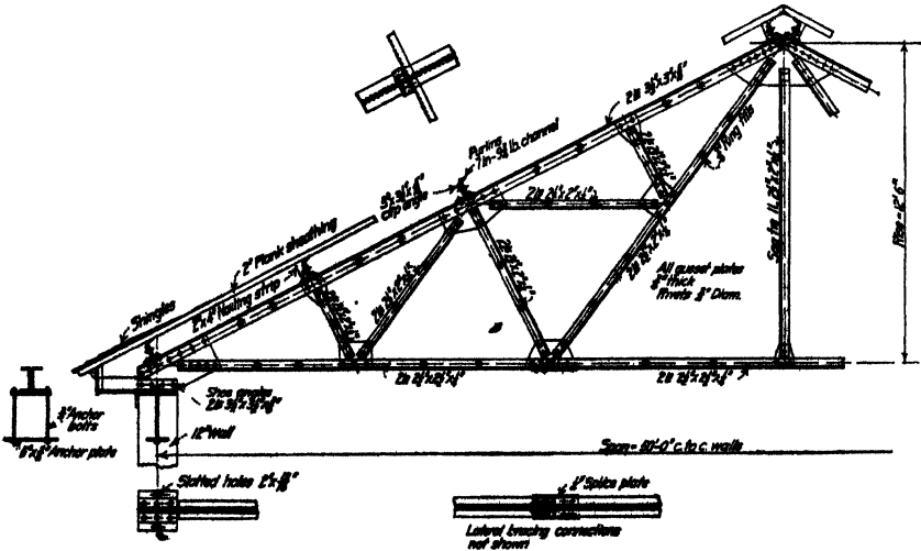
FIG. 58.—General drawing of 50-ft. steel roof truss.
