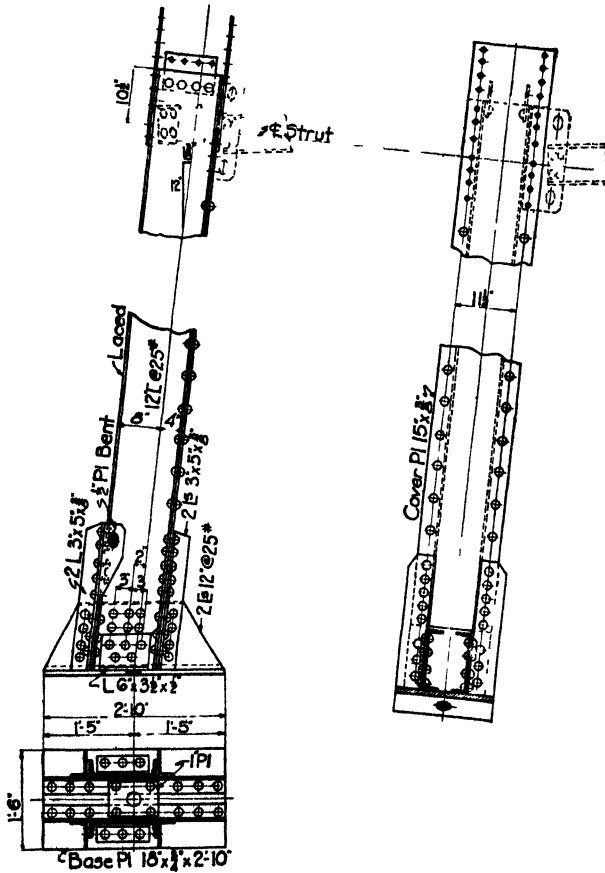
FIG. 11.—Lower tower post for 100,000-gal. tank.
