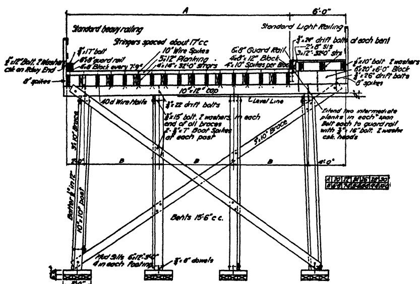
FIG. 31.—Typical section of roadway timber trestle, City of Seattle.
