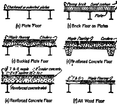
FIG. 151.—Floors above ground.
