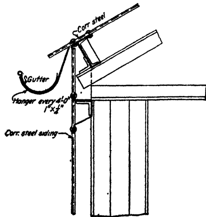
FIG. 139.—Hanging gutter.
