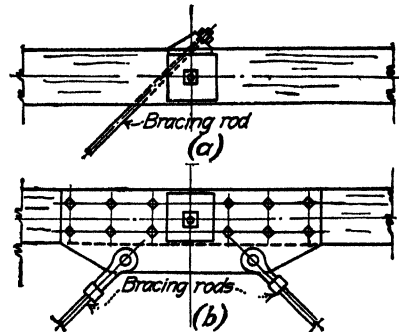
FIG. 186.—Typical details of connection of bracing rods to upper chord of roof truss.
