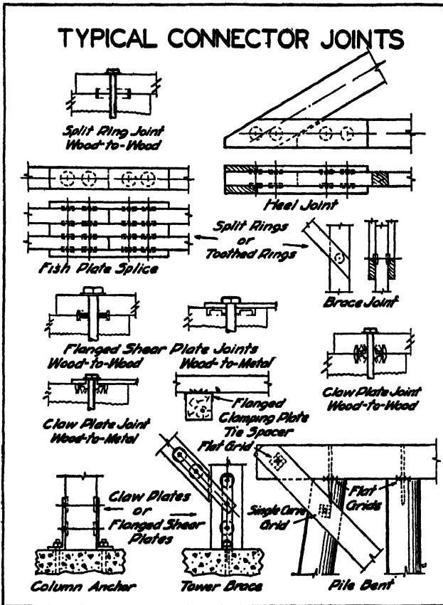
FIG. 17.—Connector joints.
