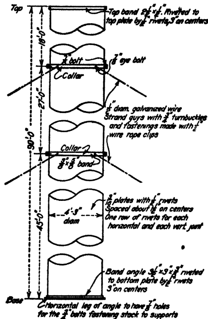
FIG. 4.—Ninety-foot guyed steel chimney.
