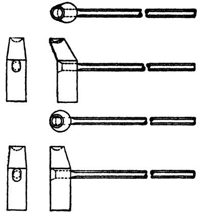
FIG. 27.—Spring dollies.
