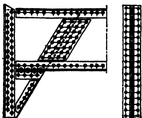
FIG. 61.—Wind-bracing girder.
