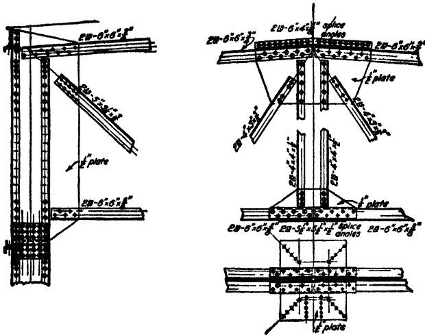
FIG. 103.—Roof truss details
