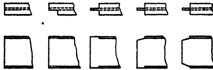
FIG. 19.—Coping I-beam.
