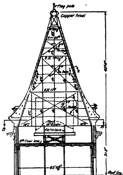
FIG. 79.—Section through tower.
