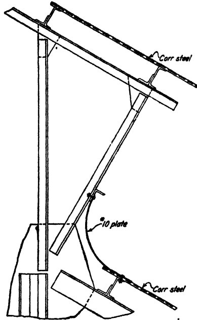
FIG. 137.—Open side monitor for open hearth building.
