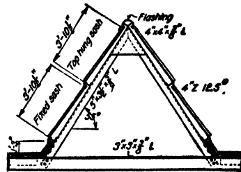
FIG. 88.—Section through skylight.
