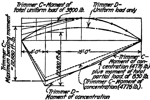
FIG. 180.—Diagram of bending moments for Trimmers C and D.
