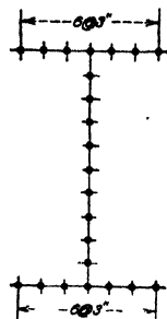
Fig. 10.—Tandem punching.
