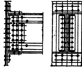
FIG. 58.—Wind-bracing girder.
