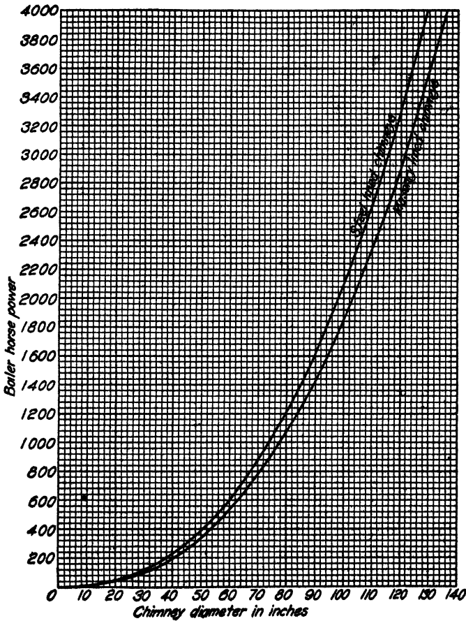
FIG. 1A.—Curves showing relation between chimney diameters and boiler horsepower served.
