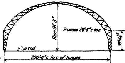
FIG. 78.—Drill hall, University of Illinois.
