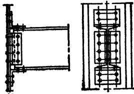
FIG. 57.—Wind-bracing girder.
