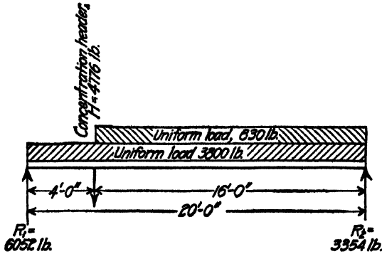
FIG. 179.—Diagram of loads on Trimmer C.
