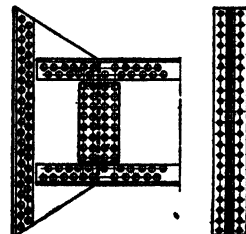
FIG. 60.—Wind-bracing girder.
