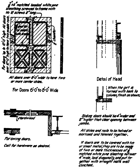
FIG. 153.—Wooden doors 6 ft. wide and over.
