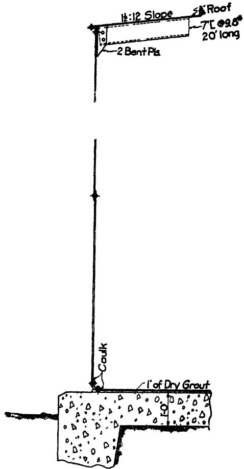
FIG 7.—Part section of tank and foundation.
