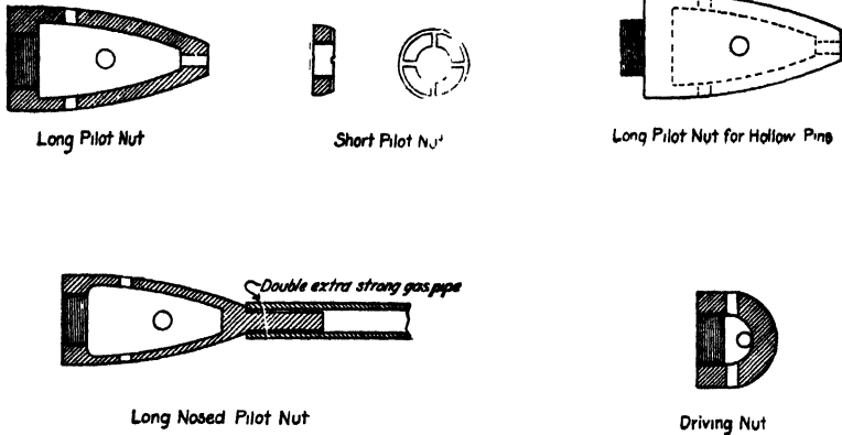
FIG. 19.—Pilot nuts.
