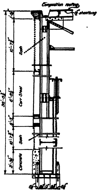
FIG. 92.—Section through outer wall of machine shop shown in Figs. 91, 92 and 93.
