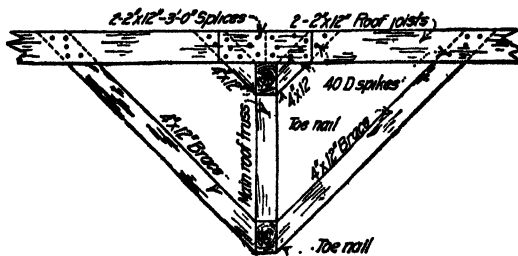
FIG. 184.—Knee brace system of truss bracing.
