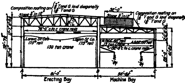
Fig. 86.—Section through locomotive boiler shop.
