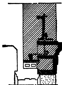
FIG. 71.—Spandrel section and lintel.
