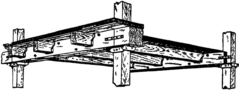
FIG. 194.—Semi-mill construction, beams in hanger
