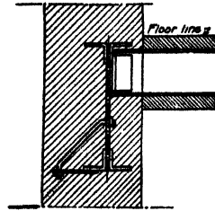
FIG. 66.—Spandrel section for solid wall.
