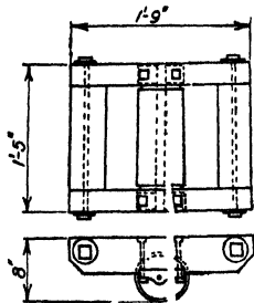
FIG. 21.—Timber buggy.
