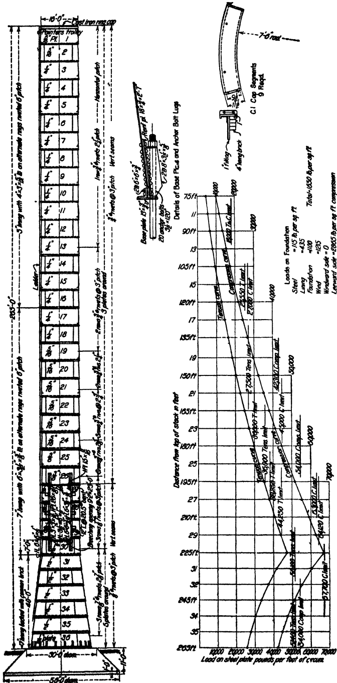
FIG. 8.—Self-supporting 265-ft. steel chimney—general design sheet.
