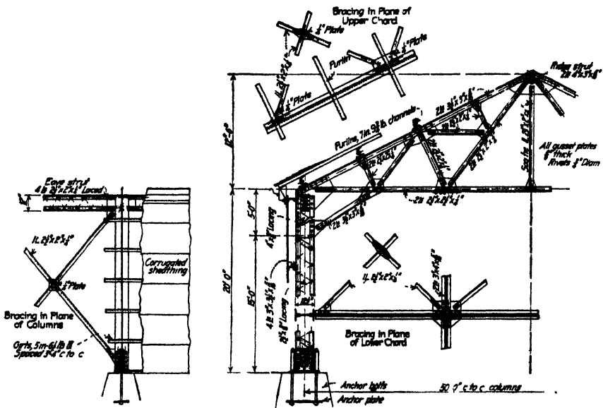
FIG. 75.—General drawing of knee-braced roof truss.
