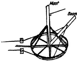
FIG. 8.—Bull wheel.
