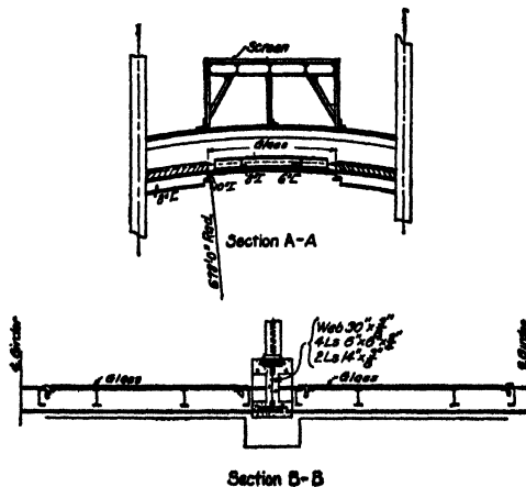
FIG. 78.—Sections through skylight framing.
