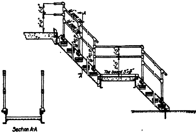
FIG. 111.—Stairs with gas pipe hand rail.
