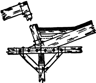
FIG. 190.—Detail of saw-tooth frame— inclined face with timber ties.
