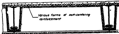
FIG. 22.—Concrete slab on self centering.
