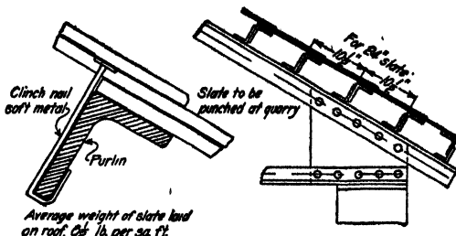
FIG. 149.—Slate on steel purlins.
