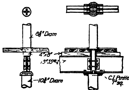
FIG. 199.—Pindle design for steel beams.
