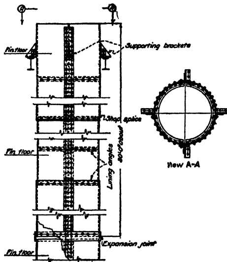
FIG. 83.—Stack supported at alternate floor levels.
