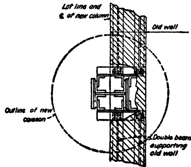
FIG. 55.—New column supporting old wall.
