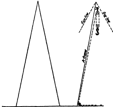
FIG. 11.—Shear legs.
