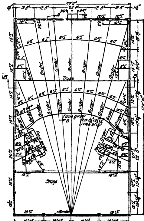
FIG. 74.—Plan of balcony construction.
