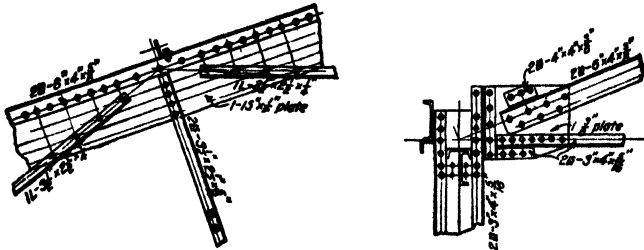
FIG. 104.—Roof truss details.
