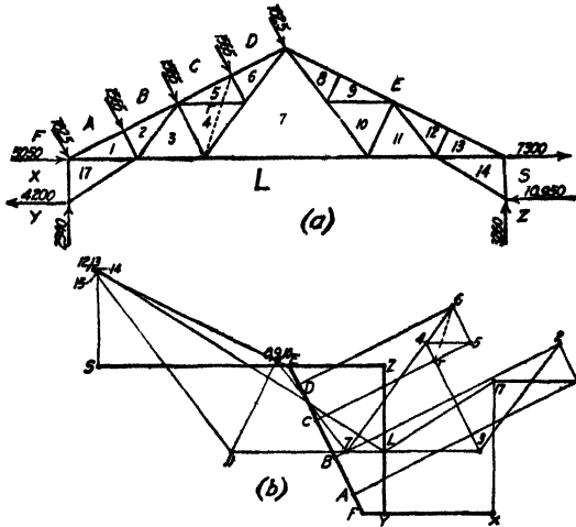
FIG. 64.—Knee-braced trusses.
