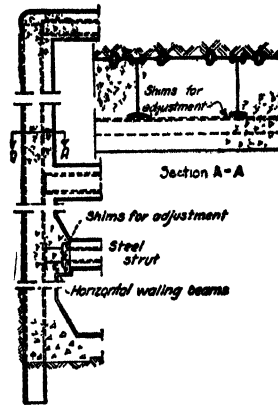
FIG. 12.—Steel sheet piling retaining wall.
