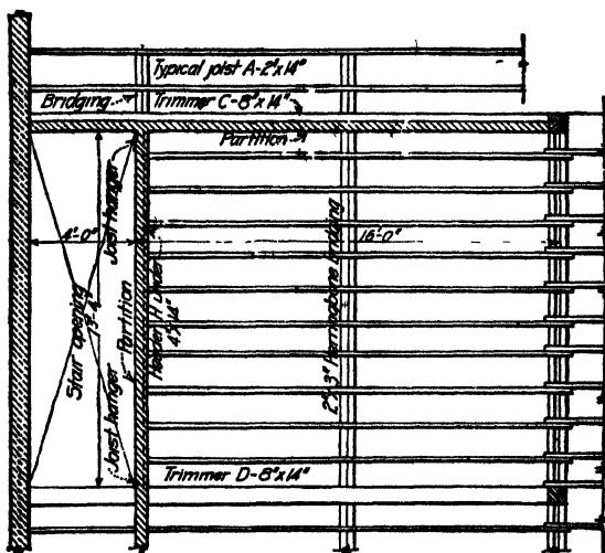
FIG. 178.—Framing plan of typical floor.
