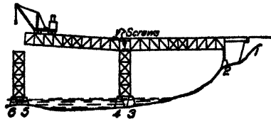
FIG. 39.—Erection of span 4-5.
