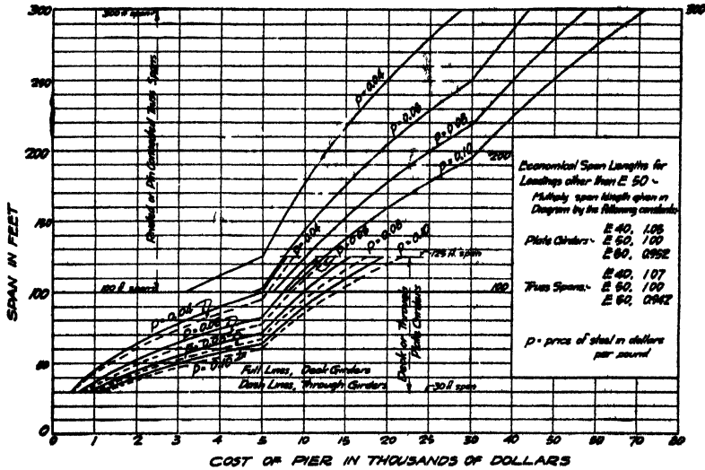
ECONOMICAL SPAN LENGTHS, E50 LOADING Fig. 1.
