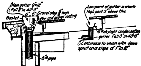
Fig. 144.—Interior gutter and down spout.
