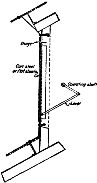
FIG. 136.—Hinged shutter.
