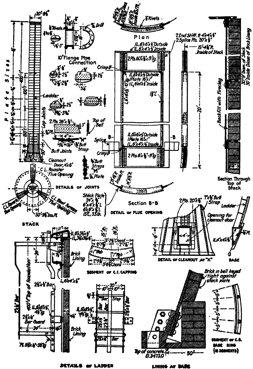
FIG. 7.—Details of 400 ft. steel chimney, Jerome, Arizona. (Chicago Bridge & Iron Works, Erectors.)
