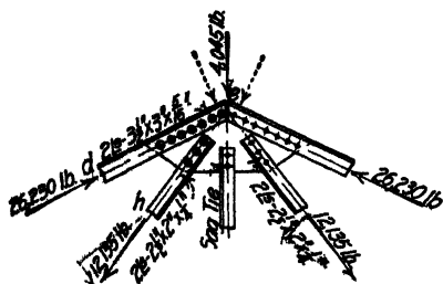
Joint e FIG. 52
