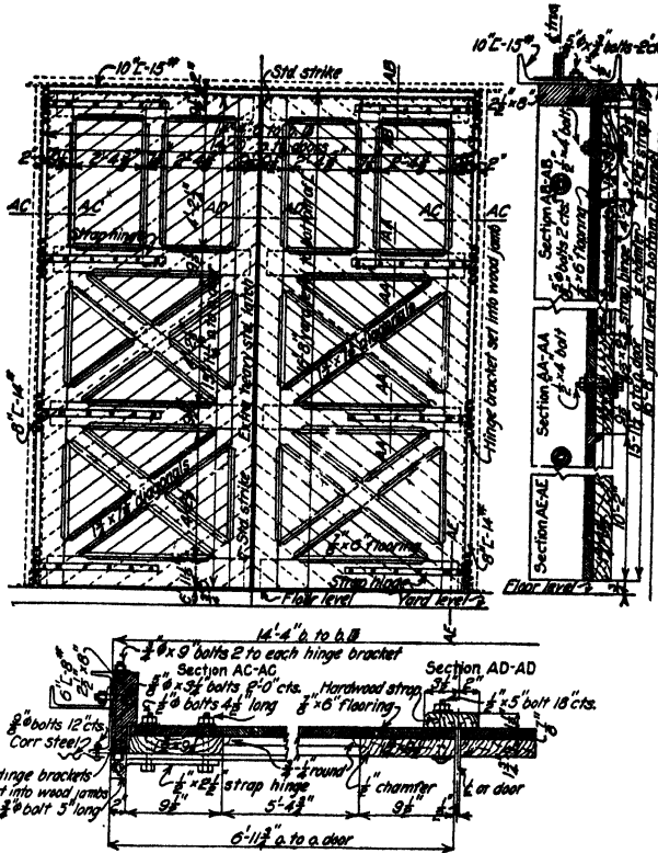
FIG. 154.—Large wooden doors.
