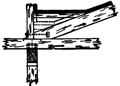
FIG. 191.—Detail of saw-tooth frame— vertical face with timber ties.
