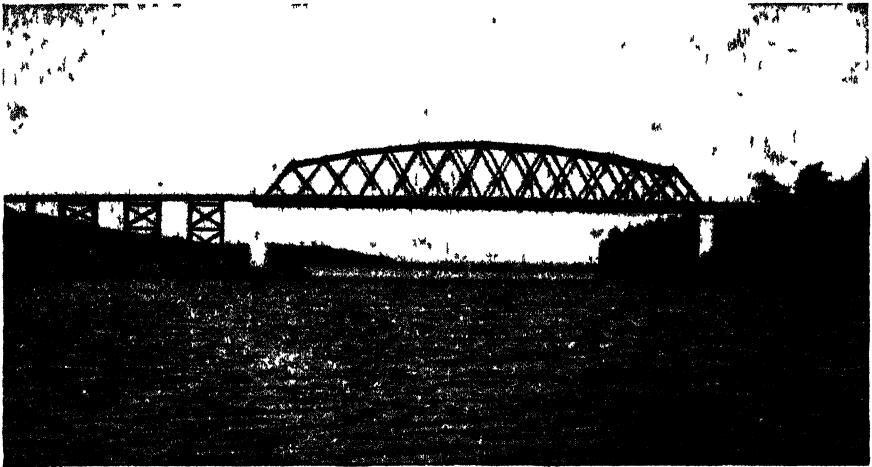
FIG. 37.—Sioux Narrows bridge, Ontario, Canada. This 210 ft span bridge, built by the Canada Creosoting Co., Montreal, is one of many connector-built bridges erected in the province of Ontario. Spans range from 90 ft to the 210-ft. bridge shown above. All framing of the approaches and superstructure made with Teco split ring connectors. (Courtesy of Timber Engineering Co.)
