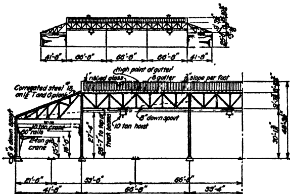
FIG. 95.—Structural steel fabricating shop. Transverse section through punching and assembling departments.
