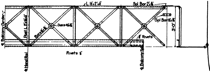
FIG. 10.—Balcony hand rail.
