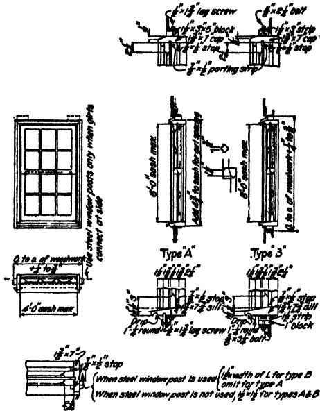
FIG. 162.—Counterbalanced window.
