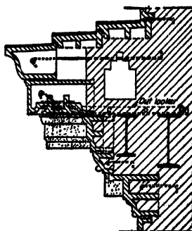
FIG. 73.—Cornice supported by outlookers.
