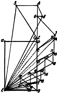
FIG. 91.—Dead load stress diagram—stresses in members of left half of arch.
