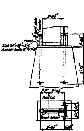
Fig. 99.—T-Shape column, base and anchorage.
