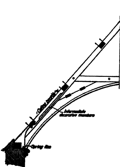
FIG 104—King post truss and bracket (Bodleian Library).
