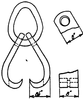
FIG. 12.—Girder hook.
