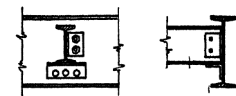
FIG. 32.—Framing into deep beams.
