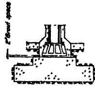
FIG. 5.—Column footing.
