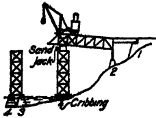
FIG. 38.—Erection of span 2-3.
