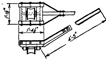
FIG. 22.—Rail jack.
