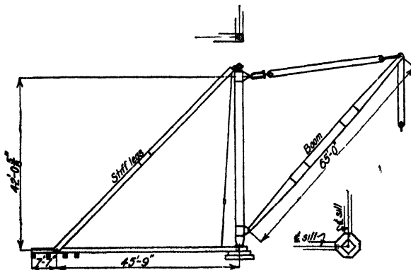
FIG. 6.—Twelve-ton stiff-leg steel derrick.
