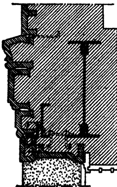
FIG. 69.—Spandrel section through wall.
