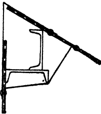
FIG. 128.—Ridge finish.
