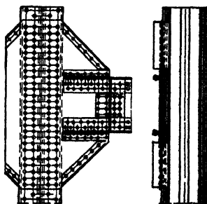
FIG. 64.—Wind-bracing girder.
