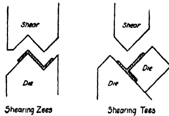
FIG. 18 -- Zee and tee shears
