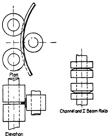
FIG. 37.—Bending rolls for angles, channels and I-beams.
