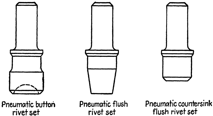
FIG. 24.—Rivet sets.
