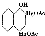
2 : 4-Diacetoxymercuri- \alpha -naphthol,
