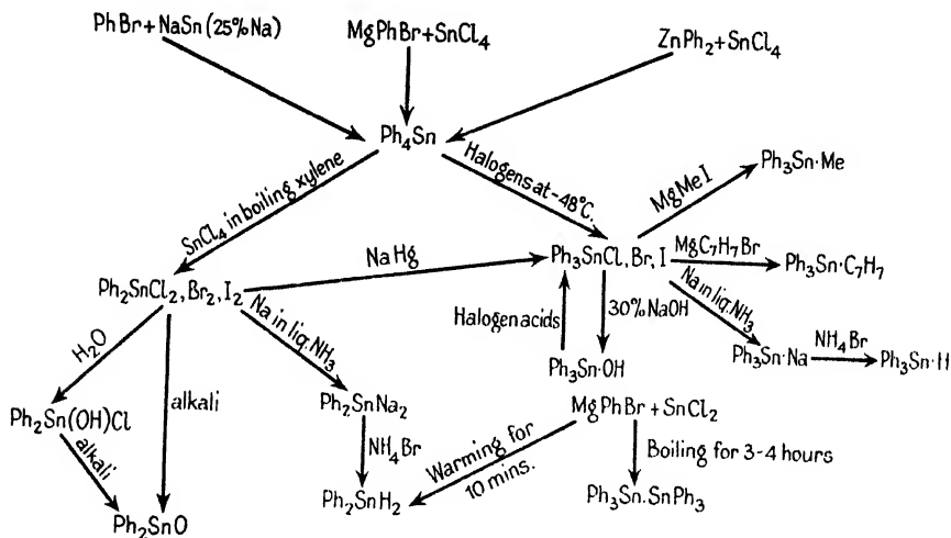
Scheme illustrating the preparation of aromatic tin compounds.
