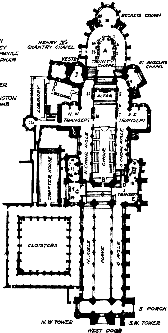
GROUND PLAN
