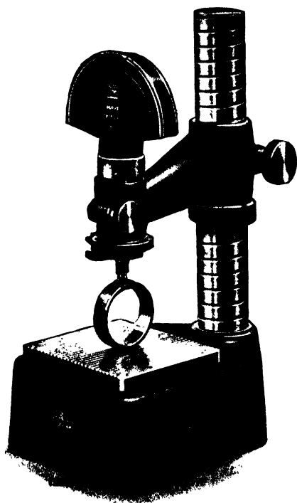
FIG. 10. 0.0001 IN. COMPARATOR (Courtesy of Messrs. Alfred Herbert, Ltd.)
