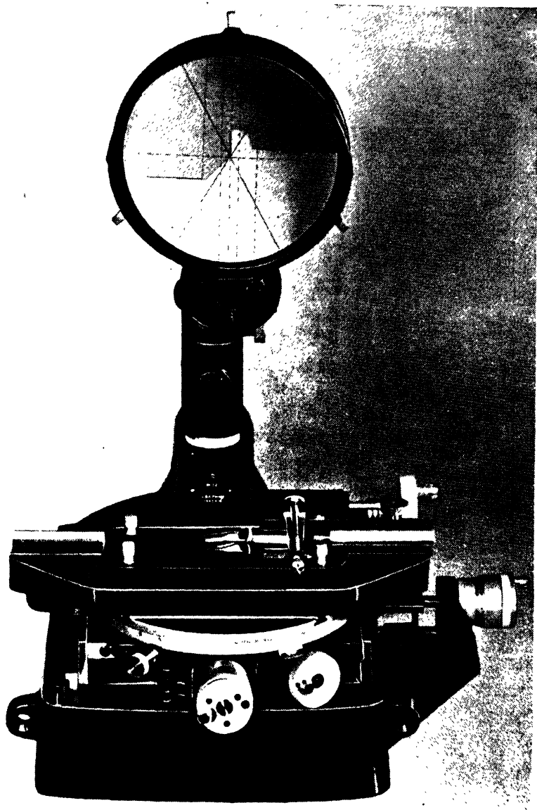
FIG. 18. TOOL-MAKER'S MICROSCOPE (Courtesy of Messrs. Alfred Herbert, Ltd.)
