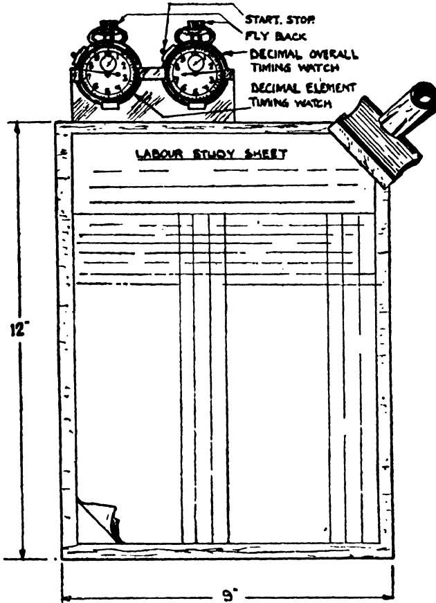
FIG. 47. TIME STUDY EQUIPMENT
