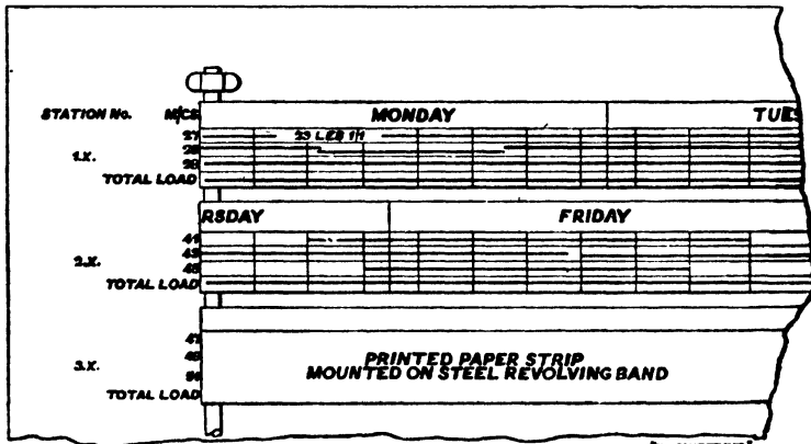
FIG. 60. SEQUENTIAL LOAD BOARD
