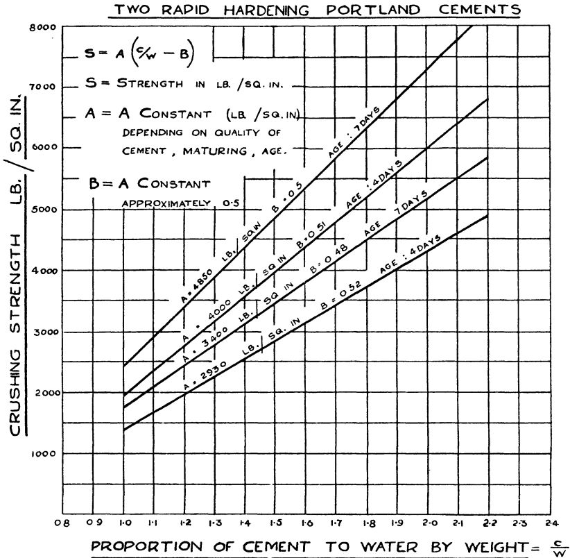
Fig. 4.—Strength and Cement-Water-Ratio.
