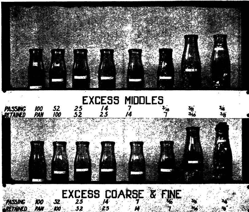
Fig. 12.—Unsuitable Gradings.
