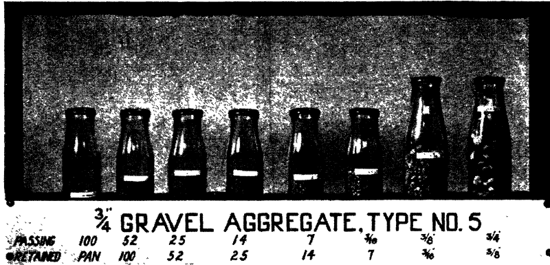
Fig. 11.—A Suitably Graded Aggregate.
