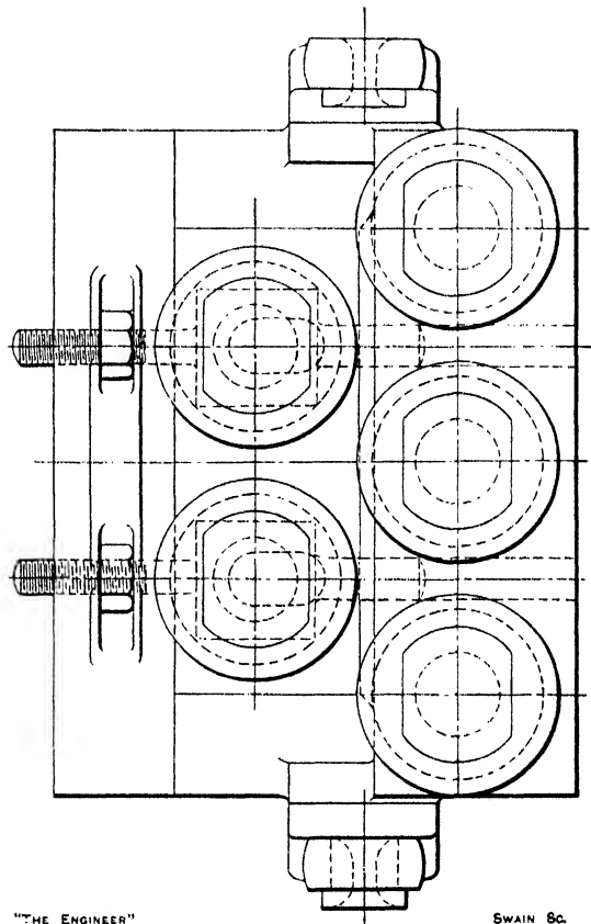
FIG. 168.—STRAIGHTENING HEAD.
