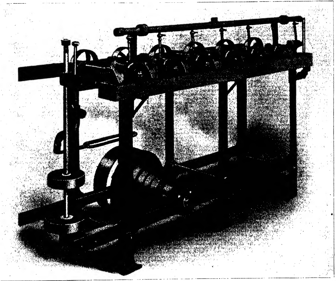
FIG. 41.—SEVEN-HOLE CONTINUOUS MACHINE—G. HATTERSLEY.
