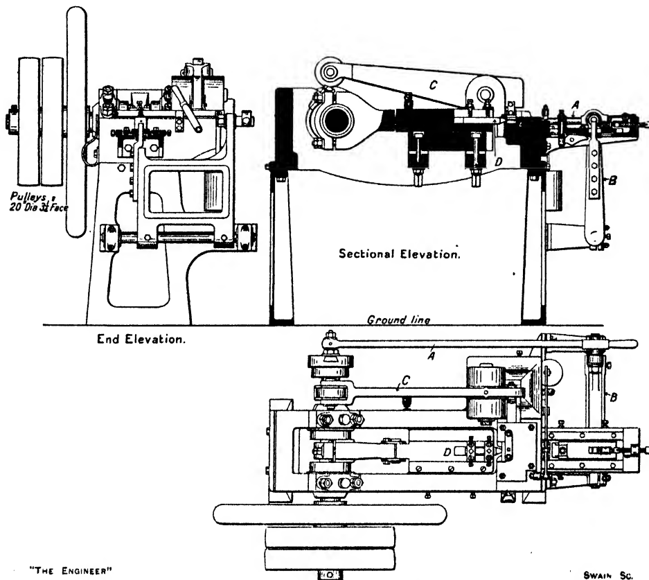
FIG. 135.—RIVET-MAKING MACHINE.
