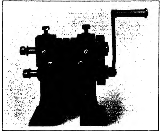
FIG. 103.—CRIMPING MACHINE—ROBERTSON.
