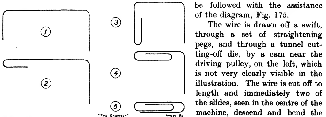
FIG. 175.—STAGES IN THE MAKING OF PAPER CLIPS.
