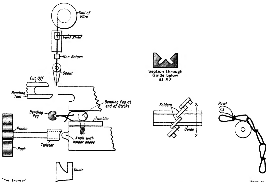
FIG. 159.—DIAGRAM OF KNOTTED CHAIN MACHINE.
