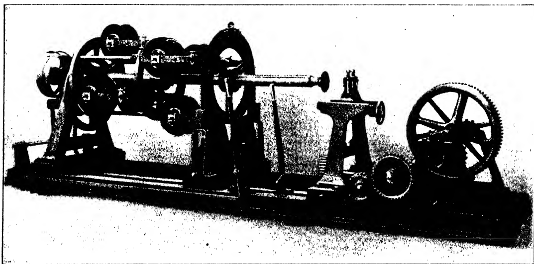
FIG. 111.—SIX-BOBBIN STRANDER.
