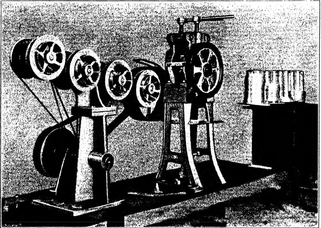
FIG. 171.—SMALL FLATTENING MILL FOR FOUR WIRES.
