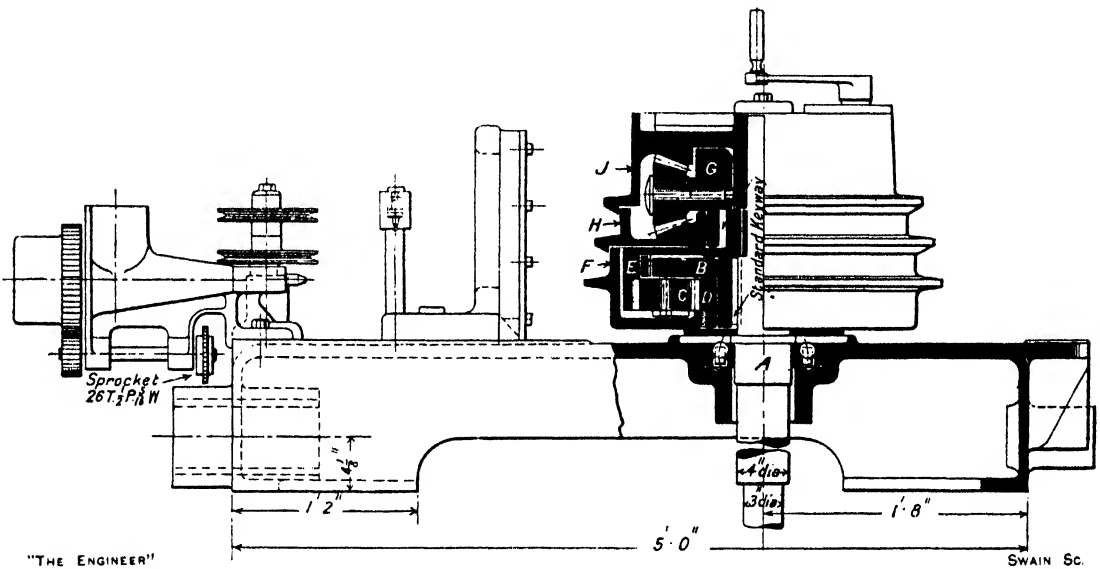
FIG. 33.—20 IN. THREE-HOLE CONTINUOUS MACHINE—BARRON AND CROWTHER.
