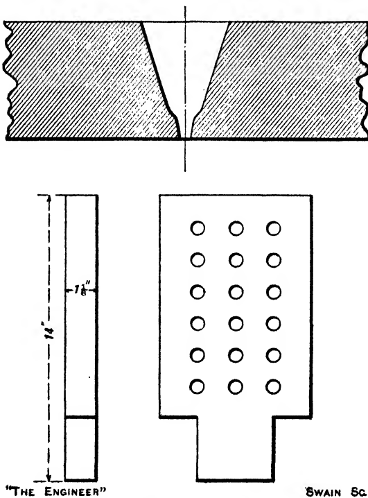
FIG. 16.—BREAKING-DOWN DIE.
