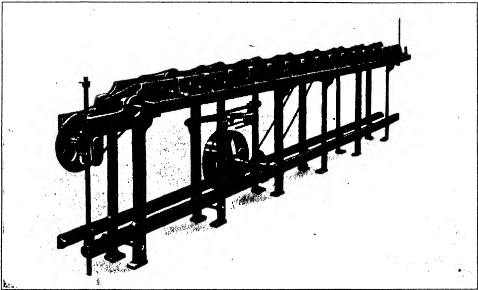
FIG. 42.—CHAIN-DRIVEN CONTINUOUS WIRE-DRAWING MACHINE—G. HATTERSLEY.
