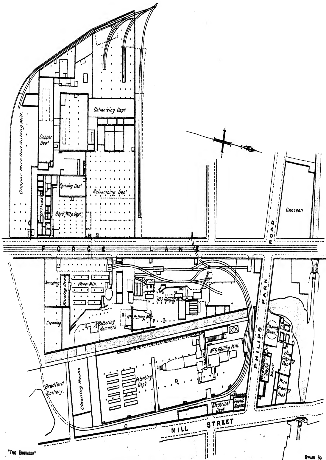
FIG. 66.—PLAN OF THE BRADFORD IRONWORKS.
