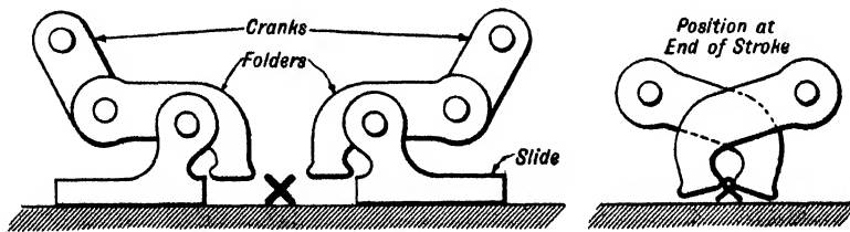
FIG. 161.—FOLDING TOOLS.
