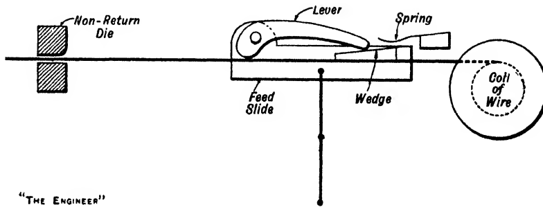
FIG. 160.—FEED GEAR.
