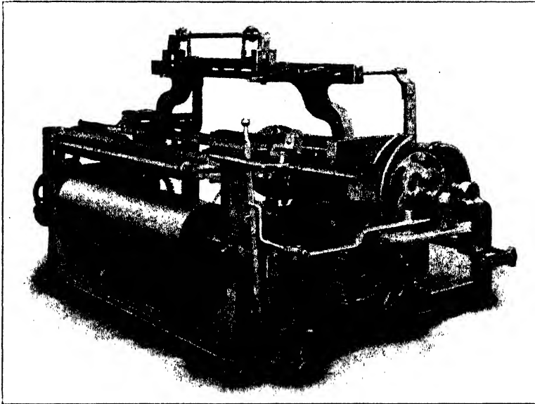
FIG. 105. WIRE-WEAVING LOOM--HATTERSLEY.
