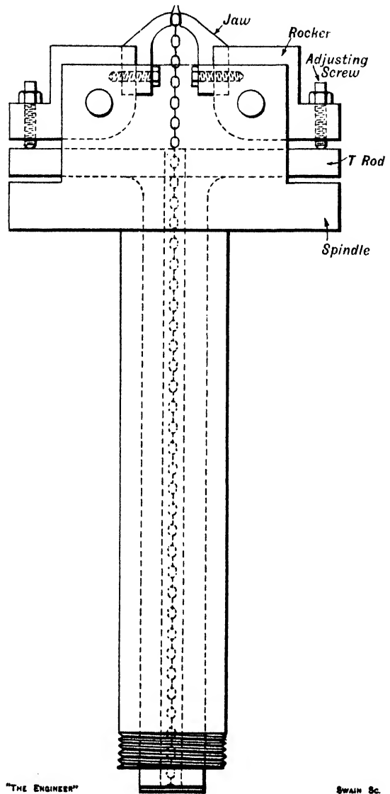
FIG. 156.—CHUCK MECHANISM.
