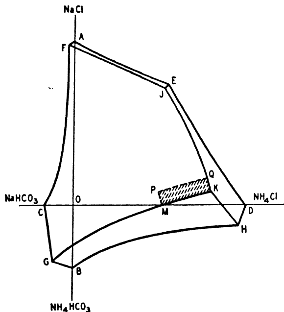
FIGURE 4-6. The System NaCl + NH_4HCO_3 \rightleftharpoons NaHCO_3 + NH_4Cl at 15°C.
