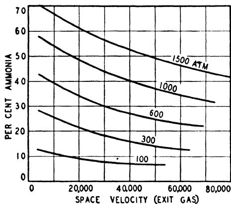
FIGURE 8-9. Effect of Space Velocity on the Conversion to Ammonia at 475°C. and Various Pressures for a Doubly Promoted Catalyst
