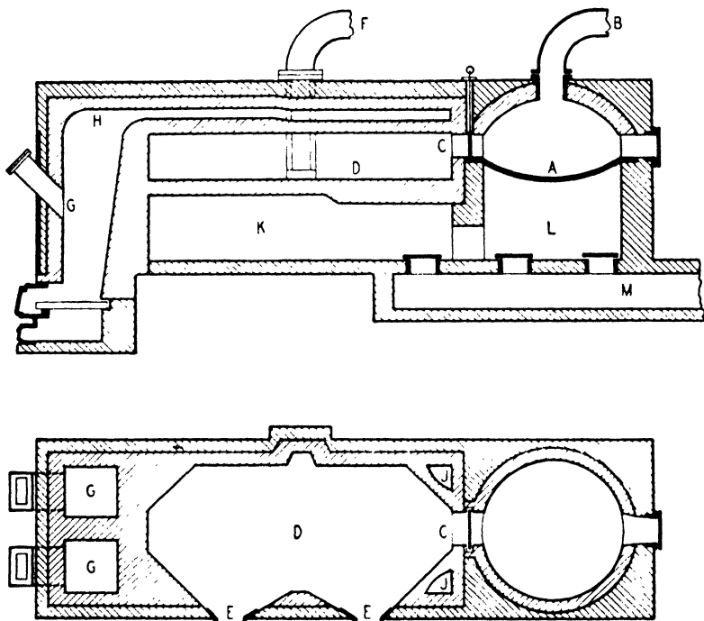
FIGURE 4-3. Saltcake Furnace
