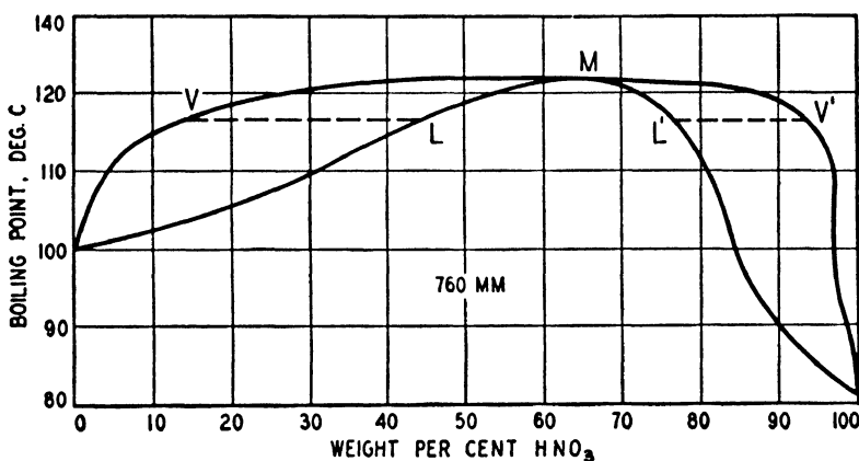
FIGURE 9-5. Vapor-Liquid Equilibrium for Aqueous Nitric Acid. M is maximum boiling point at 122^\circ\text{C} . and 68% nitric acid.
