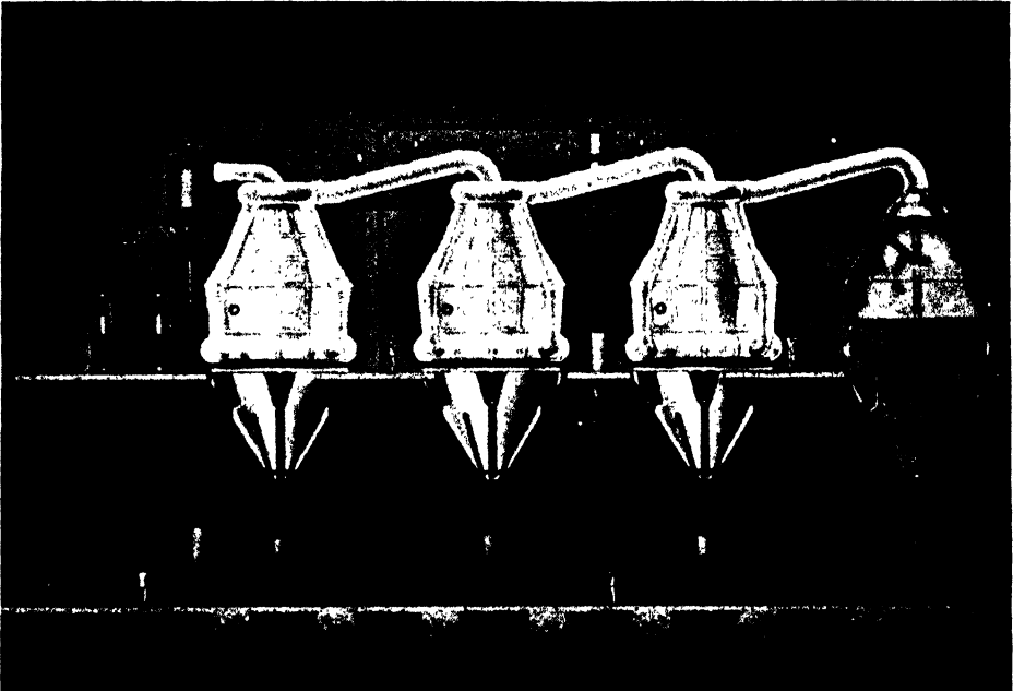
FIGURE 2-11. Quadruple Effect Salt Evaporator
