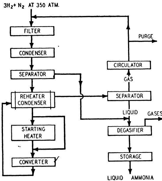
FIGURE 8-6. Ammonia Synthesis
