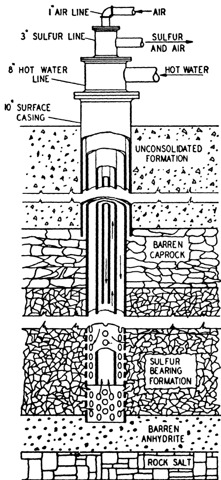
FIGURE 6-4. Frasch Process for Sulfur (redrawn from A.I.M.M.E., Industrial Minerals and Rocks , page 851, with permission)
