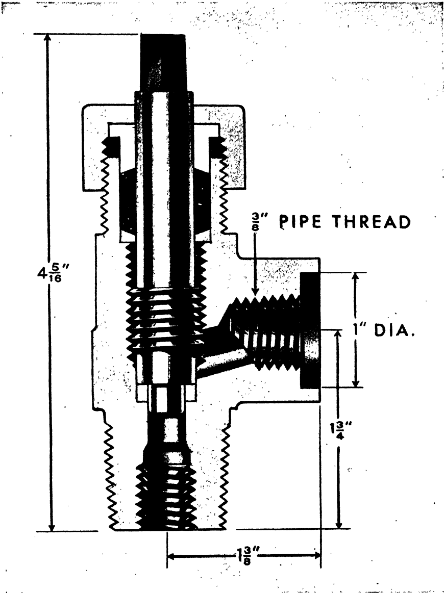
FIGURE 8-14. Valve Detail on an Ammonia Cylinder
