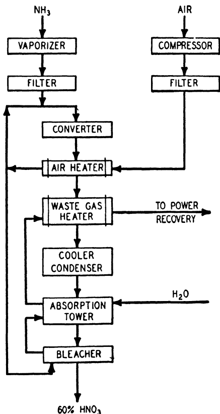
FIGURE 9-3. Ammonia Oxidation Process
