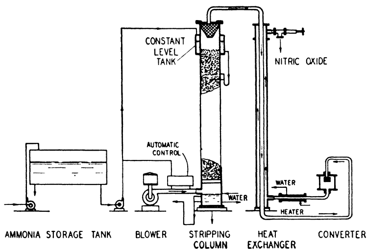
FIGURE 6-10. "Chemico" Ammonia Oxidation Process to Supply Oxides of Nitrogen
