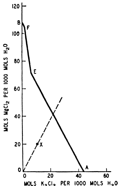
FIGURE 3-3. The System \text{KCl}-\text{MgCl}_2-\text{H}_2\text{O} , 25^\circ\text{C} . isotherm
