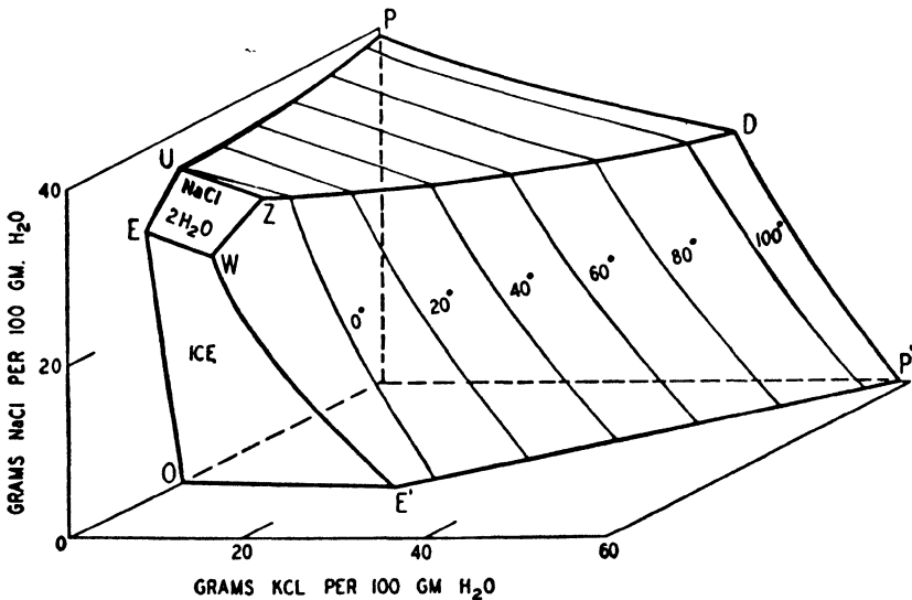
FIGURE 3-1. The System NaCl—KCl—H 2 O
