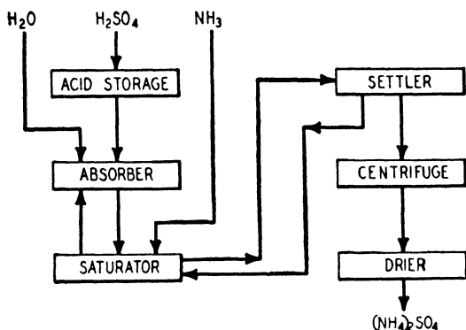
FIGURE 9-7. Wet Process for Ammonium Sulfate
