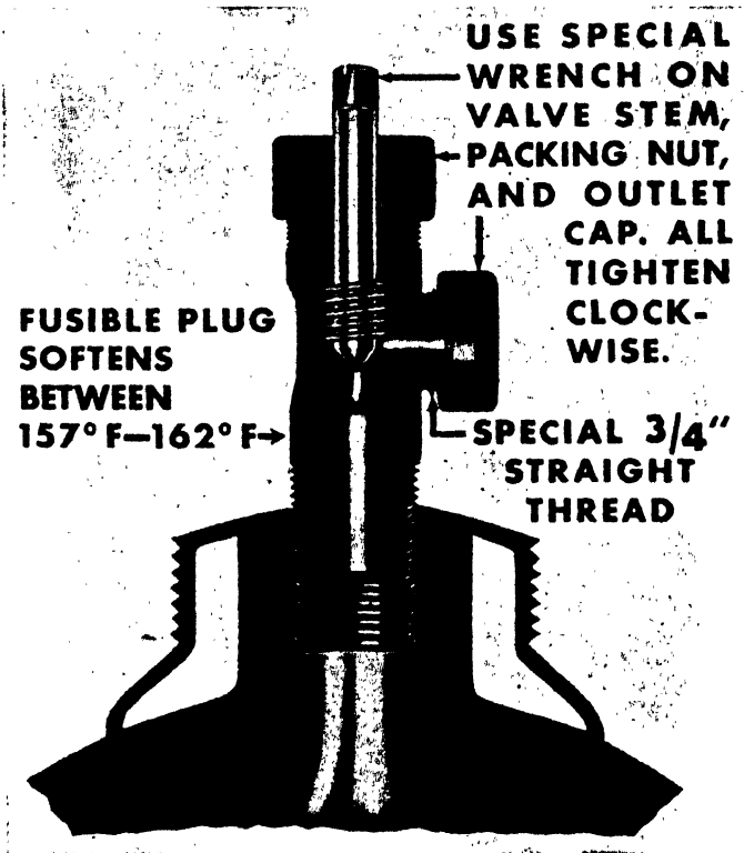
FIGURE 5-7. Cross-section of a Standard Chlorine Cylinder Valve
