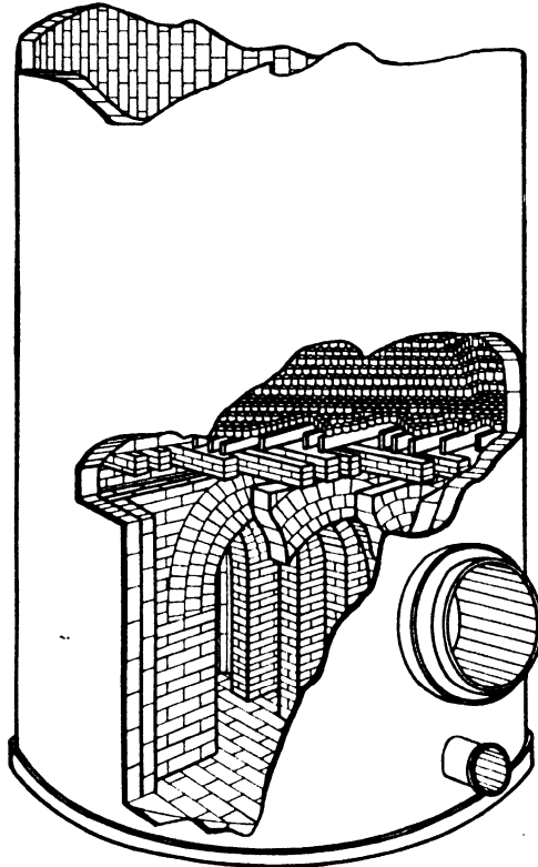
FIGURE 7-6. Absorber or Scrubber, with Metal Shell and Chemical Brick Lining Showing Construction of Arches
