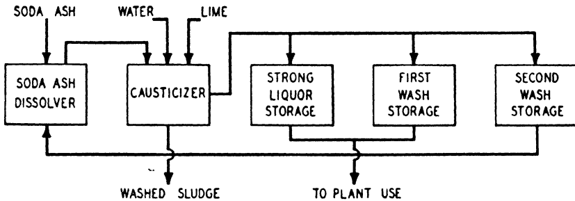
FIGURE 4-10. Batch Causticizing
