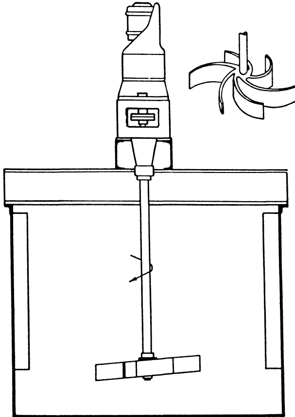
FIGURE 4 12. Turbo-Causticizer
