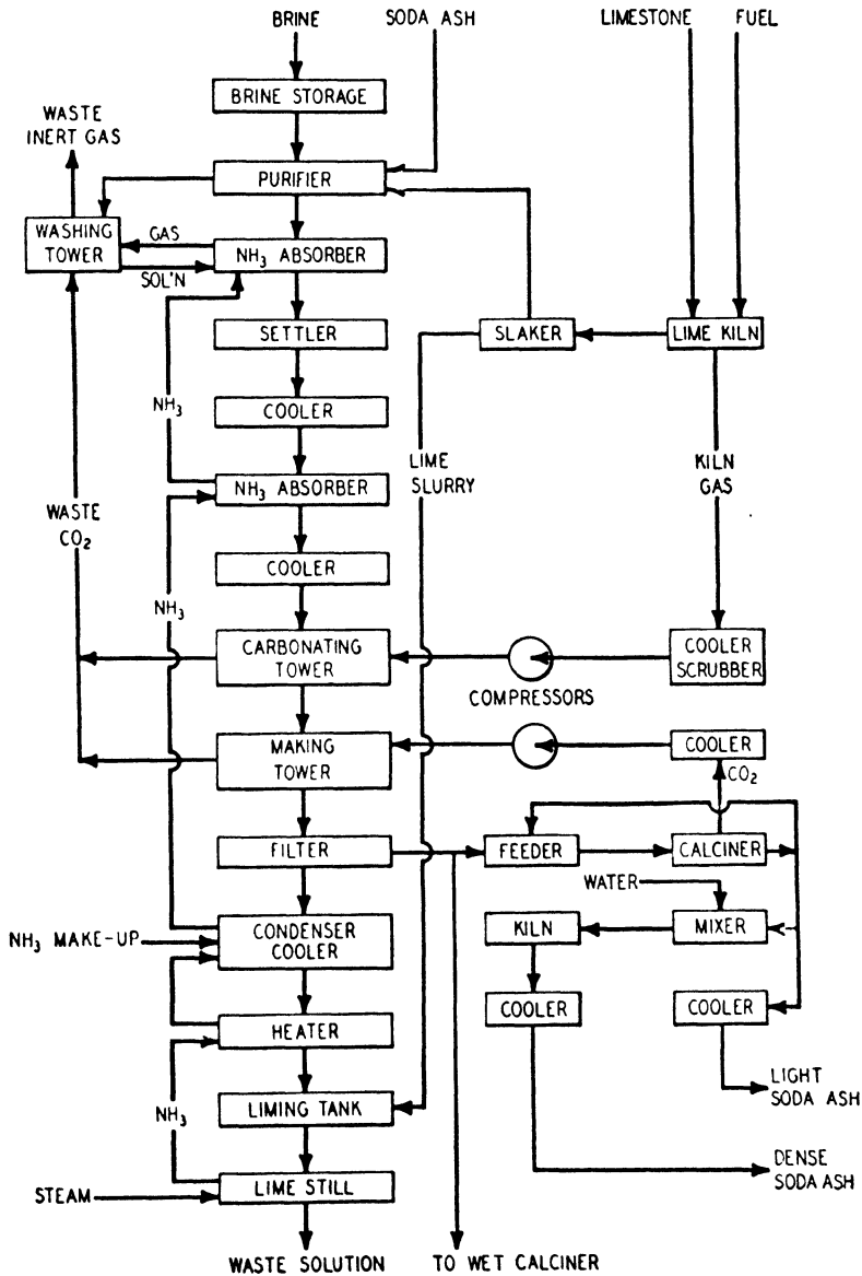
FIGURE 4-5. The Ammonia-Soda Process
