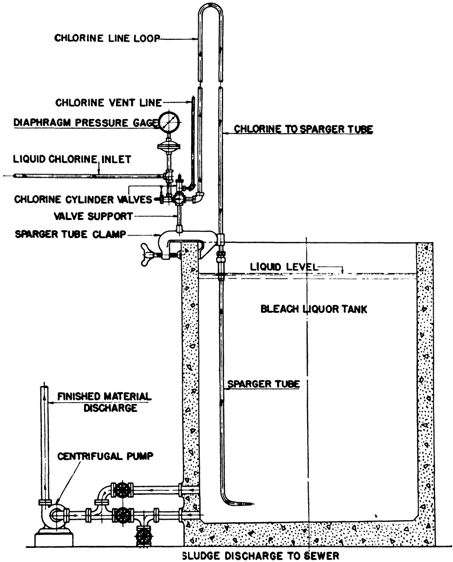
FIGURE 5-9. Manufacture of Sodium Hypochlorite by Direct Chlorination
