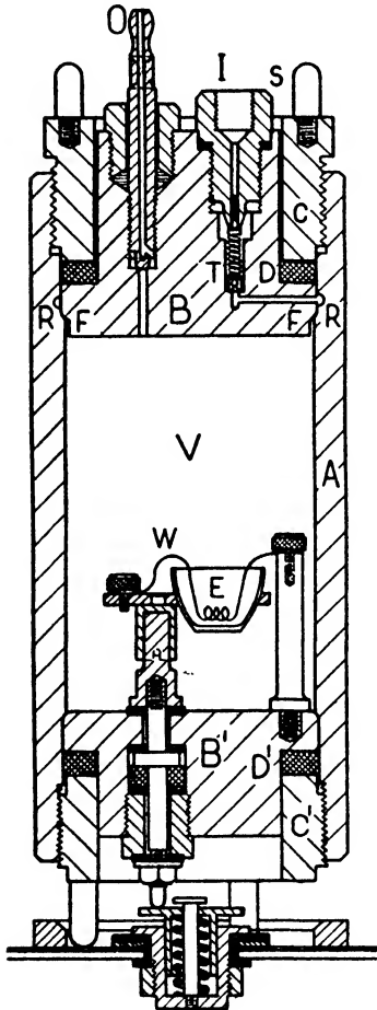
FIG. 12.—Griffin-Sutton Bomb. (By courtesy of Griffin & Tatlock, Ltd.)
