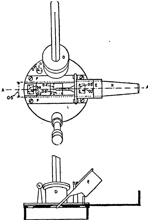
FIG. 43.—Cover, Abel Flash-Point Apparatus.
