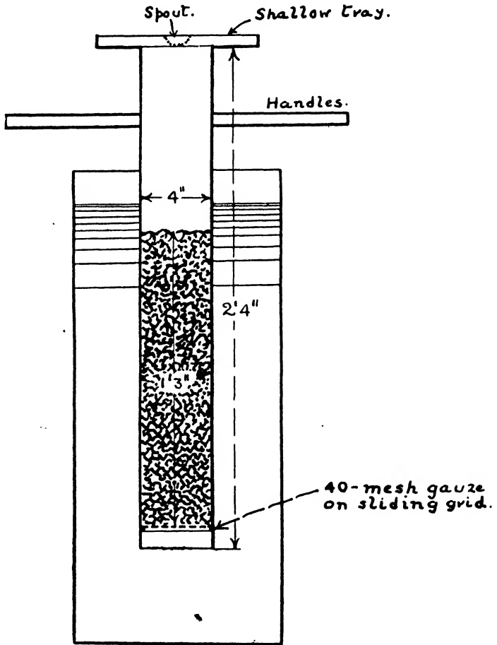
FIG. 16.—The Henry Tube for Washability Tests.
