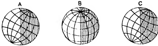
FIG. 27.—Different Inclinations of the Earth to the Sun.
