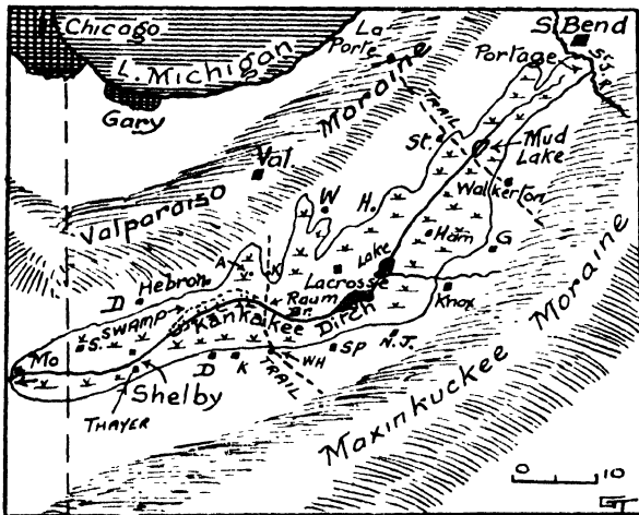
FIG. 9. The former Kankakee Swamp (Indiana), whose evolution has been described by A. Meyer. Mo.=Molence.
