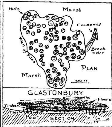
FIG. 36. Glastonbury, a late Celtic village in Somerset.
