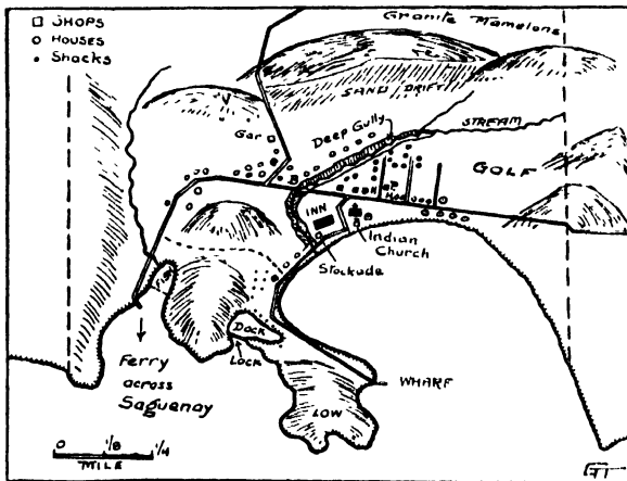
FIG. 121. A sketch map of Tadoussac looking north across the mouth of the Saguenay.
