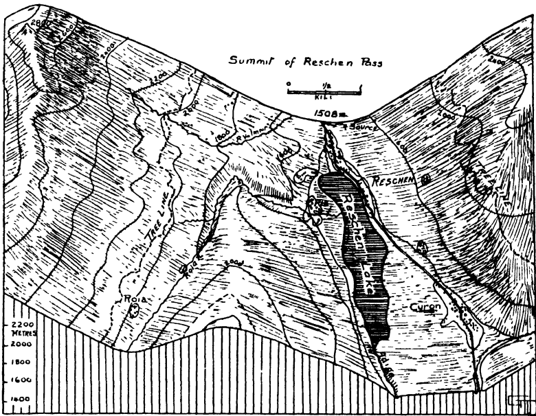
FIG. 141. Block diagram of the Reschen Pass (to natural scale) showing the sources of the Adige in a valley divide. The hamlets are enclosed in an oval line. Isolated dots are cabins. Note the tree line. (Looking north.)
