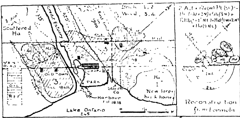
FIG. 30. (Left) A functional plan of the little town of Port Credit 12 m. west of Toronto. Two contours are charted. The houses are in four classes; Ha, Hb, Hc, and Hd, the latter are mostly shacks. (Right) A plan reconstructed from the formula shown at the top of the figure. It is to be compared with the actual plan on the left.
