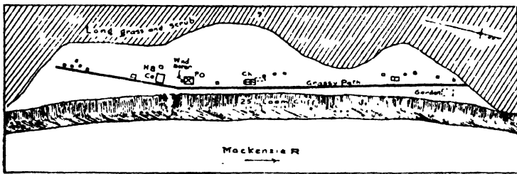
FIG. 13. A sketch survey of Fort Wrigley (62° N.), looking west. The settlement is half a mile long. (See W. in Fig. 4.)
