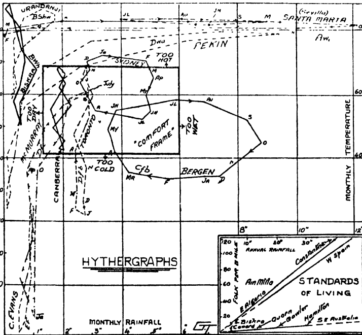
FIG. 1A. Hythergraphs of the places described in Chapter II, to show the widespread character of the discussion. Köppen formulae are added. The "Comfort Frame" includes the climates which are generally comfortable. Inset is a graph which compares the standards of living in three regions (Algeria, Spain, and South Australia), which all have the same environments.
