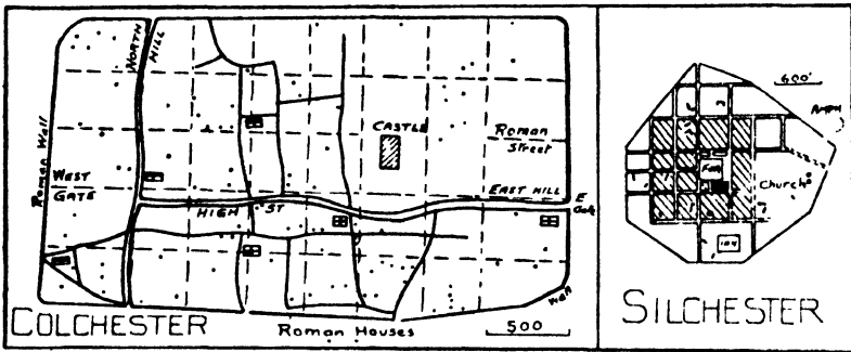
FIG. 58. A reconstruction of Roman Colchester, in which the ancient streets appear as broken lines. The modern roads are curved heavy lines. Modern churches are inserted. (After T. Adams.)
