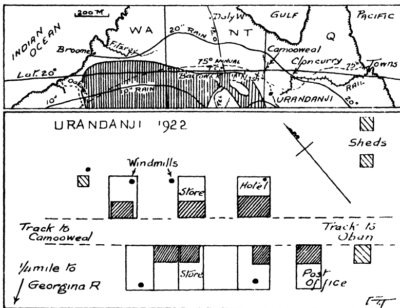
FIG. 7. (Top) A map of tropical Australia to show the position of Urandanji, just to the east of the widest expanse of empty land in Australia. Ruled areas are desert, and isotherms and isohyets are inserted. (Bottom) A sketch survey of the little settlement of Urandanji on the main stock-route from Camooweal to Marree.
