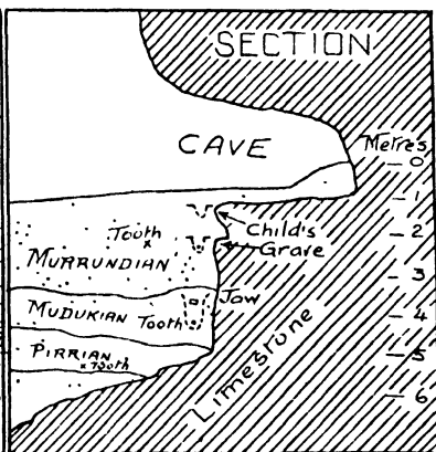
FIG. 34. Vertical section through a cave above the Murray River at Devon Downs, in South Australia (after Hale & Tindale).
