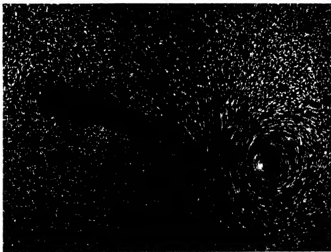
FIG. 55.—After formation of the starting vortex the airfoil was stopped and then the picture was taken.
