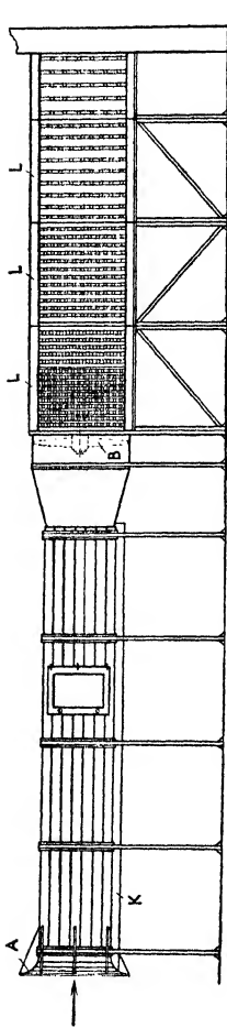
FIG. 219.—Old wind tunnel in Teddington (1912).
