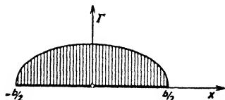
FIG. 163.—Elliptic lift distribution \Gamma = \Gamma_c \sqrt{1 - \left(\frac{x}{b/2}\right)^2}
