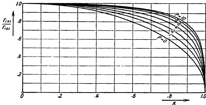
FIG. 167.—Distribution of circulation along the span of rectangular wings of various aspect ratios \left(P = \frac{2b}{\pi c}\right)
