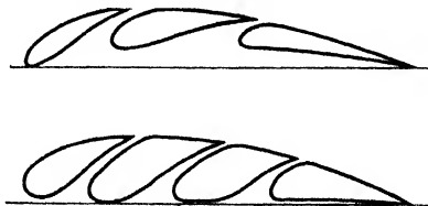
FIG. 100.—Multiply-slotted wings.
