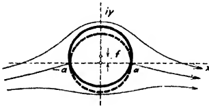
FIG. 138.—Flow round circular cylinder with a circulation such that the two stagnation points are in -a and +a .
