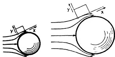
FIG. 4.—Streamlines round two spheres of different size.
