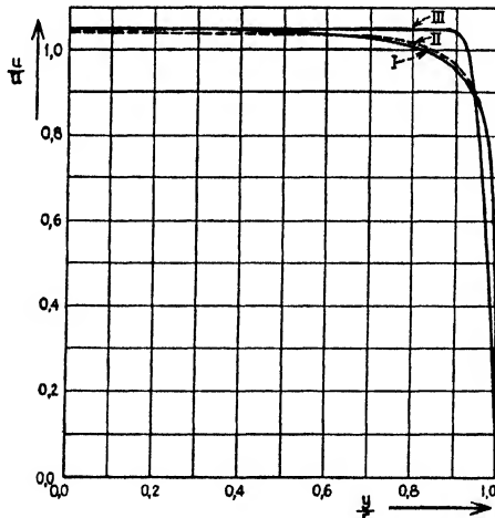
FIG. 27.—I, velocity distribution in turbulent flow, 5 radii from entrance; II, the same curve calculated by the method of Lutzko; III, velocity distribution for laminar flow at same distance from entrance.
