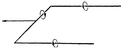
FIG. 148.—Simple picture of vortex system of finite wing.
