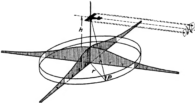
FIG. 150.—Transfer of airplane weight to ground.
