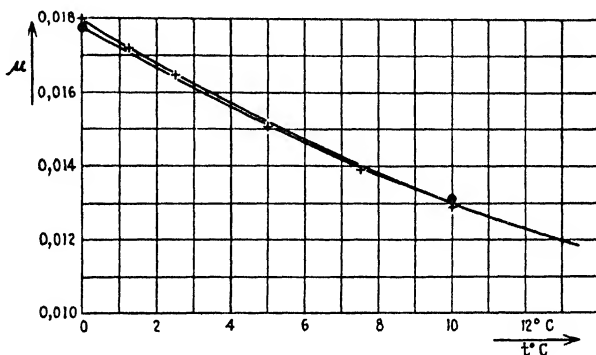
FIG. 6.—Viscosity of water as a function of the temperature. The upper curve after Bingham and White; the lower one after Thorpe and Rodger. The + points by Hagen (1839); the ⊗ by Poiseuille (1841).
