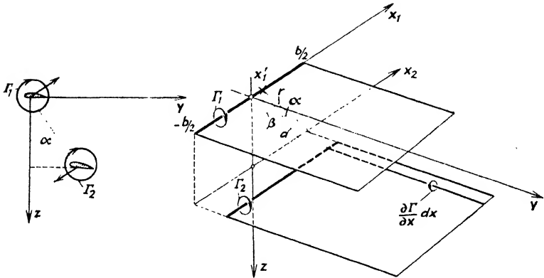
FIG. 177.—Staggered biplane.
