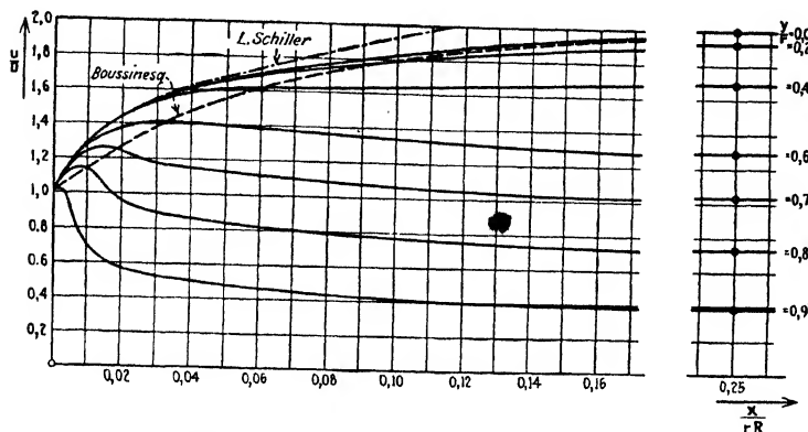
FIG. 13.—Laminar velocity distribution after tests by Nikuradse.
