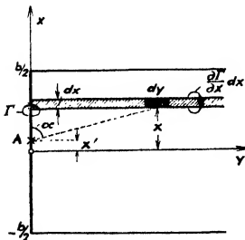
FIG. 161.—The surface of discontinuity behind a wing of given lift distribution.
