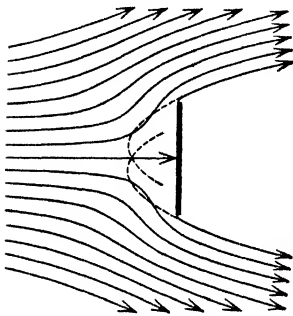
FIG. 60.—Discontinuous potential flow round plate (two dimensional). The boundary consists approximately of two parabolic arcs.
