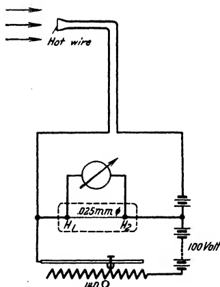
FIG. 206.—Hot-wire hook-up of Huguenard.
