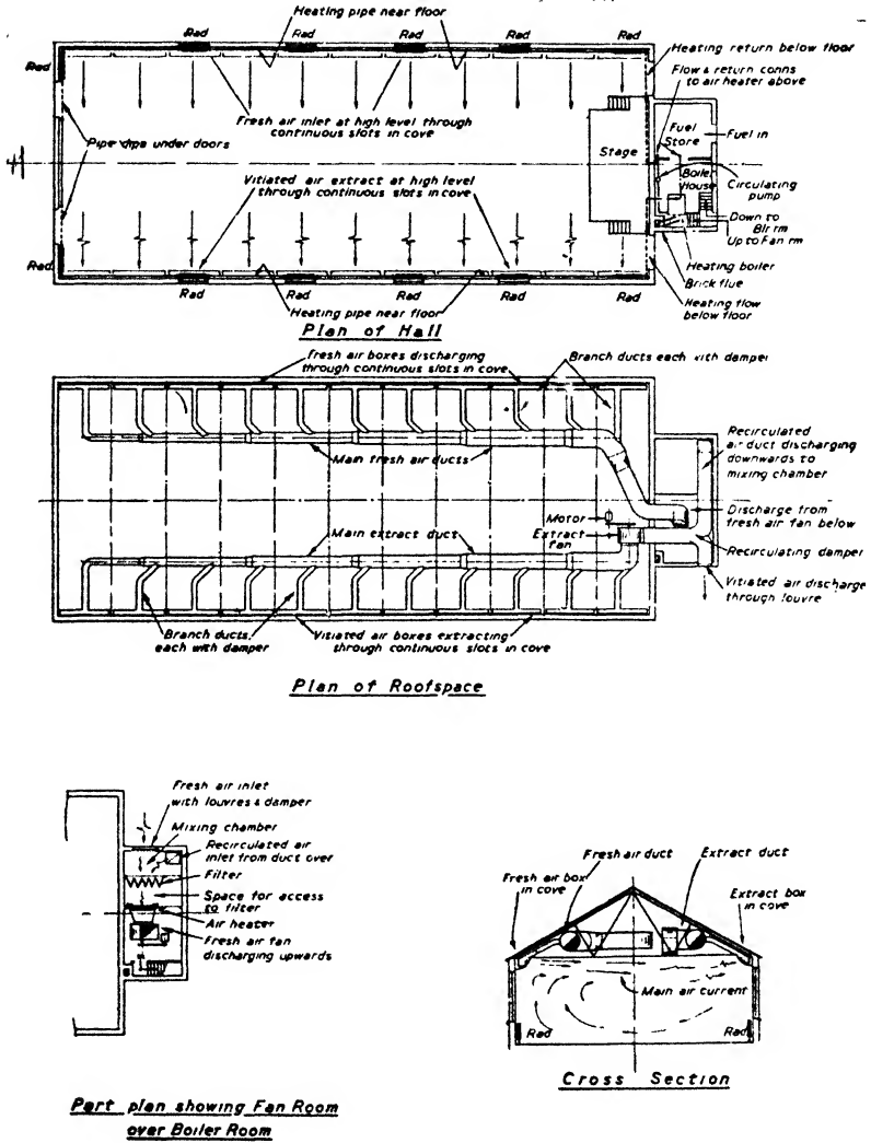
FIG. 39 ASSEMBLY HALL SHOWING HEATING AND VENTILATING PLANT
