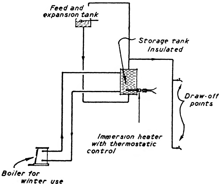
FIG. 23 DIAGRAM OF DOMESTIC H.W.S. SYSTEM WITH IMMERSION HEATERS
