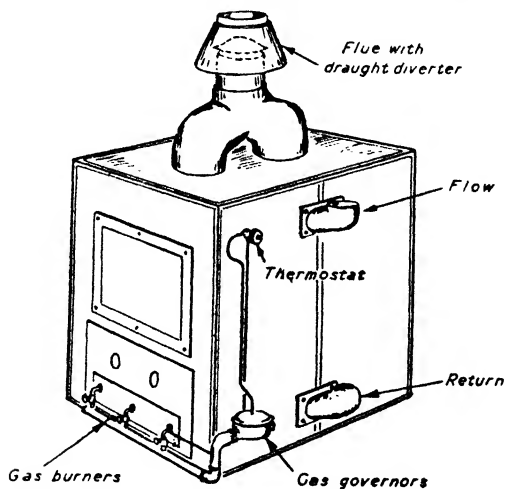
FIG. 14 GAS BOILER
