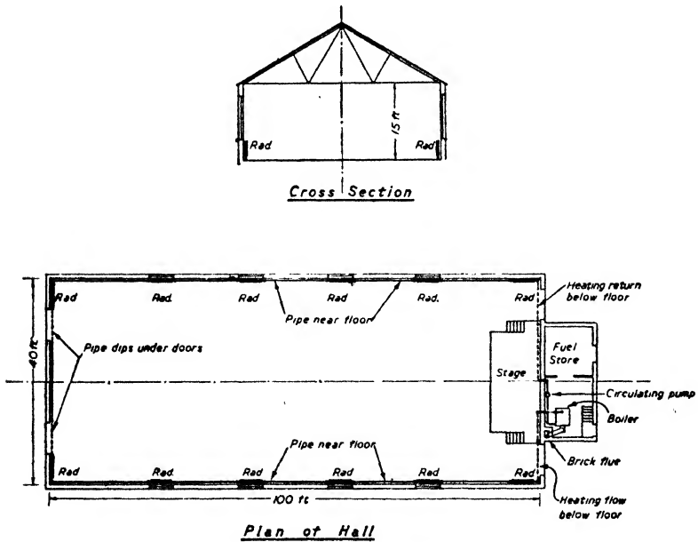
FIG. 33 ASSEMBLY HALL SHOWING HEATING PLANT
