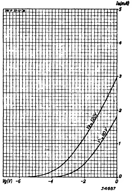
Fig. 4 Anode current as a function of the grid bias at V_a = 90 V and 120 V.
