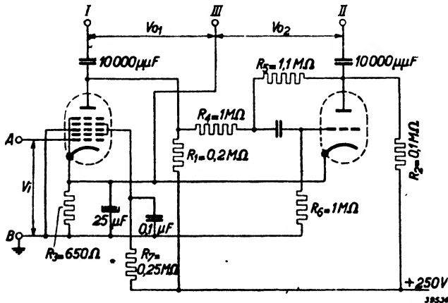
Fig. 6 Circuit diagram of the ECH 21 employed as A.F. amplifier and phase inverter preceding a push-pull output stage; the output voltages V_{01} and V_{02} are exactly in counter-phase and are applied to the grids of two output valves. For clarity, the triode and heptode sections are depicted as separate valves.
