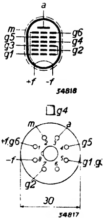
Fig. 2 Arrangement and sequence of contacts.
