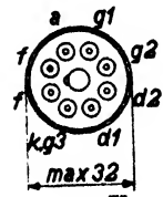
Fig. 3 Arrangement and connections of the electrodes.
