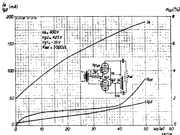
Fig. 7 Anode current I_a , screen grid current I_{g2} and distortion d as function of output power W_o of two EL 50 valves in push-pull circuit with fixed grid bias, at V_a = 400V , V_{g2} = 425V , V_{g1} = -35V and R_{aa} = 5000 Ohms.
