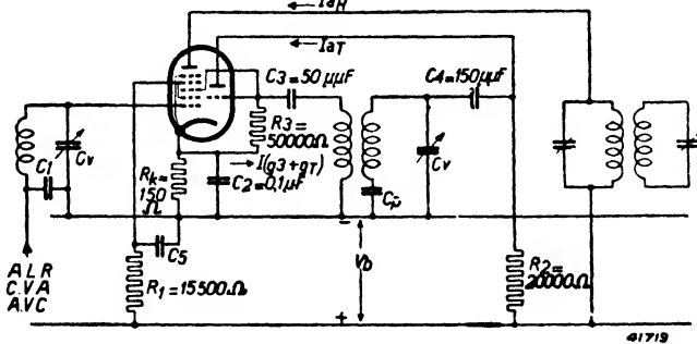
Fig. 8 Circuit diagram showing the ECH 4 employed as mixer valve.
