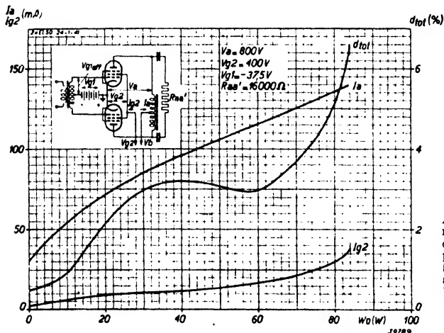
Fig. 9 Anode current I_a , screen current I_{g2} and total distortion d_{tot} as function of the output power W_o of two push-pull EL 50 valves, with fixed grid bias, at V_a = 800V , V_{g2} = 400V and V_{g1} = -37.5V ; R_{aa} = 16,000 Ohms.
