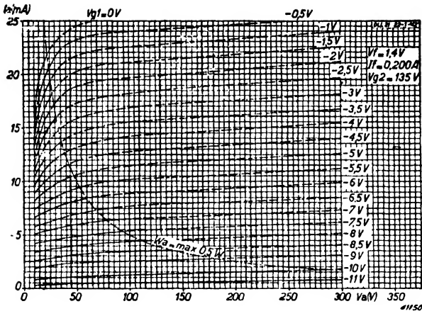
Fig. 12 Anode current of one pentode section as function of anode voltage at V_{g_2} = 135 \text{ V} , V_f = 1.4 \text{ V} and I_f = 200 \text{ mA} , with V_{g_1} as parameter.
