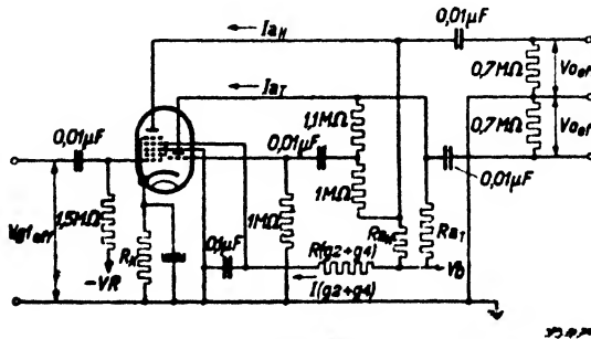
Fig. 16 Circuit diagram of the ECH 21 employed as phase inverter with feedback, to illustrate the above remarks and symbols.
