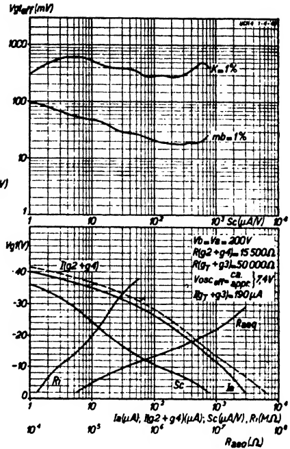
Fig. 7 Upper diagram; Maximum permissible effective value of R.F. alternating voltage at 1% cross modulation ( K = 1\% ) and also at 1% modulation hum ( mb = 1\% ), both in respect of the interfering signal at the grid, as a function of conversion conductance, with screen grid fed through a resistance of 15,500 ohms from the 200 V line.
