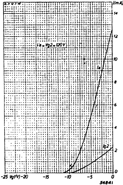
Fig. 3 Anode and screen current as a function of the grid bias at V_a = V_{g_2} = 120 V.
