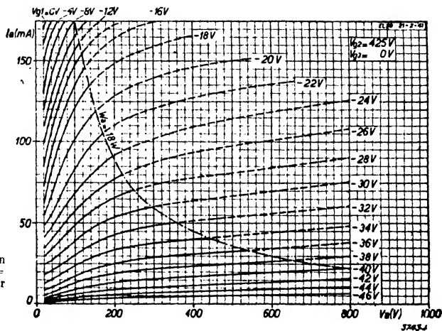
Fig. 4 Anode current as a function of anode voltage at V_{g2} = 425 \text{ V} , with V_{g1} as parameter (400 V operation).
