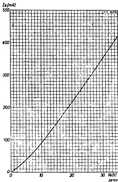
Fig. 4 Anode current as a function of direct voltage.
