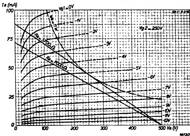
Fig. 5 Anode current as a function of anode voltage at V_{g2} = 250V , with grid bias as parameter. In the figure the load lines in respect of R_a = 5700 \text{ Ohms} (11 W operation) and R_a = 7000 \text{ Ohms} (9 W operation) are also shown.
