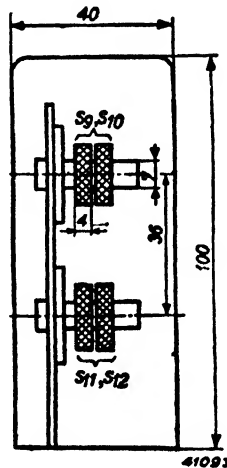
Fig. 2 Sketch of the I.F. bandfilter coils. S_9 , S_{10} , S_{11} and S_{12} = 2 \times 155 turns Litz wire wound on iron cores and mounted in a "Phillite" box.
