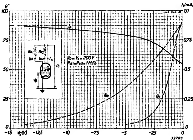
Fig. 4 Shadow angles \Theta_1 and \Theta_2 , measured at the edge of the screen, and screen current I_s as a function of grid voltage at a supply potential of 200 V.
