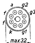
Fig. 2 Arrangement and sequence of contacts.
