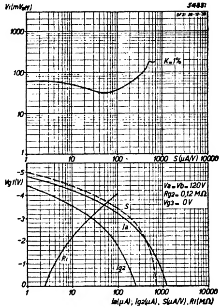
Fig. 9 Upper diagram. Effective value of alternating grid voltage as a function of mutual conductance with 1 % cross modulation, at V_a = V_{g_1} = 120 V. Lower diagram. Mutual conductance S , anode current I_a , screen current I_{g_2} , and internal resistance R_i as function of grid bias, at V_a = V_b = 120 V.
