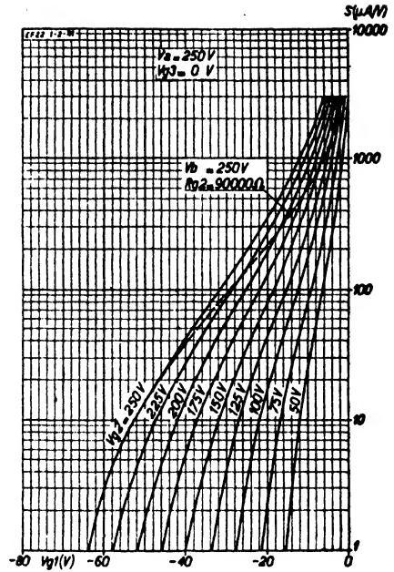
Fig. 4 Mutual conductance as a function of grid bias at V_a = 250 V and V_{g_3} = 0 V, with screen grid voltage as parameter.
