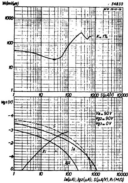
Fig. 8 Upper diagram; Effective value of alternating grid voltage as a function of mutual conductance with 1 % cross modulation, at V_a = V_{g_2} = 90 V. Lower diagram. Mutual conductance S , anode current I_a , screen current I_{g_2} , and internal resistance R_i as function of grid bias, at V_a = V_{g_2} = 90 V.
