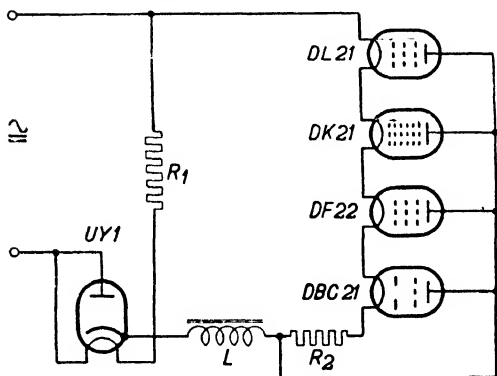
Fig 1 Circuit diagram of the supply section of an AC/DC-Battery receiver.
