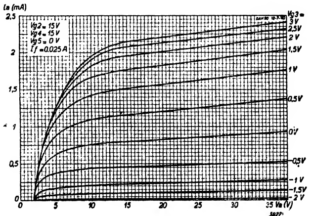
Fig. 5 Anode current as a function of anode voltage, with V_{g3} as parameter.
