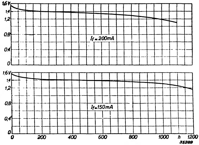
Fig. 2 Characteristic curves of the life of a battery giving a nominal voltage of 1.4 at about 225 A hours, assuming that the receiver is used for 4 hours per day. The upper curve was plotted in respect of a receiver having a total filament current of 200 mA. The life of the battery is then about 1100 hours. Using the battery 4 hours per day, this means a total life of about 9 months. On a total filament current of 150 mA (lower curve), employing the new "economy" valves, the life of the battery can be extended to 1200 hours.
