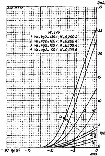
Fig. 4 Anode and screen current of one pentode section of the DLL 21 as a function of the grid bias at V_f = 1.4 V, in respect of different values of anode and screen voltage and filament current.
