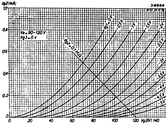
Fig. 6 Screen grid current as a function of screen voltage at V_a = 90 - 120 V, with V_{g1} as parameter.
