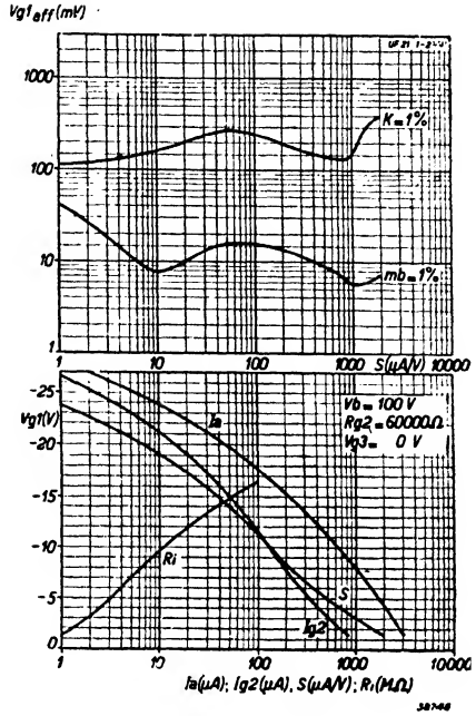
Fig. 8 At V_b = 100 V , R_{g2} = 60,000 Ohms (screen fed through a resistance) and V_{g3} = 0 V . Upper diagram; maximum permissible effective value of alternating grid voltage with 1% cross modulation ( K = 1\% ) and also with 1% modulation hum ( mb = 1\% ), as function of mutual conductance. Lower diagram; Mutual conductance, anode current, screen grid current and internal resistance as function of grid bias.
