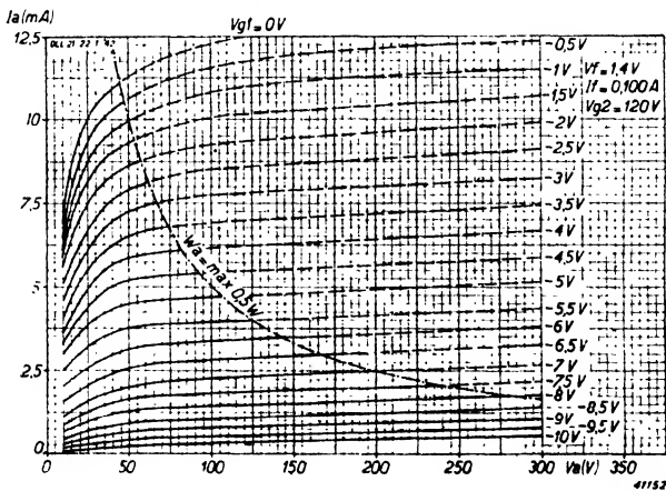
Fig. 8 Anode current of one pentode section as function of anode voltage at V_{g2} = 120 V, V_f = 1.4 V and I_f = 100 mA, with V_{g1} as parameter.
