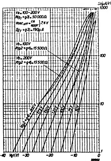
Fig. 5 Upper diagram; Maximum permissible effective value of R.F. alternating voltage at 1% cross modulation ( K = 1\% ) and also for 1% modulation hum ( mb = 1\% ), both in respect of the interfering signal at the grid, as a function of conversion conductance. Screen grid fed through a resistance of 15,500 ohms from the 100 V line. Lower diagram; Conversion conductance Sc , anode current I_a , screen grid current I(g_2 + g_3) , internal resistance R_i and equivalent noise resistance R_{aeg} as a function of grid bias.
