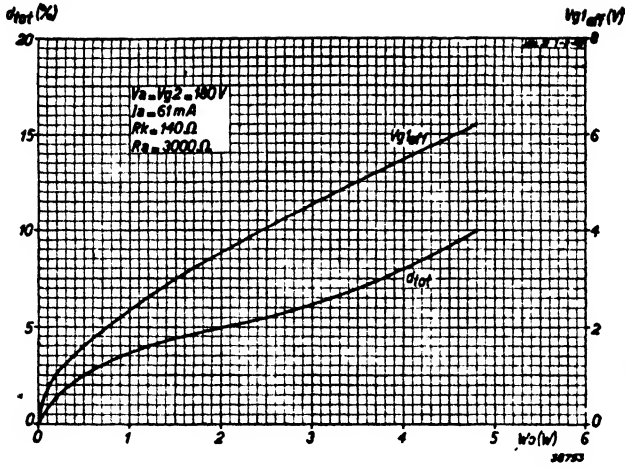
Fig. 8 Total distortion and required alternating grid voltage as a function of output power at V_a = V_{g2} = 180\text{ V} and R_a = 3,000\text{ Ohms} .
