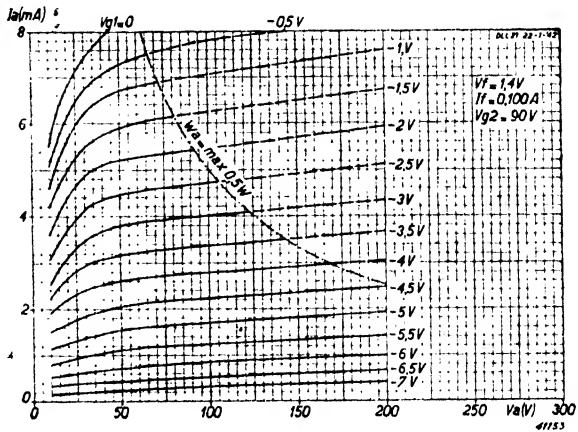
Fig. 5 Anode current of one of the sections of the DLL 21 as a function of the anode voltage, at V_{g2} = 90 V, V_f = 1.4 V and I_f = 100 mA, with V_{g1} as parameter.
