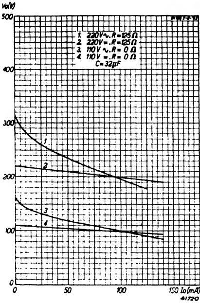
Fig. 3 Load lines for the rectifier UY 1 (N).
