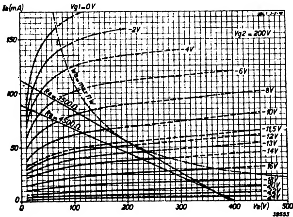
Fig. 6 Anode current as a function of anode voltage at V_{g2} = 200 V , with V_{g1} as parameter. The load lines for 9 W ( R_a = 4500 \text{ Ohms} ) and 11 W ( R_a = 3500 \text{ Ohms} ) operation are also shown.
