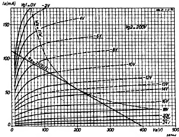
Fig. 6 Anode current as function of anode voltage at V_{g_2} = 200 V, with V_{g_1} as parameter. The load line for R_a = 3,500 Ohms is also given.
