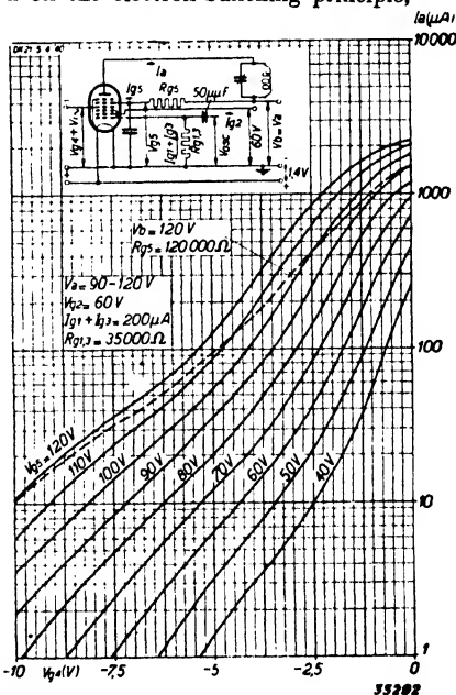
Fig. 5. Anode current as a function of grid bias at V_a = 90 - 120 \text{ V} , with the voltage of grid 5 as parameter. The broken line shows the anode current when the screen is fed from the 120 V source through a resistance of 120,000 Ohms.
