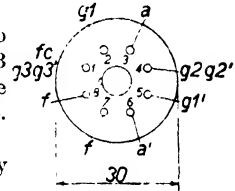
Fig. 2 Arrangement and sequence of contacts.
