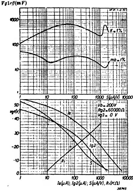
Fig. 7 At V_b = 200 V , R_{g2} = 60,000 Ohms (screen fed through a resistance) and V_{g3} = 0 V . Upper diagram; maximum permissible effective value of alternating grid voltage with 1% cross modulation ( K = 1\% ) and also 1% modulation hum ( mb = 1\% ), as function of mutual conductance. Lower diagram; Mutual conductance, anode current, screen grid current and internal resistance as function of grid bias.
