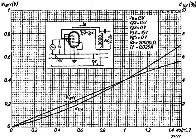
Fig. 6 Alternating input voltage and total distortion as function of power; DAH 50 used as output valve.
