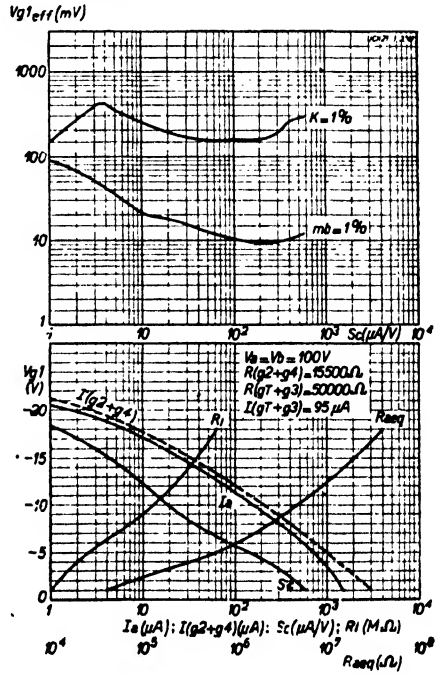
Fig. 7 At an anode or working voltage of 100 V, with screen fed through a resistance of 15,500 Ohms. Upper diagram: Highest permissible effective value of R.F. alternating voltage with 1% cross modulation ( K = 1\% ) and with 1% modulation hum ( mb = 1\% ), both in respect of the interfering signal at the grid, as a function of conversion conductance. Lower diagram: Anode current I_a , screen current I(g_2 + g_4) , conversion conductance Sc , internal resistance R_i , and equivalent noise resistance R_{aeg} as a function of grid bias V_{g1} .
