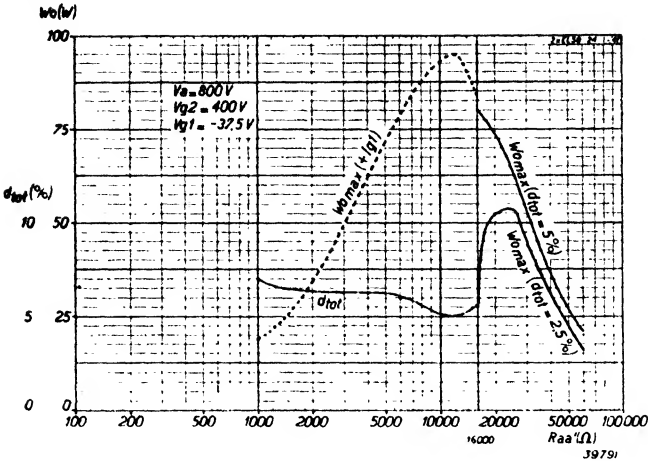
Fig. 10 Maximum output power W_0 as a function of load resistance R_{aa'} for two push-pull EL 50 valves with fixed grid bias, at V_a = 800 V, V_{g2} = 400 V, V_{g1} = -37.5 V. The broken line W_{omax} (+ I_{g1}) represents the limit to which the valves can be modulated without grid current flowing, in which case, however, the maximum anode dissipation is exceeded.
