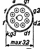
Fig. 2 Arrangement and sequence of connections.
