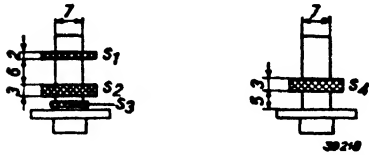
Fig. 3 Sketches of the coils
