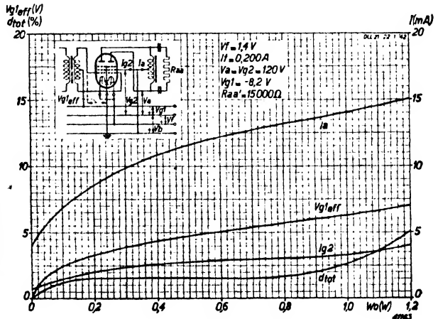
Fig. 11 Total anode current and screen current, total distortion and required alternating grid voltage per grid, as function of output power, at V_b = V_a = V_{g2} = 120 V, V_f = 1.4 V and I_f = 200 mA in class B circuit.
