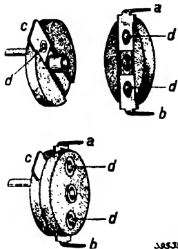
Fig. 2 Construction of a low-value differential condenser.
