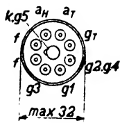
Fig. 3 Order of connection of the electrodes.
