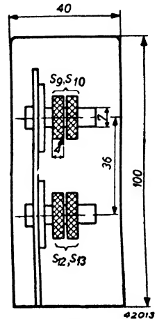
Fig. 1 Sketch of the I.F. band-filter coil unit. S_9 , S_{10} , S_{12} and S_{13} (also S_{11} in the circuit diagram) — 2 \times 155 turns of Iitz wire 24 \times 0.04 mm wound on iron cores and mounted in a Phllite box.
