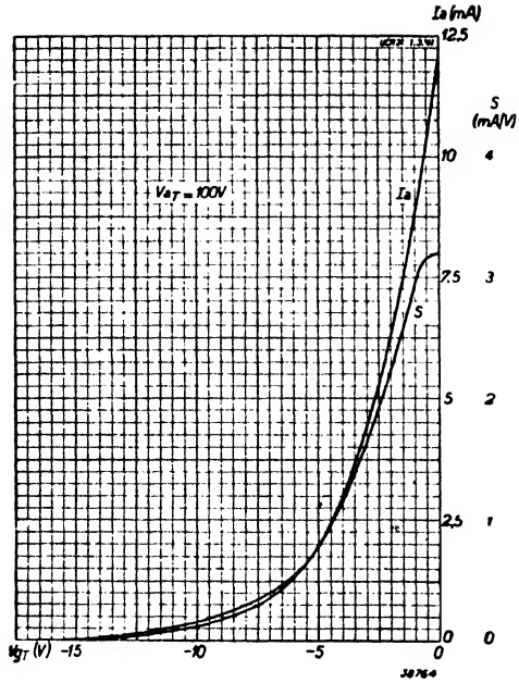
Fig. 17 Anode current and mutual conductance of the triode as function of grid bias at V_{aT} = 100 V.
