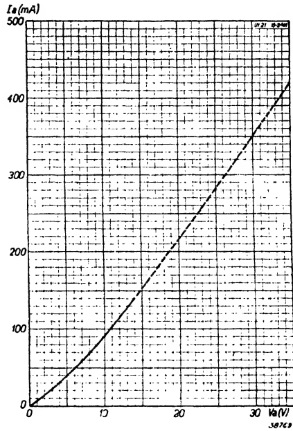
Fig. 4 Current as a function of applied direct voltage.
