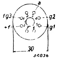
Fig. 2. Arrangement and sequence of contacts.
