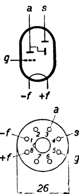
Fig. 2 Arrangement and sequence of contacts.
