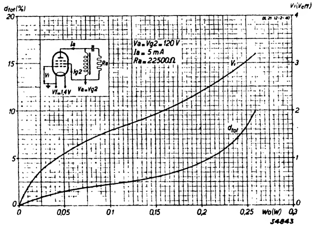
Fig. 5 Total distortion and required alternating grid voltage as function of output power at V_a = V_{g_2} = 120 V.
