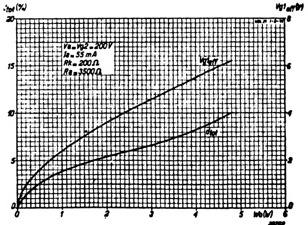
Fig. 9 Total distortion and required alternating grid voltage as a function of output power, at V_a = V_{g2} = 200\text{ V} and R_a = 3,500\text{ Ohms} .
