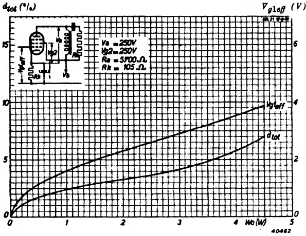
Fig. 6 Total distortion and required alternating grid voltage as a function of output power at V_a = V_{g_2} = 250 V and R_a = 5700 Ohms (11 W operation).
