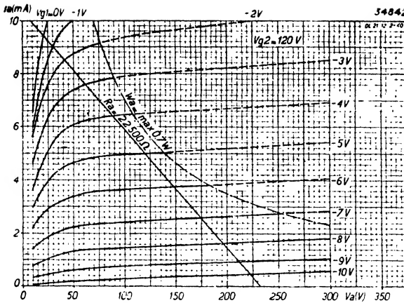
Fig. 4 Anode current as a function of the anode voltage at V_{g_2} = 120 V, with V_{g_1} as parameter.
