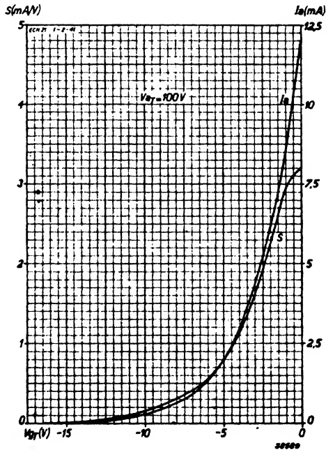
Fig. 18 Anode current and mutual conductance of the triode section as a function of grid bias, at V_{aT} = 100 V .
