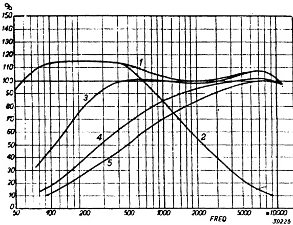
Fig. 2 Frequency characteristic of the amplifier. Curve 1; Tone controls for the high and low tones inoperative ( C_{11} in circuit). Curve 2. Tone control for the high tones ( R_{24}-C_{18} ) operative. Curve 3. Tone control for high tones inoperative, C_{21} in circuit. Curve 4. Tone control for the high tones inoperative, C_{20} in circuit. Curve 5. Tone control for the high tones inoperative, C_{11} in circuit. By means of the condensers C_{18} , C_{20} and C_{21} the lower frequencies are thus suppressed as required.
