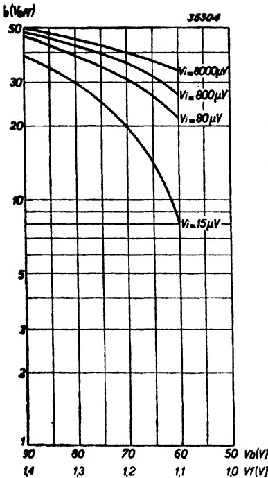
Fig. 4 Alternating output voltage as a function of H.T. battery and filament voltage in respect of different alternating input voltages, in a receiver fitted with .DK 21, DF 22, DBC 21 and DL 21 valves. Due to the compensating action of the automatic gain control, the alternating output voltage does not drop very steeply on strong input voltages. Conditions are less favourable, however, with very weak signals, below the level at which the A.G.C. operates (e.g. at V_i = 15 \mu V ).
