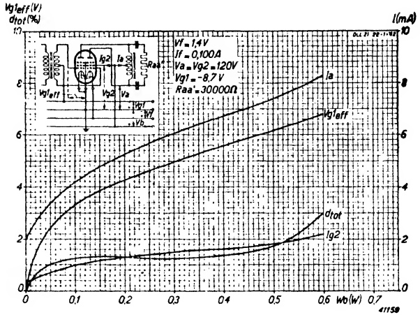
Fig. 9 Total anode current and screen current, total distortion and required alternating grid voltage per grid as function of output power, at V_b = V_a = V_{g2} = 120 V, V_f = 1.4 V and I_f = 100 mA, in push-pull circuit.
