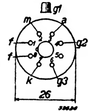
Fig. 2. Arrangement of electrodes and contacts.
