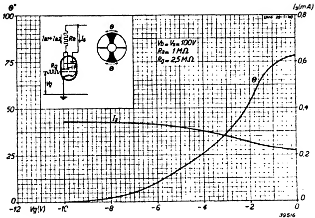
Fig. 6 Shadow angle ( \theta ) of the two sectors, and screen current I_s as a function of grid voltage, with the two anodes of the triodes fed in parallel through a 1 M Ohm resistance, on a supply of 100 V.
