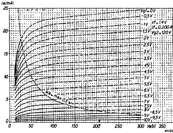
Fig. 10 Anode current of one pentode section as function of anode voltage, at V_{g2} = 120 V, V_f = 1.4 V and I_f = 200 mA, with V_{g1} as parameter.
