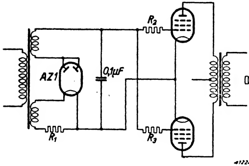
Fig. 13 Circuit employed to obtain fixed grid bias for two push-pull output valves EL 50.
