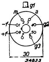
Fig. 2 Arrangement and sequence of contacts.
