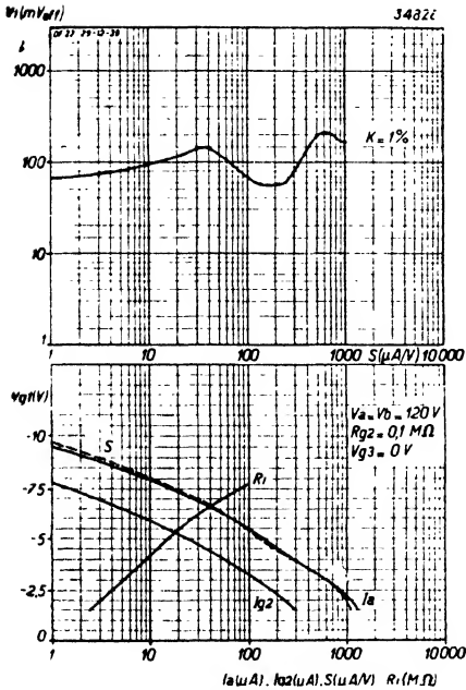
Fig. 7 Upper diagram; Effective value of alternating grid voltage as a function of mutual conductance, with 1 % cross modulation, at V_a = V_b = 120 V. Lower diagram; Mutual conductance S , anode current I_a , screen current I_{g2} and internal resistance R_i as a function of grid bias, at V_a = V_b = 120 V.
