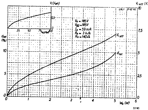
Fig. 8. Total distortion and alternating grid voltage as a function of output power at V_a = V_{g_s} = 185 V .
