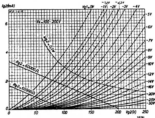
Fig. 9 Screen grid current as a function of screen voltage, with grid bias as parameter. The curves are a fair approximation in respect of all anode voltages between 100 and 200 V.
