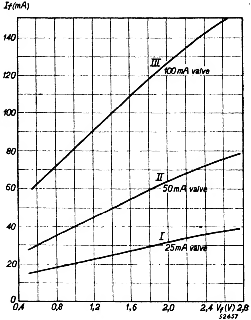
Fig. 4 Filament voltage as a function of filament current of 25, 50 and 100 mA valves.
