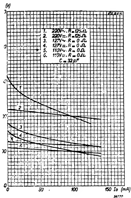
Fig. 3 Load lines for the UY 21
