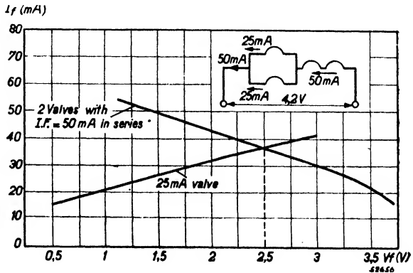
Fig. 6 Graph showing excess voltage on one of two 25 mA valves in parallel, when the filament of the other is open-circuited. DK 21—DF 21—DAC 21—DL 21 connected for feeding from a 4.2 V battery.
