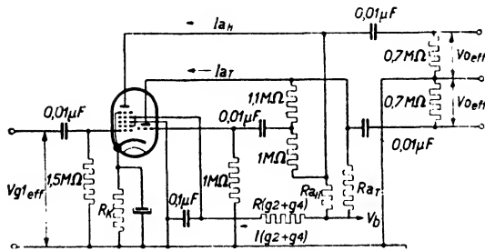
Fig. 6 Circuit diagram showing the UCH 21 employed as A.F. amplifier and phase inverter with feedback, for a push-pull output stage.
