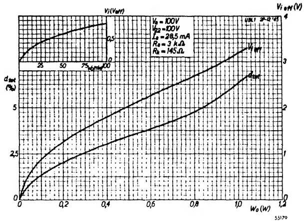
Fig. 7. Total distortion and alternating grid voltage as a function of output power at V_a = V_{g_s} = 100 V .
