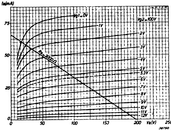
Fig. 4 Anode current as a function of anode voltage at V_{g_2} = 100 V, with V_{g_1} as parameter. The load line in respect of R_a = 3000 Ohms is also included in the diagram.
