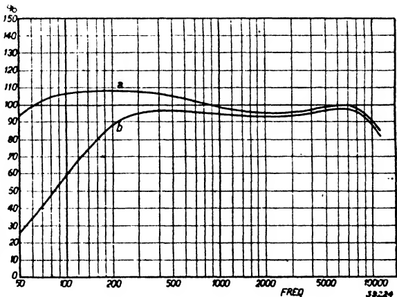
Fig. 3 Frequency characteristic of the amplifier, with condenser C_{18} inoperative (curve a) and operative (curve b). (Suppression of the low tones in microphone reproduction).
