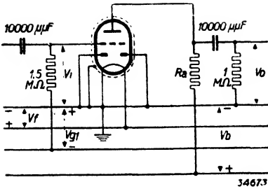
Fig. 3 Circuit diagram showing the triode section of the DBC 21 used as R.C. coupled A.F. amplifier, to illustrate the symbols employed in the Operating Data.
