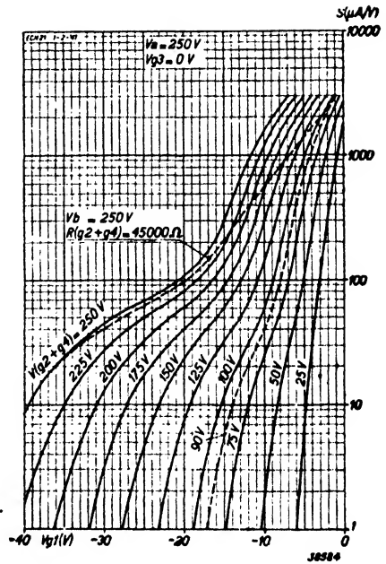
Fig. 13 Mutual conductance as a function of grid bias of the heptode section at V_a = 250 V and V_{g_3} = 0 V, with screen voltage as parameter.
