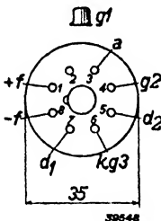
Fig. 2 Arrangement of electrodes and contacts
