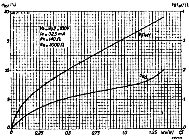
Fig. 7 Total distortion and required alternating grid voltage as a function of output power at V_a = V_{g_2} = 100 V and R_a = 3,000 Ohms.
