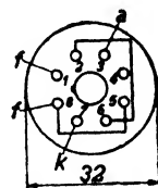
Fig. 2 Arrangement of electrodes and contacts.
