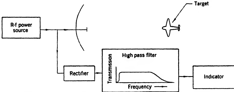
FIG. 5-1.—Simplest possible radar system, using single transmitted frequency, with modulation derived from target motion.
