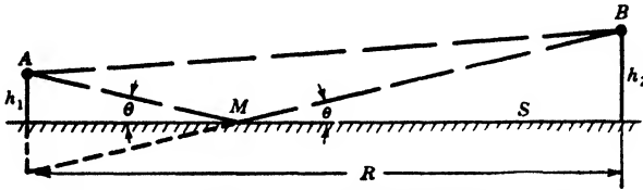
FIG. 2-9.—Propagation over a flat reflecting surface.
