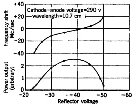
FIG. 11-23.—Reflector characteristics of the 707A.
