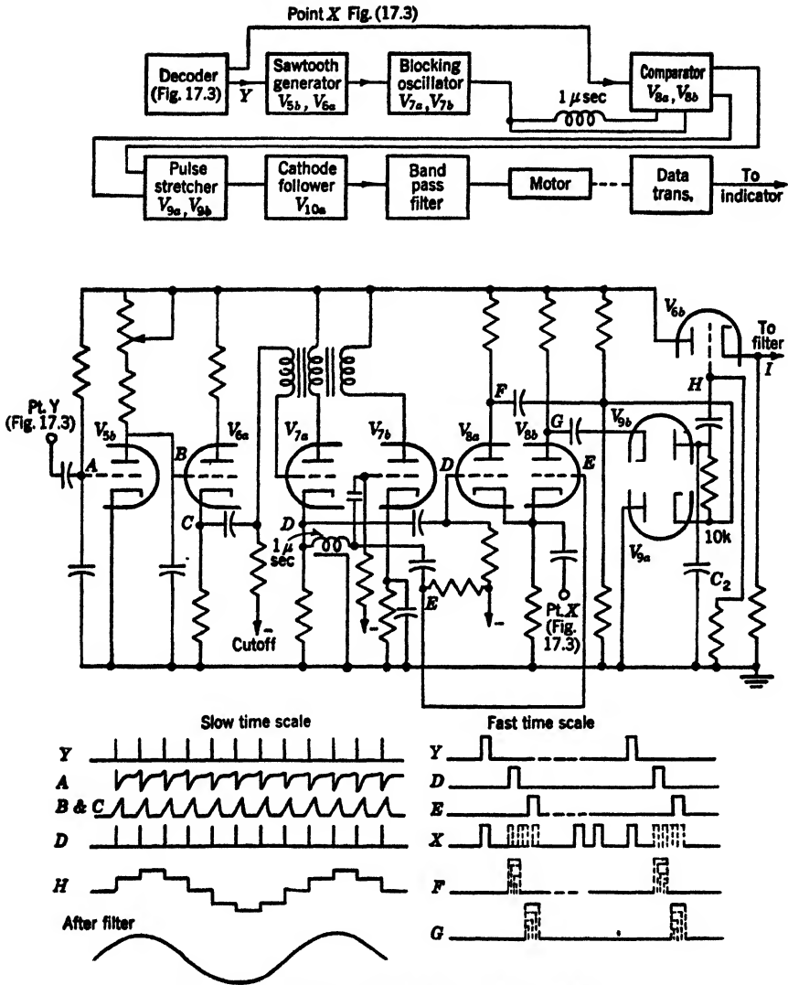
FIG. 17-5b.—Jittered-pulse system, receiving station.
