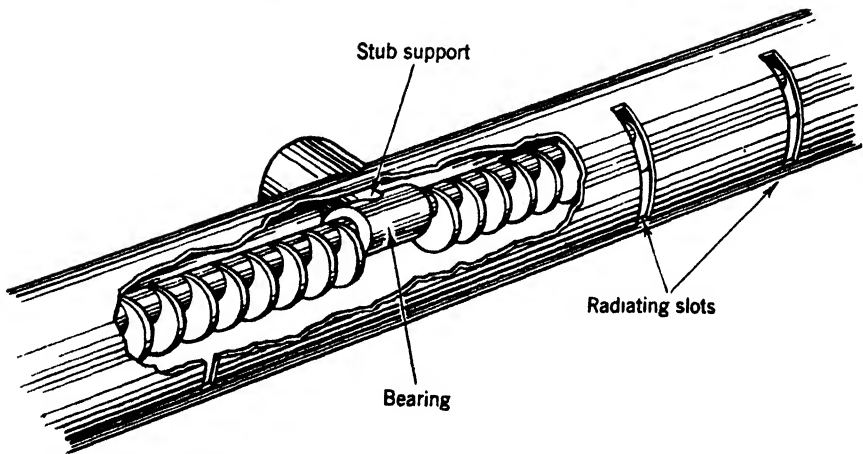
Fig. 9-33.—Cutaway section of eccentric line scanner
