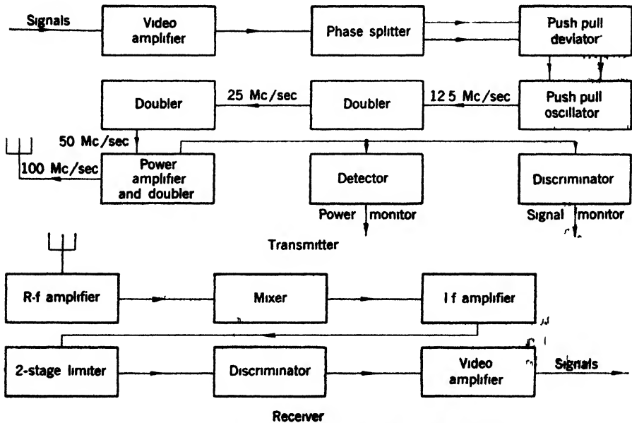
Fig. 17-18—100-Mc/sec frequency-modulated equipment
