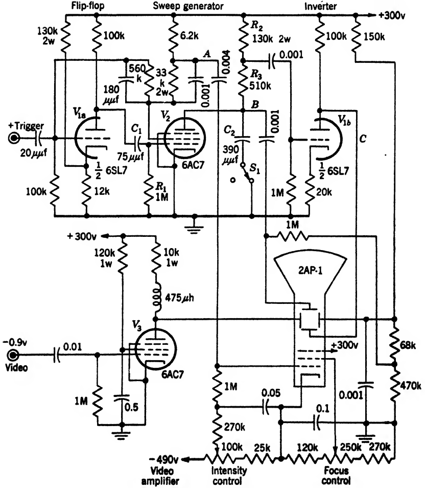
FIG. 13-41.—Simple A-scope.
