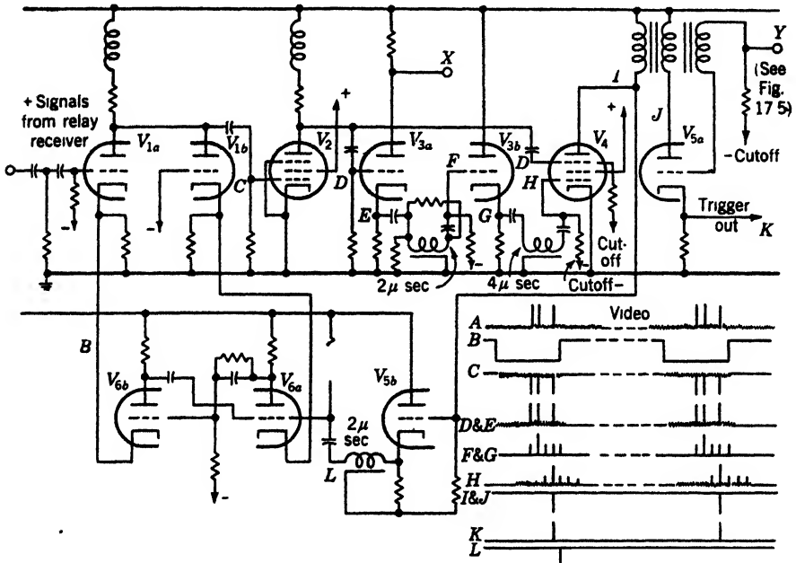
FIG. 17-3.—Interference blander and triple-pulse decoder.
