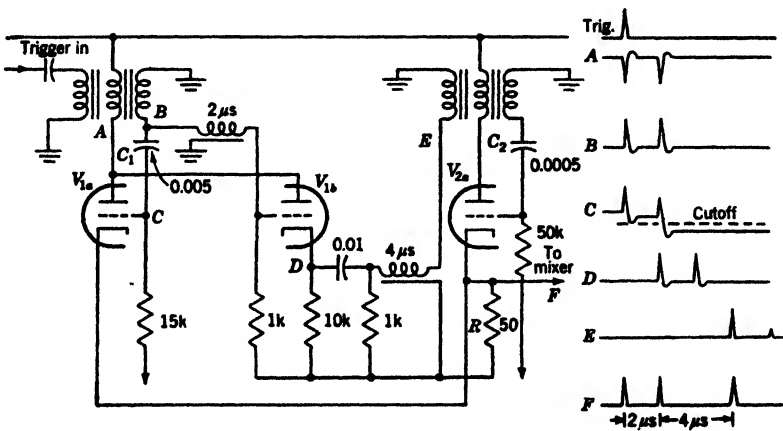
FIG. 17-2.—Triple-pulse coder.
