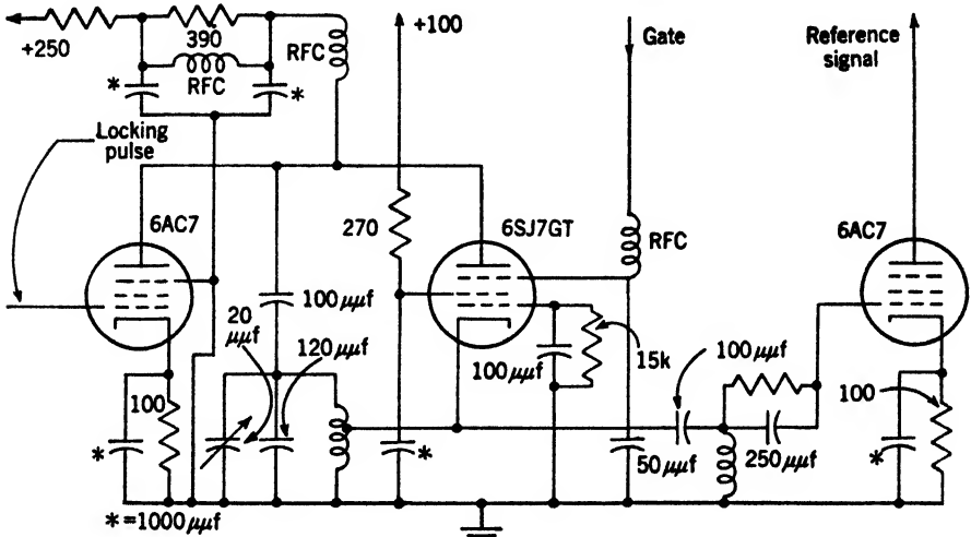
FIG. 16-27.—A typical 30-Mc/sec coherent oscillator circuit.
