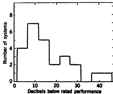
FIG. 15-3.—Radar performance survey, July 1945.
