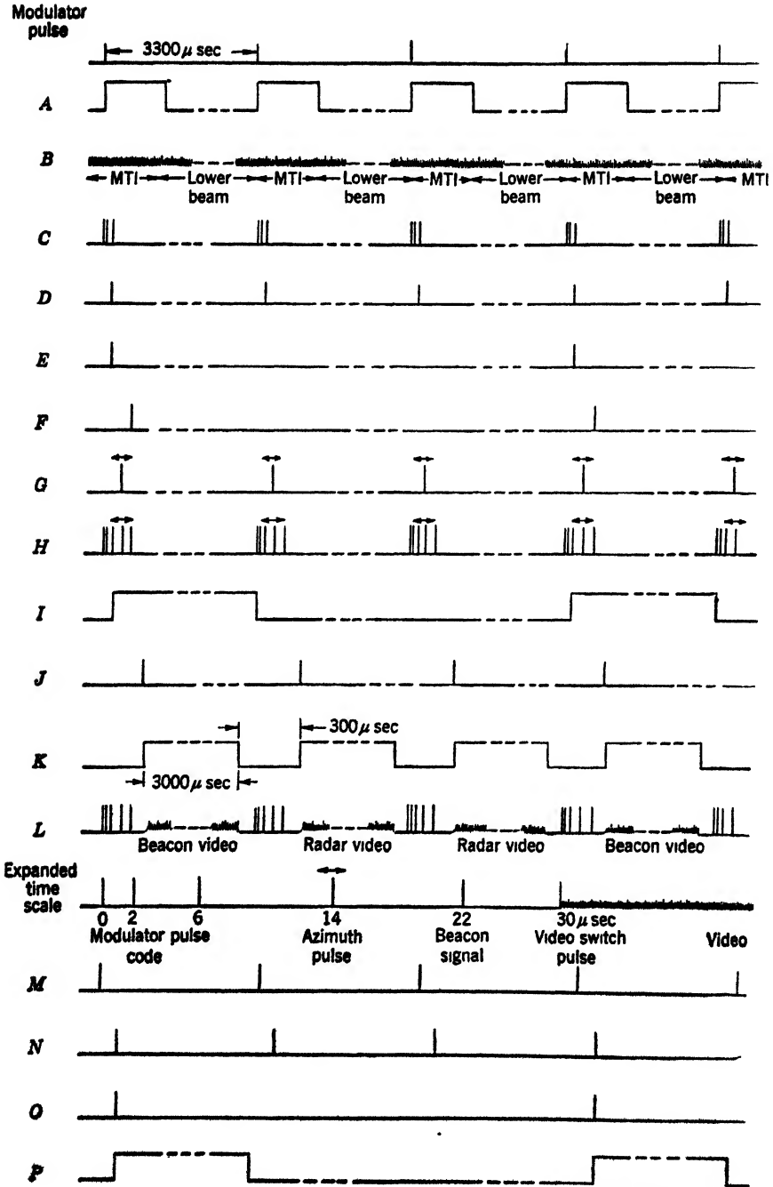
FIG. 17-20.—Ground-to-
