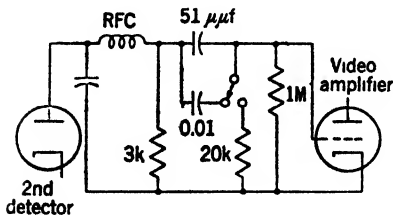
FIG. 12-14.—Fast-time-constant circuit.
