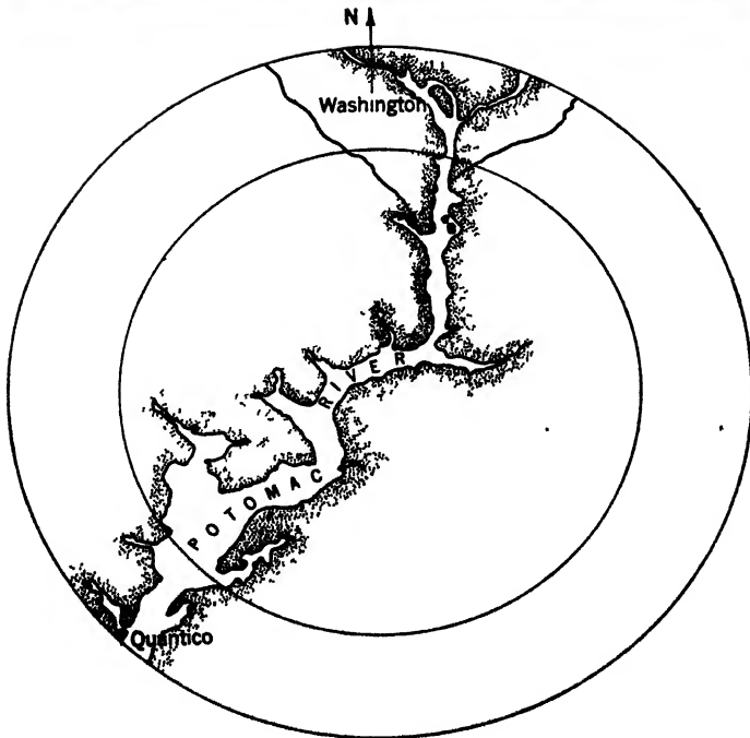
FIG. 15-11.—AN/APS-10 low-altitude PPI. Range mark at 10 miles; altitude 1600 ft., Washington, D. C. at 0°, 8 to 13 miles. (a) Photograph of scope. (b) Sketch from map. A20
