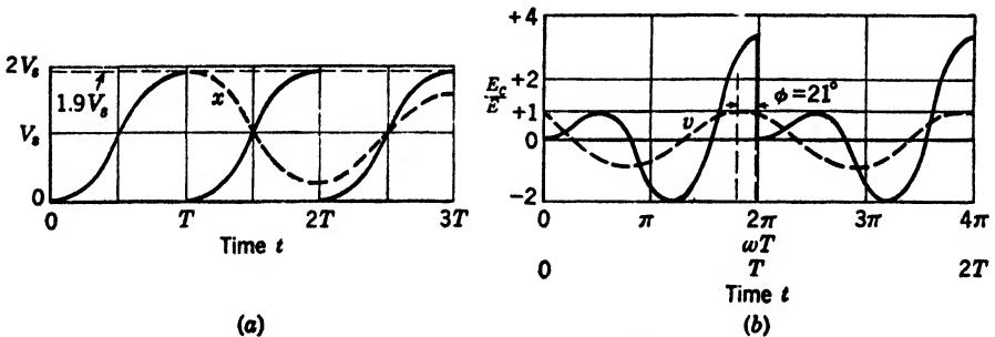
FIG. 10-44.—Line-type pulser charging waves. T = charging time; switch fires at t = T, 2T, \dots (a) Network voltage for d-c resonance charging. Power supply voltage = V_s ; pulse recurrence frequency = \frac{1}{T_r} = \frac{2}{2\pi LC} cps; curve x is network voltage if switch misfires. (b) Network voltage for a-c non-resonance charging under conditions of maximum step-up ratio. Curve v is impressed a-c voltage; v = E \cos(\omega t - \phi) .
