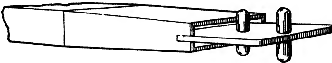
FIG 9 5—Two-dipole feed radiating toward the left
