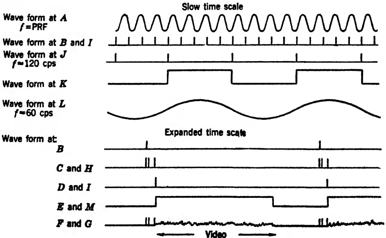
FIG. 17-4.—Simple incremental-angle synchronization.
