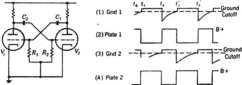
FIG. 13-13.—Eccles-Jordan multivibrator.
