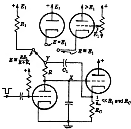
FIG. 13-31.—Bootstrap sawtooth generator. Switch indicates alternate methods.
