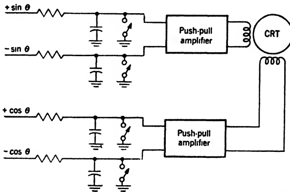
FIG. 13 51.— Pre-time-base resolution method of PPI synthesis.
