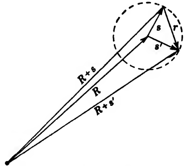
FIG. 16-23.—Moving target in clutter: clutter = R ; target = s ; target at next pulse = s' ; variation between pulses = \tau .
