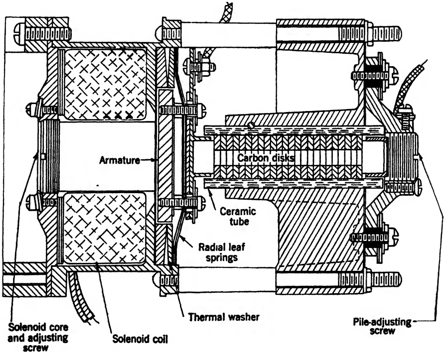
FIG. 14-9.—Cross section of carbon-pile voltage regulator.
