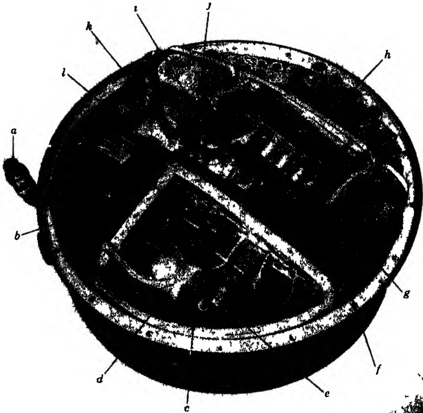
FIG 11 28 —Interior view of a 3-cm airborne r-f head, (a) pulse input; (b) pulse transformer, (c) pulse compartment, (d) pulse transformer bushing, (e) magnetron cathode bushing, (f) blower motor; (g) AFC chassis, (h) receiver chassis; (i) beacon reference cavity; (j) shield for local oscillators, (k) double mixer, (l) TR tube
