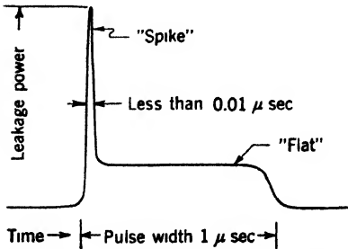
FIG. 11-16.—TR leakage power during a 1\text{-}\mu\text{sec} pulse.
