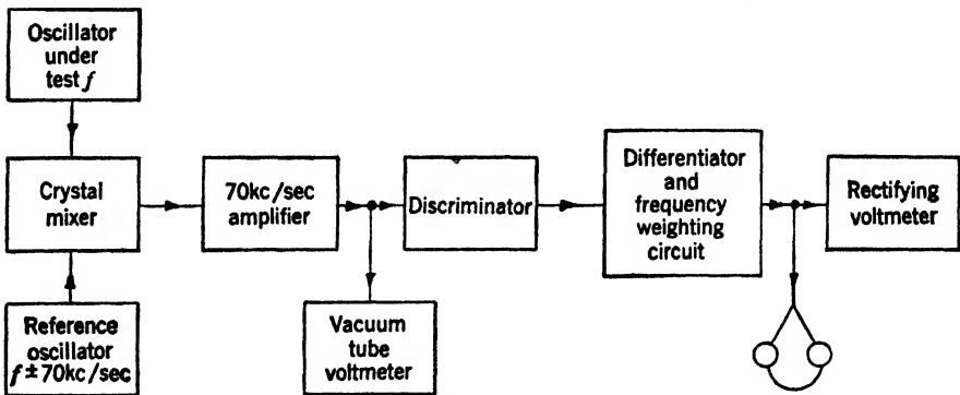
FIG. 16-36.—Block diagram of oscillator stability tester.
