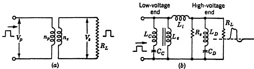
FIG. 10-45.—Pulse transformer circuit diagram.
