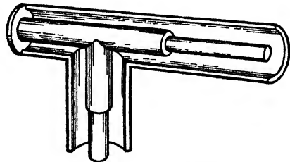
FIG. 11-4.—Stub-supported elbow.
