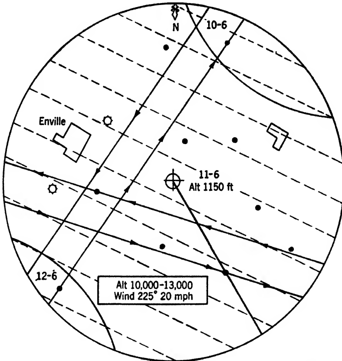
FIG. 7 18.—Schematic drawing of Teleran presentation in an aircraft flying at 11,000 ft.
