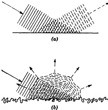
FIG. 3-16.—(a) Specular reflection. (b) Diffuse reflection.
