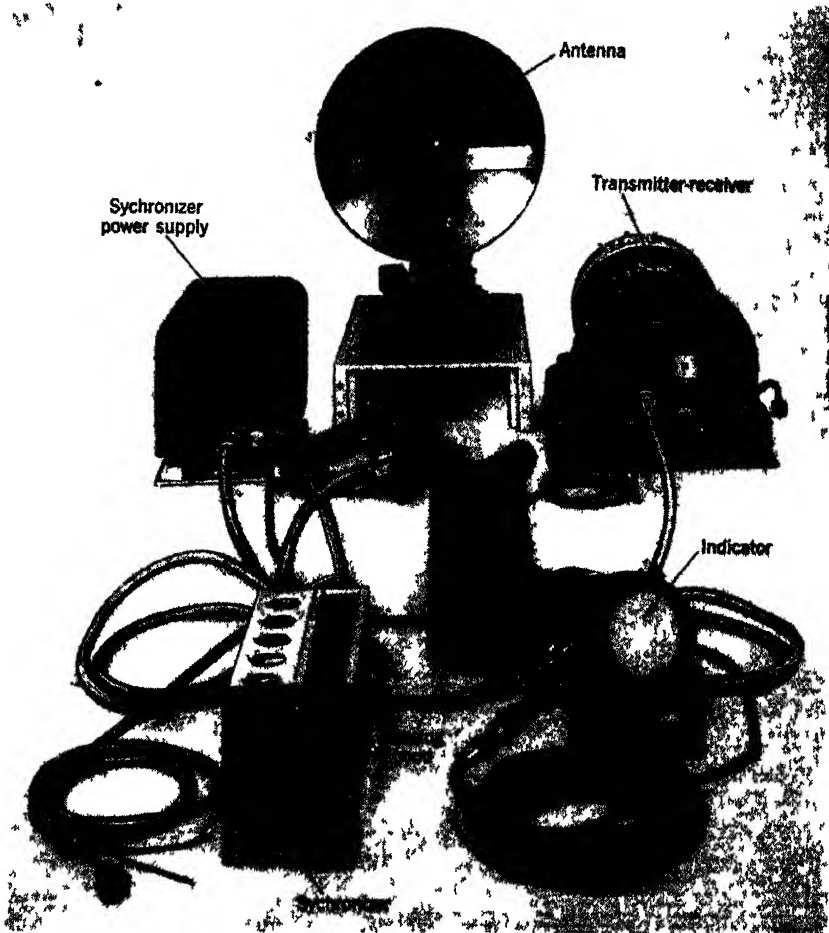
FIG. 15-9—Units of AN/APS-10
