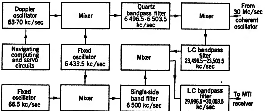
FIG. 16-28.—Block diagram of a phase-shift unit.
