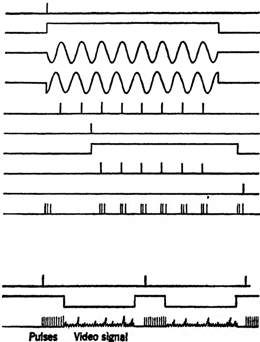
FIG. 17-8a —Phase-shifted pulses, transmitting station.
