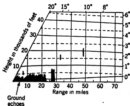
FIG. 6-23.—Range-height indicator of Type 13.
