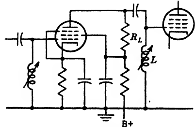
FIG. 12-6.—Single-tuned i-f amplifier.
