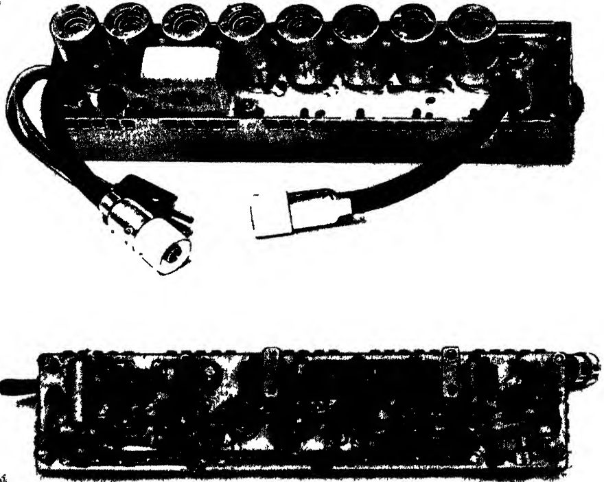
FIG 12 19 —AN/APS-10 receiver; top and bottom views.
