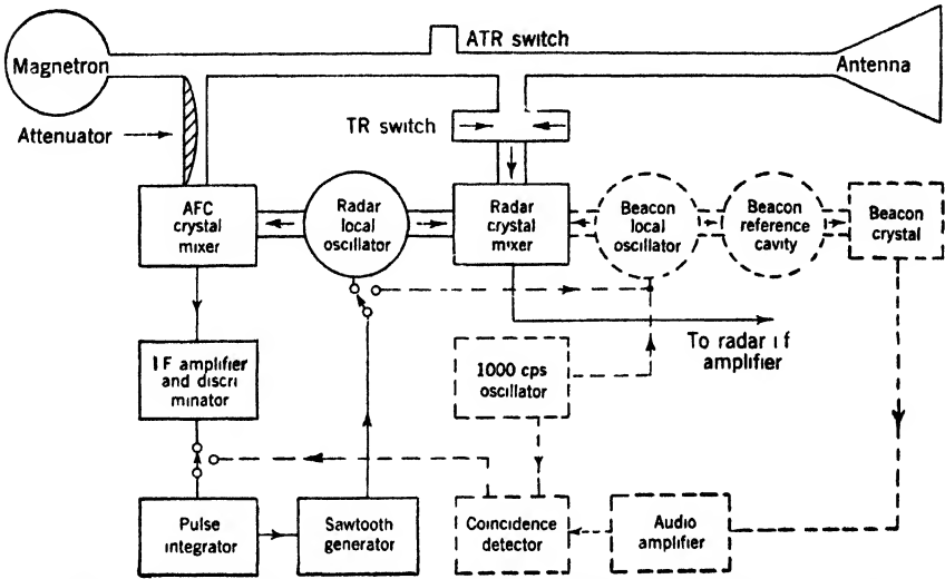
FIG. 12-12.—Block diagram of typical AFC; beacon AFC portion is shown as dotted line. in signals of proper polarity to operate a circuit which stops the sawtooth. This circuit will find the correct frequency if crossover is anywhere within the electronic tuning range of the local oscillator. Half a second is a typical period of one sawtooth search cycle.
