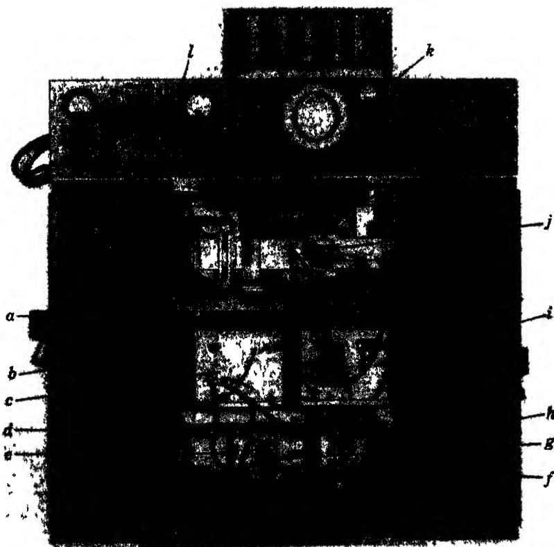
FIG 11-30—Front view of r-f head, shipborne radar: (a) pulse input; (b) transmitter compartment, search radar; (c) receiver, search radar; (d) ATR mount; (e) AFC mixer; (f) radar mixer; (g) TR-tube mount; (h) r-f switch for noise source; (i) receiver, height-finder radar; (j) duplexer, height-finder radar; (k, l) built-in control and test equipment.
