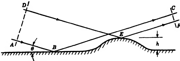
FIG. 2-13.—Reflection from an irregular surface.
