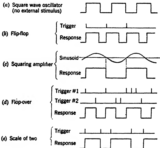
FIG. 13-12.—Response of various waveform generators.
