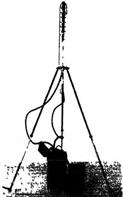
FIG. 8-6.--The AN/UPN-1, a portable battery-operated 10-cm beacon.
