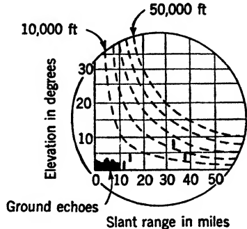
FIG. 6-10.—E-scope. Lines of equal height are shown dotted.
