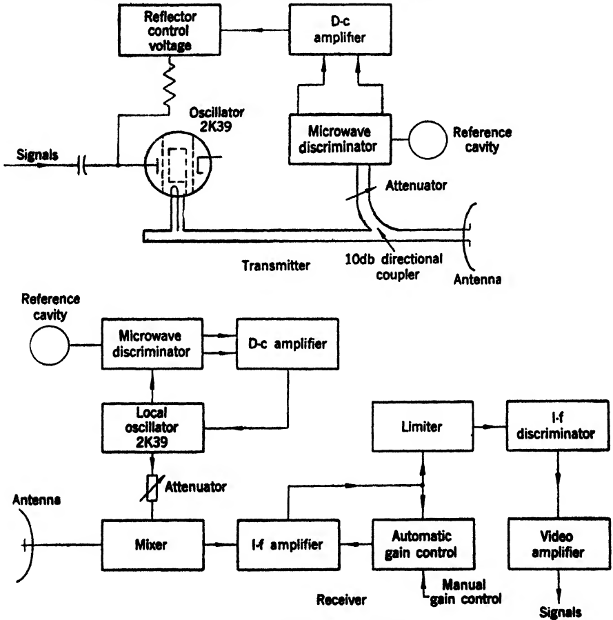
FIG. 17-19.—Microwave equipment.
