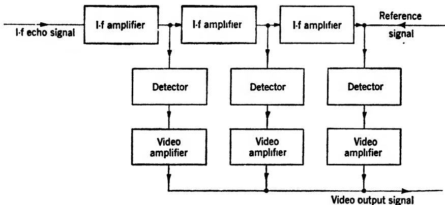
FIG. 16-29.—Circuit to give lin-log response.
