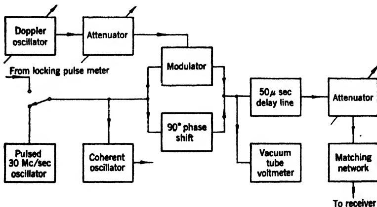
FIG. 16-37.—Subclutter visibility meter.
