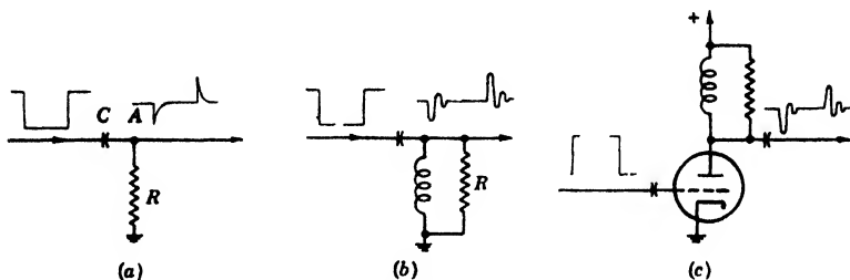
FIG. 13-18. Simple pulse-generating circuits.
