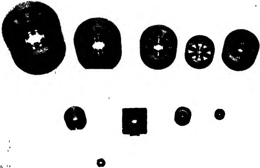
FIG. 10-19.—An array of anode blocks showing the effect of wavelength and pulse power output. Top row—10 cm, pulse power 2500 to 0.1 kw, second row—3 cm, pulse power 600 to 0.025 kw; single block—1.25 cm, 80 kw.
