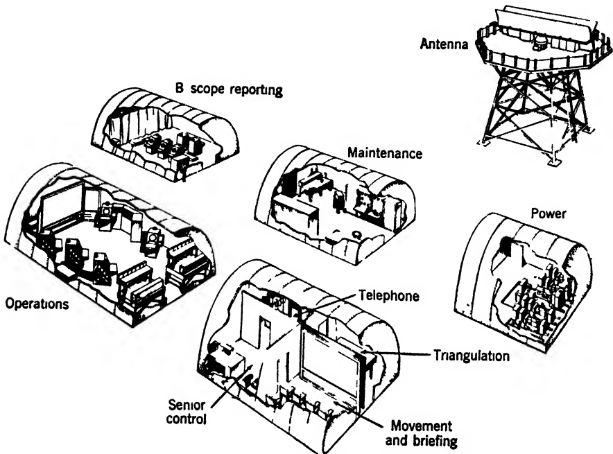
FIG. 7-11.—Layout of radar control center.
