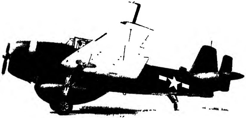
FIG 9 40 -The largest airborne radome It houses an 8-ft antenna under a TBM aircraft
