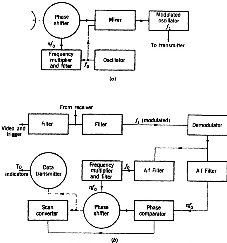
FIG. 17-7.—Phase-shift data transmission using one c-w subcarrier.
