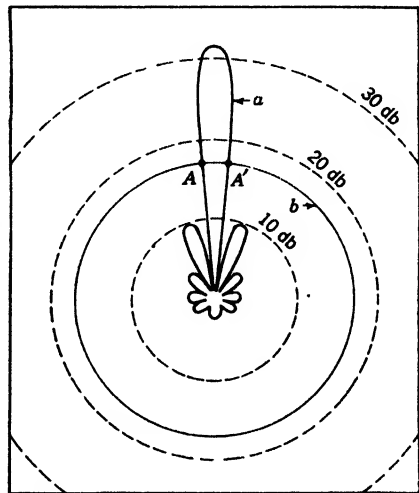
FIG. 8-7.—Schematic logarithmic polar diagram of the antenna pattern of a microwave radar. The triggering of a beacon occurs when the energy radiated in a given direction is in excess of some necessary minimum amount.
