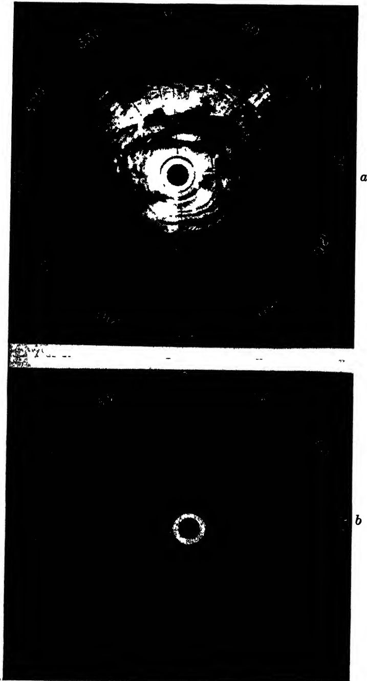
FIG. 8-2.—Radar and beacon signals of a 3-cm radar set: (a) shows only the radar echoes, (b) shows the beacon reply; both were received at nearly the same position.
