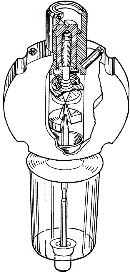
FIG. 11-17.—1B24 TR tube; 3-cm band.
