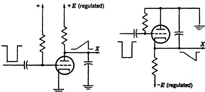
FIG. 13-30.—Sawtooth generators using triode clamps.
