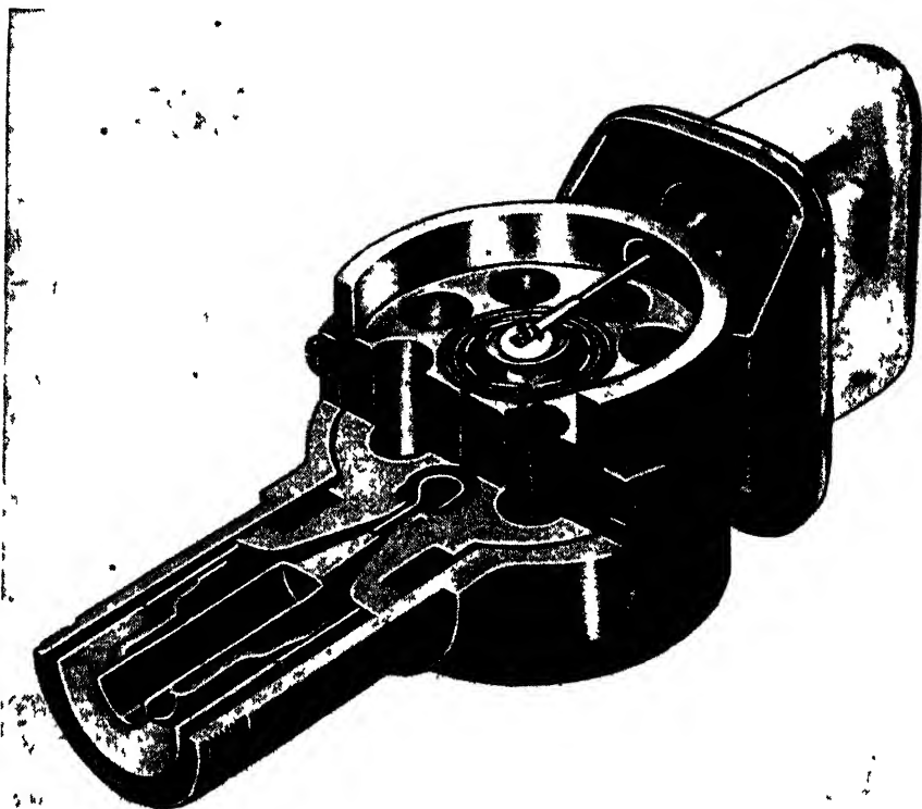
FIG. 10 20.—A high-power magnetron (type 720); 10 cm, 1000-kw pulse power output (Courtesy of Bell Telephone Laboratories)
