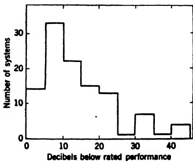
FIG. 15-2.—Radar performance surveys, 1943-1944.
