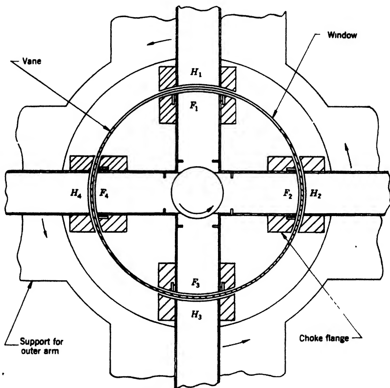
FIG. 9-27.—Four-way r-f switch used in the AN/MPG-1.
