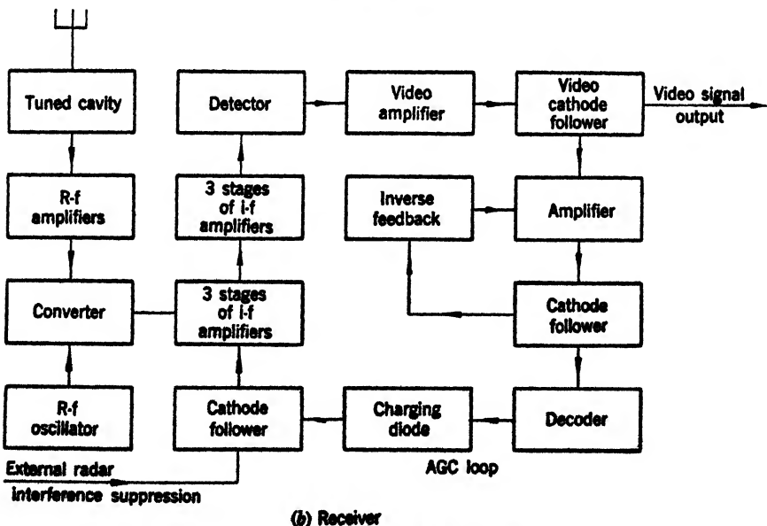
FIG. 17-17.—800-Mc/sec amplitude-modulated equipment.
