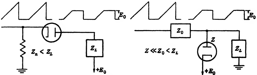
FIG. 13-21.—Diode limiters.
