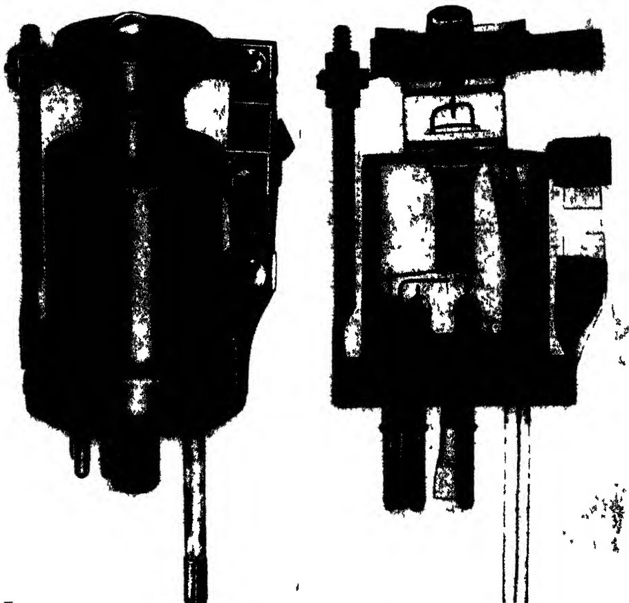
FIG 11 24 —2K25 reflex klystron, 3-cm band (a) exterior view, (b) x-ray view.
