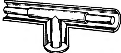
FIG. 11-3.—Broadband stub support.
