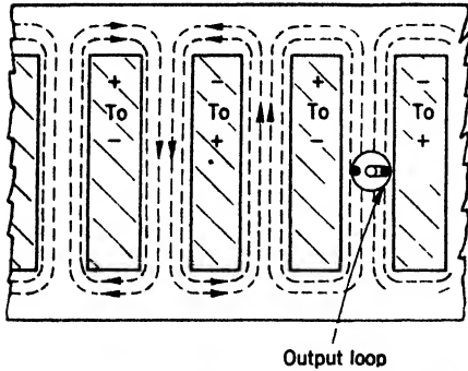
FIG. 10-7.—View from cathode of anode block opened out to show longitudinal distribution of magnetic field.
