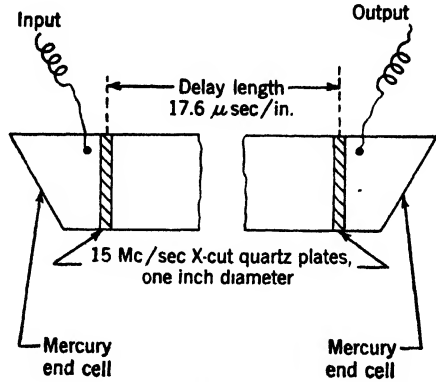
FIG. 16-10. - Laboratory-type supersonic delay line.
