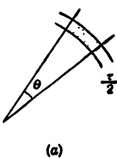
FIG. 16-18.—Composite nature of ground clutter. (a) Illuminated area of clutter. (b) Contributions to signal: fixed clutter = R_1 ; moving clutter = R_2 ; resultant signal = R ; resultant for next pulse = R' ; variation between pulses = r .
