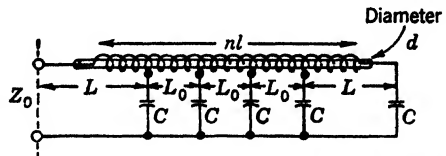
FIG. 10-37.—Type E pulse-forming network.
