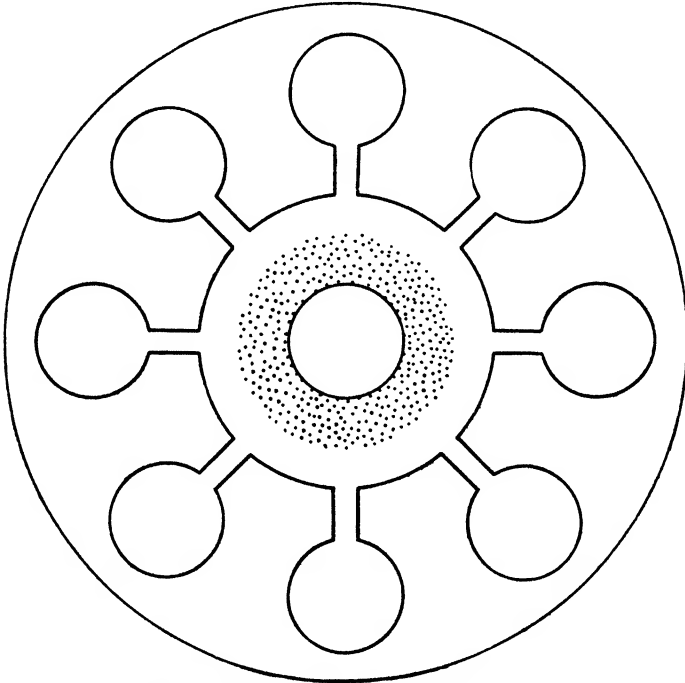
FIG. 10-14.—Space charge in nonoscillating magnetron.
