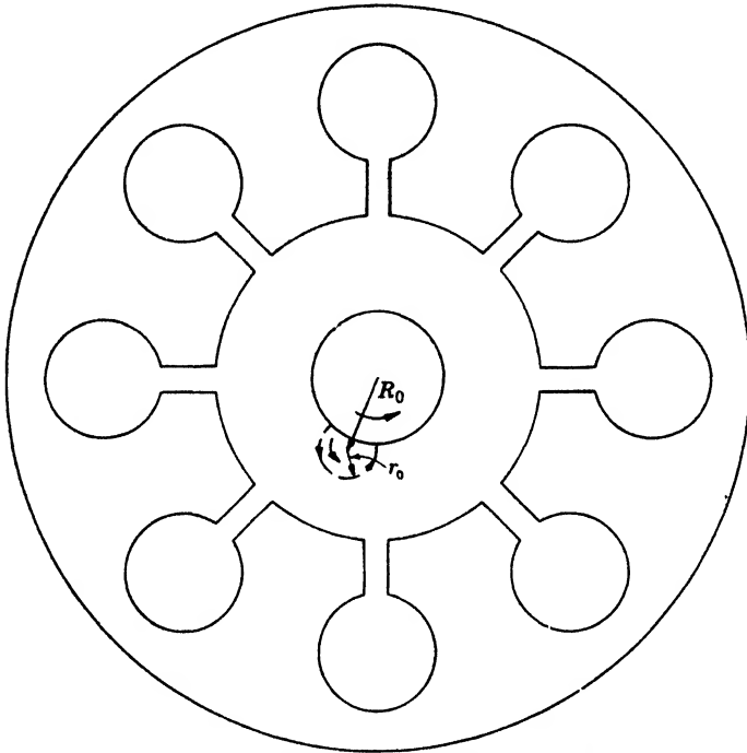
FIG. 10-11. —Path of electron in nonoscillating magnetron.
