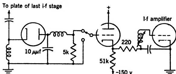
FIG. 12-15.—Instantaneous automatic gain control.
