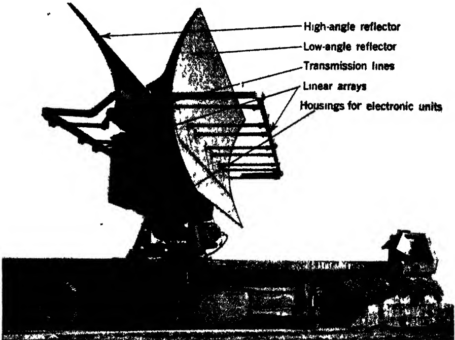
FIG. 9-15 —Long-range microwave antenna mount with two 25-ft cylindrical reflectors
