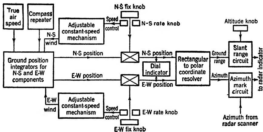
Fig. 7-3. —Simplified schematic diagram of Ground Position Indicator.
