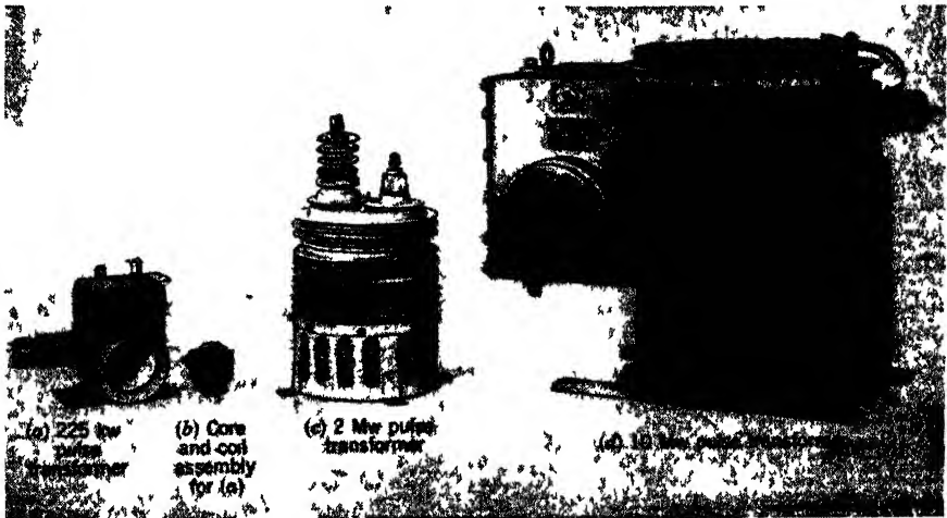
FIG 10 46 —Pulse transformers
