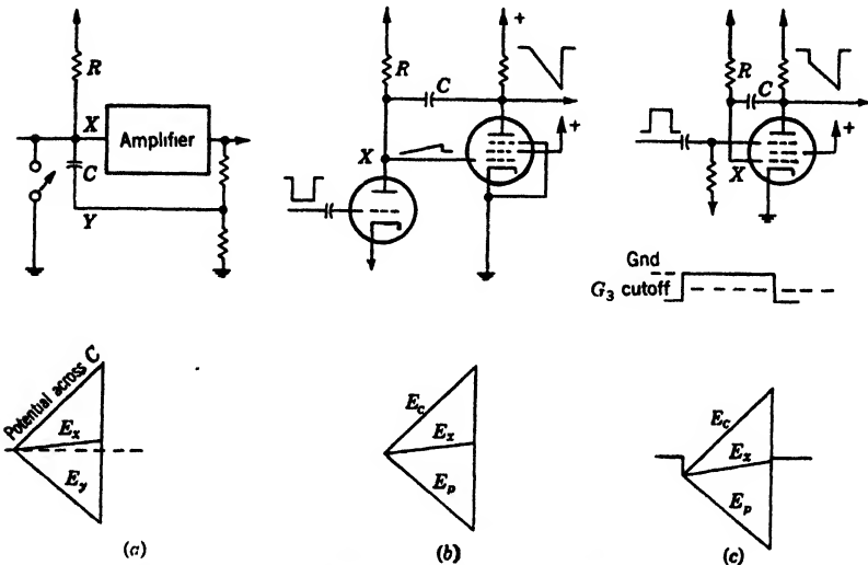
FIG. 13-32.--Sawtooth generators incorporating negative feedback.
