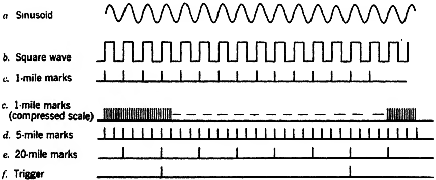
FIG. 13-37.—Derivation of pulses from c-w oscillator.
