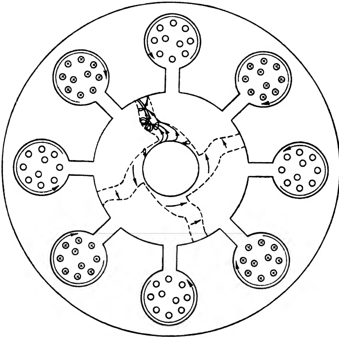
FIG. 10-15.—Space charge in oscillating magnetron.
