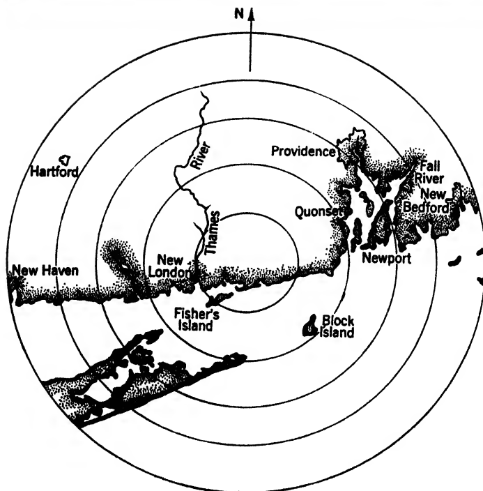
FIG. 15-12.—AN/APS-10 medium-altitude PPI. Special 30-in. antenna used. Range marks 10 miles apart; altitude 6000 ft.; Narragansett Bay at 350^\circ , 20 to 30 miles; Long Island at 160^\circ , 20 to 40 miles. (a) Photograph of scope. (b) Sketch from map.
