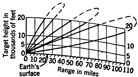
FIG. 6-19.—Typical elevation lobe pattern.
