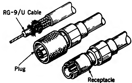
FIG. 11-7.—Coaxial cable and matched type N fittings.
