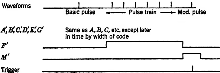
Fig. 17-8b.—Phase-shifted pulses, receiving station.
