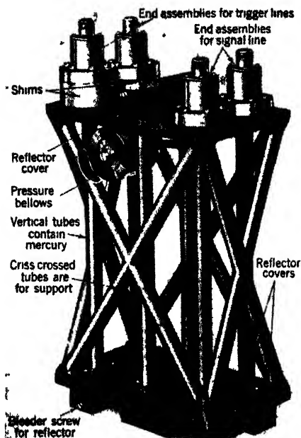
FIG 16-33—A folded mercury delay line.
