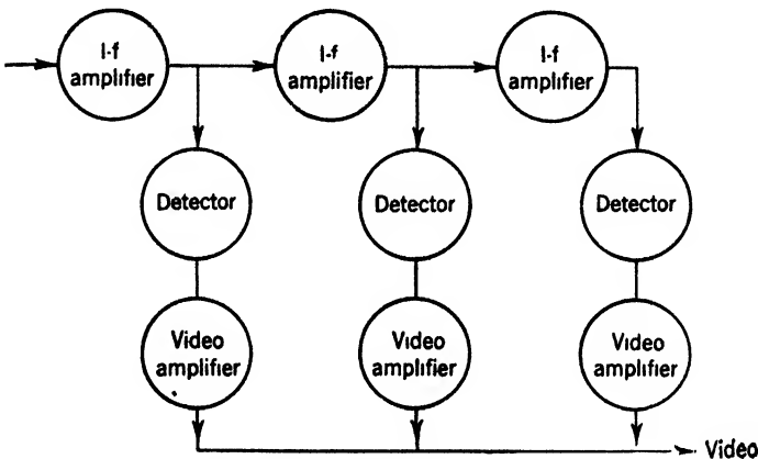
FIG. 13-56.—Logarithmic receiver.
