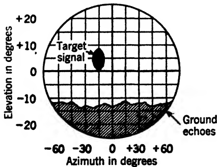
FIG. 6-11.—C-scope.
