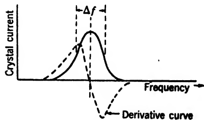
FIG. 12-13.—Beacon crystal current.
