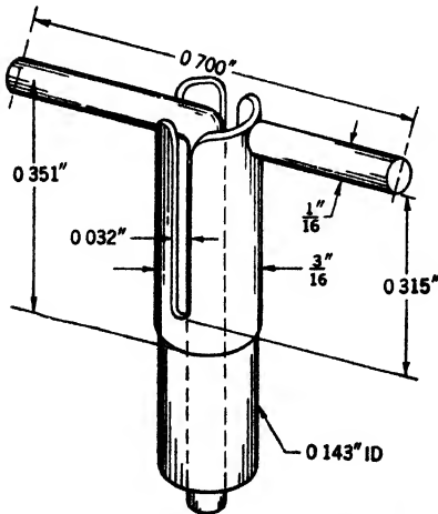
FIG. 9-22.—Construction of dipoles used in AN/APQ-7 antenna
