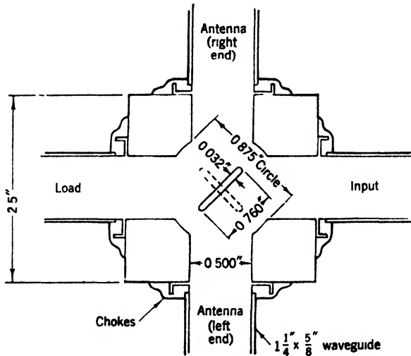
FIG. 9-24. - Detail of AN/APQ-7 r-f switch.
