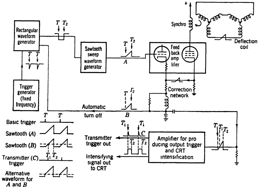
FIG. 13-48.—Resolved-current PPI using automatic transmitter triggering.
