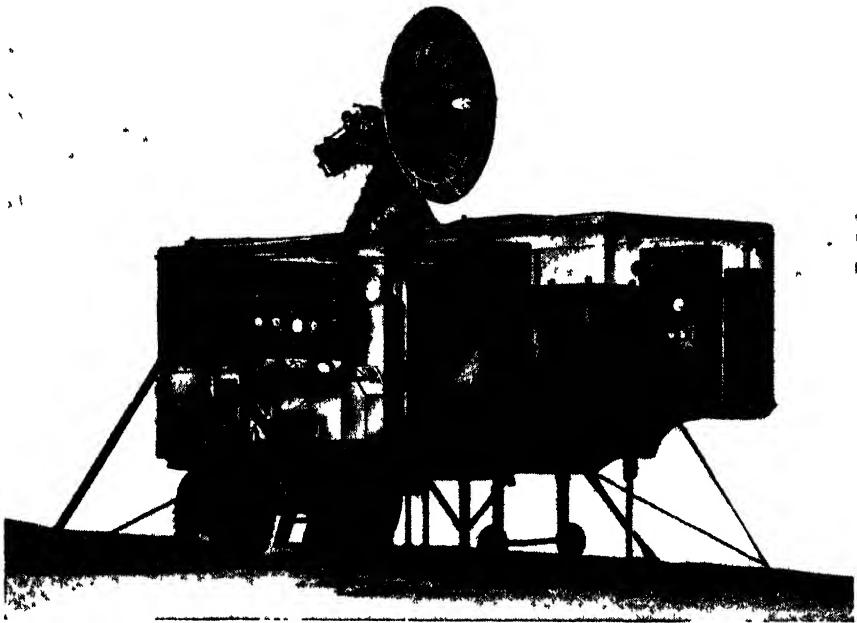
FIG. 6-37.—SCR-584 in operating position.
