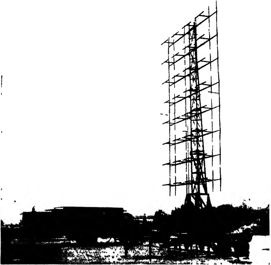
FIG 6 18 —SCR-270D.
