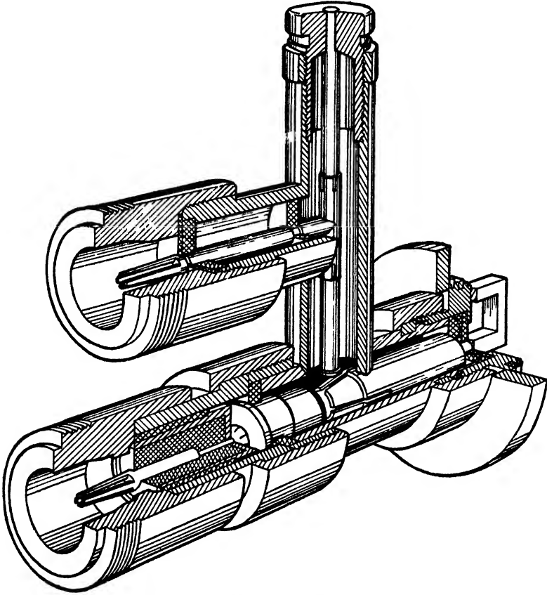
FIG. 11-25.—Coaxial-type mixer; 10-cm band.
