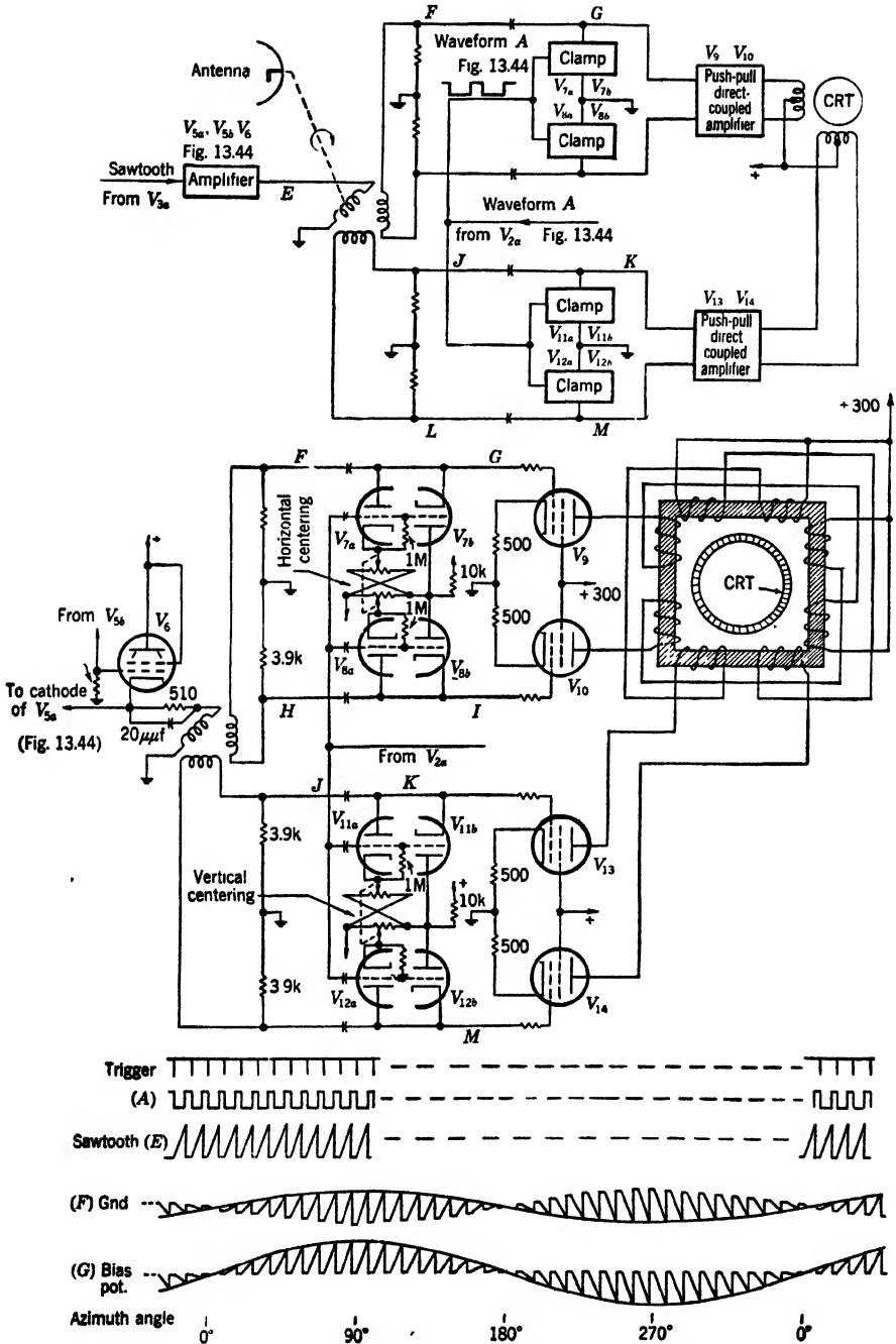
FIG. 13-46.—Resolved-sweep PPI using amplifiers.
