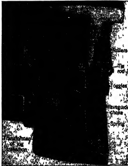
FIG 9 21 —End view of AN/APQ-7 scanner.
