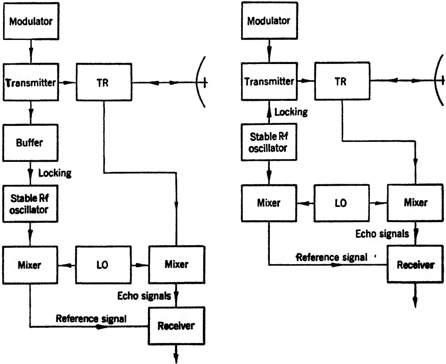
FIG. 16-15.—R-f locking, i-f addition. (a) R-f locking by transmitter, i-f addition. (b) R-f locking by oscillator, i-f addition.
