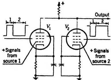
FIG. 13-28.—Switching of alternate signals.
