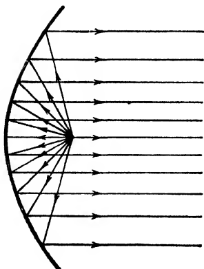
FIG. 9-2.—Ray diagram of a paraboloid antenna.
