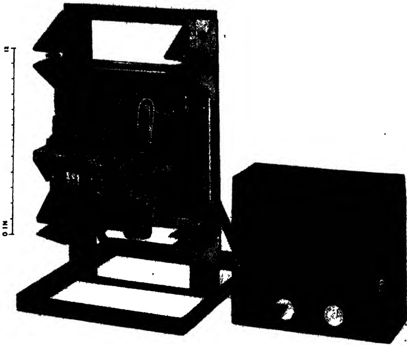
FIG. 14-7.—KS-15055 electronic voltage regulator designed by Bell Telephone Laboratories.
