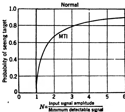
FIG. 16-22.—Probability of seeing a moving target.
