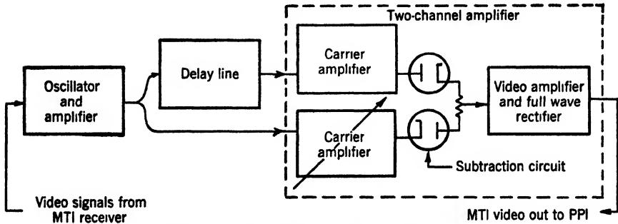
FIG. 16-11.—Block diagram of delay-line circuits.
