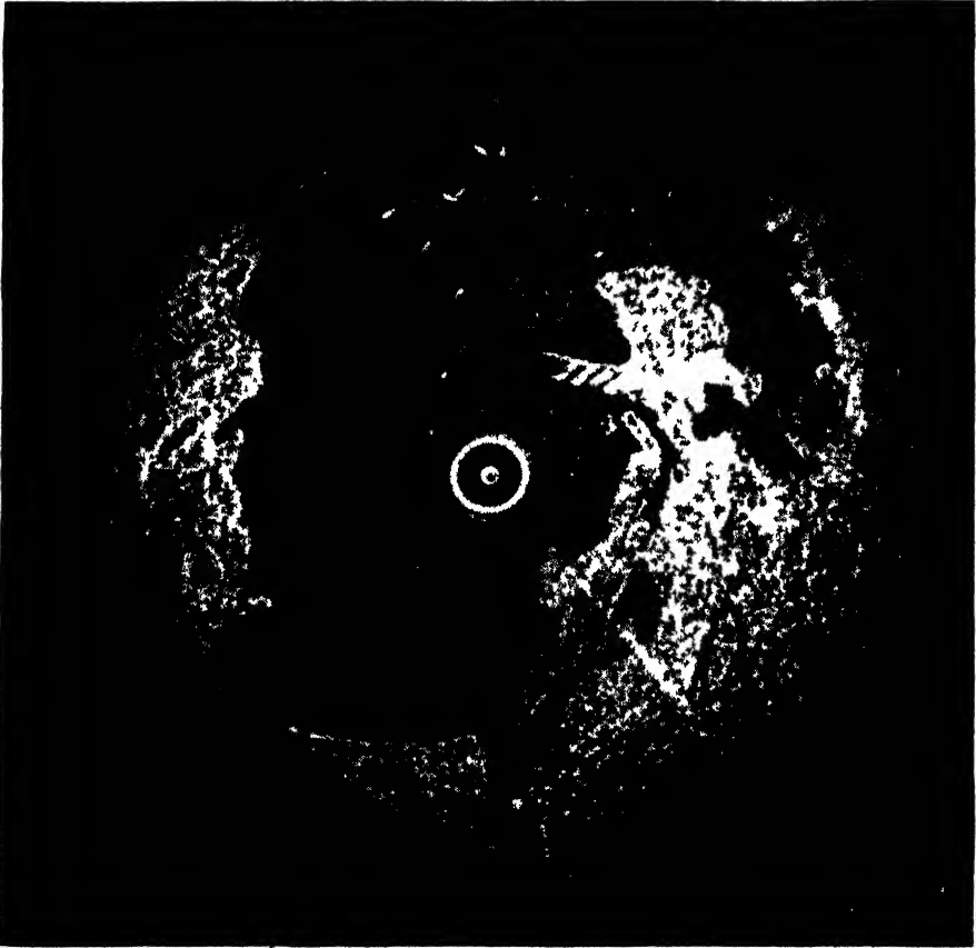
FIG. 3 22.—Atlantic entrance of the Panama Canal, with the docking facilities at Cristobal. Wavelength = 1.25 cm, 0.8^\circ beam, altitude 1500 ft, radius 3 nautical mi. 9^\circ 21' N . 79^\circ 59' W .
