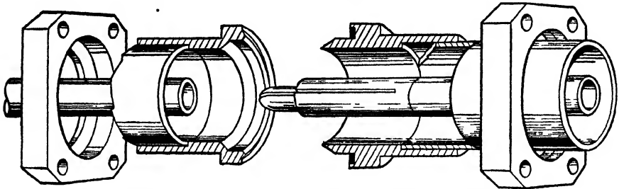
FIG. 11-5 Coupling for coaxial line
