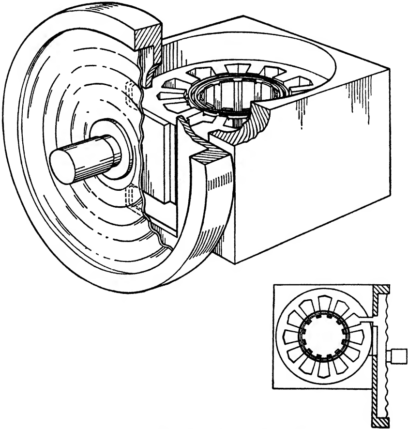
FIG. 10-23.—Magnetron with unsymmetrical tuning cavity.
