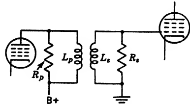
FIG. 12-7.— Double-tuned i-f amplifier.
