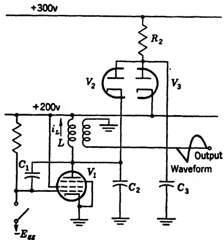
FIG. 13-49.—Balanced-waveform generator using an inductance.
