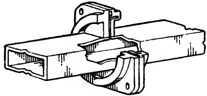
FIG. 11-10.—Waveguide choke coupling, 3-cm band.
