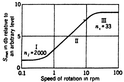
FIG. 2-8.—Effect of scanning speed on storage gain, assuming 6° beamwidth, and 4-sec storage time, with PRF = 500 pps.
