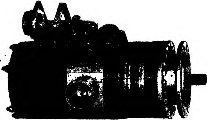
FIG. 14 2 —Eclipse NEA-7 dual-voltage generator
