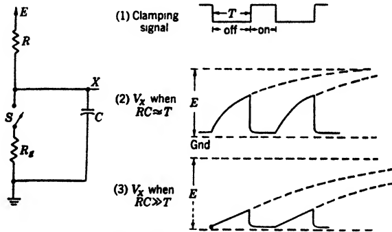
Fig. 13-29.—Basic sawtooth generator.
