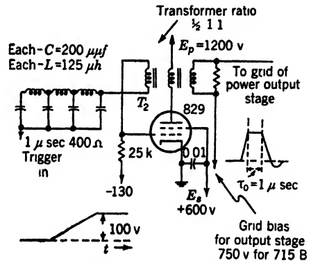
FIG. 10-33.—Schematic diagram of regenerative pulse generator used as driver of hard-tube pulser.
