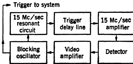
FIG. 16-12.—Trigger generator:
