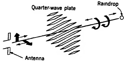
FIG. 3-13.—Scheme for reduction of rain echo.
