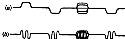
FIG. 16-17.—Effect of detuning the coherent oscillator. (a) Oscillator in tune with i-f signals. (b) Oscillator detuned.
