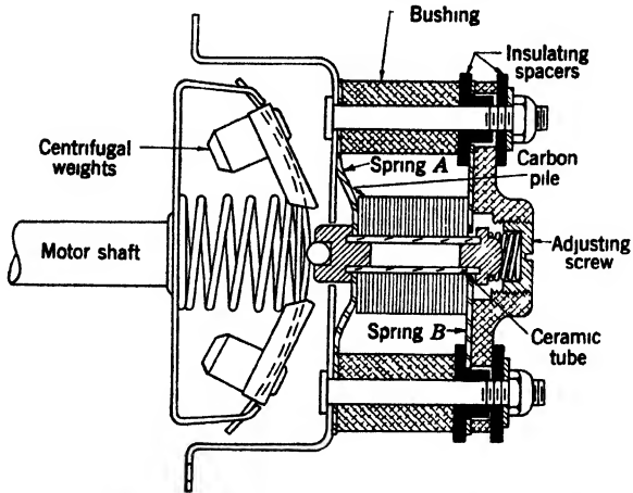
FIG 14 20 —Holtzer-Cabot Electric Company carbon-pile speed governor
