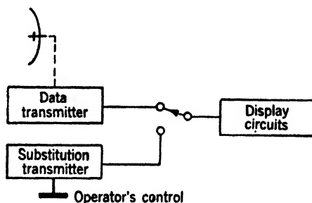
FIG. 13-35.—Substitution method for movable angle index.
