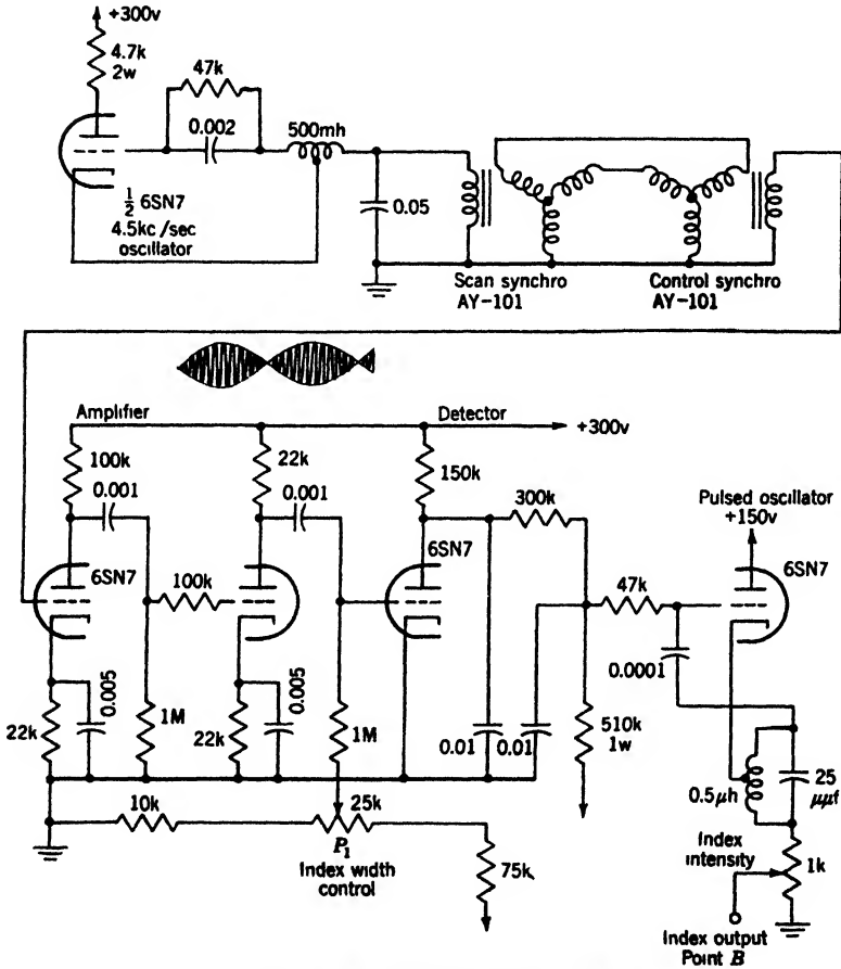
FIG. 13-34.—Synchro null indices.
