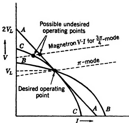
FIG. 10-28.—Pulsar and magnetron voltage-current characteristics. (a) line-type pulser load line, (b) hard-tube pulser (adequate emission available), (c) hard-tube pulser near saturation.
