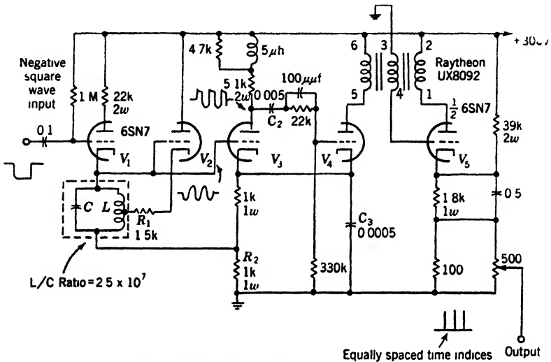
FIG. 13-38.—Switched generator for multiple time indices.
