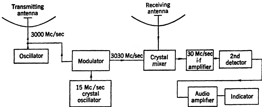
FIG. 5-5.—Block diagram of simple doppler-type radar system.
