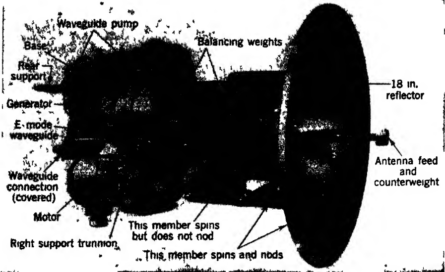
FIG 9-17—The AN/APS-6 spiral scanner (Courtesy of Dalmo Victor Manufacturing Company)
