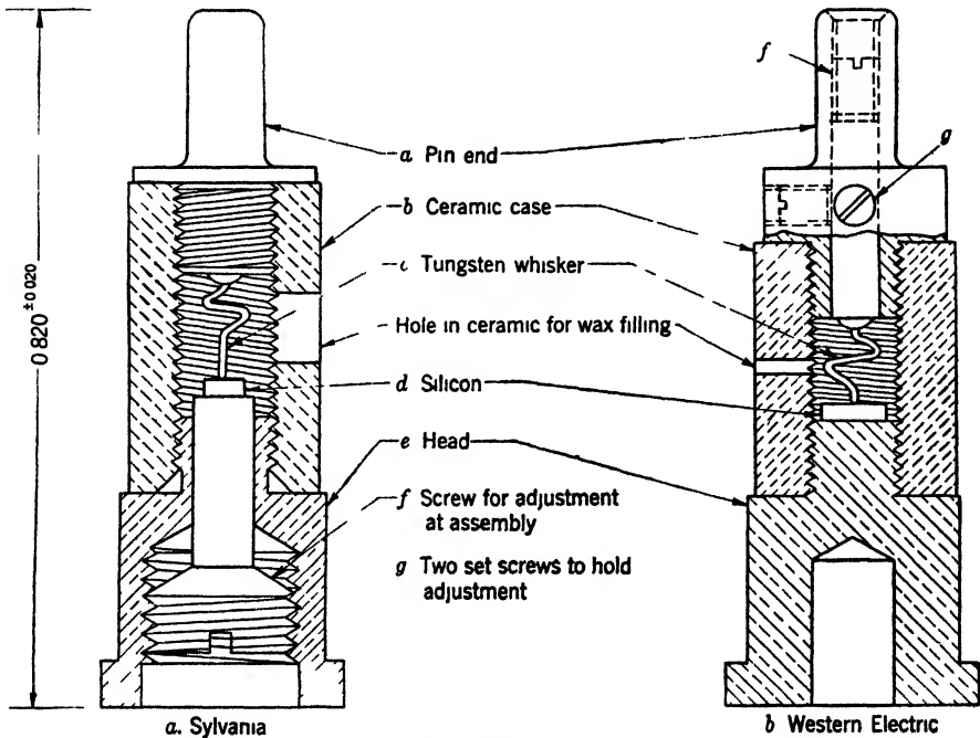
FIG. 11-19.—Microwave mixer crystals.
