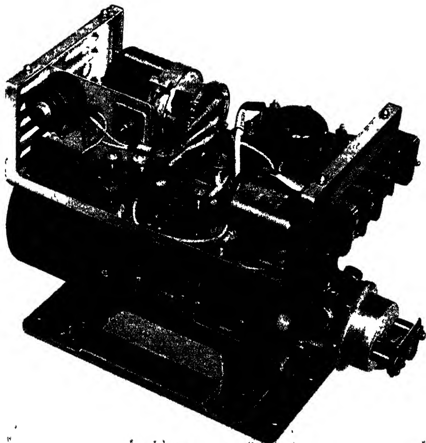
motor-alternator with Holtzer-Cabot speed control.
