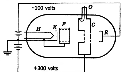
FIG. 11-22.—Schematic of reflex klystron.
