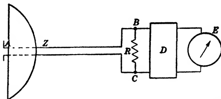
FIG. 2-3.—Schematic diagram of an ideal receiving system.
