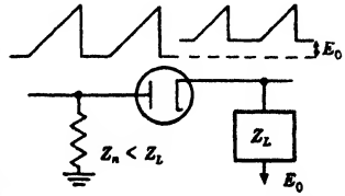
FIG. 13-22.—Bottom clipper (biased diode “pick-off” circuit).
