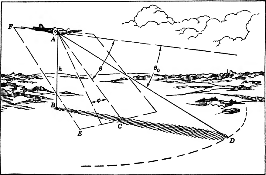
FIG. 2-2.—The problem of the ground-mapping antenna.
