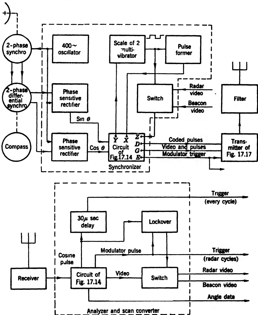
FIG. 17-22.—Air-to-surface relay system.
