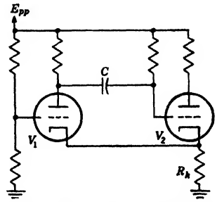
FIG. 13-16.—Cathode-coupled flip-flop circuit.
