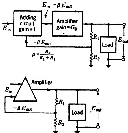
FIG. 13-10.—Negative feedback principle.
