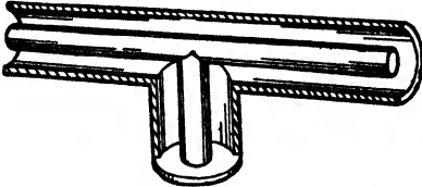
FIG. 11-2.—Simple quarter-wave stub support.
