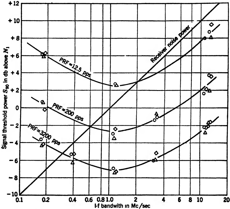
FIG. 2-5.—Signal threshold vs. i-f bandwidth for a pulse duration of 1 \mu sec. The signal power is measured in units of the noise power, N_1 , within a band 1 Mc/sec wide. In these experiments the video bandwidth was 10 Mc/sec, the signal presentation time was 3 sec, and the length of the pulse on the screen of the A-scope was 1.7 mm.
