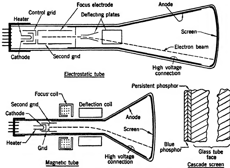
FIG. 13-1.—Elements of cathode-ray tube.
