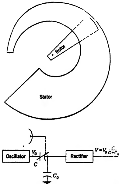
FIG. 13-7.—Special variable condenser.
