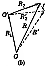
FIG. 16-18.—Composite nature of ground clutter. (a) Illuminated area of clutter. (b) Contributions to signal: fixed clutter = R_1 ; moving clutter = R_2 ; resultant signal = R ; resultant for next pulse = R' ; variation between pulses = r .
