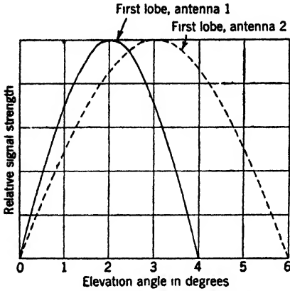
FIG. 6-20.—Elevation coverage diagram.
