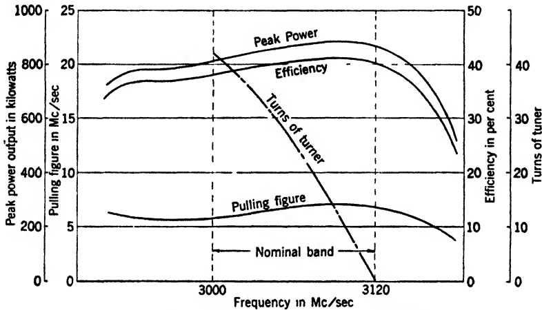
FIG. 10-24.—Characteristics of the 4J70 series.
