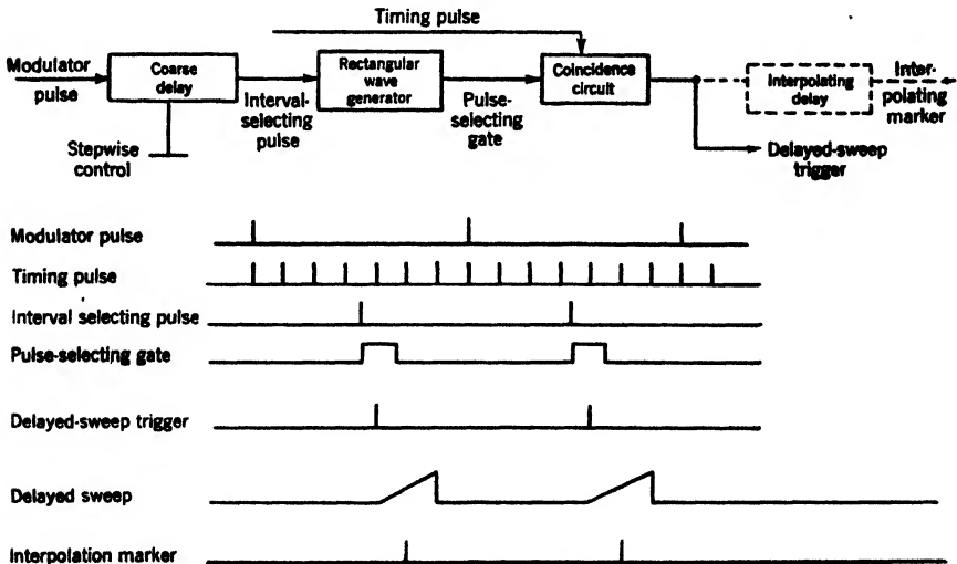
FIG. 13-40.—Discrete sweep delay.
