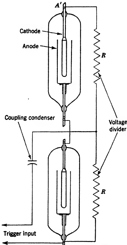
FIG. 10-39.—Series gaps.
