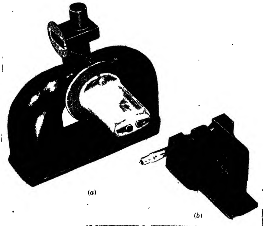
FIG. 10-4.—Two types of magnetron construction: (a) radial cathode and separate magnet; (b) axial cathode with attached magnet.
