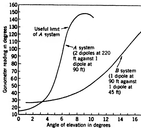
FIG. 6-17.—Height curves for CH station. Wavelength = 13.22 meters.
