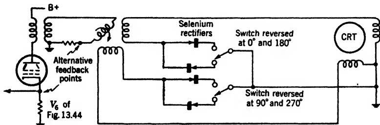
FIG. 13-47.—Resolved-current PPI using switched rectifiers.
