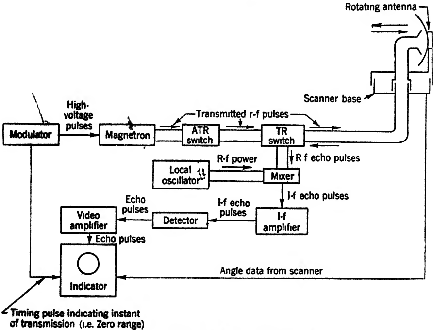
FIG 1 4.—Block diagram of a simple radar.
