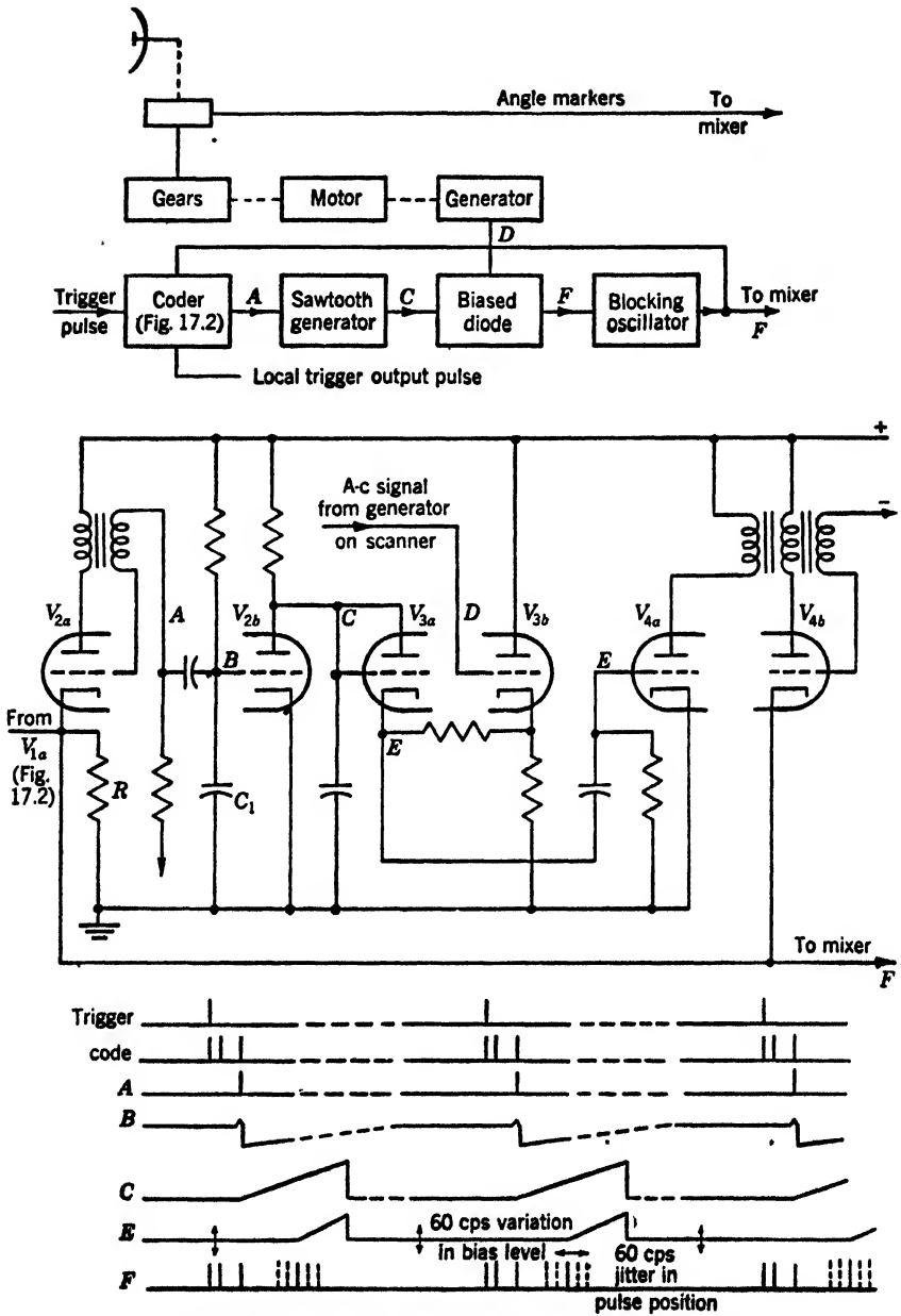
FIG. 17-5a.—Jittered-pulse system, transmitting station.
