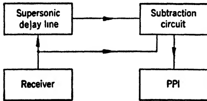
FIG. 16-8.—Cancellation of signals of constant pulse-to-pulse phase.
