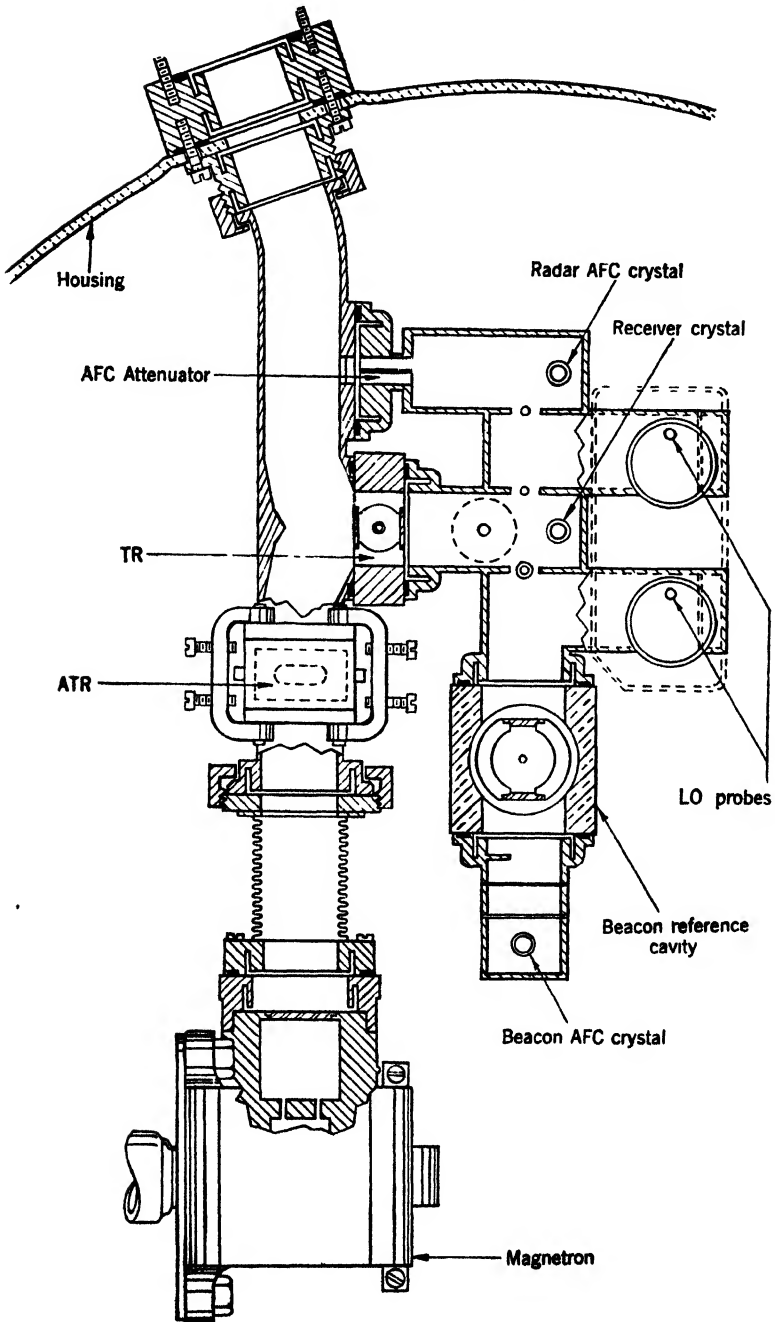
FIG. 11-29.—R-f system.
