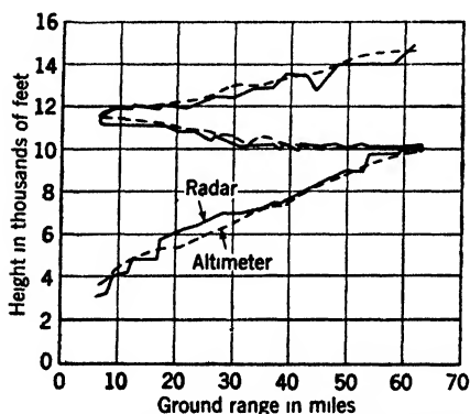
FIG. 6-24.—Calibration of height readings of AN/TPS-10.
