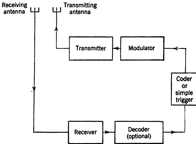
FIG. 8-1.—Block diagram of a beacon.
