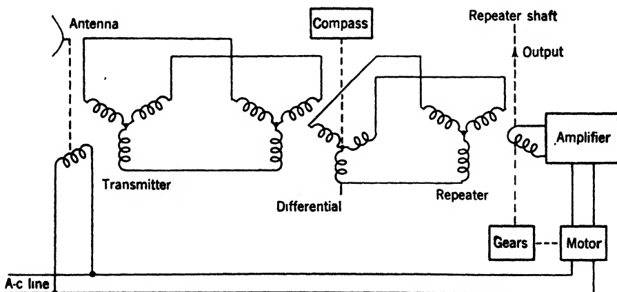
Fig. 13-9.—Servo system including compass-driven differential.
