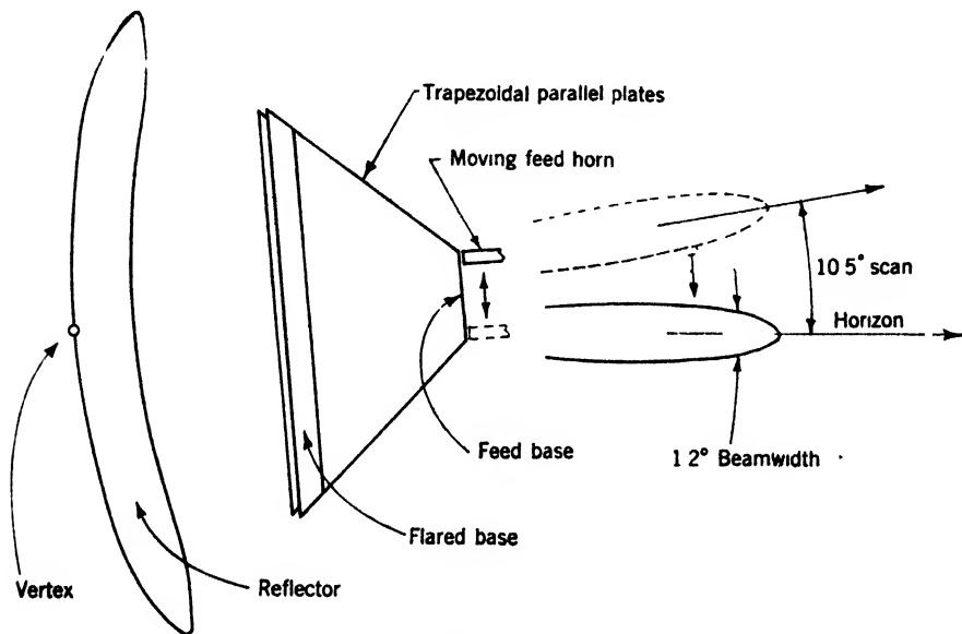
FIG. 9-29. —Simplified SCI height finder, side view.
