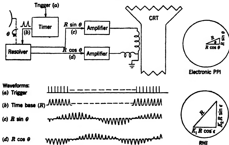
FIG. 12-3.—Electronic PPI and RHI.
