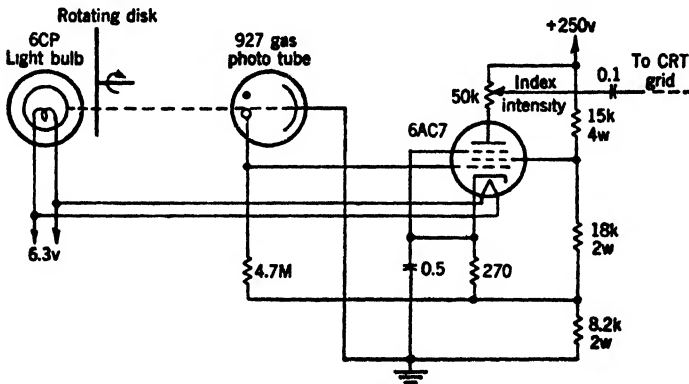
FIG. 13-33.—Photocell index circuit.
