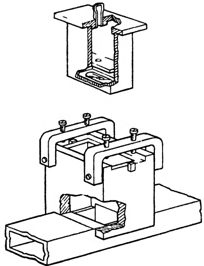
FIG. 11-18.—1B35 broadband ATR tube and mount; 3-cm band.
