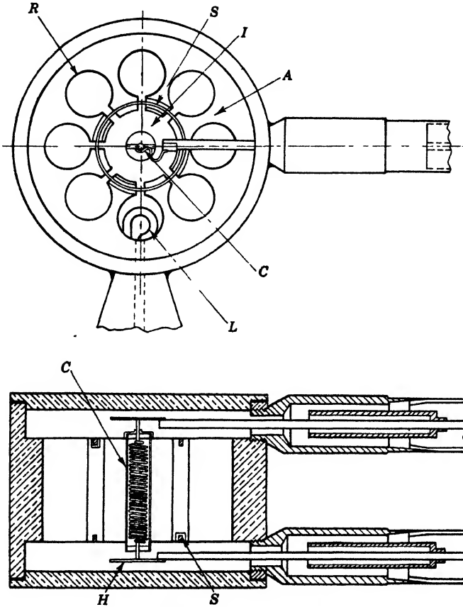
FIG. 10-1.—A typical cavity magnetron.
