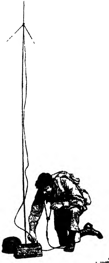
FIG. 8-5.--The AN/PPN-2 beacon. The AN/PPN-2 is a 1.5-m beacon designed for use principally by paratroops.
