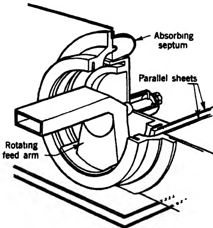
FIG 9-31.—Detail of radial feed horn.
