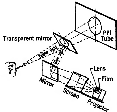
FIG. 7-1.—Schematic diagram of chart projector.
