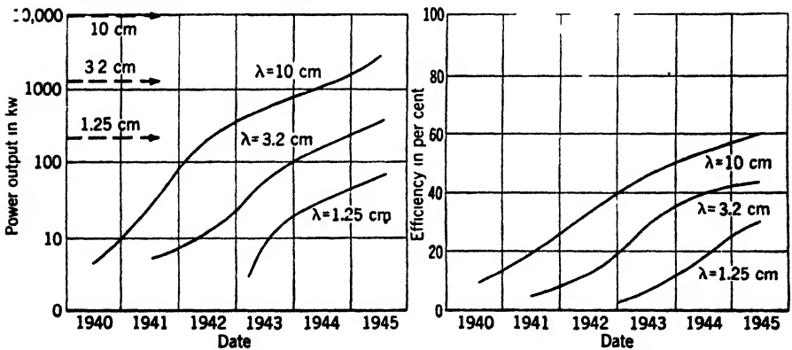
FIG. 1.5.—Historical development of microwave magnetrons.
