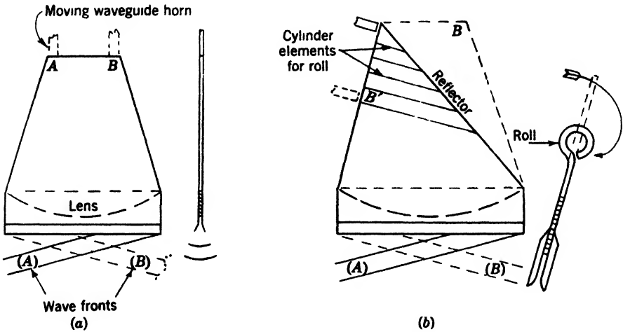
FIG. 9-34 Reflector roll scanner
