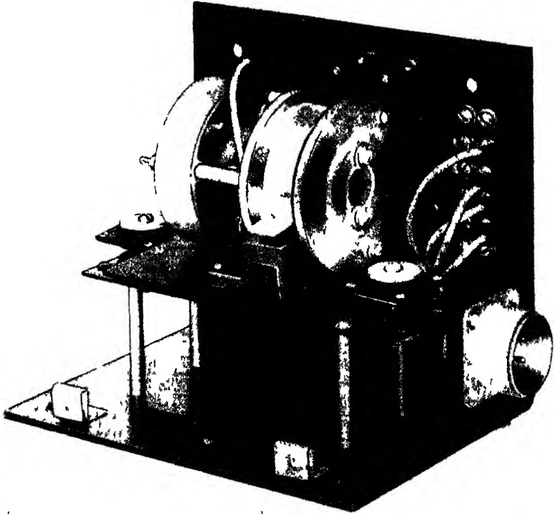
FIG. 14-12.—Typical vibration mount for voltage regulator.
