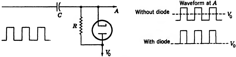
FIG. 13-20.—D-c restorer.
