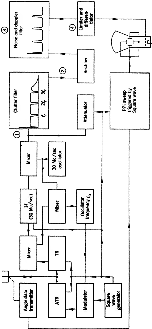
FIG. 5-15.—Block diagram of pulse-modulated doppler system.
