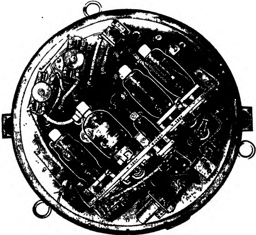
FIG. 10 48 —Medium-power airborne pulser.
