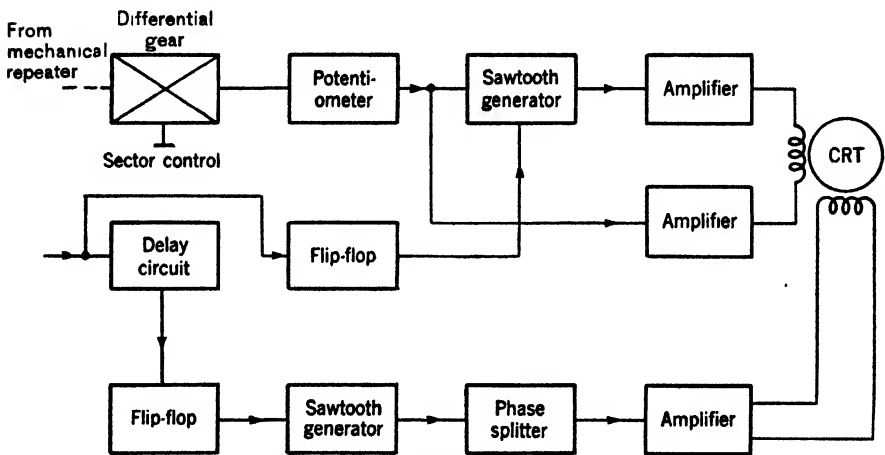
FIG. 13-53.—V-beam height indicator.
