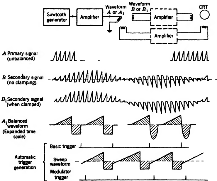
FIG. 13-45.—Resolved-sweep PPI methods
