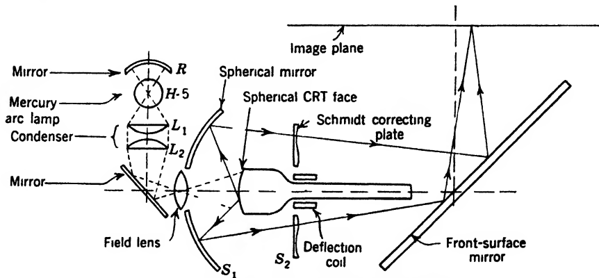
FIG. 7-6.—Schmidt projection system for skiatron.
