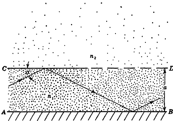
FIG. 2-15.—Propagation within a duct (oversimplified).
