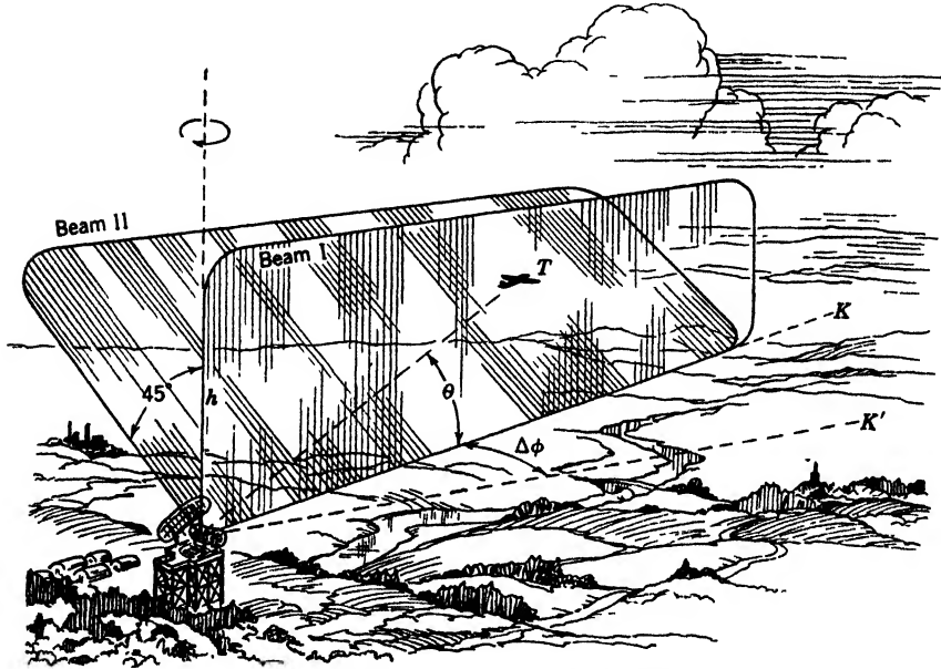
FIG. 4-1.—Principle of V-beam height measurement.
