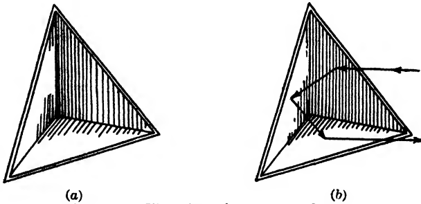
FIG. 3-2.—The triangular corner reflector.
