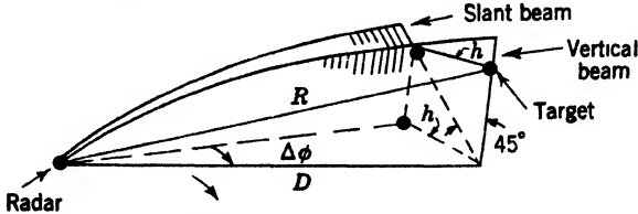
FIG. 6-26.—Schematic view of V-beam principle. For clarity, vertical and slant beams are shown without the 10^\circ separation in azimuth which is used in practice.
