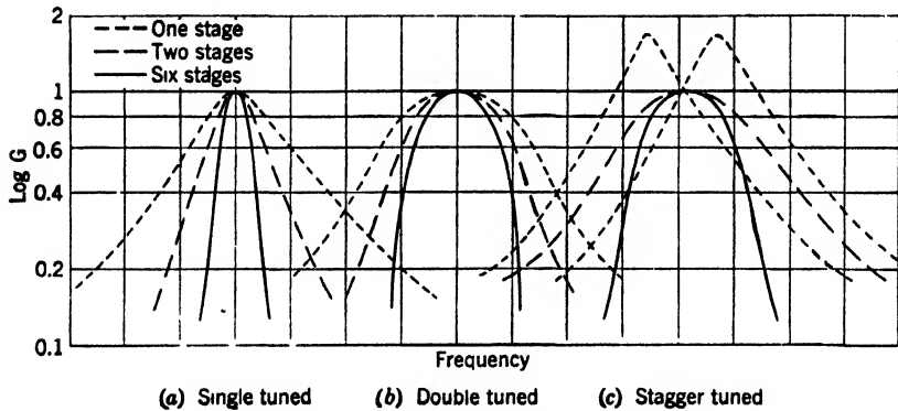
FIG. 12-8.—Amplifier response curves.
