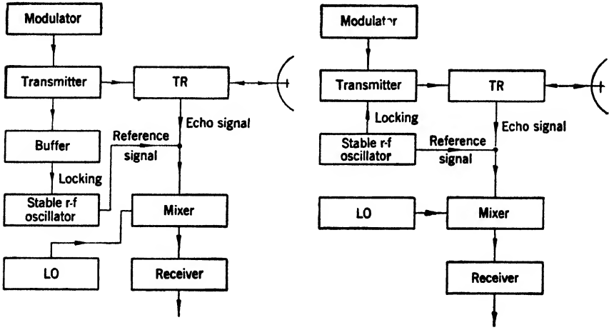
FIG. 16-14.—R-f locking, r-f addition. (a) R-f locking by transmitter, r-f addition. (b) R-f locking by oscillator, r-f addition.
