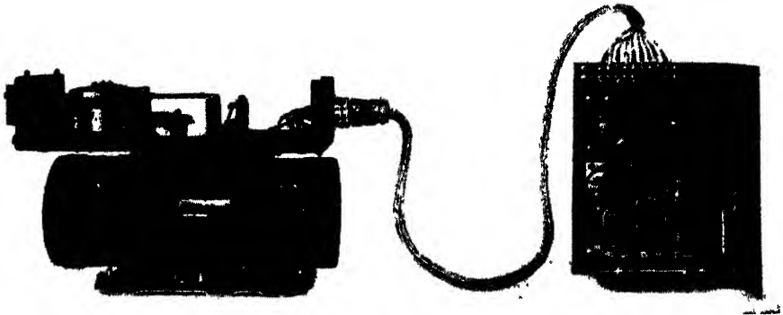
FIG. 14-8.—General Electric 1500-va aircraft inverter type PE-218-D, 115 volts, 400 cps, and electronic voltage regulator.
