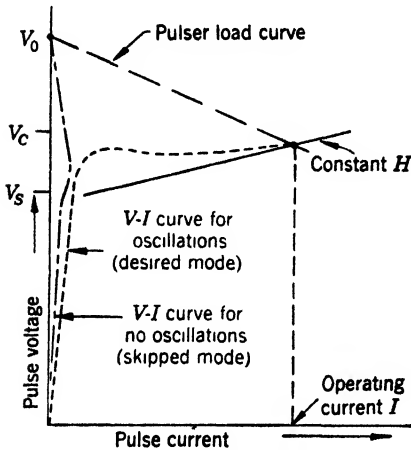
FIG. 10-25.—V-I plot of a magnetron illustrating the problem of mode skipping. V_s = magnetron starting voltage V_c = critical voltage above which oscillations will not start V_0 = pulser voltage with no load.
