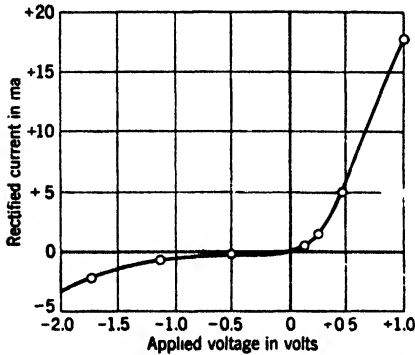
FIG. 11-20.—Typical characteristic curve of a silicon rectifier.
