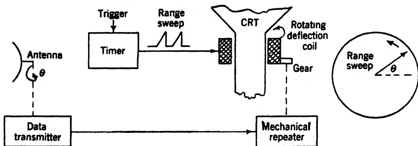
FIG. 12-2.—Rotating-coil PPI.
