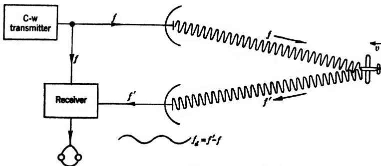
FIG. 16-3.—Doppler effect with c-w system.
