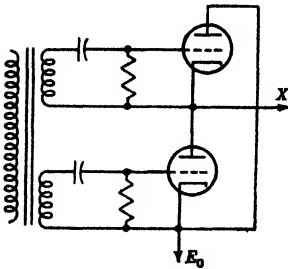
FIG. 13-26.—Two-way double-triode clamp with transformer-coupled switching.
