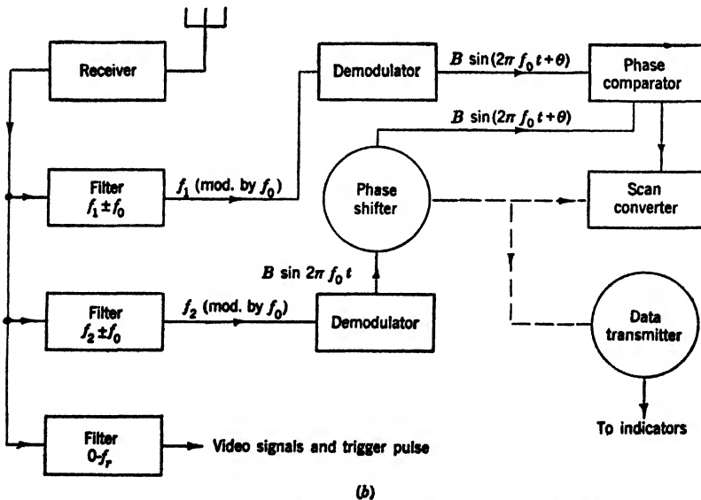
FIG. 17-6.—Phase-shift data transmission using two c-w subcarriers.
