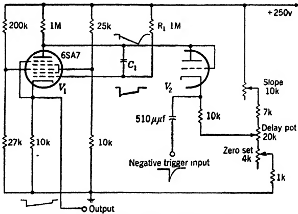
FIG. 13-17.—Phantastron delay circuit.
