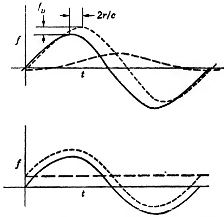
FIG. 5-14.—The full curve in the upper graph shows the instantaneous transmitter frequency as a function of time; the dotted curve shows the received signal; and the dashed curve, the beat between the two. The lower curve shows the same quantities when 2r/c = n f_r , in which case the beat frequency is constant at the doppler value.
