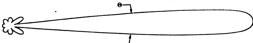
FIG. 9-1.—A typical antenna pattern showing the main beam of width \theta and the side lobes. shows that the beamwidth \theta is the full beamwidth at half power. A small amount of power is unavoidably radiated in undesired directions, forming the "side lobes" shown in this figure.
