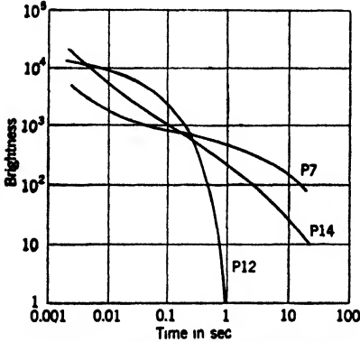
FIG. 13-4.—CRT screen characteristics.
