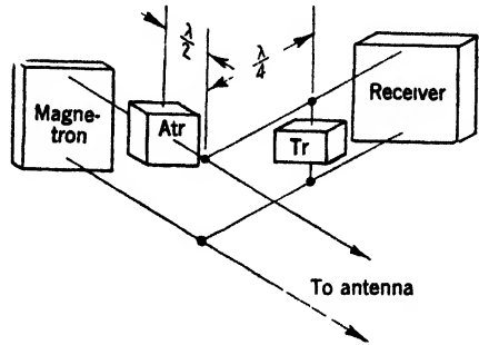
FIG. 11-14.—Duplexing system on two-wire transmission line.
