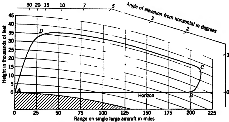
FIG. 15-4.—Desirable coverage for long-range air-surveillance radar.
