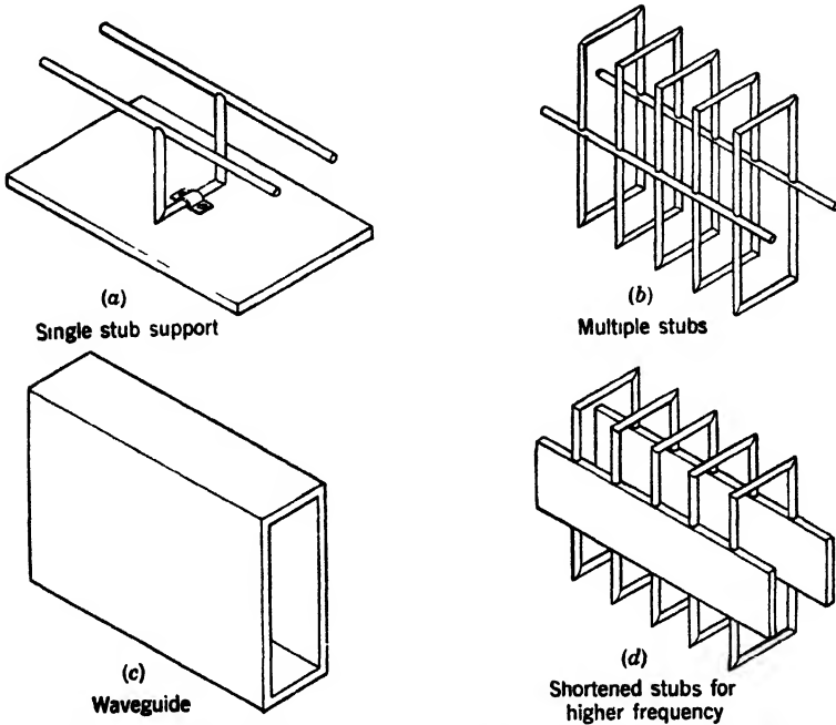
FIG. 11-8.—Waveguide derived from stub-supported two-wire transmission line.
