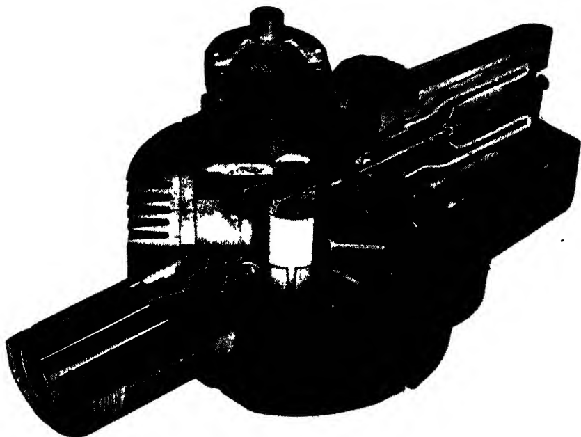
FIG 10 22 —Cutaway view of a 1000-Mc/sec tunable magnetron showing the C-ring tuning mechanism and the slot-type resonators (Courtesy of Bell Telephone Laboratories.)
