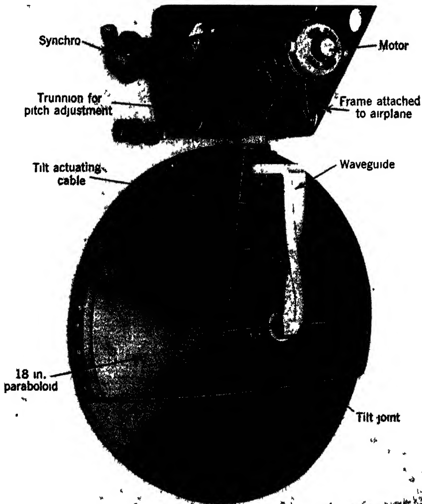
FIG 9 16 — The AN/APS-10 airborne navigation scanner with an 18-in reflector (Courtesy Houston Corporation)
