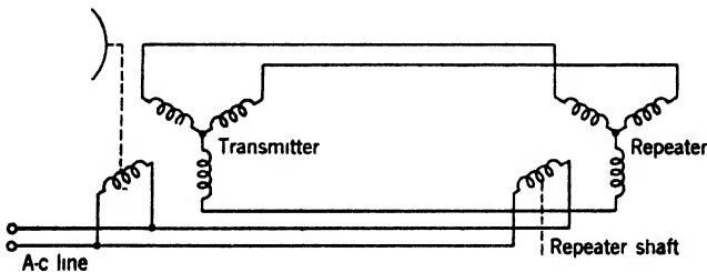
FIG. 13-8.—Synchro-driven repeater.
