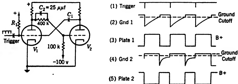
FIG. 13-14.—Eccles-Jordan flip-flop.
