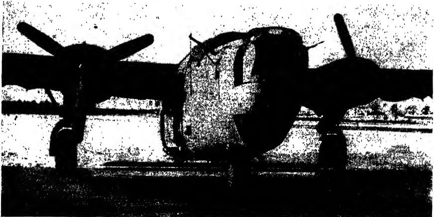
FIG. 9-18.—AN/APQ-7 antenna housing on a B-24.
