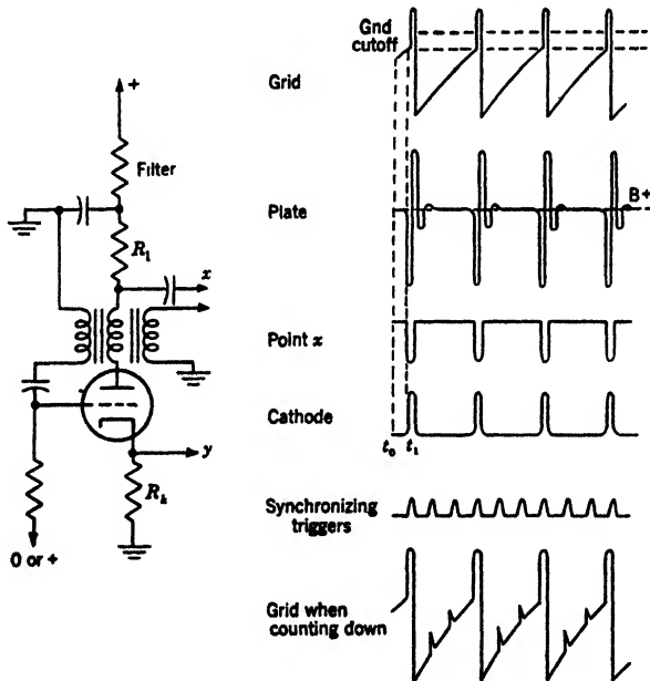
FIG. 13-19.—The blocking oscillator.
