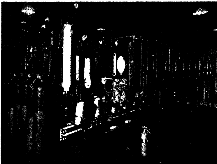
FIG. 8. Catalyst testing units in Bureau of Mines Fischer-Tropsch laboratory, showing recording and indicating flowmeters. (Courtesy of H. H. Storch, U.S. Bureau of Mines.)
