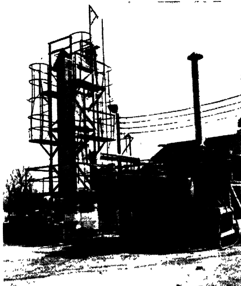
FIG. 6. Synthesis-gas pilot plant unit, using natural gas. (Courtesy of Phillips Petroleum Co.)
