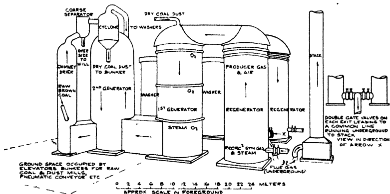
FIG. 5. Schmalfeldt-Wintershall synthesis gas unit. (Simplified but roughly to size.)
