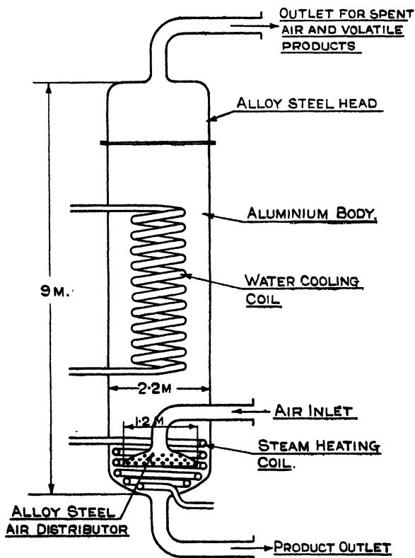
FIG. 15. German wax oxidation kettle for the production of fatty acids.
