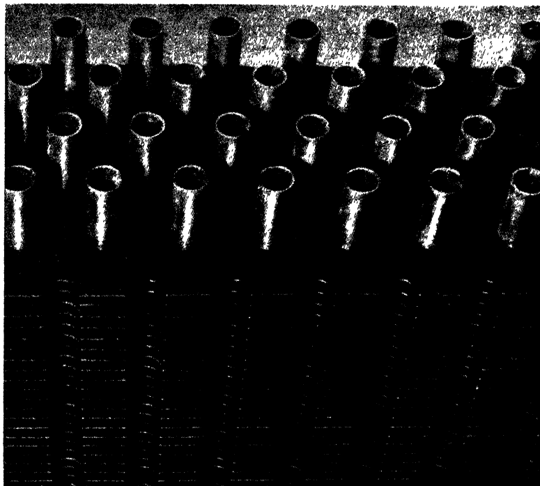
FIG. 9. Section of Ruhrchemie A.-G. finned tube atmospheric pressure converter. (Courtesy of H. H. Storch, U.S. Bureau of Mines.)
