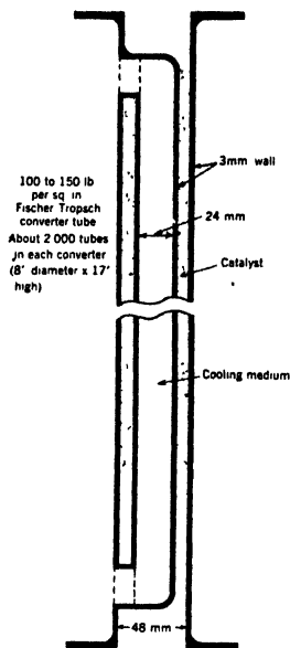
FIG. 10. Section of Middle-Pressure Ruhrchemie Synthine reactor tube. (Courtesy of H. H. Storch, U.S. Bureau of Mines.)
