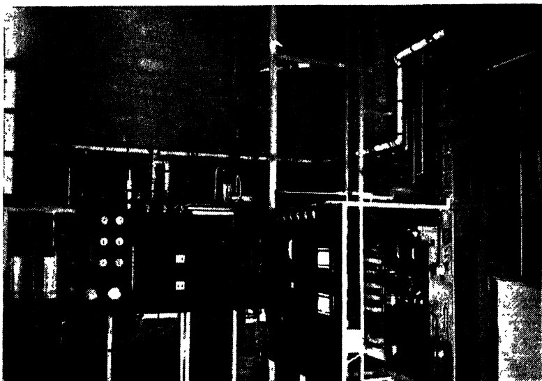
FIG. 19. Internally-cooled, experimental Fischer-Tropsch plant of Bureau of Mines. (Courtesy of H. H. Storch, U.S. Bureau of Mines.)
