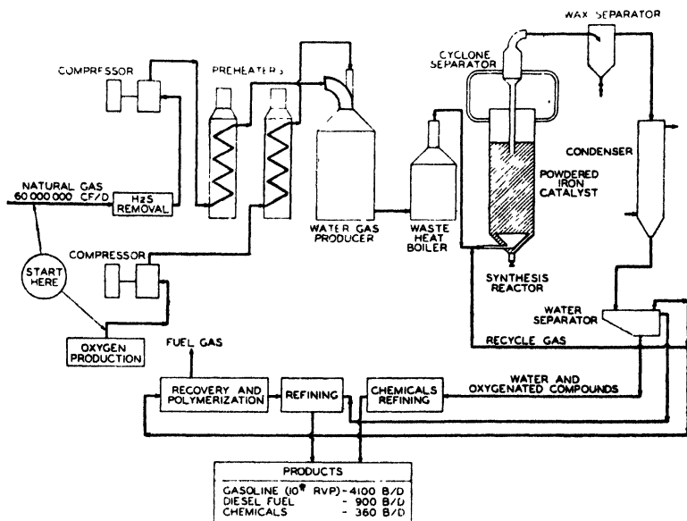
FIG. 18. Flow diagram of the conversion of natural gas to motor fuel.
