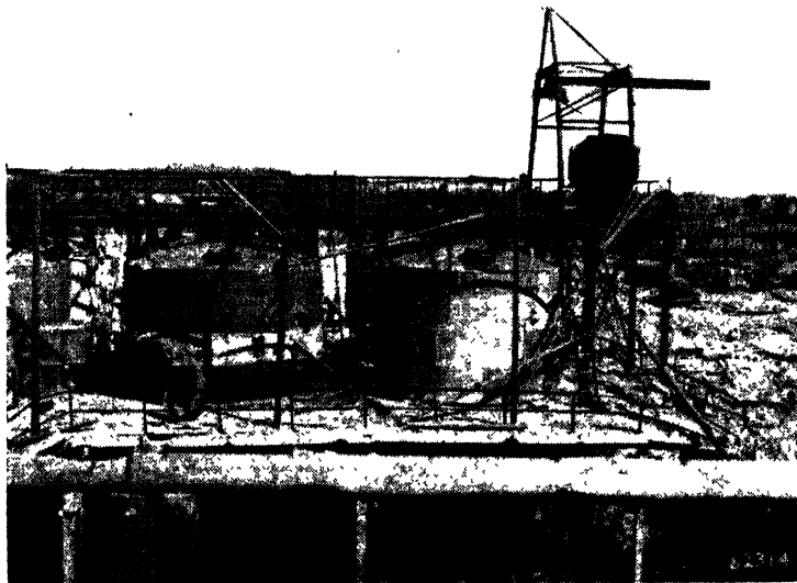
FIG. 12. Charcoal absorption plant for Fischer-Tropsch gasoline recovery. Such plants were used extensively by the Germans. (Courtesy of W. C. Schroeder, U.S. Bureau of Mines.)
