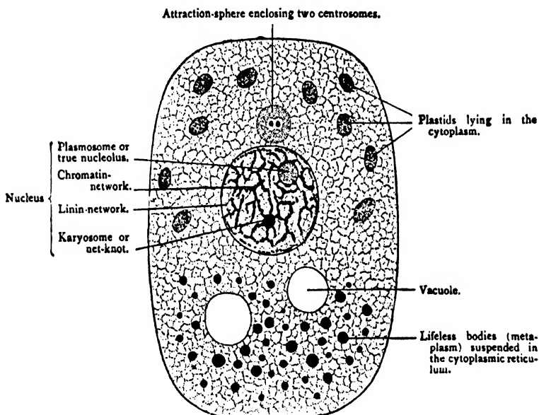
Diagrammatic representation of the structures present in a typical cell. (After Wilson.)
