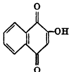
Lawson
