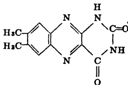
6,7-Dimethylalloxazine
