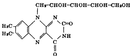
Lactoflavin
