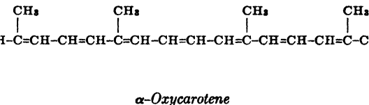
\alpha -Oxycarotene
