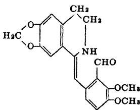
Aldehyde form
