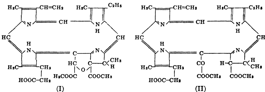
Purpurin 7
