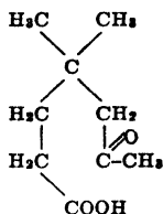
Isogeronic acid
