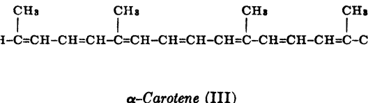
\alpha -Carotene (III)
