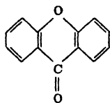
Xanthone
