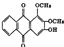
Ether B
