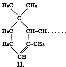
Isogeronic acid
