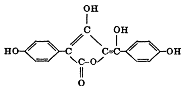
Lactone of atromentic acid
