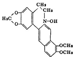
Ammonium form
