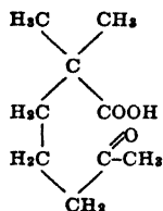
Geronic acid
