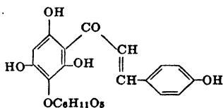
Isocarthamin
