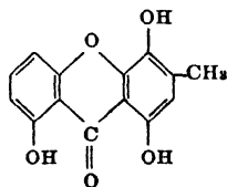
Ravenilin
