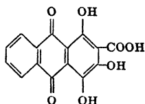
Pseudopurpurin
