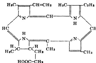
Phyllochlorin
