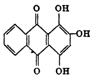
Purpurin
