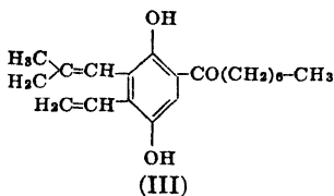
Flavoglaucin
