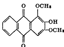
Anthragallol dimethyl ether A
