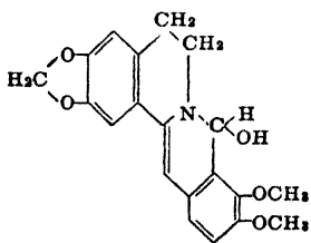
Carbinol form
