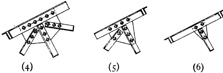
RAFTER AND STRUT JOINTS
