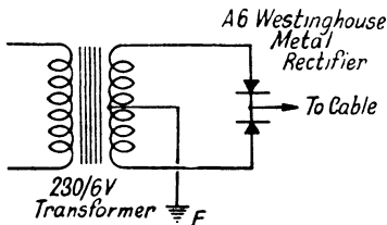
FIG. 133. DOUBLE-FREQUENCY RECTIFICATION
