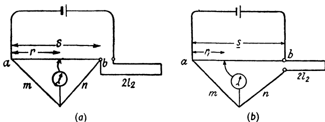
FIG. 83. CALIBRATION OF PILOT WIRE IN SLIDE WIRE DIVISIONS
