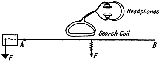
FIG. 129. SIMPLE SEARCH COIL METHOD
