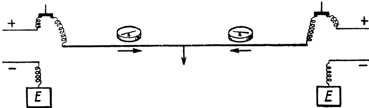
FIG. 135. COMPASS METHOD ON D.C. CABLES
