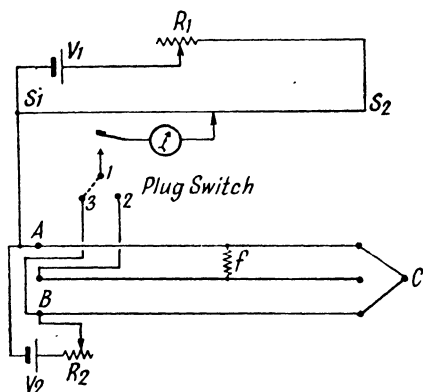
FIG. 106B. POTENTIOMETER METHOD WITH FAULT BETWEEN TWO CORES OF A THREE-CORE CABLE
