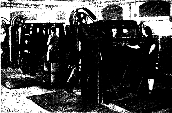
FIG. 138. GROUP OF SPARK TESTING SETS IN FACTORY
