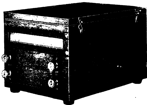
FIG. 13. ONWOOD SELF-CONTAINED PORTABLE REFLECTING GALVANOMETER
