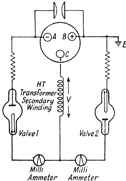
FIG. 37. TWO-VALVE RECTIFICATION
