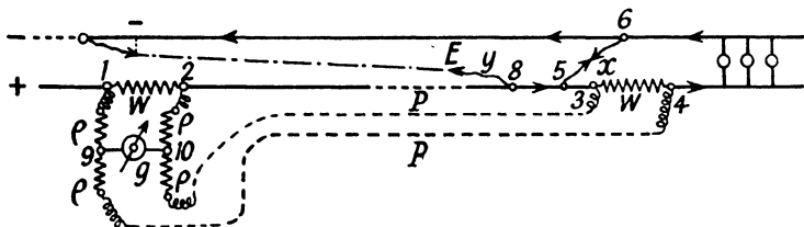
FIG. 49. INSULATION TEST OF FEEDERS
