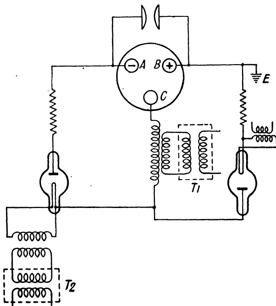
FIG. 39. CALLENDER-SMITH CONNECTION
