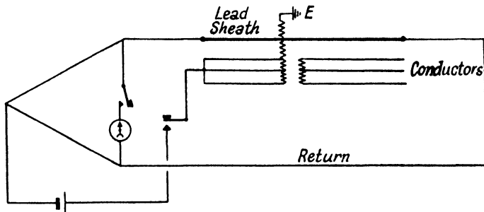
FIG. 94. LOOP TEST ON LEAD SHEATH
