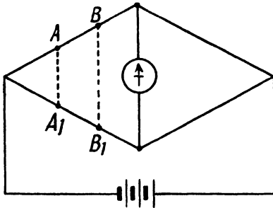
FIG. 87. EQUIPOTENTIAL POINTS ON WHEATSTONE BRIDGE
