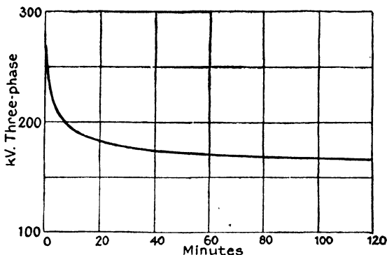
FIG. 5. TYPICAL TIME-BREAKDOWN CURVE
